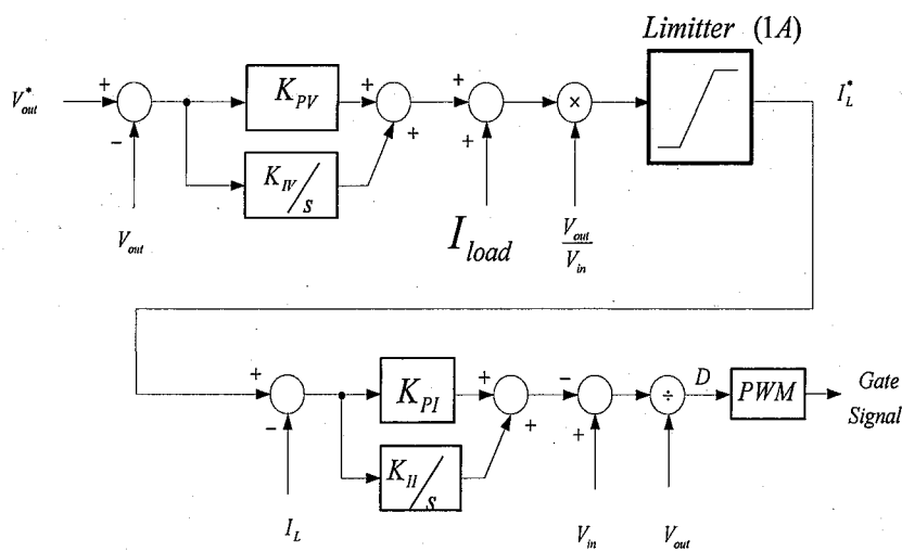
Fig. 4.2 Control block of the boost chopper.
