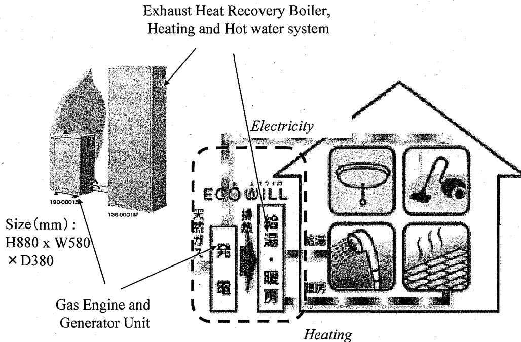
Fig. 1.3 the gas engine cogeneration system (GECS)
