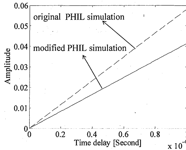
Fig. 3.14 E_{VI-TFP} versus time delay for original and modified PHIL simulation.
