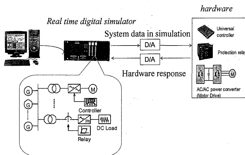
Fig.1.1 Configuration of a HIL simulation.
