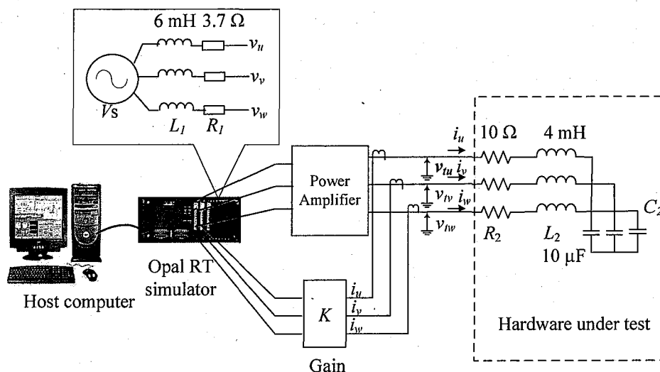
Fig. 3.3 a PHIL simulation of inductor coupled system.
