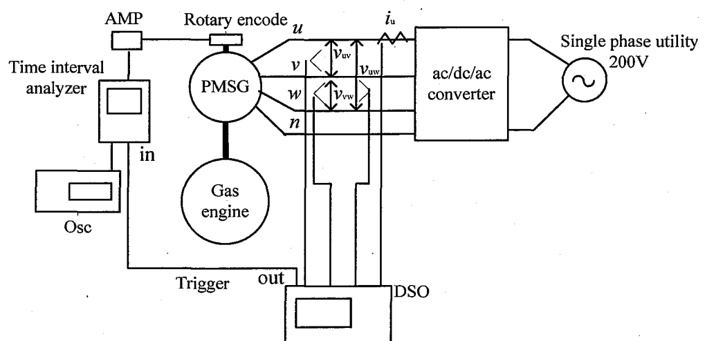
Fig. 2.6 Experimental setup.
