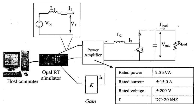
Fig. 4.3 PHIL for chopper.
