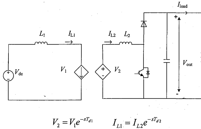
Fig. 4.7 Offline simulation of PHIL based on PSCAD/EMTDC
