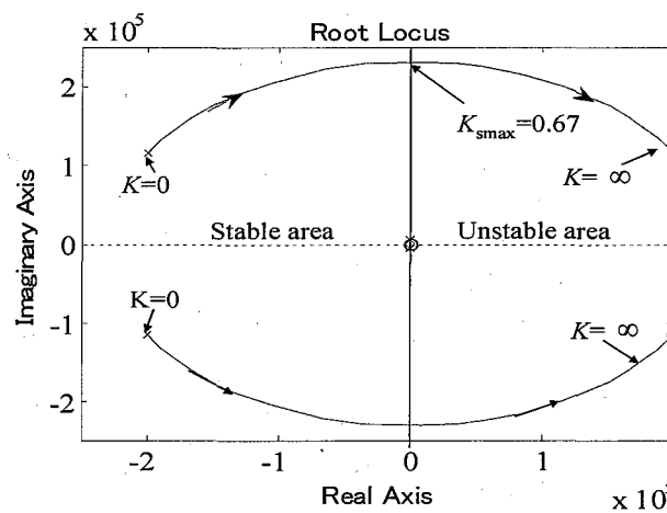
Fig. 3.6 Root locus figure of the closed-loop PHIL simulation with time delay.
