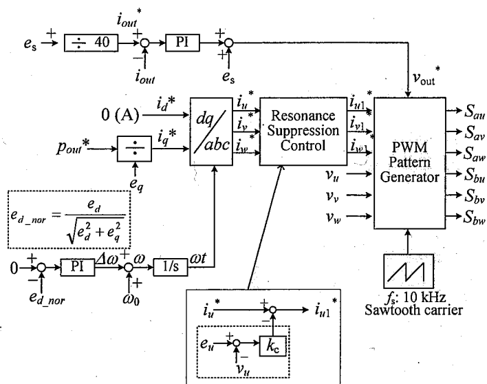
Fig. 2.12 Control block diagram of the matrix converter.
