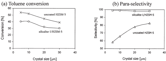
Fig. 3 Toluene conversion and p -xylene selectivity in toluene alkylation as a function of crystal size of the zeolite catalysts. T=673\text{K} , W/F=0.14 [kg-cat h mol -1 ], [MeOH]/[toluene] = 1.0, Reaction time = 60 min.
