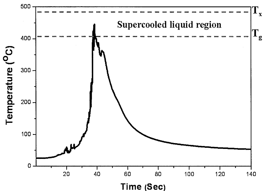
Fig. 4.9 Temperature profile of the bottom of between BMG and Al during friction stir welding (400rpm, 100mm/min).
