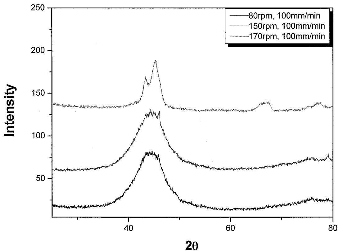
Fig. 3.4 X-ray diffraction patterns of the stir zone.
