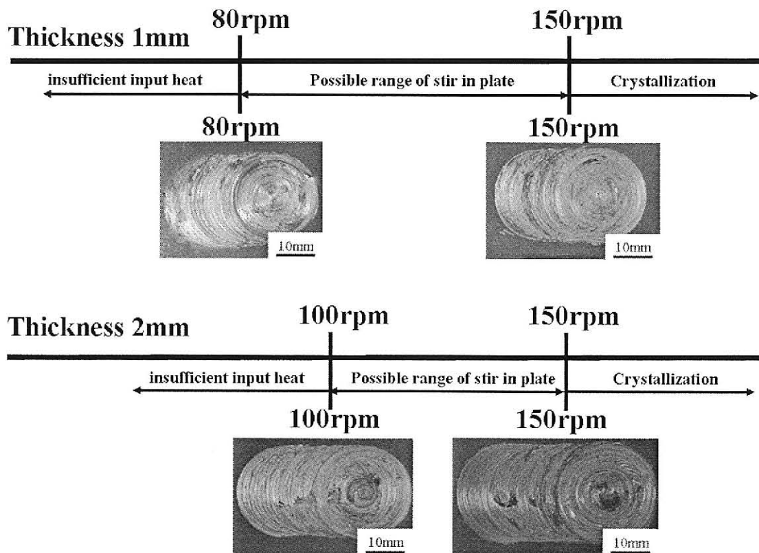
Fig. 3.11 Possible welding range and surface appearance for 1 mm and 2mm thick \text{Zr}_{55}\text{Cu}_{30}\text{Al}_{10}\text{Ni}_5 Bulk metallic glass.
