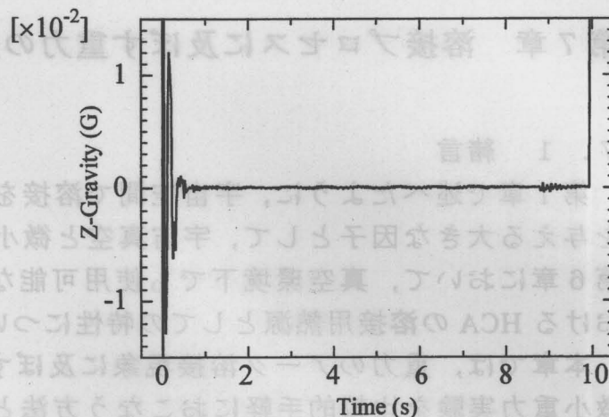
Fig.7.2 Change of Z-gravity by drop tower
