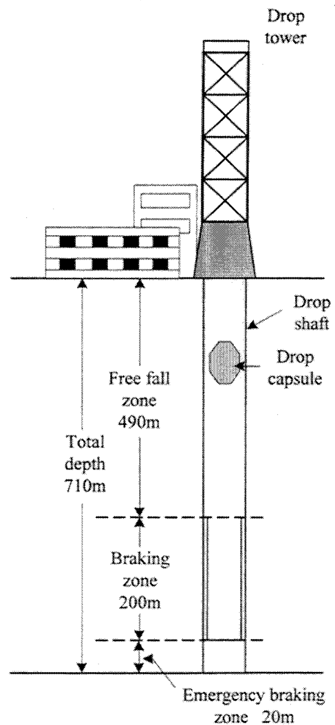
Fig.7.1 Schematic of the Japan Microgravity Center (JAMIC)
