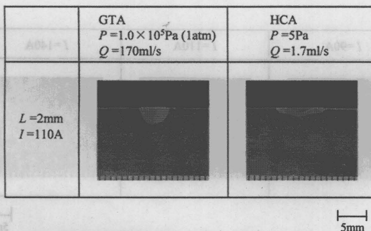
Fig.3.4 Penetrations in GTA and HCA melting HCA: hollow tungsten cathode ( D=4.0\text{mm} , d=1.8\text{mm} )
