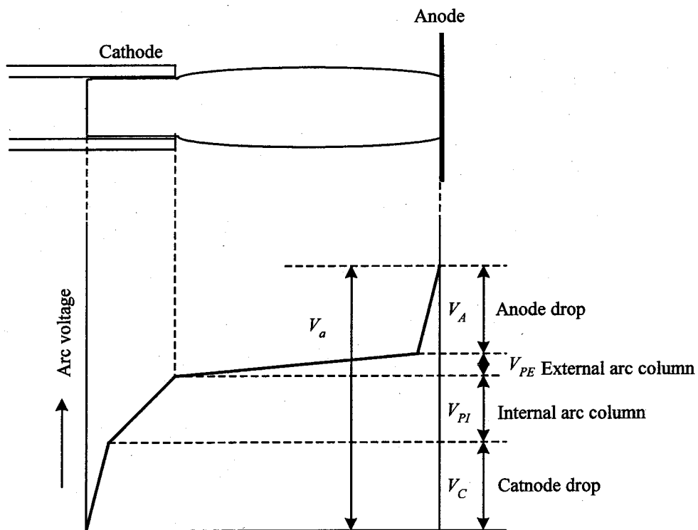
Fig.2.14 Schematic diagram of the potential distribution on the axis of HCA
