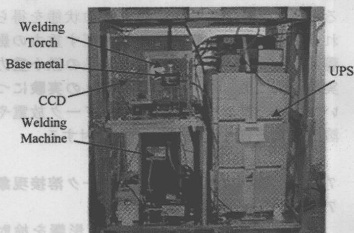
Fig.7.3 Experimental apparatus
