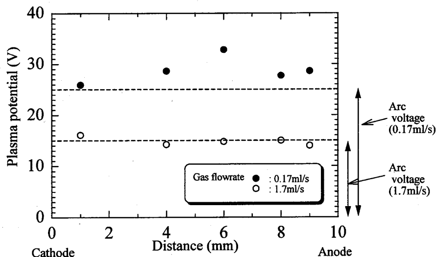
Fig.4.14 Plasma potential between electordes ambient pressure 5Pa, arc current 100A, arc length 10mm, anode Copper
