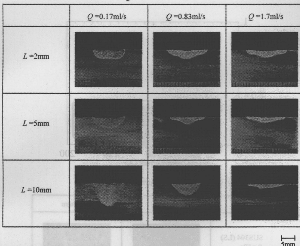
Fig.3.9 Effect of arc length and gas flow rate on penetration in HCA melting ambient pressure 5Pa, arc current 150A hollow tantalum cathode( D=4.0\text{mm} , d=3.4\text{mm} )
