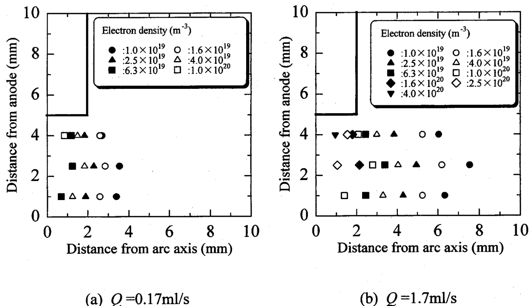
Fig.4.8 Electron density distribution between electrodes: ambient pressure 5Pa, arc current 100A, arc length 5mm, anode Copper
