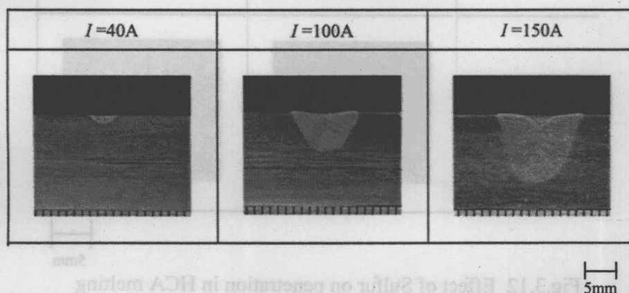
Fig.3.10 Effect of arc current on penetration in HCA melting: ambient pressure 5Pa, arc length 10mm, gas flowrate 0.17ml/s hollow tungsten cathode( D=4.0\text{mm} , d=3.0\text{mm} )
