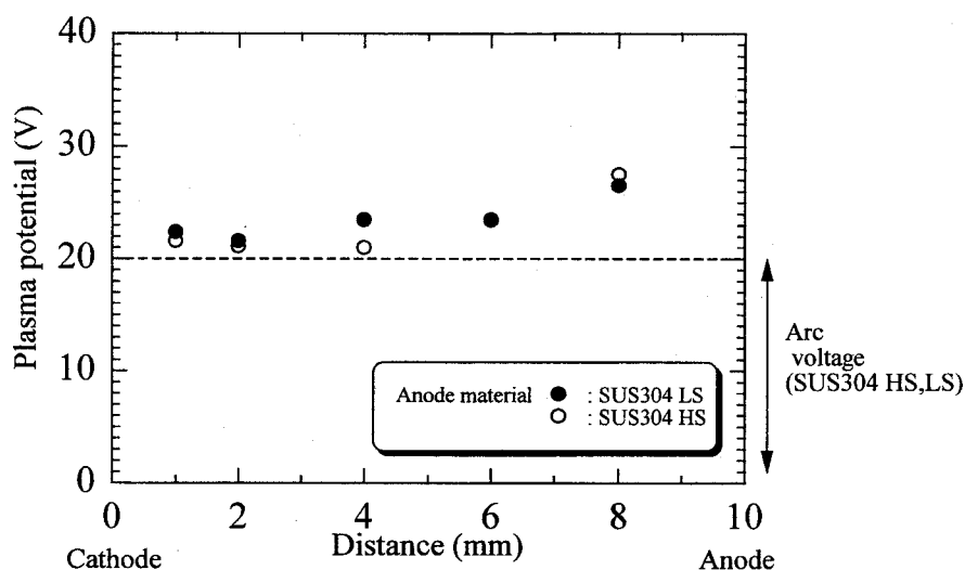
Fig.4.15 Plasma potential between electordes ambient pressure 5Pa, arc current 100A, arc length 10mm, gas flowrate 0.17ml/s, anode SUS304
