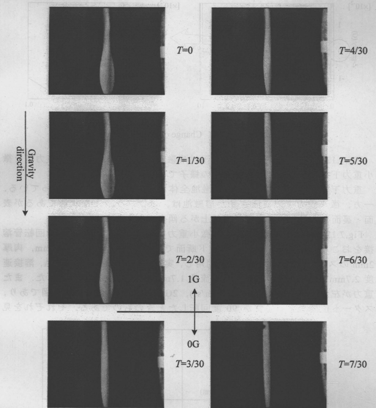
Fig.7.10 Change of molten pool profile with gravity (GTA, I=80A , L=2mm , Q=170ml/s )
