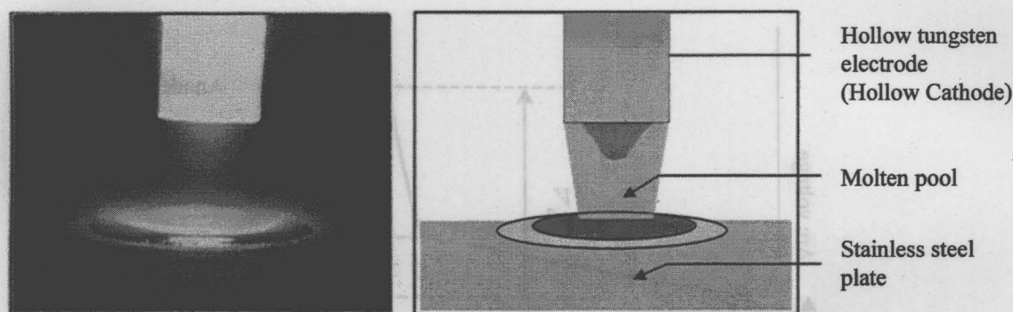
Fig.2.12 Photograph and schematic diagram of HCA. ( P=5\text{Pa} , I=150\text{A} , L=5\text{mm} , Q=1.7\text{ml/s} )
