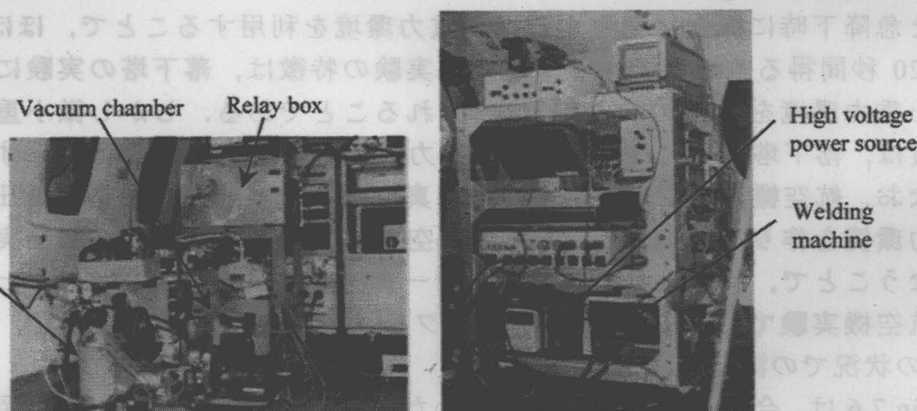
Fig.7.7 Pictures of experimental apparatus in flying laboratory
