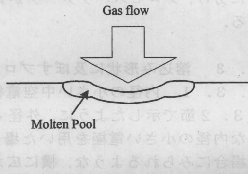
Fig.3.5 Effect of gas flow on penetration in HCA melting
