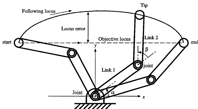
Fig. 4.3 Locus error of an industrial articulated robot arm of two-degree-of-freedom; bold line: links of the robot arm, \odot : joints of the robot arm, (\alpha, \beta) : joint angle.
