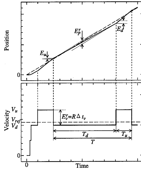
Fig. 2.5 Deterioration of ramp response
