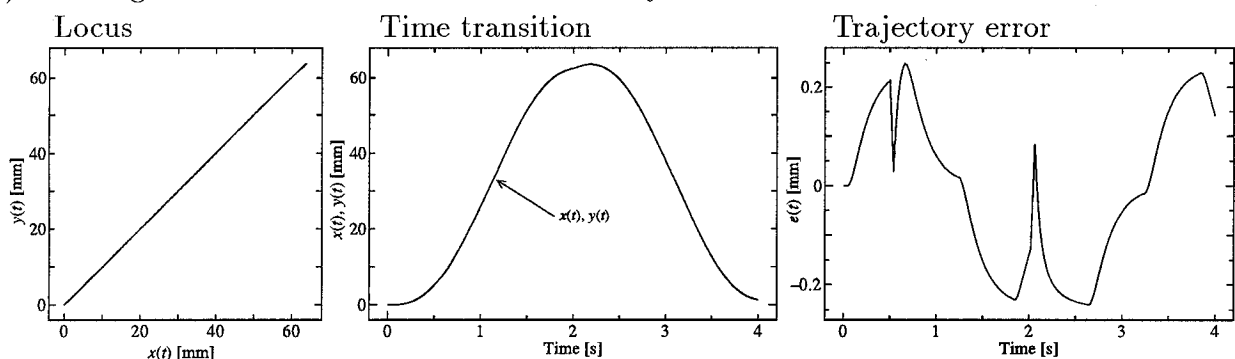
Fig. 8.5 Simulation results of the XY table equipment under the step disturbance.
