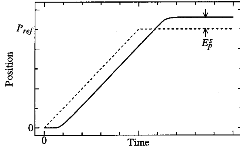
Fig. 2.4 Deterioration of positioning of the software servo system.
