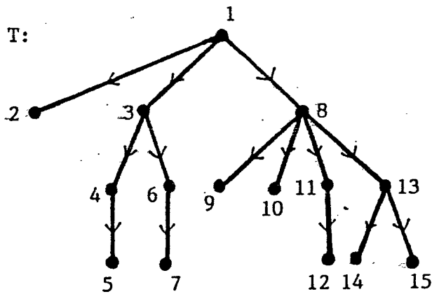
(a) A given 4-ary tree T.
