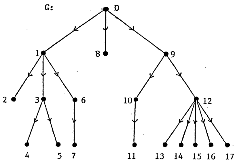
(a) The depth-first-order of G.
