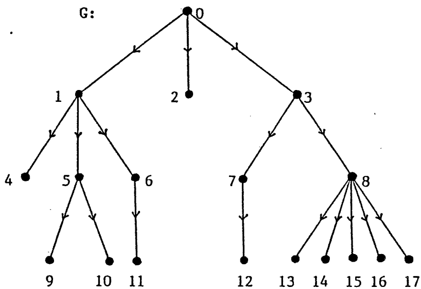
(b) The breadth-first-order of G.
