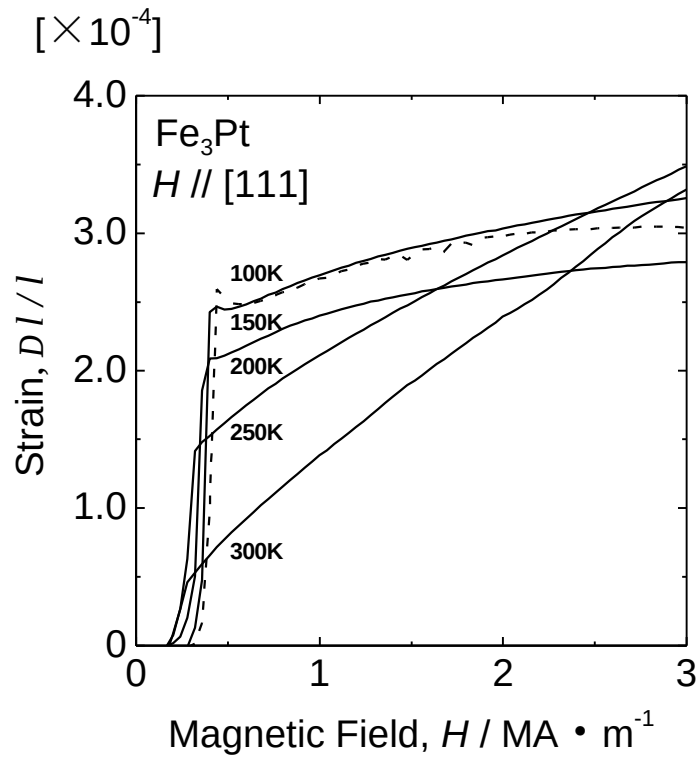
Fig. 2-20 Temperature dependence of magnetostriction due to dipole-dipole interaction of Fe 3 Pt under the [111] magnetic field. The contribution of the forced volume magnetostriction is included after the magnetization is saturated.
