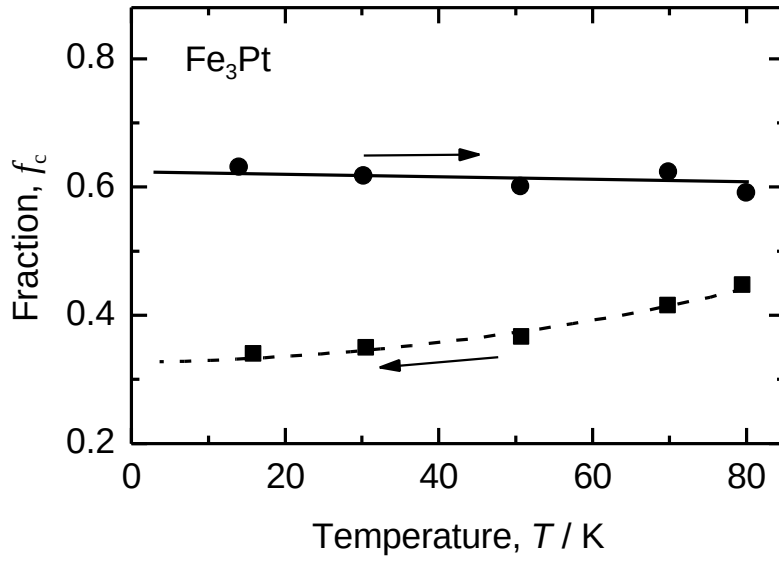
Fig. 5-3 Temperature dependence of the fraction of the variants whose c axis lies along [001]_p in the zero-field-cooling process (broken line) and the zero-field-heating process (solid line). Lines are guides for eyes.
