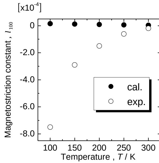
Fig. 2-23 Temperature dependences of the experimental and the calculated magnetostriction constants of \text{Fe}_3\text{Pt} under the [100] field.
