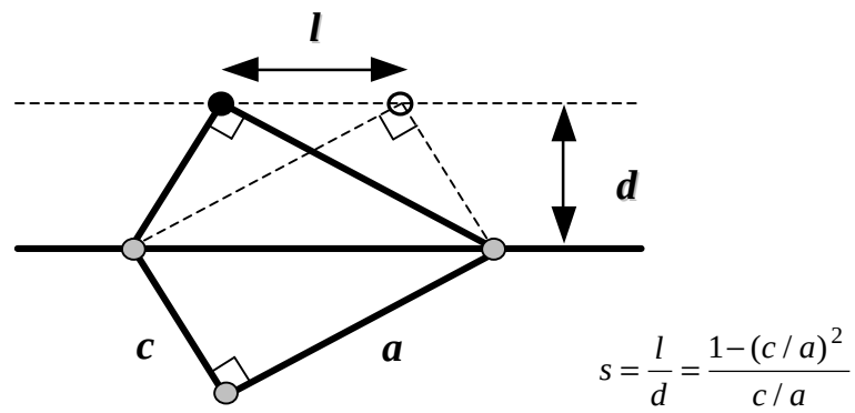
Fig. 7-10 The method for the calculation of the twinning shear.
