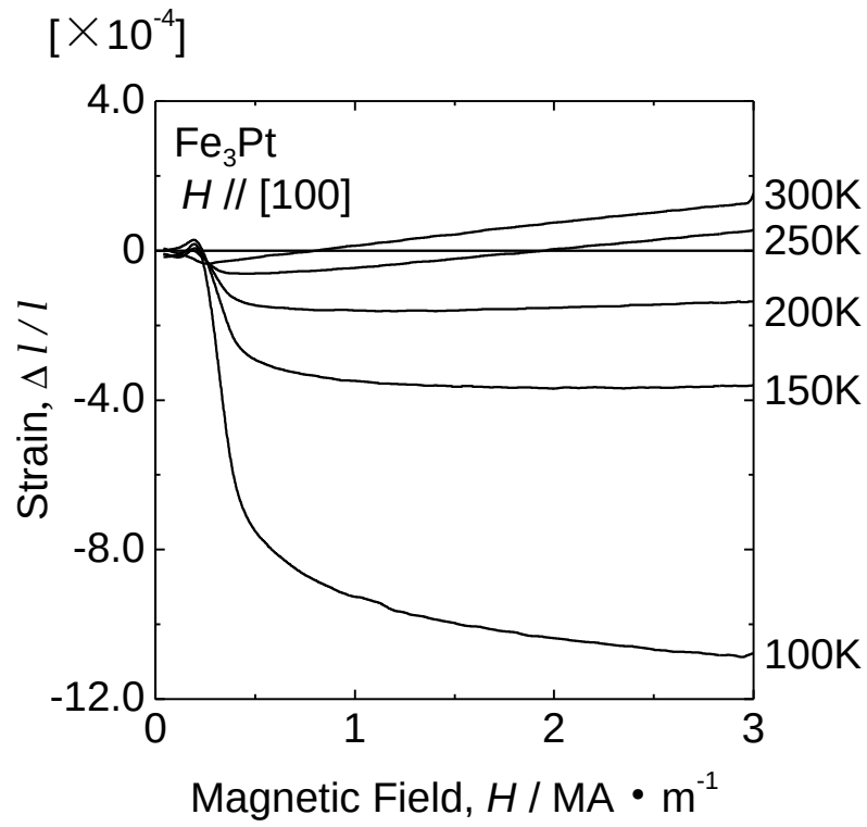
Fig. 2-19 Temperature dependence of magnetostriction due to dipole-dipole interaction of Fe 3 Pt under the [100] magnetic field. The contribution of the forced volume magnetostriction is included after the magnetization is saturated.
