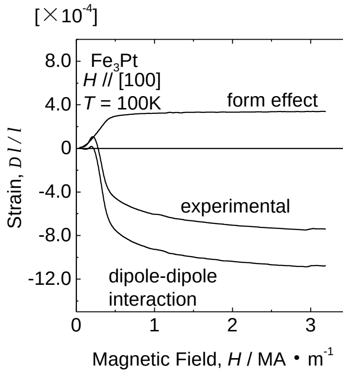
Fig. 2-16 Evaluation of magnetostriction due to dipole-dipole interaction by subtracting the form effect from the experimental data of Fe 3 Pt at 100 K.
