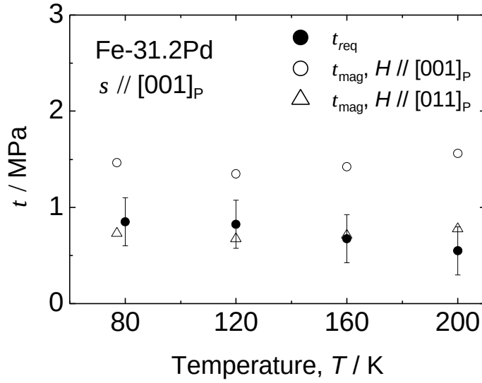
Fig. 8-6 Temperature dependence of the maximum magnetic shear stress, t_{\text{mag}} , and the twinning shear stress, t_{\text{req}} .
