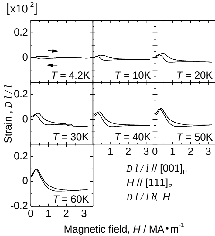
Fig. 6-10 Temperature dependence of the recoverable strain of an \text{Fe}_3\text{Pt} single crystal under the [111]_p field. The strain was measured along [001]_p .
