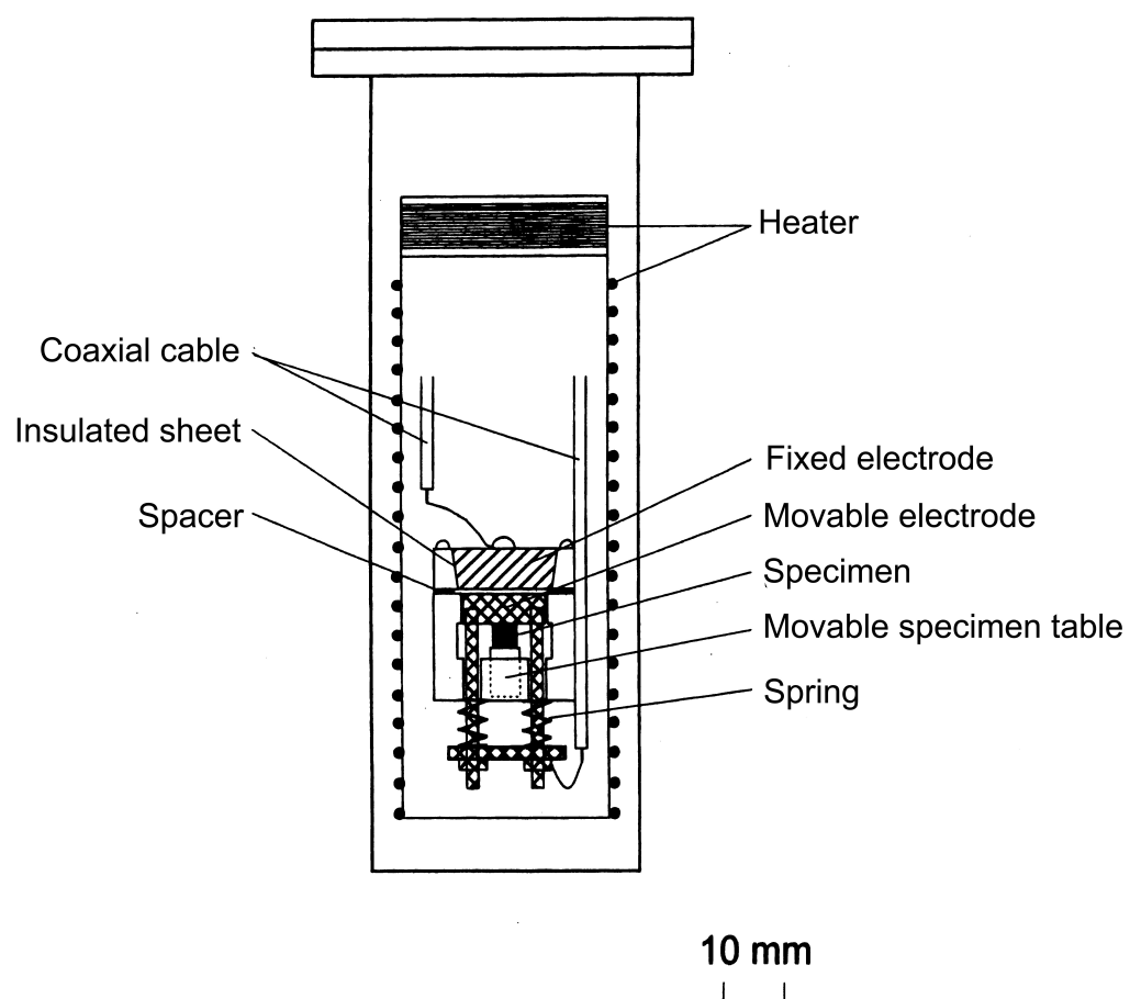
Fig. 3-2 Schematic illustration of the capacitance cell and the cryostat.
