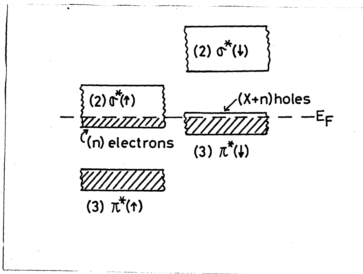
Fig. 28 Band model for (\text{La}_{1-x}\text{Sr}_x)\text{CoO}_3 .
