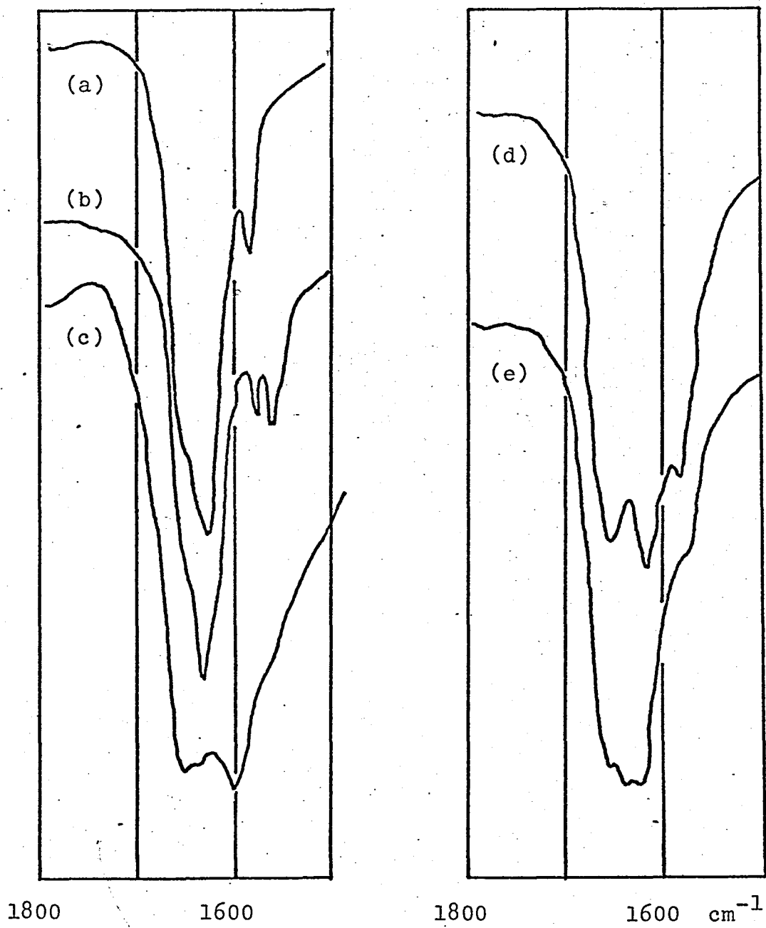
Figure 23. Infrared spectra of the isomers of [\text{Co}(\text{acms})_2]\text{Cl} in the antisymmetric COO stretching band region; (a) tr.tr.tr., (b) trans(O), (c) trans(S), (d) cisciscis and (e) trans(N).
