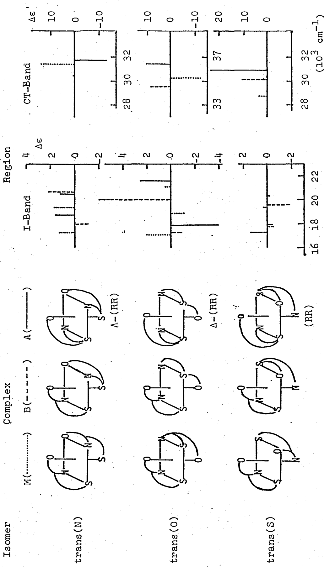
Figure 36. Comparison of CD spectra between bis(tridentate) and mixed type complexes. A, B, and M denote the complexes of [\text{Co}(\text{acms})_2]^+ , [\text{Co}(\text{L-met})(\text{acms})]^+ and [\text{Co}(\text{L-met})_2]^+ , respectively.
