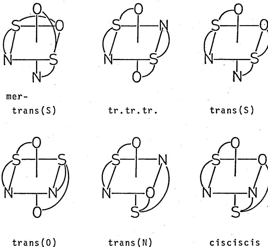
Figure 3. Six possible geometrical isomers for [\text{Co}(\text{N,S,O-tridentato})_2]^+ type complexes.
