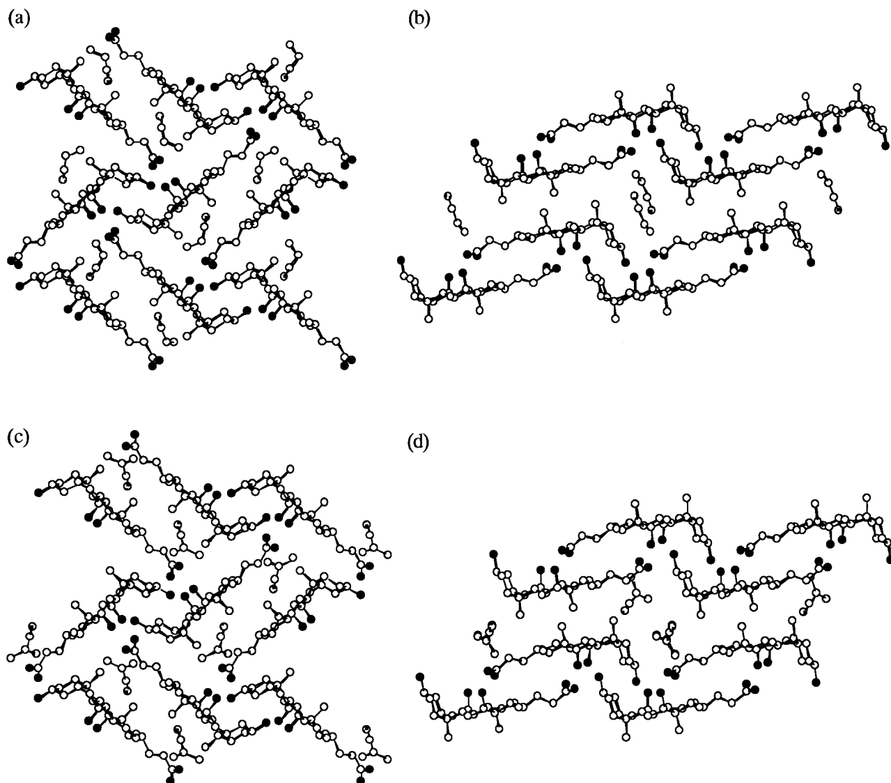
Figure 4-11. Molecular packing diagrams of (a) a crossing structure of CA•185 , (b) a bilayer structure of CA•185 , (c) a crossing structure of CA•187 , and (d) a bilayer structure of CA•187 . The carbon, nitrogen, and oxygen atoms are represented by open, dotted, and filled circle, respectively.
