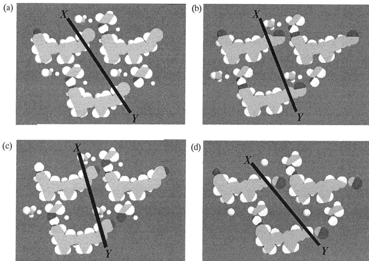
Figure 2-6. Cross sections of the host channels sliced perpendicular to the direction of the channel; (a) CA with 1 as a typical example for \alpha - gauche type, (b) CA with 3 as \beta - trans type, (c) CA with 5 as \beta - gauche type, and (d) CA with 57 as \alpha - trans type, respectively. The guest molecules are omitted. Carbon, hydrogen, and oxygen atoms are represented in gray, white, and black, respectively. The bold line of X-Y indicates the position sliced parallel to the direction of the channel which is shown in Figure 2-7.
