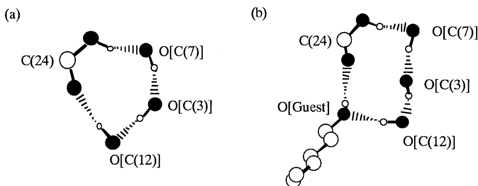
Figure 4-4. Hydrogen bond networks of typical bilayer structures of CA with (a) 113 , (b) 106 . Hydrogen atoms of a guest molecule are omitted for clarity. The carbon and oxygen atoms are represented by open and filled circle, respectively.
