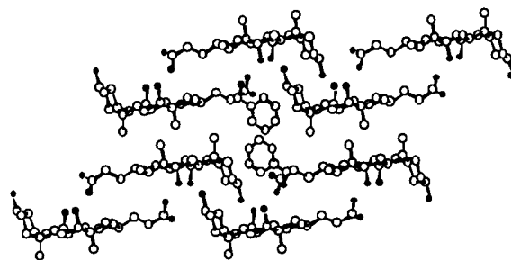
Figure 2-4. Molecular packing diagram of a \alpha - trans type inclusion crystal of CA with 57 . The figure is viewed down along the crystallographic b -axis. The carbon and oxygen atoms are represented by open and filled circle, respectively.
