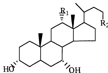
Chenodeoxycholic acid (CDCA) ; R_1=H R_2=CO_2H Methyl cholate (MCA) ; R_1=OH R_2=CO_2CH_3
