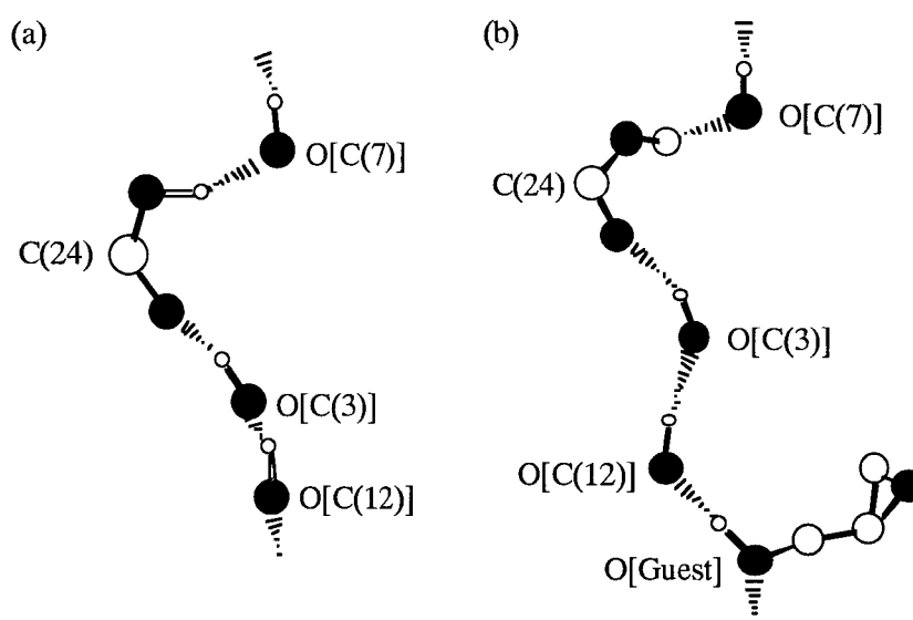
Figure 4-3. Hydrogen bond networks of typical crossing structures of CA with (a) 196 , (b) 82 . Hydrogen atoms of a guest molecule are omitted for clarity. The carbon and oxygen atoms are represented by open and filled circle, respectively.
