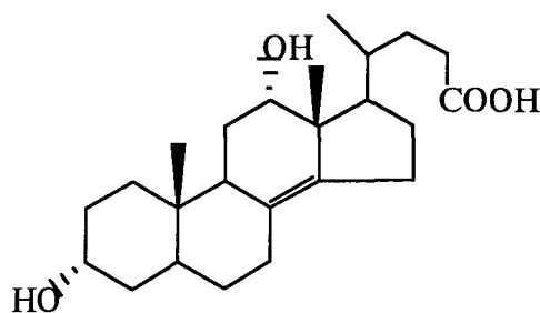
Apocholic acid (ACA)
