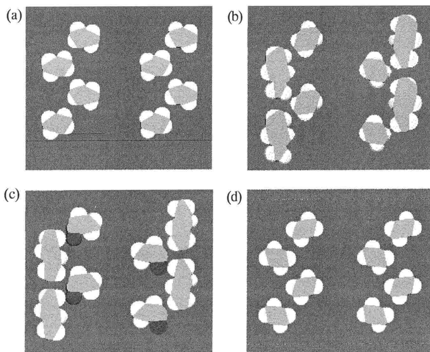
Figure 2-7. Cross sections of the host channels sliced parallel to the direction of the channel; (a) CA with 1 as a typical example for \alpha - gauche type, (b) CA with 3 as \beta - trans type, (c) CA with 5 as \beta - gauche type, and (d) CA with 57 as \alpha - trans type, respectively. The guest molecules are omitted. Carbon, hydrogen, and oxygen atoms are represented in gray, white, and black, respectively.
