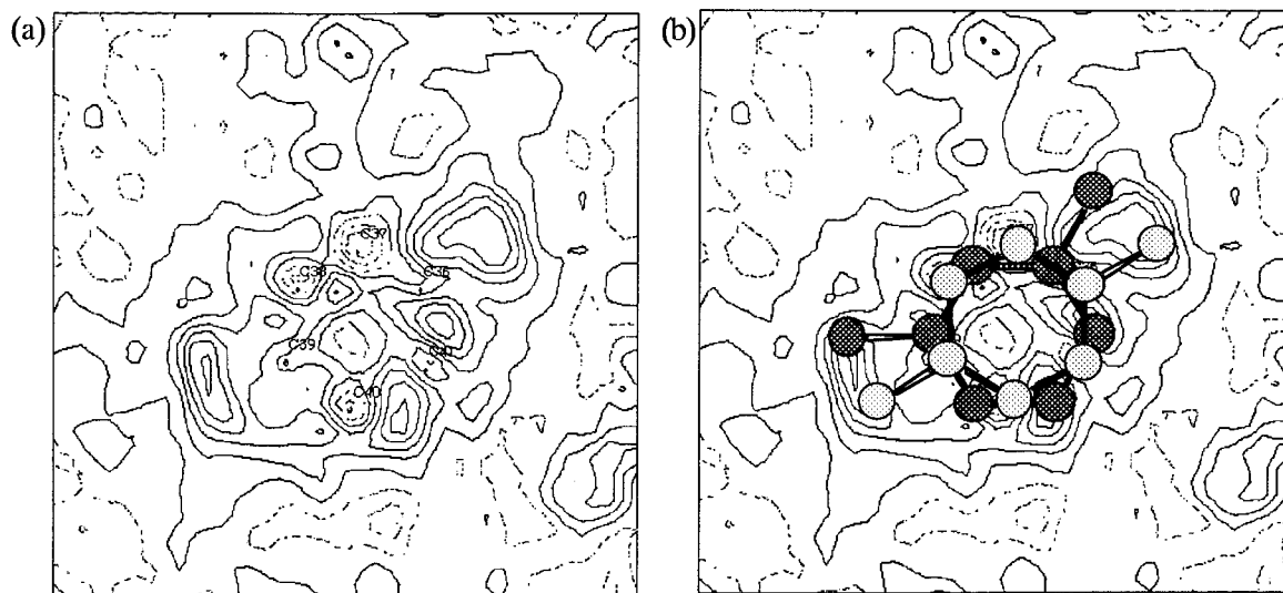
Figure 3-4. (a) Difference Fourier ( F_o-F_c ) map without guest components in the host cavity of CA • 63 + 64 (1:1), (b) Models of 63 and 64 applied in the difference Fourier map of the host cavity of CA • 63 + 64 (1:1). The filled and shadowed circles represent 63 and 64 , respectively.
