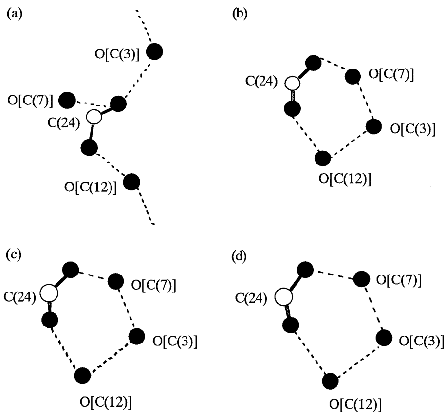
Figure 3-2. Hydrogen bond networks of CA with (a) 62 (Form I), (b) 62 (Form II), (c) 63 , and (d) 64 . The carbon and oxygen atoms are represented by open and filled circle, respectively.
