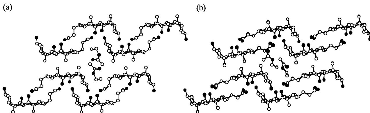
Figure 4-13. Molecular packing diagrams of CA•155 ; (a) Form I and (b) Form II. The carbon and oxygen atoms are represented by open and filled circle, respectively. The carbon and oxygen atoms are represented by open and filled circle, respectively.
