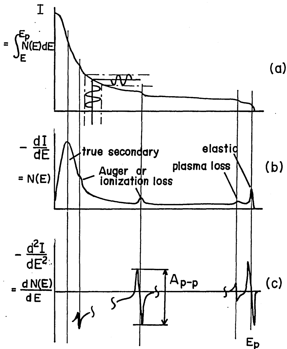
Fig.42 Principles of energy analysis by the retarding method.
