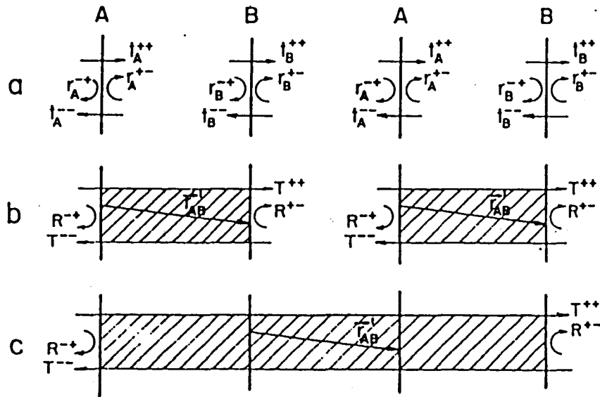
Fig.50 Mechanism of Layer Doubling. 3)
