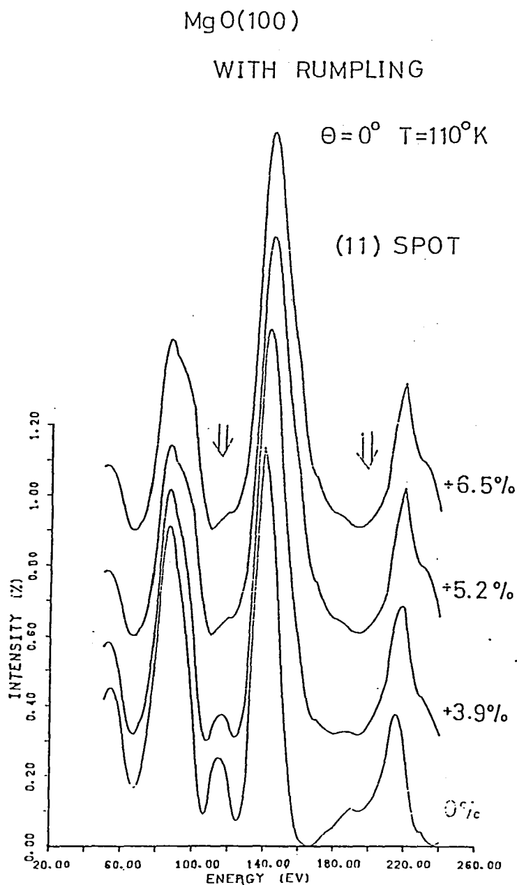
Fig.29 Calculated I-V curves of (11) spot with various degrees of the surface rumpling, by W.Okamoto (ref.41). The + sign indicates that the plane containing O ions is located outside of the plane containing Mg ions.
