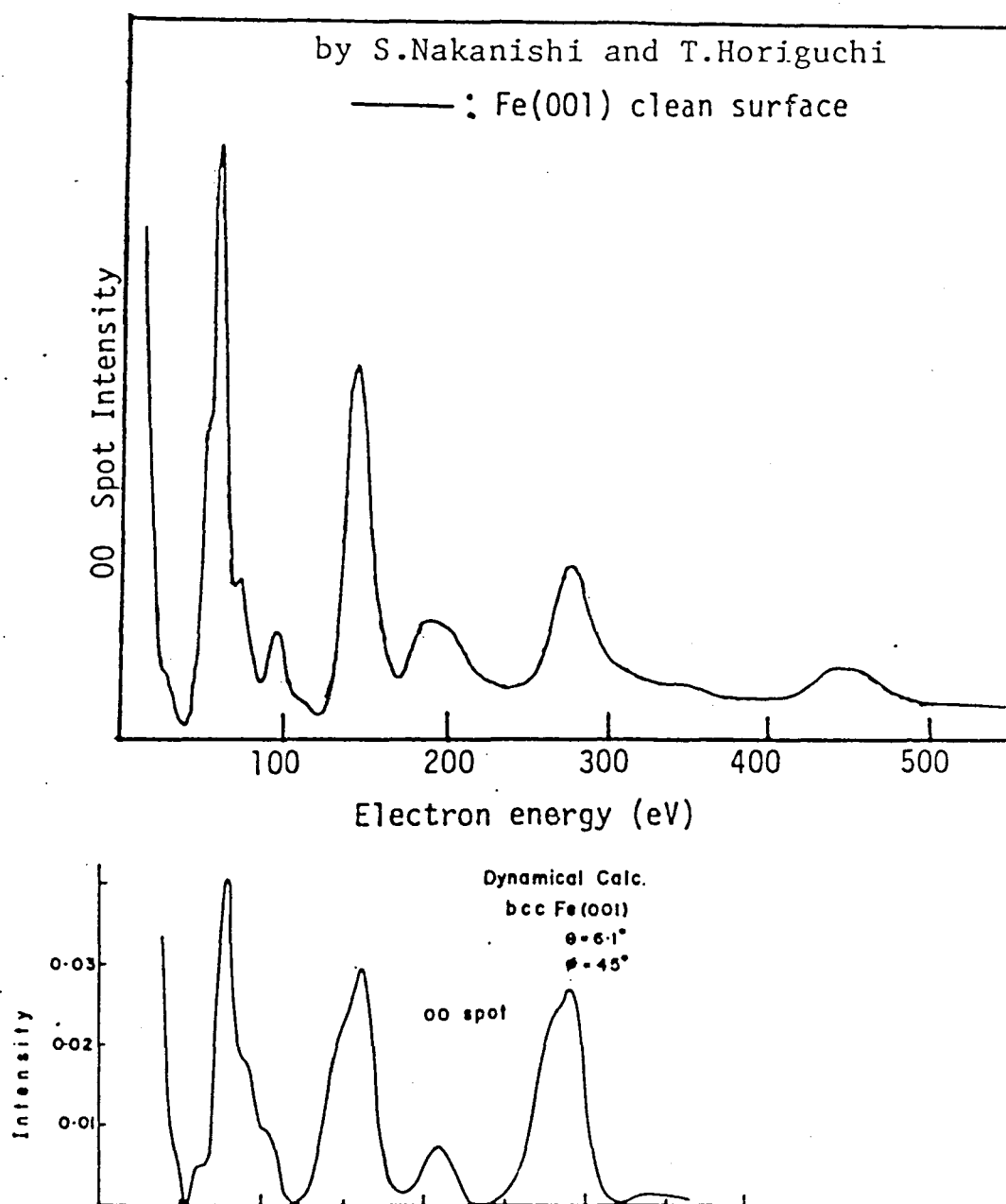
Fig.33 Experimental 43) and calculated I-V curves of (00) beam for Fe(001) surface.
