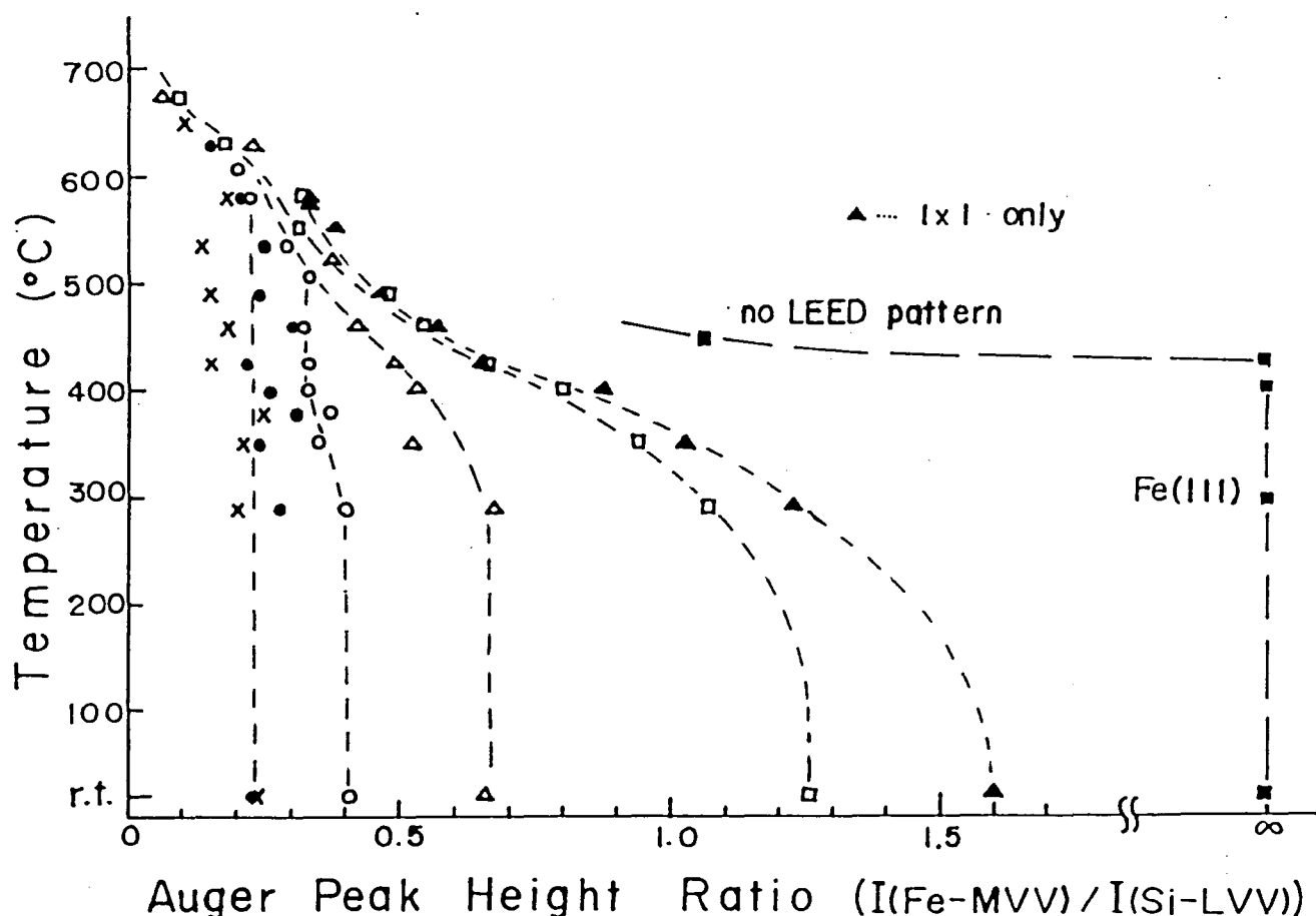
Fig.9 Change of the Auger peak height ratio of Fe-MVV(48eV) to Si-LVV(92eV) with increasing temperature of annealing. The parameter is the Auger peak height ratio immediately after the deposition at room temperature. The ratio of 0.3 corresponds to about one layer (ML) film thickness of Fe(111) plane. For example, the film indicated by a mark \square shows about 1.26 Auger peak height ratio after the deposition, and this value has changed to about 1.1 after annealing at 290°C during 10 minutes. This ratio has changed to 0.95 after annealing at 350°C and so on.
