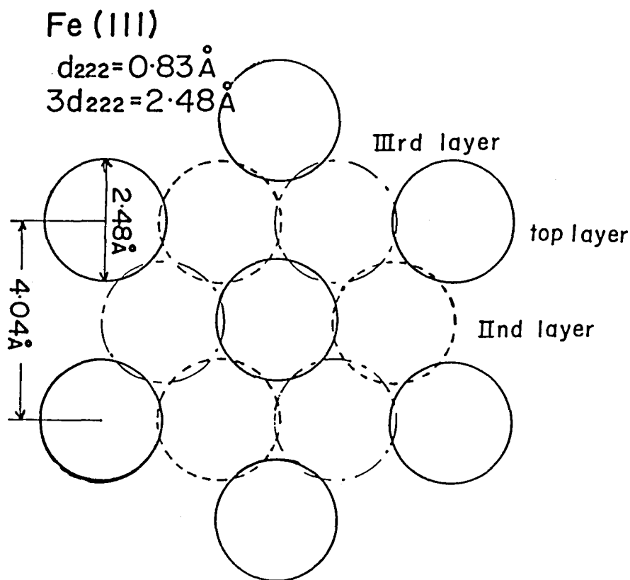
Fig.8 Marble model of the Fe(111) surface. Because the density of iron atoms in the (111) plane is low, three layers are necessary to screen the substrate.
