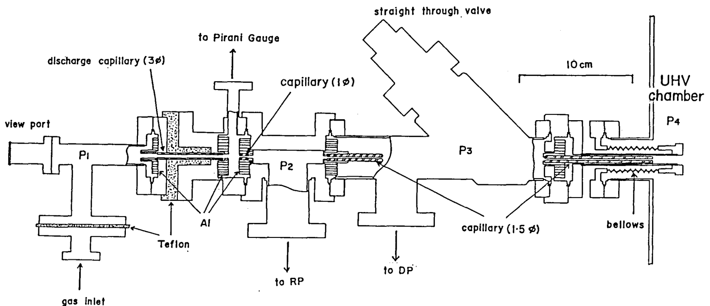
Fig.2 Schematic diagram of the UV photon source. A negative high electric potential (about 3 kV) is supplied to the end electrode on the left hand side. A differential pumping system is used between the discharge part and the UHV chamber. Typical pressures in operation are P_1=260 Pa, P_2=10 Pa, P_3=4 \times 10^{-3} Pa, and P_4=8 \times 10^{-7} Pa, respectively.
