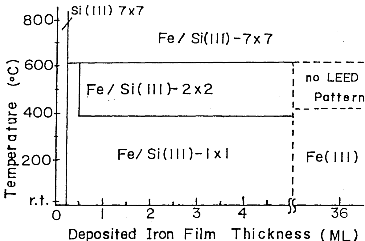
Fig.10 Two-dimensional phase diagram of deposited iron film on Si(111) surface. Iron atoms have been deposited at room temperature, and each film has been annealed at higher temperatures successively. The average thickness of iron film is indicated by that immediately after the deposition.
