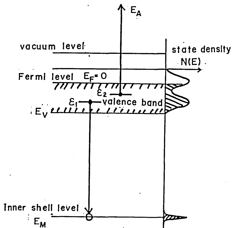
Fig.40 Schematic diagram of the MVV Auger transition.
