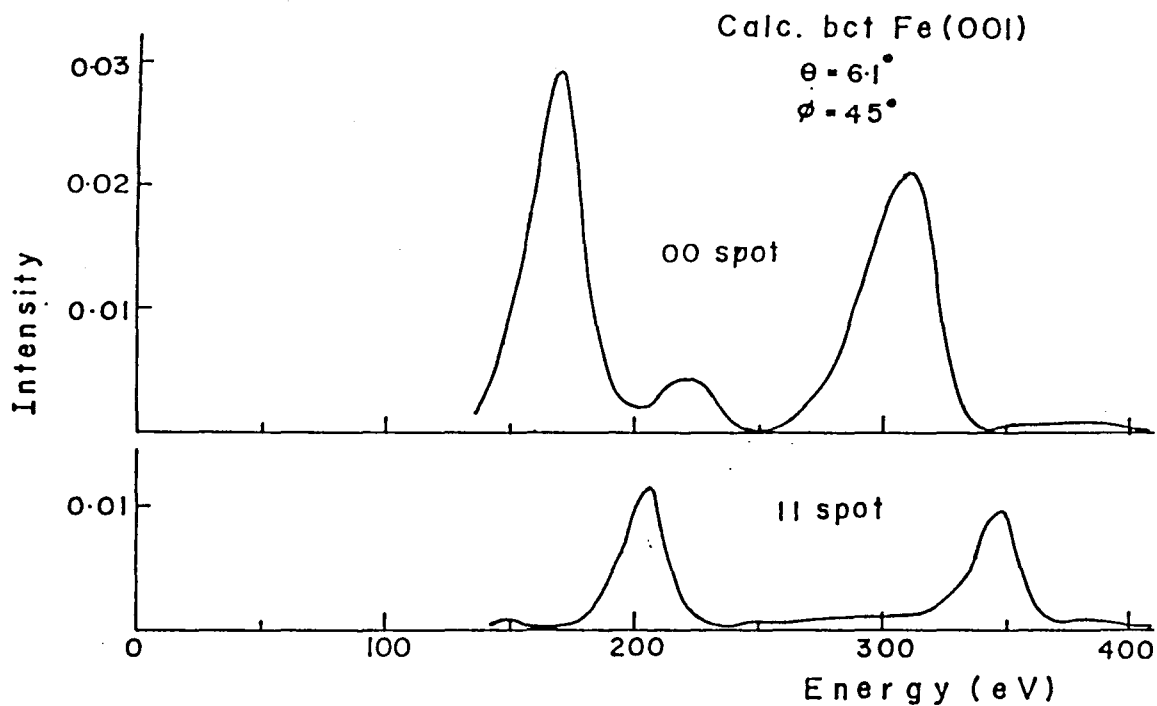
Fig.34 Calculated I-V curves of (00) and (11) beams for body-centered tetragonal Fe(001) surface.
