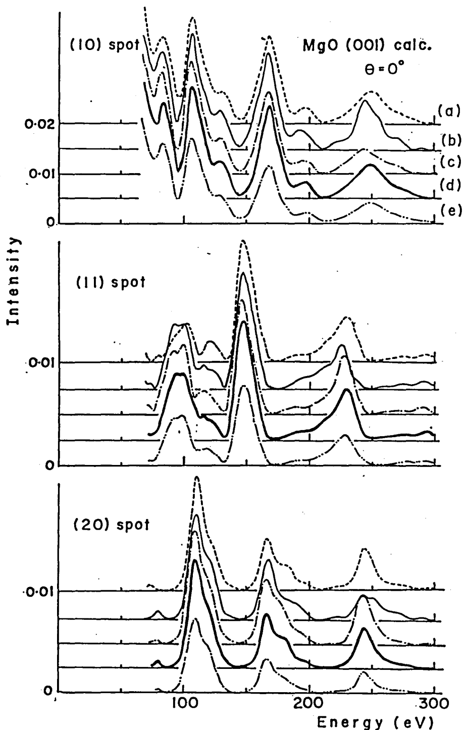
Fig.51 Calculated I-V curves of (10), (11) and (20) beams for MgO(001) surface. Curve d is calculated under the following conditions; (i) phase shifts of the Hartree-Fock approximation are used, (ii) 29 beams are included, (iii) l_{\max} = 4 , (iv) T = 0K . Other curves are calculated by using one different parameter in comparison with the curve d, namely, curve a: phase shifts of the Hartree approximation are used, curve b: 69 beams are included, curve c: l_{\max} = 6 , curve e: T = 400K ( \Theta_D = 900K ).
