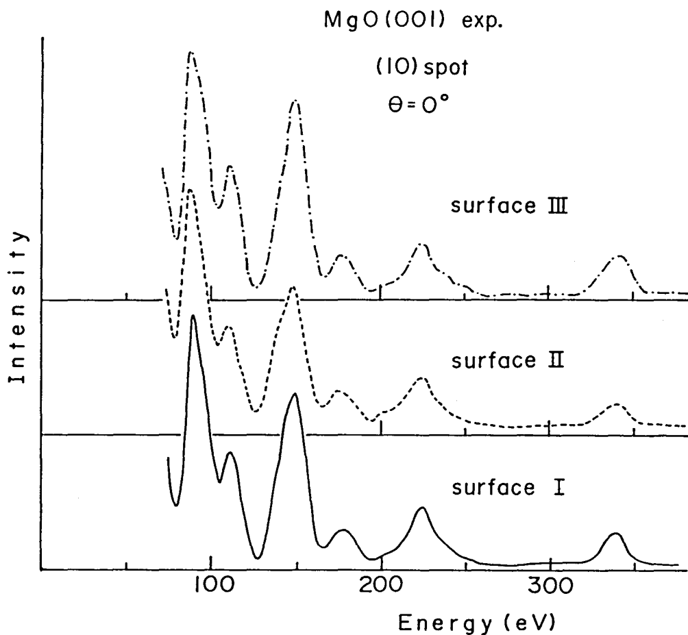
Fig.22 Experimental I-V curves of (10) spot for the three clean MgO(001) surfaces. Surface I is the vacuum-cleaved surface, surface II is the surface which has been heated up to 300°C after vacuum-cleavage, and surface III is the air-cleaved surface.
