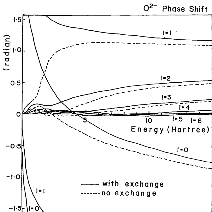
Fig.26 Calculated phase shifts for (a) \text{Mg}^{2+} and (b) \text{O}^{2-} ; ——— Hartree-Fock approximation, - - - Hartree approximation. The muffin-tin radii for Mg and O ions are 0.65 and 1.46 Å, respectively.
