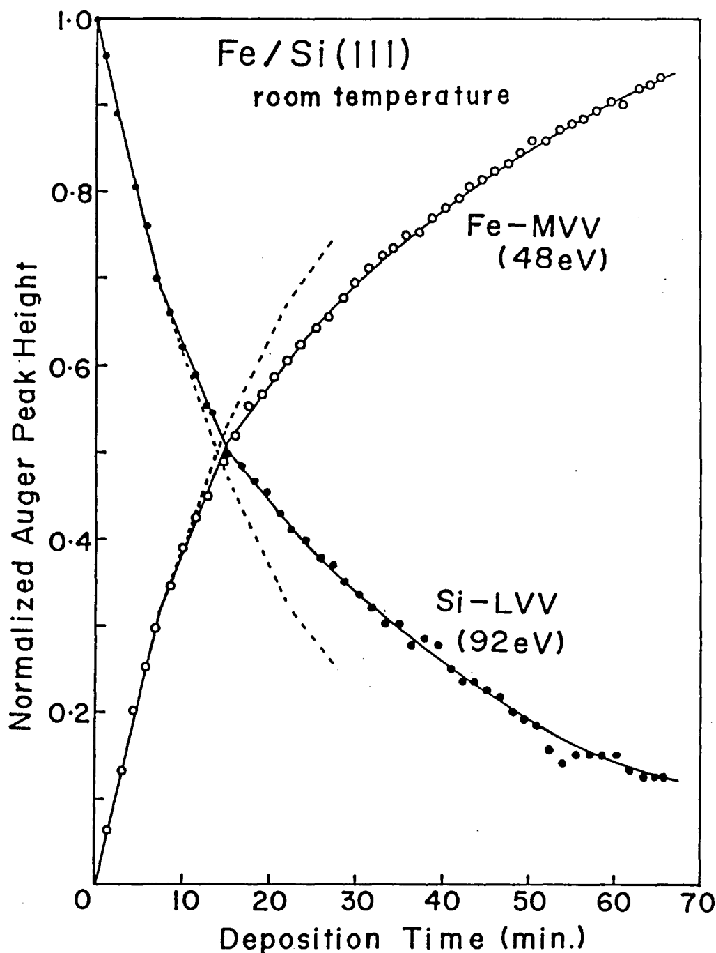
Fig.7 Normalized Auger amplitudes vs. time of deposition for iron film on Si(111) surface at room temperature. Deposition rate is about 0.43 \text{ \AA}/\text{min} . Two break points are shown in each curve. According to the Jackson's criterion, it is indicated that the film has grown in layer-by-layer growth mode.
