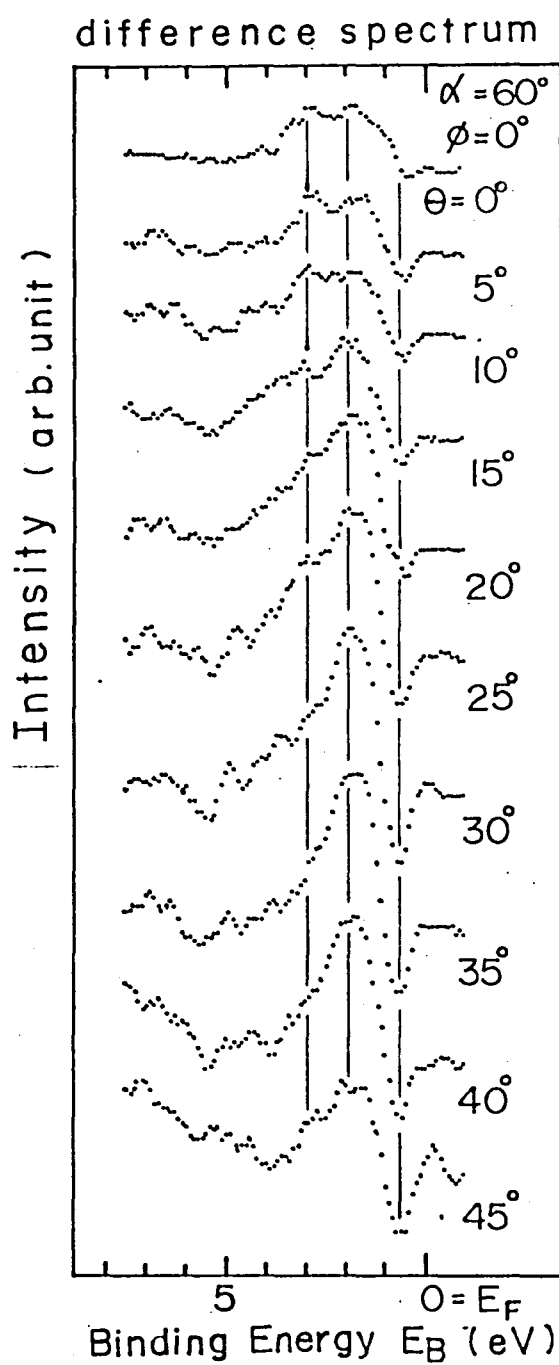
Fig.37 Difference spectra for the iron film of about 1ML thickness on Si(111) surface for various polar angles of emission in the case of glancing incidence of light.
