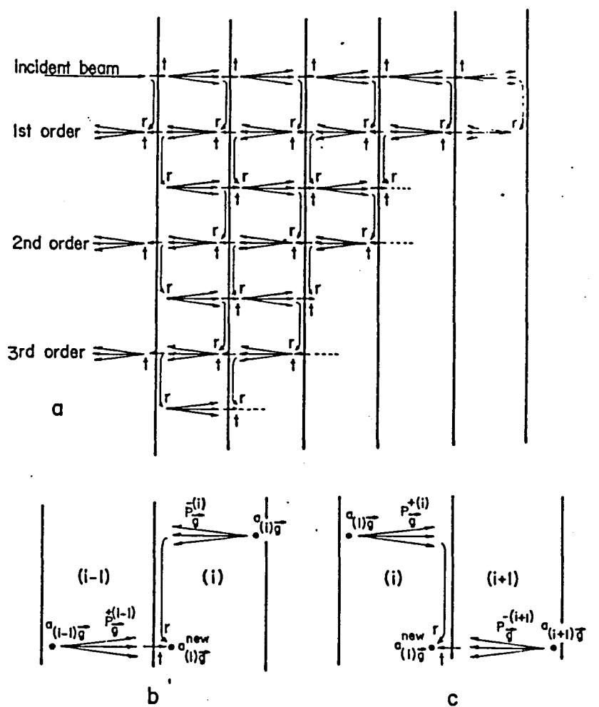
Fig.49 Mechanism of the Renormalized Forward Scattering perturbation method 3) , (a) overall scheme, (b) and (c) details of each propagation step for penetration into and emergence out of the surface, respectively.
