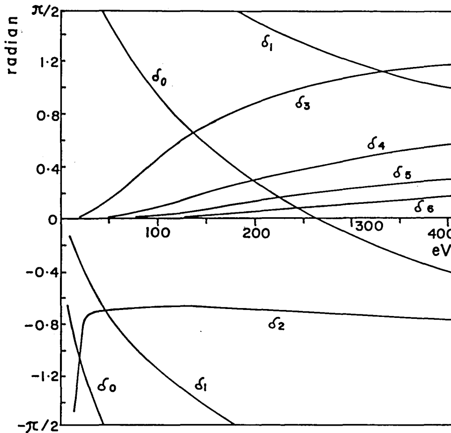
Fig.30 Calculated phase shifts for iron atom as the function of energy. Electron configuration is assumed to be as 6 3d-state electrons and 2 conduction electrons. Muffin-tin radius is 1.24\text{\AA} which corresponds to one-half of the nearest neighbour distance for bcc iron crystal.
