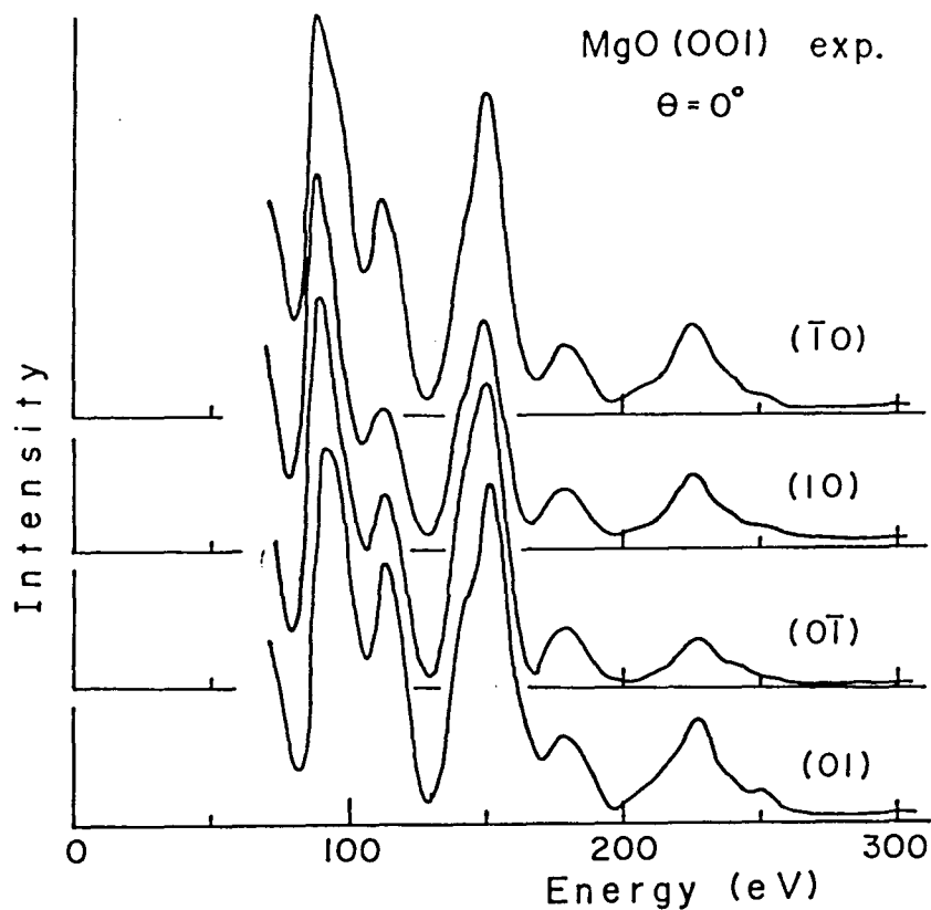
Fig.21 Four symmetrical I-V curves of 10 beam for the MgO(001) surface III (air-cleaved and eliminated carbon contamination by heating up to 800°C in oxygen atmosphere of 10^{-5} Pa) for the confirmation of the condition of normal incidence. Although the four curves are not precisely similar, the similarity is considered to be sufficient for the present purpose.
