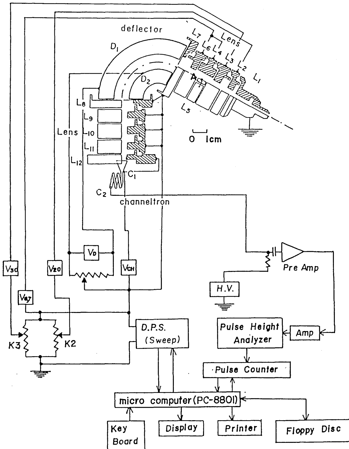
Fig.3 Composition of photoelectron energy analyzer system. The 127° type electron energy analyzer is composed of four parts, namely, "input lens", "deflector", "output lens", and "channeltron". In order to obtain an energy distribution curve electrons are retarded (or accelerated) in the input lens system in proportion to their energies by sweeping the output voltage of a conventional digital programable power source (D.P.S.). In order to remove the aberration the best operation of the input lens system has been determined experimentally (see text).
