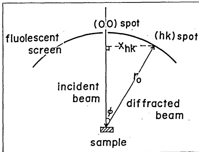
Fig.4 (a) Schematic diagram of the geometry of LEED arrangement in real space and (b) the diffraction condition in reciprocal space.
