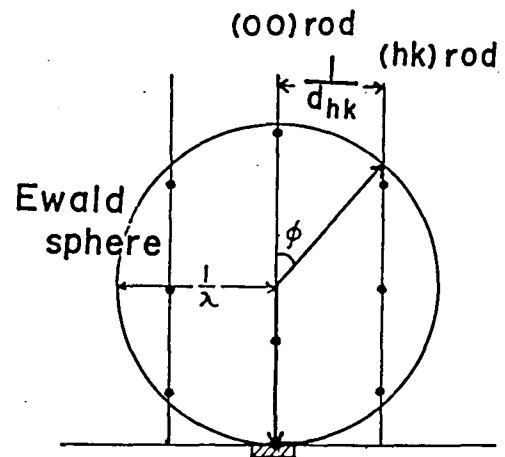
Fig.4 (a) Schematic diagram of the geometry of LEED arrangement in real space and (b) the diffraction condition in reciprocal space.
