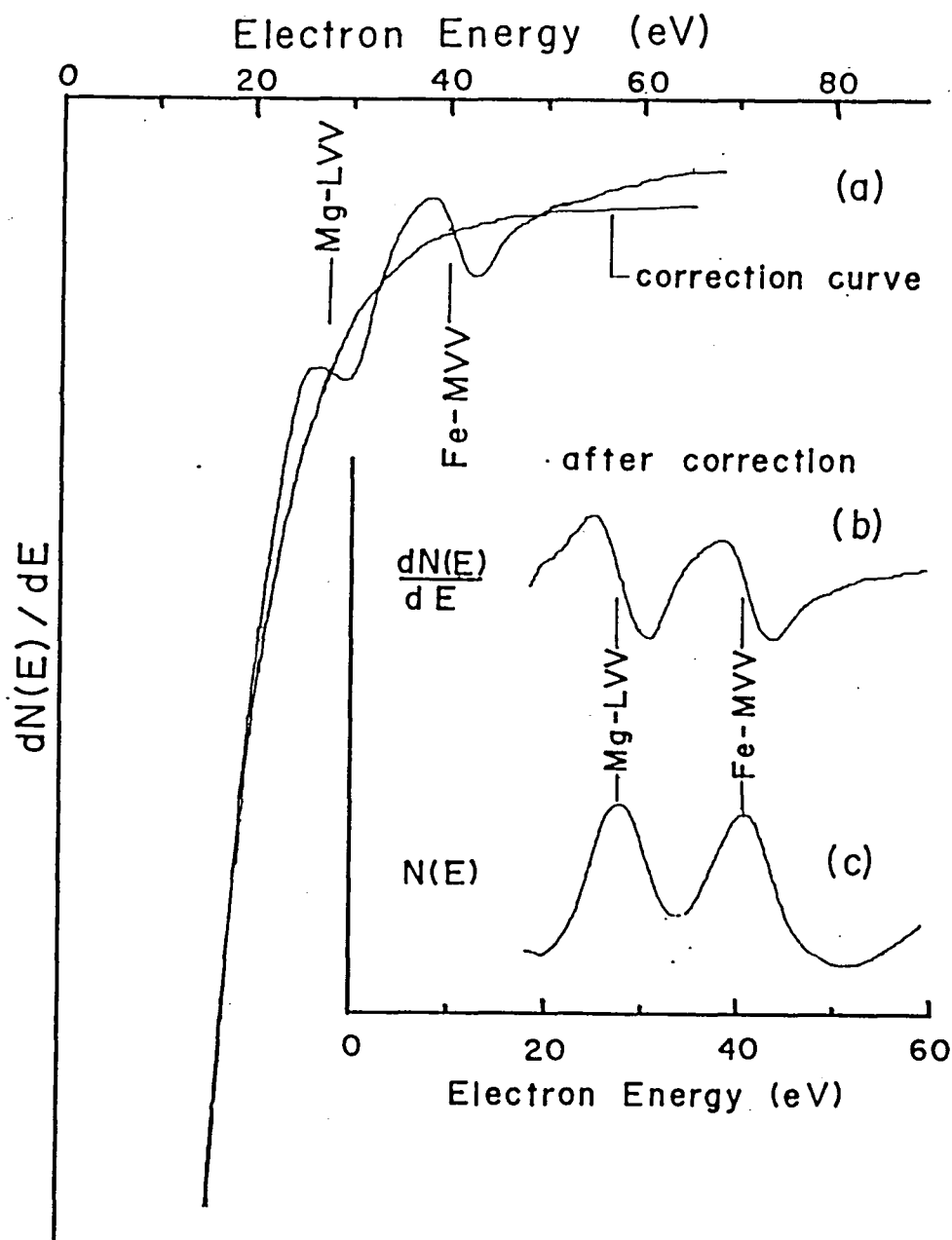
Fig.38 The principle of searching for N(E) curve by means of integration of the dN(E)/dE curve after the subtraction of the background. (a) An approximate curve ("correction curve") is adjusted to coincide with the back ground of the experimental dN(E)/dE curve, (b) The "correction curve" is subtracted from the experimental curve, and finally, (c) the dN(E)/dE curve is integrated.
