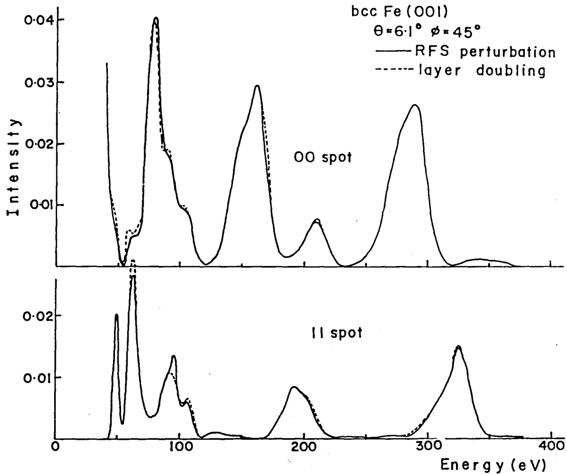
Fig.52 Calculated I-V curves for bcc Fe(001) surface by different layer stacking methods of RFS perturbation and Layer Doubling.
