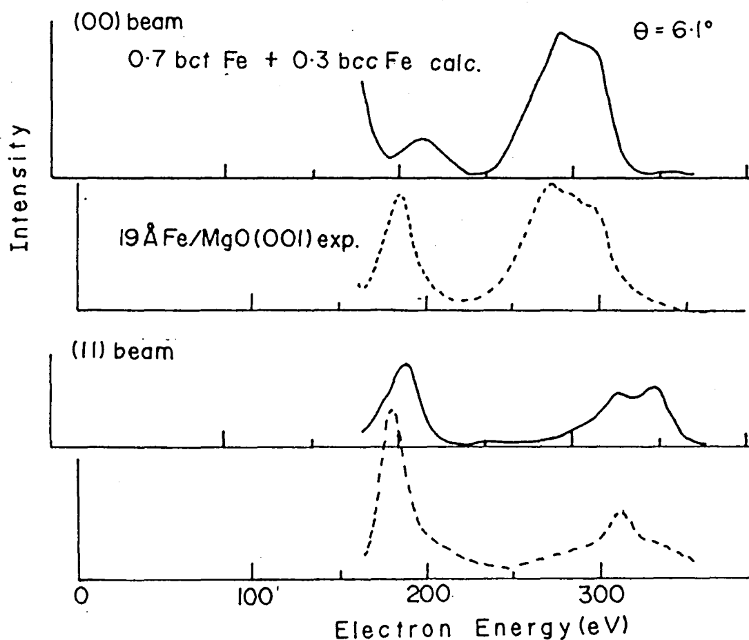
Fig.35 Calculated I-V curves added in the ratio of 0.7 bct Fe (Fig.34) to 0.3 bcc Fe (Fig.33 or Fig.52) for the comparison with the experimental I-V curves for the iron film of 19 Å thickness on MgO(001) surface shown in Fig.25.
