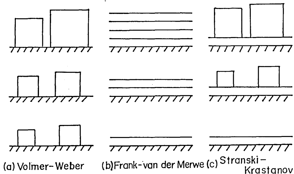
Fig.6 Three basic growth modes: (a) Volmer-Weber (3-D island) growth mode, (b) Frank-van der Merwe (layer-by-layer) growth mode and (c) Stranski-Krastanov growth mode.
