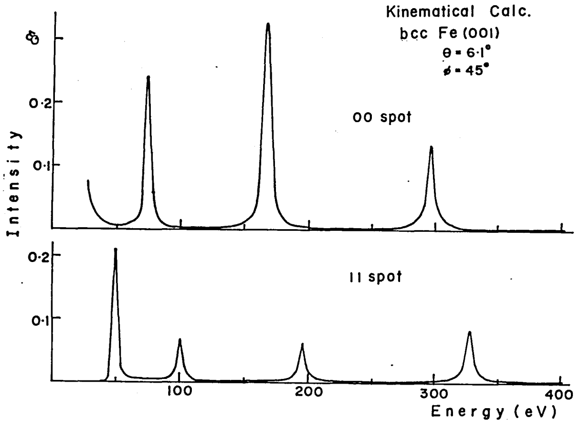
Fig.48 An example of intensity vs. energy spectrum for Fe(001) surface calculated in the kinematical theory.
