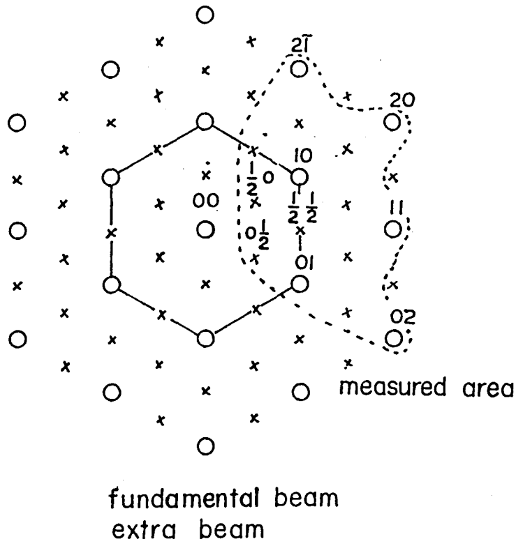
Fig.12 Schematic indication of LEED spots indices.
