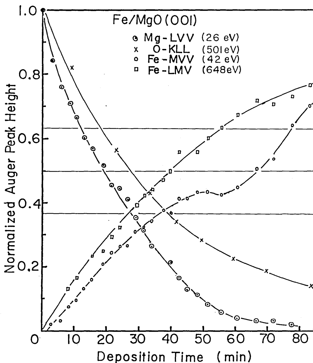
Fig.20 Normalized Auger amplitudes vs time of deposition for iron film on MgO(001) surface at room temperature. Deposition rate is about 0.2 Å/min. Since four curves separate with one another, according to the Palmberg's criterion, it is indicated that the iron film dominantly has grown in layer-by-layer growth mode.
