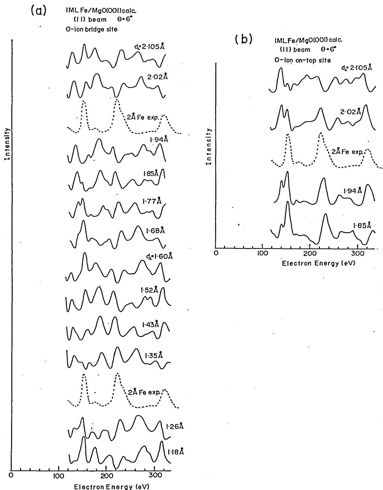
Fig.32 Calculated I-V curves of (11) beam for the monolayer iron film on MgO(001) surface (solid curve) for the comparison with the experimental curve (broken curve), (a) bridge site of the O ions and (b) on-top site of the O ion.
