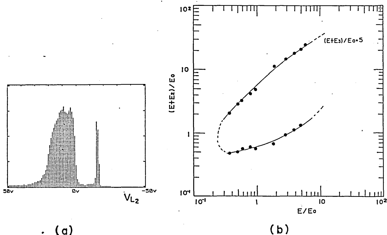
Fig.44 (a) An example of variation of counting rate when the potential of the electrode, L_2 , is changed, (b) An example of experimental focal line obtained by changing an incident energy.
