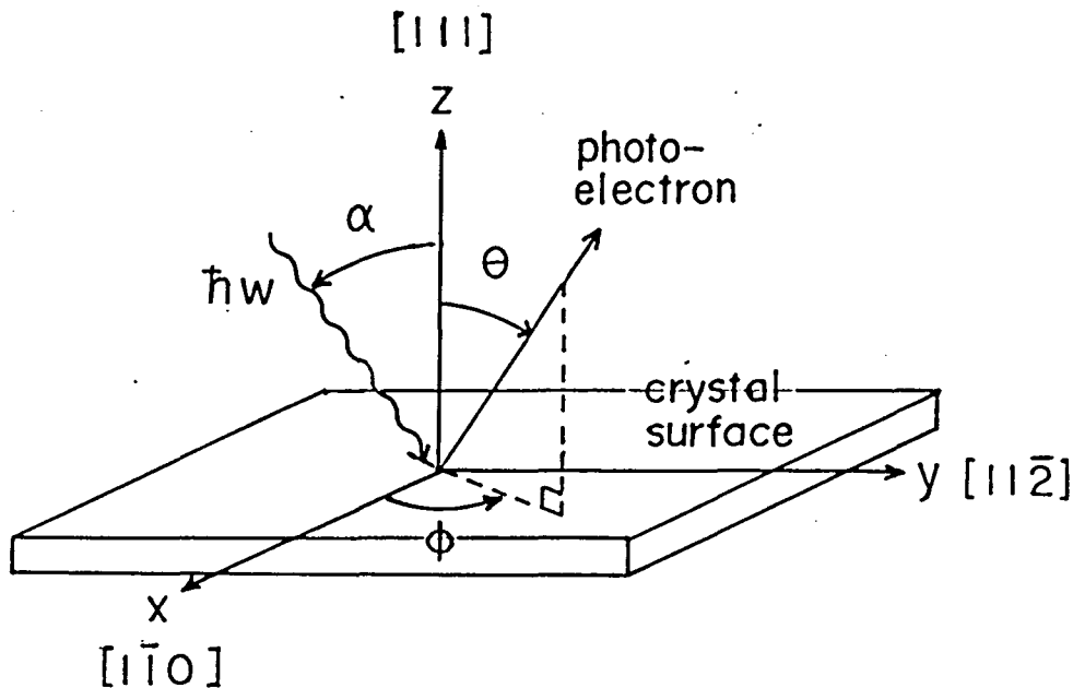
Fig.17 Angle setting of the light beam and the detector.
