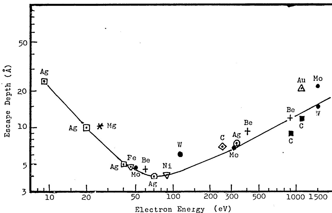
Fig.45 Relation between the electron escape length and its energy 40) .
