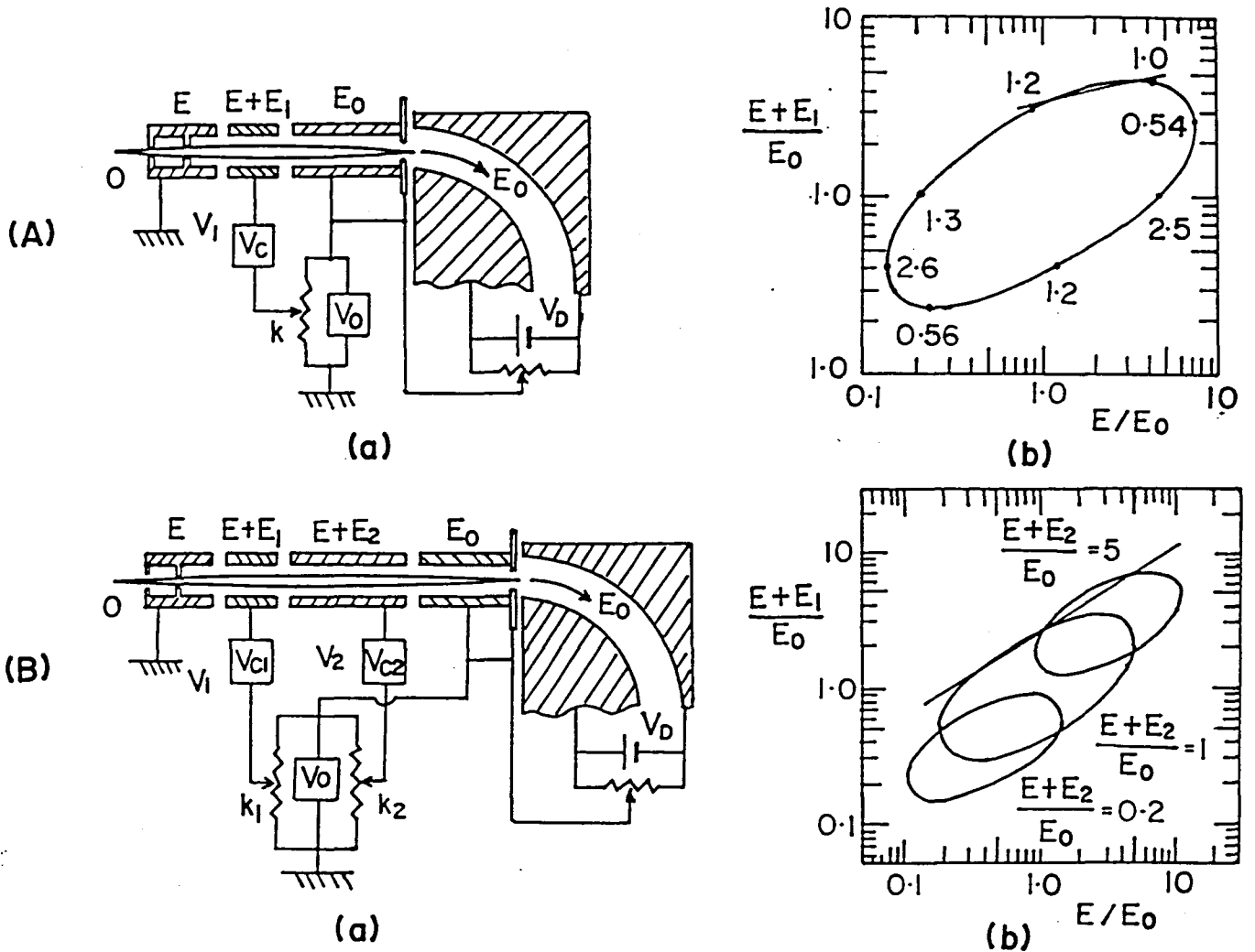
Fig.43 Schematic diagram of focal properties with input lens system 17) , (A) a lens composed of three electrodes, (B) a lens composed of four electrodes, and (a) electric circuit to remove the aberration effect, (b) focal locus.
