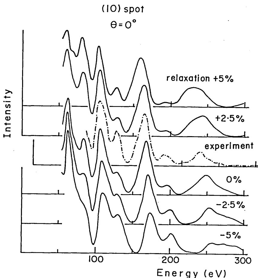
Fig.27 Calculated I-V curves of (10) spot (solid curve) for the comparison with the experimental curve (dash-dotted curve). The indices present the ratio of the relaxation to the normal lattice spacing, \Delta d/d , and the + and - signs represent expansion and contraction, respectively.
