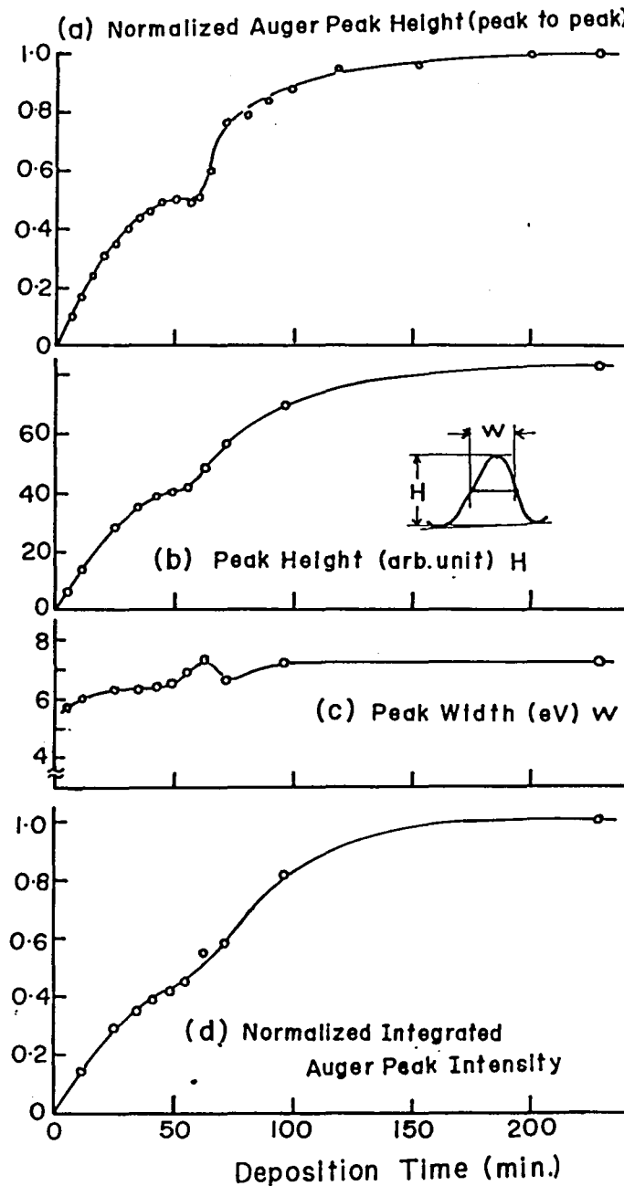
Fig.39 Change of the Fe-MVV Auger signal: (a) peak-to-peak amplitude in the dN(E)/dE curve, and (b) peak height, (c) peak width, (d) integrated intensity in the N(E) curve.
