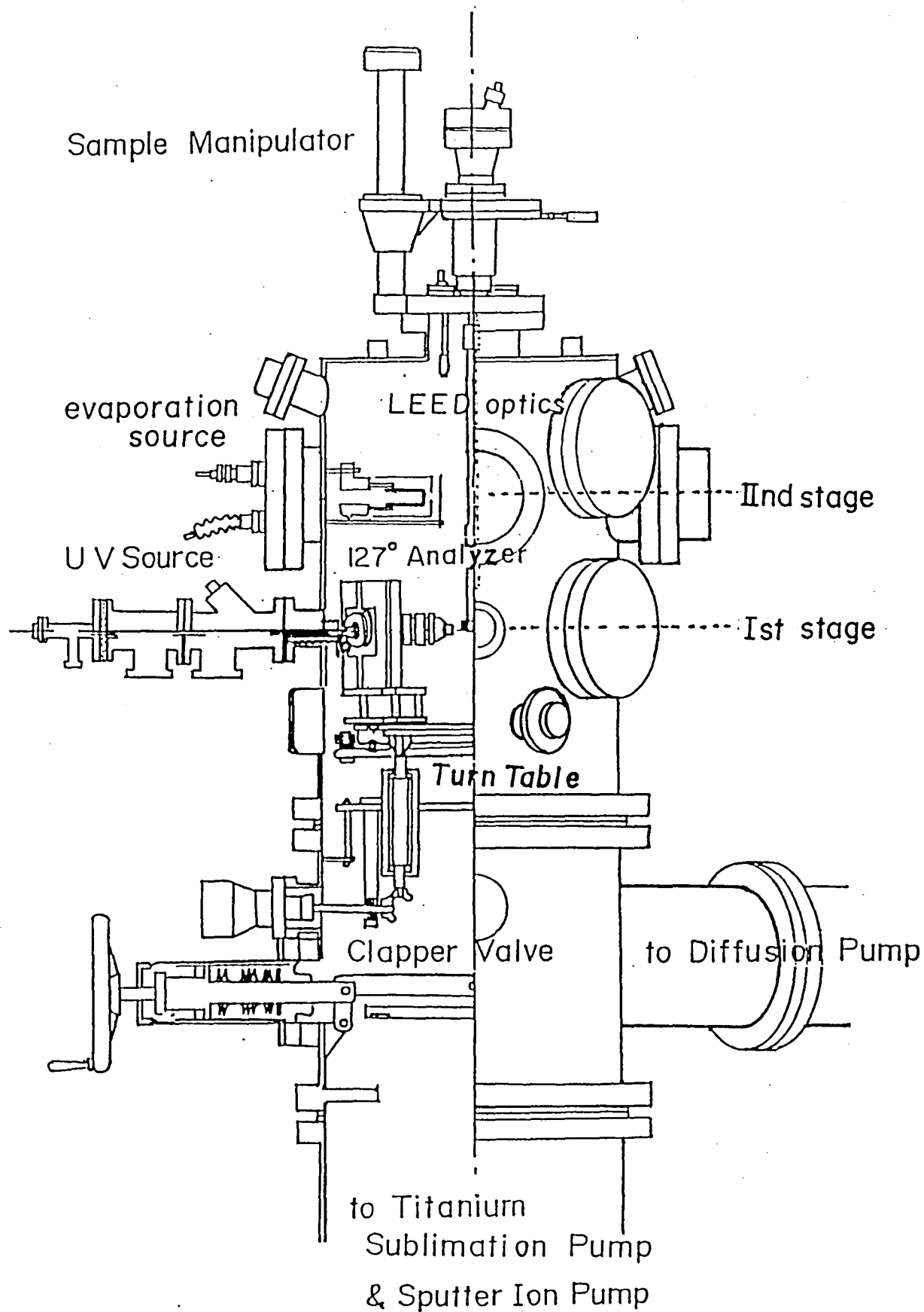
Fig.1 Schematic diagram of the experimental apparatus. At the "Ist stage" the 127° type electron energy analyzer on a turn table and the ultraviolet (UV) photon source are settled, and at the "IInd stage" LEED optics for LEED-AES and a metal vapour evaporation source are installed. A long stroke sample manipulator transfers the sample between these stages.
