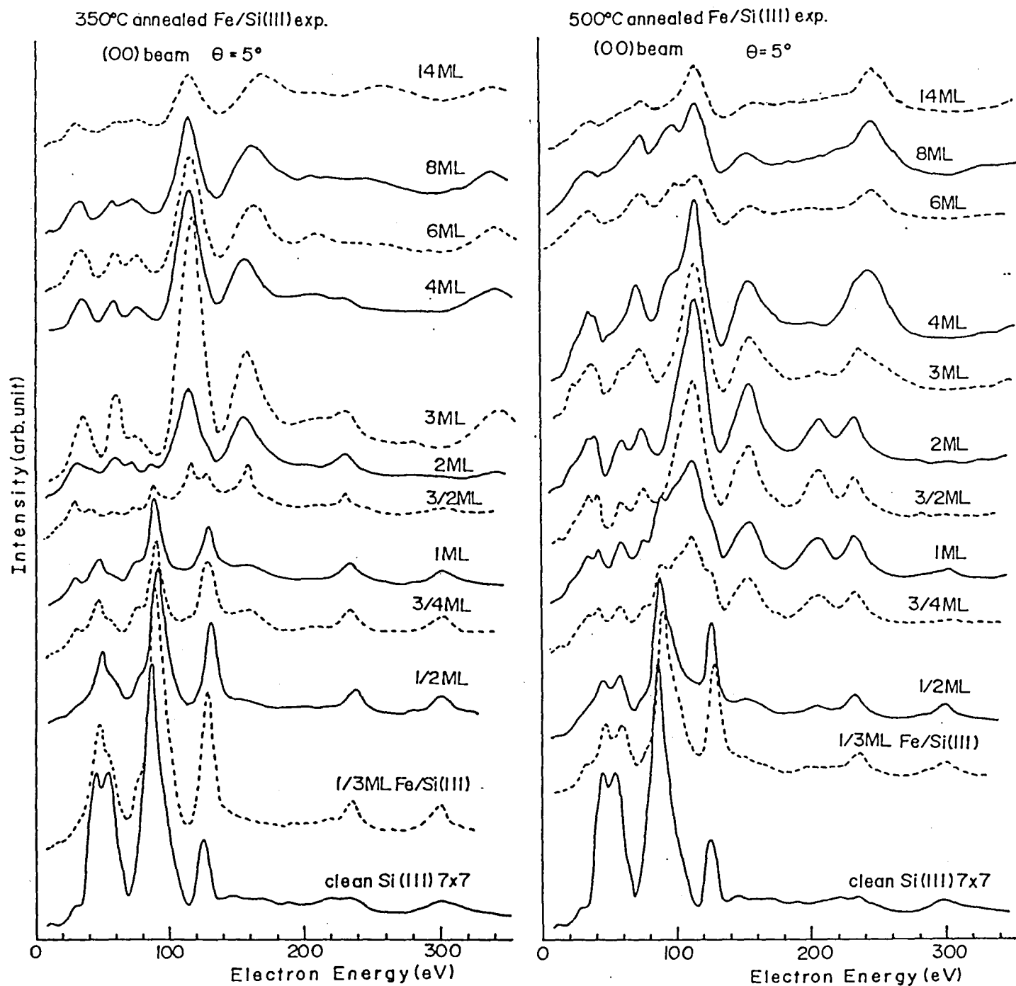
Fig.16 Experimental I-V curves of (00) beam for iron films of various thicknesses on Si(111) under the condition of \theta = 5^\circ and \phi = 0^\circ , (a) for the films annealed at 350°C, (b) for the films annealed at 500°C, respectively, after the deposition at room temperature.
