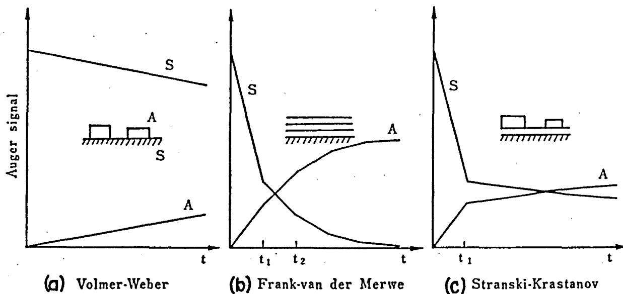
Fig.47 Variations of the Auger signals for the substrate S and the adsorbate A during the film growth by different mechanism (ref.50), t_1 is the time for the completion of the first monolayer.
