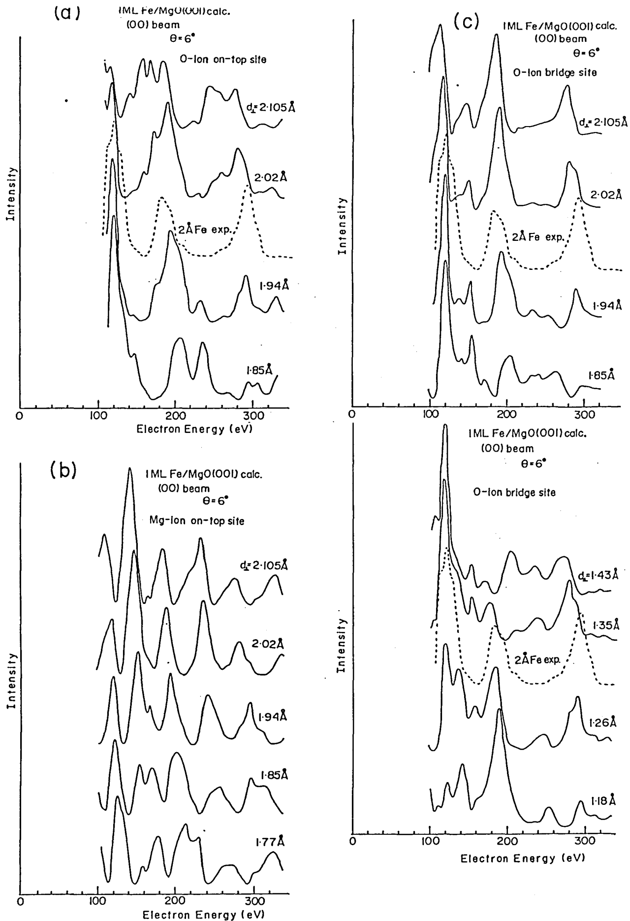
Fig.31 Calculated I-V curves of (00) beam for the monolayer pseudomorphic iron film on MgO(001) surface with the different degree of the relaxation (solid curve) for the comparison with the experimental curve of 2 Å average thickness (broken curve). Three probable sit-sites of iron atoms are shown, (a) on-top site of the O ion, (b) on-top site of the Mg ion and (c) bridge site of the O ions. d_{\perp} represents a spacing between the iron layer and the topmost layer of MgO(001) surface.
