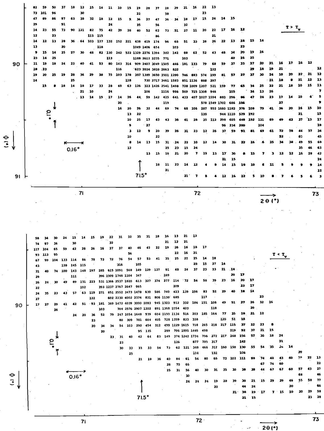
Fig. 3-9 The X-ray reflection intensity distribution in the two-dimensional reciprocal lattice space near (10,10,10) Bragg spot.
