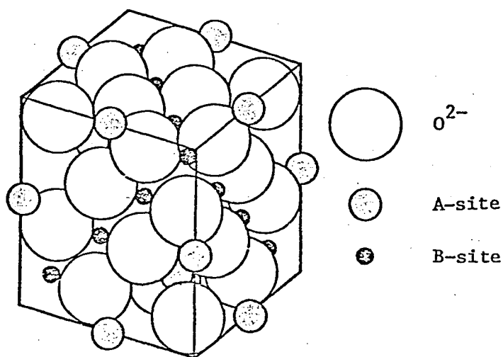
Fig. 3-1 Spinel structure
