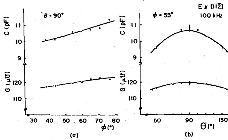
Fig. 3-17 Capacitance and conductance along [11\bar{2}] , as a function of the magnetization direction. The frequency was 100 kHz.
