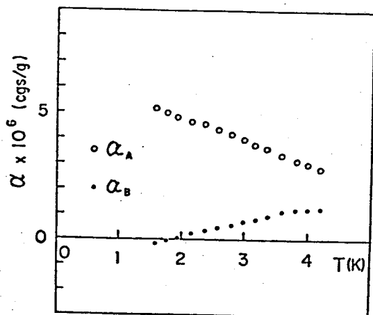
Fig. 2-6. Extraordinary temperature dependence of \alpha below 4.2 K.
