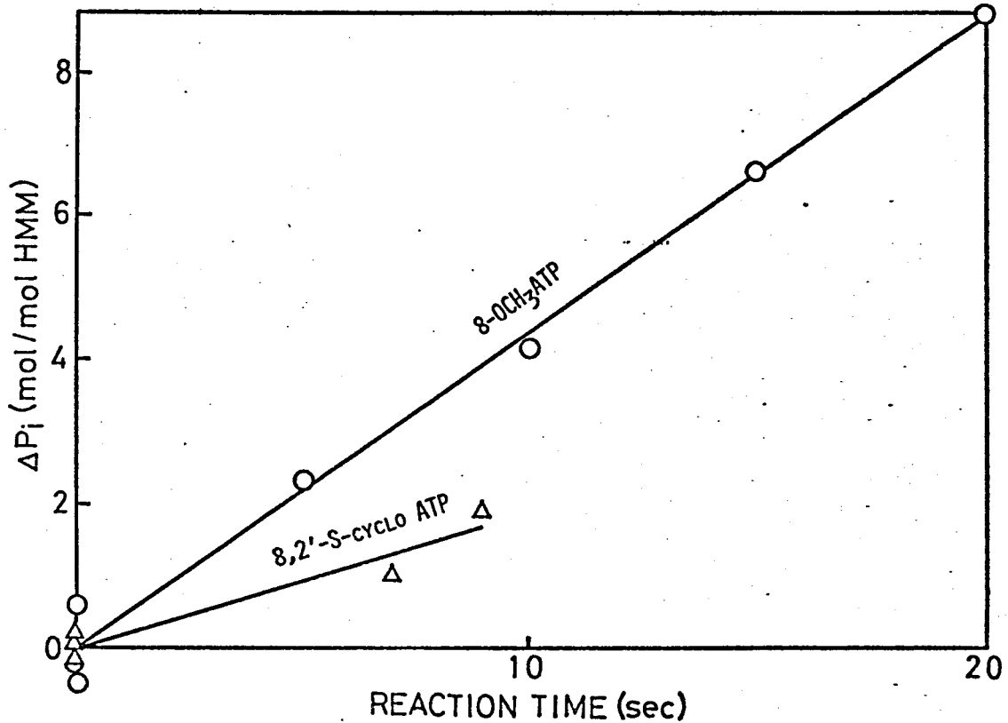
Fig. 15. Time course of Pi-liberation from HMM-NTP systems. 0.3mM NTP, 6.8 mg/ml HMM, 0.5M KCl, 5mM \text{MgCl}_2 , 20mM Tris-HCl, pH 7.8, 0-1°. NTPs used were indicated in the figure.
