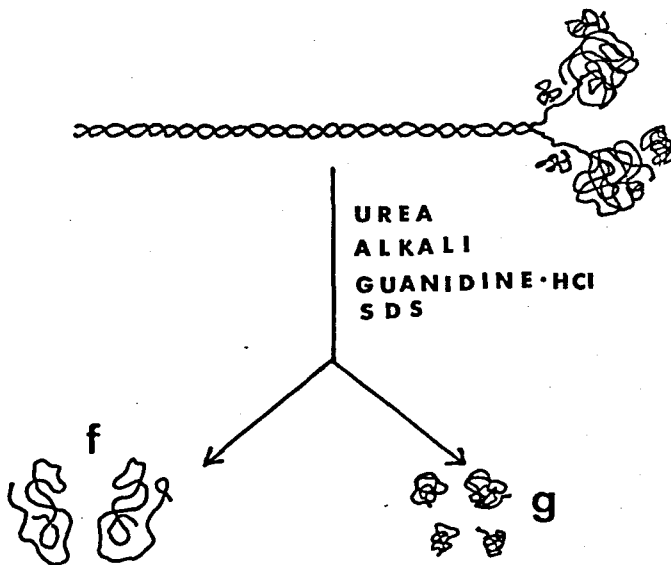
Fig. 6. A schematic structure of subunit composition of myosin molecule. One myosin molecule dissociates into two f-chains and four g-chains.
