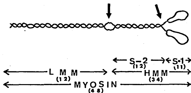
Fig. 3. A schematic representation of the myosin molecule. The number in parentheses are the molecular weight \times 10^{-4} . Arrows indicate protease-sensitive regions.
