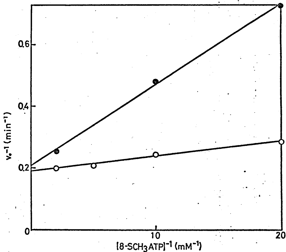
Fig. 13. Double-reciprocal plots of 8-SCH 3 ATPase activity of myosin in the presence and absence of FA versus the concentration of 8-SCH 3 ATP. 0.1 mg/ml myosin, 50mM KCl, 2mM MgCl 2 , 20μM CaCl 2 , 20mM Tris-HCl, pH 7.8, 20°. Activities were measured in the presence (●) and absence (○) of 0.4 mg/ml FA-RP.
