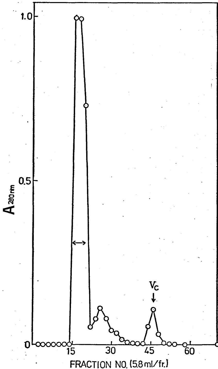
Fig. 4. Sephadex G-100 gel-filtration of HMM treated with CMB. HMM (10mg/ml) was treated with 4 moles of CMB/ 10^5 g of HMM in 50mM KCl, 50mM Tris-maleate, and 5mM EDTA at pH 7.0 and 20° for 20 min. The solution was applied to a column (2.9x41-cm) equilibrated with 50mM KCl, 50mM Tris-HCl, and 0.5mM EDTA at pH 7.6 and 4°. The column was eluted with the same buffer at a flow rate of 23ml/hr, and fractions of 5.8ml were collected. v_c indicates the column volume.
