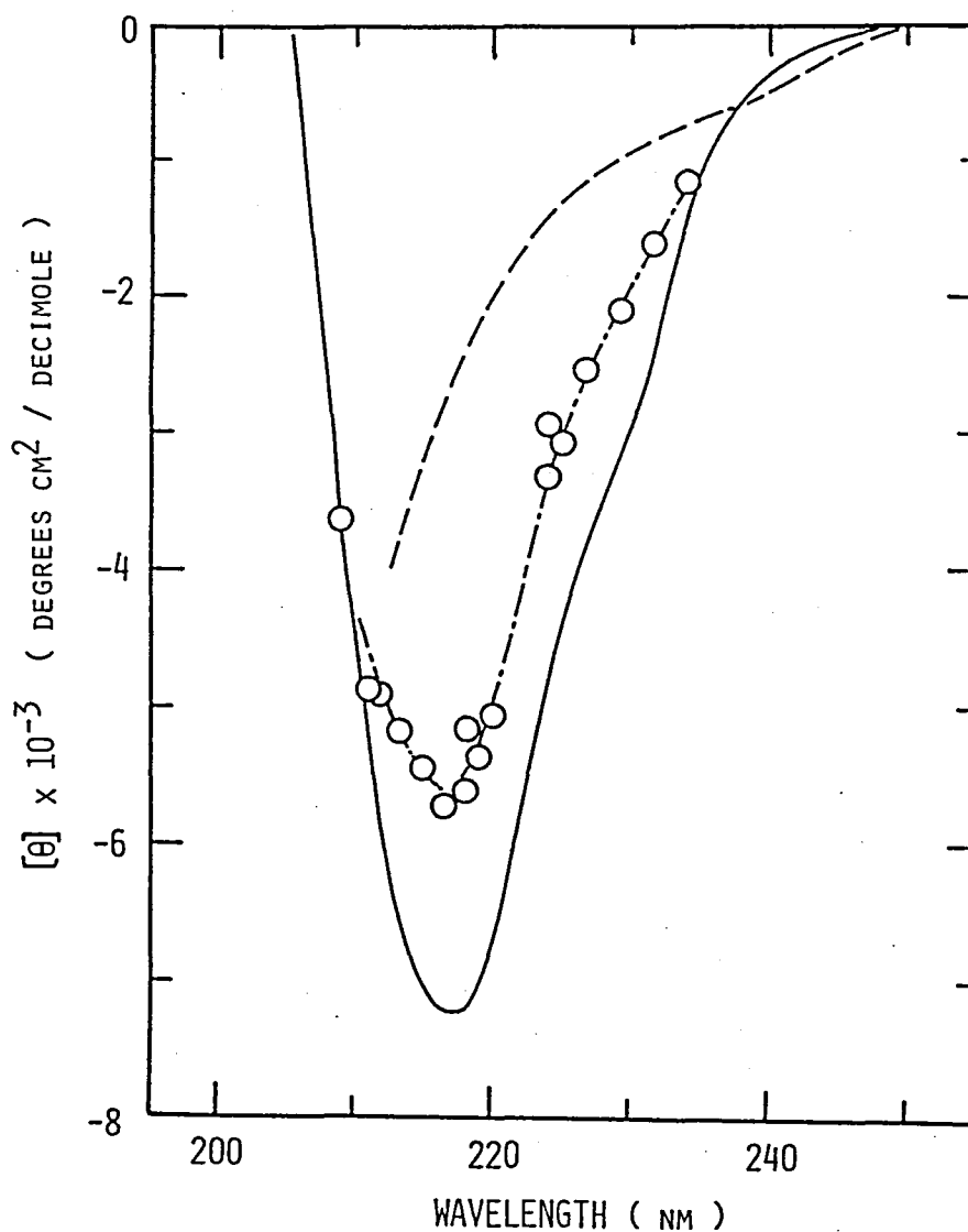
Fig. 4.9. The initial points for the slow phases of refolding kinetics of the C_L fragment measured by CD at various wavelengths. pH 7.5, 25°C. Initial conditions: 4 M GuHCl; protein concentration, 7 mg/ml. Final conditions: 0.1 M GuHCl; protein concentration, 0.2 mg/ml. The solid and broken lines indicate the spectra of native protein and unfolded protein in 4 M GuHCl, respectively.
