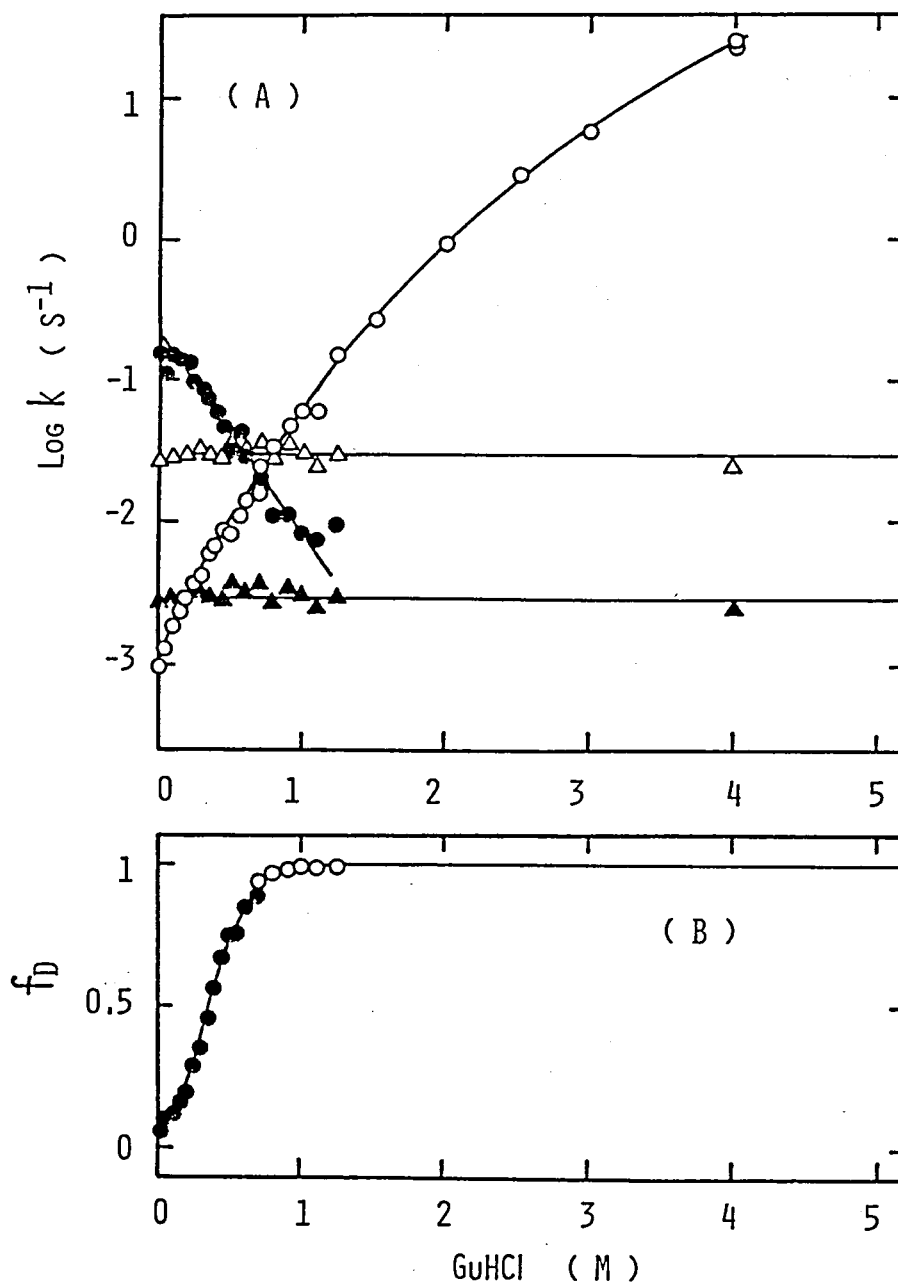
Fig. 5.7. The dependence on GuHCl concentration of the microscopic rate constants estimated based on mechanism 5.1 for folding of the reduced C_L fragment (A) and the transition curve for unfolding obtained from kinetic measurements (B). pH 7.5, 25°C. (A) ( \circ ), k_{32} ; ( \circ ), k_{23} ; ( \Delta ), k_{21} ; ( \Delta ), k_{12} . (B) ( \bullet ), the amplitude of the fast phase determined by SH titration shown in Fig. 5.4(B); ( \circ ), the fraction of the unfolded species calculated using the four microscopic rate constants. The solid line indicates the transition curve for unfolding obtained from equilibrium measurement.
