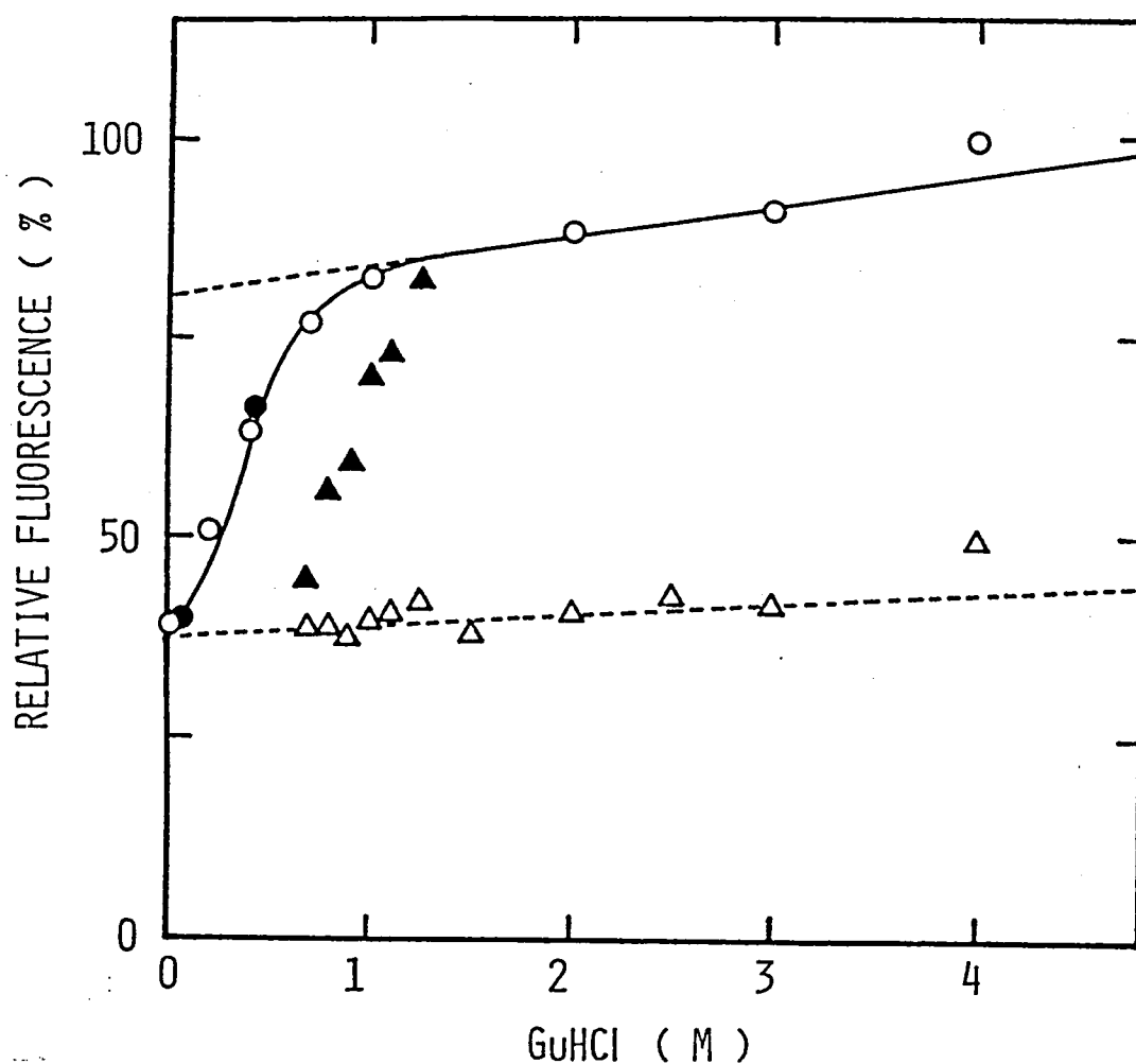
Fig. 5.1. Equilibrium and kinetic data for the denaturation of the reduced C_L fragment by GuHCl. pH 7.5, 25°C. Measurements were carried out by fluorescence using a stopped-flow apparatus at a protein concentration of 0.02 mg/ml. The initial concentrations of GuHCl for unfolding (○) and refolding (●) equilibria were 0 M and 4 M, respectively. The initial points of the slow and fast phases of unfolding kinetics are shown by ▲ and △, respectively. They were obtained by extrapolating the respective phases to time zero. Initial conditions for unfolding kinetics: 0 M GuHCl, protein concentration, 0.04 mg/ml. The solid line indicates the theoretical curve constructed using Eqs. (3.1) and (3.2) and the values of \Delta n and \Delta G_D^{H_2O} obtained on the basis of k = 0.6 (Table 3.II) (see Chapter 3).
