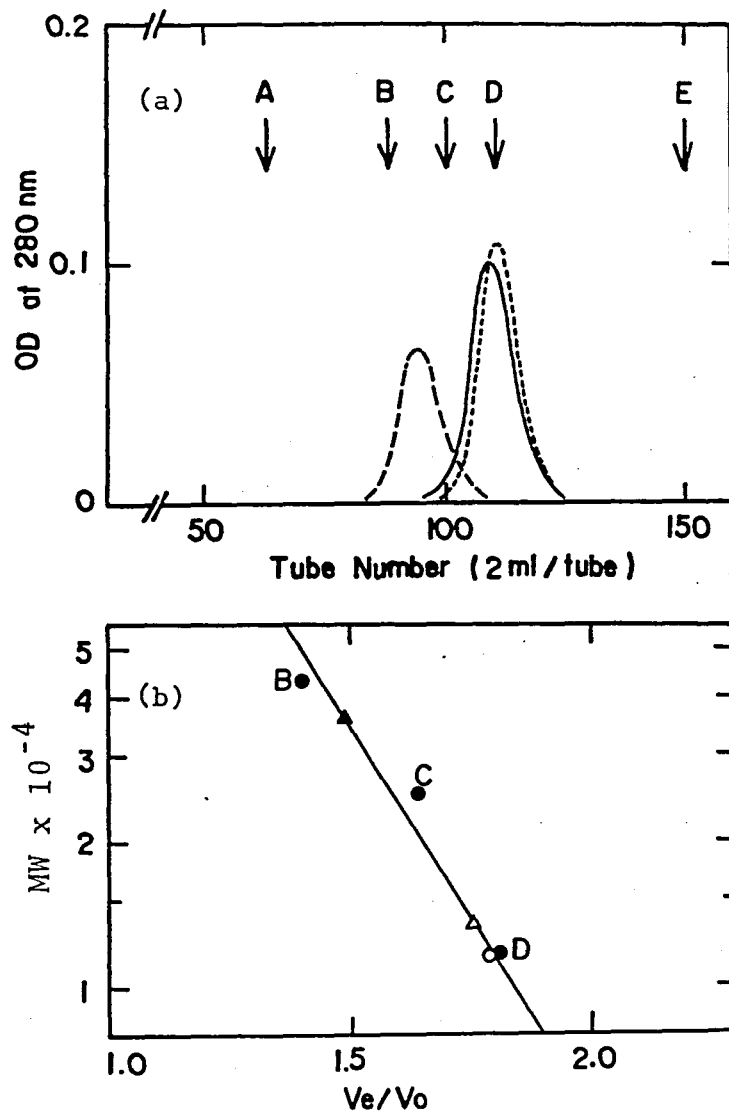
Fig. 3.7. Gel filtration patterns (a) of intact C_L fragment (dotted line), reduced C_L fragment (solid line), and CAM- C_L fragment on a Sephadex G-75 column (1.6 x 164 cm) equilibrated with 5 mM acetate buffer at pH 6.1 containing 1 mM EDTA and 0.15 M KCl, and estimation of apparent molecular weight (b) of intact C_L fragment ( \circ ), reduced C_L fragment ( \triangle ), and CAM- C_L fragment ( \blacktriangle ). One to two mg of the protein samples were applied to the column. Blue dextran (A), ovalbumin (B), \alpha -chymotrypsinogen (C), cytochrome c (D), and dithiothreitol (E) were run on the same column as standards. Their absorbance peak positions are indicated by arrows. Abscissa in (b) indicates the ratio of elution volume ( V_e ) to void volume ( V_o ).
