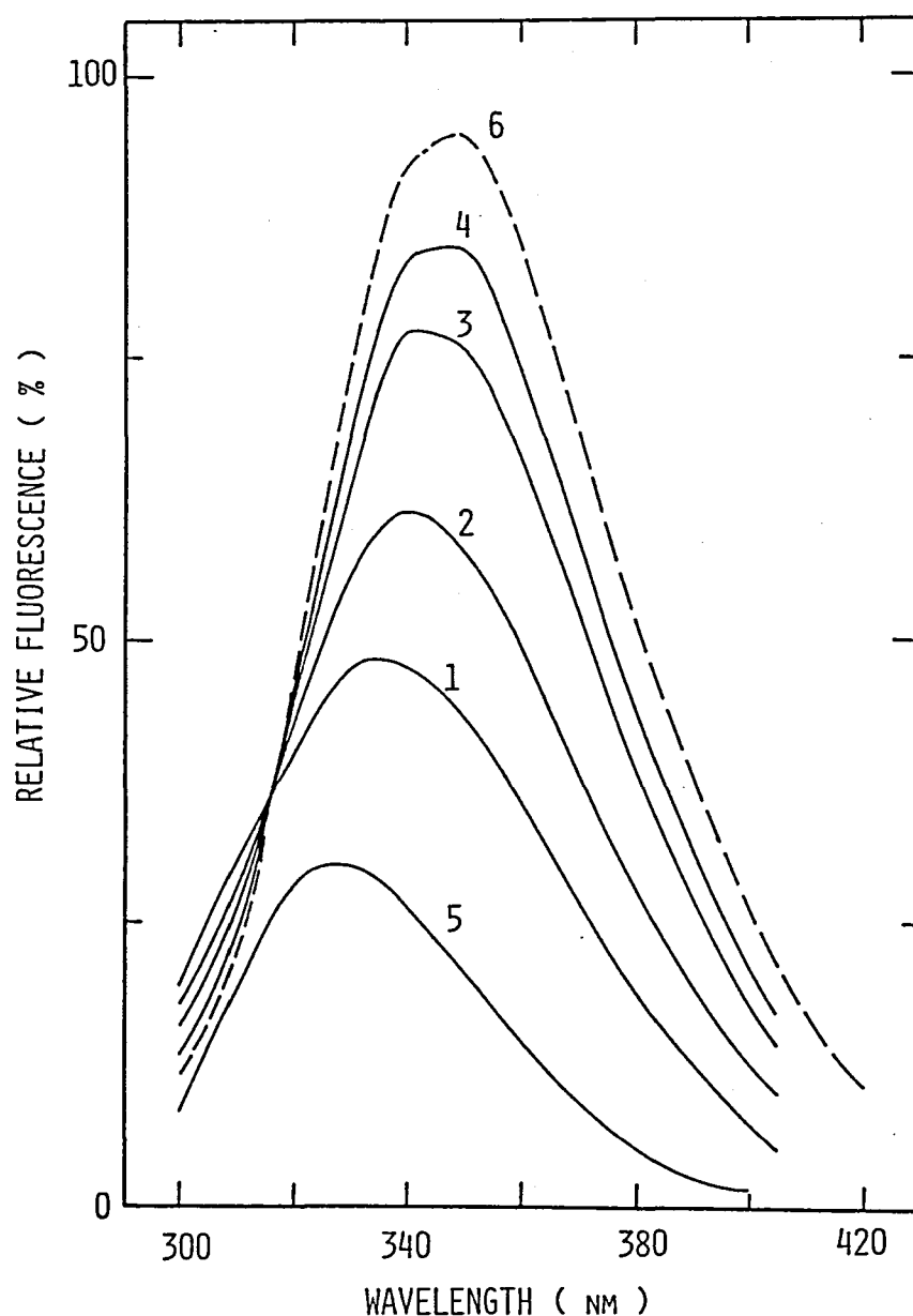
Fig. 4.11. Dependence on the final concentration of GuHCl of the fluorescence spectrum of the C_L fragment measured immediately after initiation of refolding. pH 7.5, 25°C. Initial conditions: protein concentration, 1 mg/ml; 4 M GuHCl. Final conditions: protein concentration, 0.02 mg/ml; (1), 0.07 M; (2), 0.26 M; (3), 0.46 M; (4), 0.66 M GuHCl. Curves 5 and 6 show the fluorescence spectra of native C_L fragment and reduced and alkylated C_L fragment, respectively.
