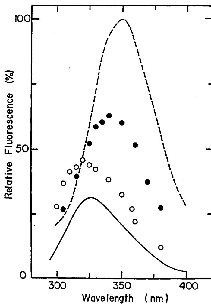
Fig. 4.10. The initial points for the slow phases of refolding kinetics of the C_L fragment in 0.07 M GuHCl (○) and 0.4 M GuHCl (●) measured by fluorescence at various wavelengths. pH 7.5, 25°C. Initial conditions: protein concentration, 1 mg/ml; 4 M GuHCl. Final protein concentration, 0.02 mg/ml. The solid and broken lines indicate the spectra of native protein and unfolded protein in 4 M GuHCl, respectively.
