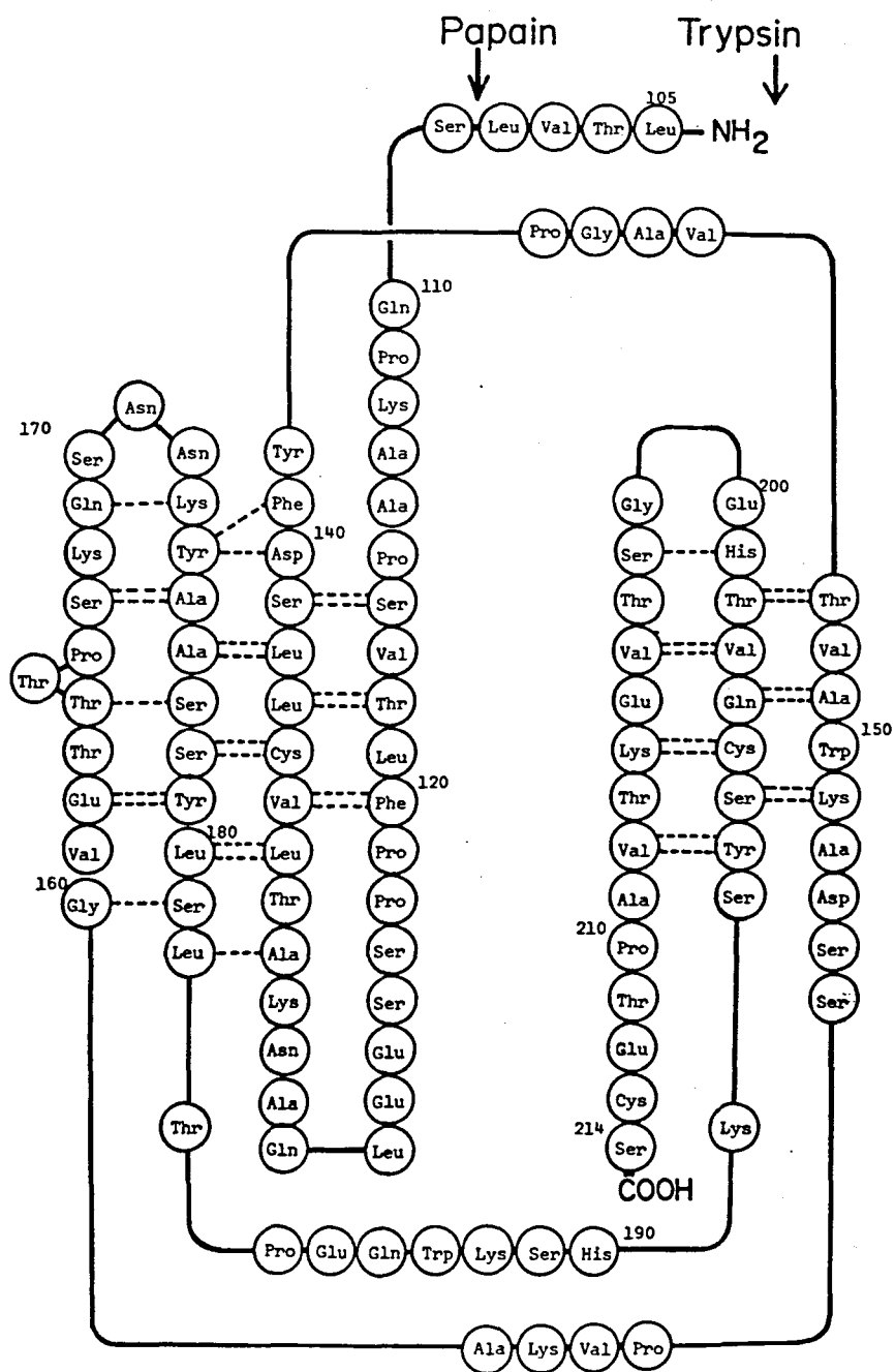
Fig. 3.1. Diagram of amino acid sequence and hydrogen bonding (broken line) between the main chain atoms of C L fragment. The hydrogen bonded clusters correspond to the two \beta -sheet structures of the domain. Produced from the original diagram by Amzel and Poljak (1979).
