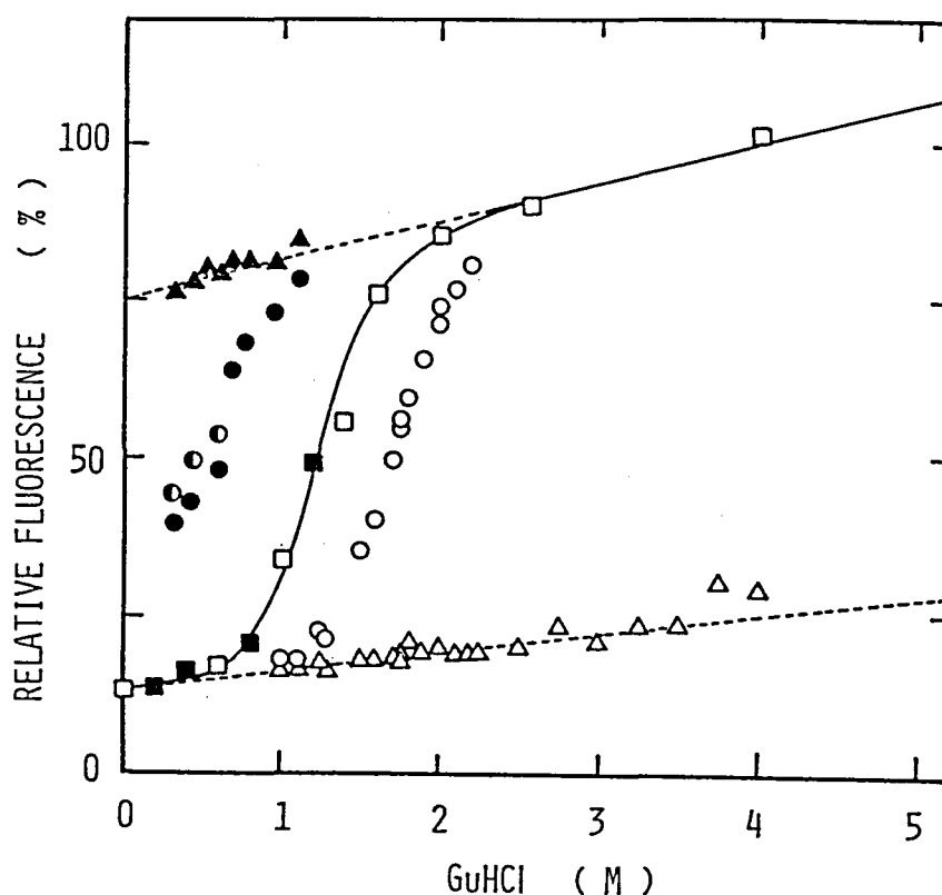
Fig. 4.4. Equilibrium and kinetic data for the denaturation of the C_L fragment by GuHCl, at 25°C and pH 7.5. Measurements were carried out by fluorescence using a stopped-flow apparatus. Unfolding ( \square ) and refolding ( \blacksquare ) equilibria were measured at a protein concentration of 0.02 mg/ml. The initial points of the slow and fast phases of unfolding kinetics are shown by \circ , and \triangle , respectively, and the initial points of the slow, fast, and intermediate phases of refolding kinetics are shown by \bullet , \blacktriangle , and \odot , respectively. They were obtained by extrapolating the respective phases to time zero. The initial concentrations of GuHCl for the unfolding and refolding kinetic experiments were 0 and 2.5 M, respectively. The initial protein concentration for unfolding and refolding kinetic experiments were 0.04 and 0.15 mg/ml, respectively. All measurements were made at a protein concentration of 0.02 mg/ml. The solid line indicates the theoretical curve constructed using Eqs. (3.1) and (3.2) and the values of \Delta n and \Delta G_D^{H_2O} obtained on the basis of k = 0.6 (Table 3.II) (see Chapter 3)
