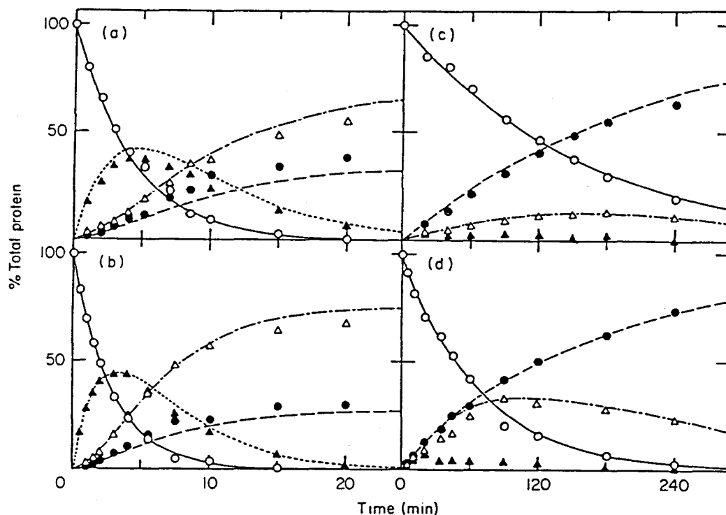
Fig. 7.3. Kinetics of the reaction of reduced C_L fragment with (a) 2 mM and (b) 3 mM GSSG in the presence of 8 M urea and with (c) 3 mM and (d) 9 mM GSSG in the absence of urea. Reduced C_L fragment (0.03 mM) was reacted with GSSG at pH 8.1 and 25°C, and the time-dependent concentrations of C_{LSH}^{SH} (O), C_{LSH}^{SSG} (▲), C_{LSSG}^{SSG} (Δ), and C_{LS}^S (●) were determined electrophoretically as in Fig. 7.2. The curves for (a) and (b) were calculated with kinetic mechanism 7.1 (see the text) and the values for the rate constants in Table 7.I, and the curves for (c) and (d) were calculated with kinetic mechanism 7.3 (see the text) and the values for the rate constants in Table 7.I.
