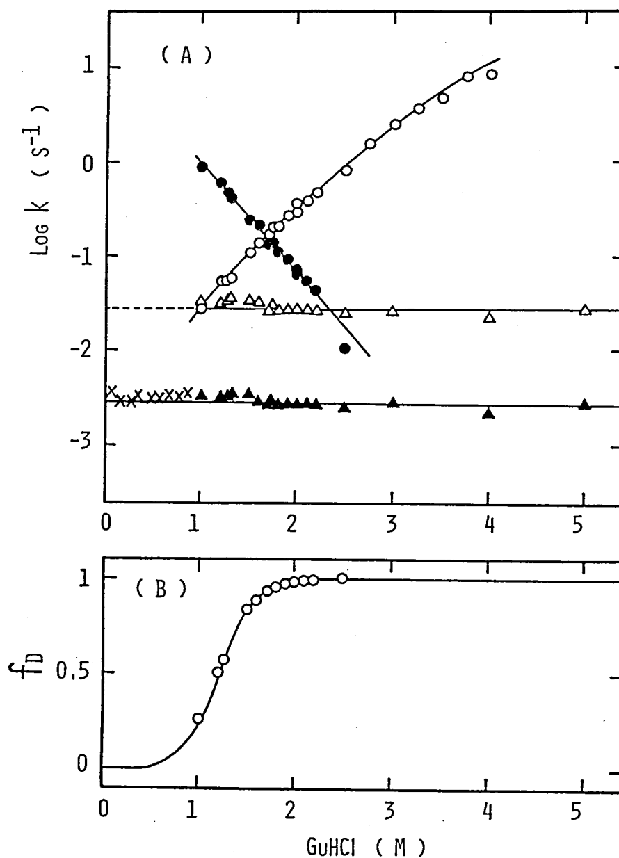
Fig. 4.13. Dependence on GuHCl concentration of the microscopic rate constants estimated based on mechanism 4.1 for folding of the C_L fragment (A) and the transition curve for unfolding calculated using the microscopic rate constants (B). pH 7.5, 25°C. ( \circ ), k_{32} ; ( \bullet ), k_{23} ; ( \triangle ), k_{21} ; ( \blacktriangle ), k_{12} . The crosses represent the values of \lambda_1 taken from Fig. 4.3. The solid line in (B) indicates the transition curve for unfolding obtained from equilibrium measurement.
