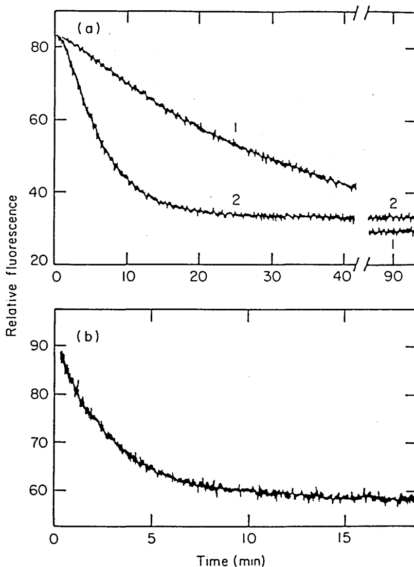
Fig. 7.6. (a) Kinetics of the reaction of C_{LSSG}^{SSG} with GSH obtained by fluorescence measurement. Change with time in the fluorescence intensity at 350 nm excited at 295 nm was measured after the addition of GSH to 0.17 mM (1) and 1.25 mM (2) to a solution of C_{LSSG}^{SSG} (0.03 mM) at pH 8.1 and 25°C. (b) Kinetics of the formation of disulfide bond in C_{LSH}^{SSG} by a pH jump from 5 to 8.1. Change in the fluorescence intensity at 350 nm excited at 295 nm of a solution that contains C_{LSH}^{SSG} was measured after the pH of the solution was raised from 5 to 8.1.
