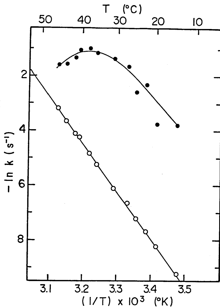
Fig. 5.5. The temperature-dependence of the apparent rate constant (○) for the slow phase determined by SH titration of the reduced C_L fragment by DTNB. The conditions are as described in the legend to Fig. 5.5. The closed circles represent the refolding rate ( k_{23} ) calculated with equation (5.2) and the values for K_{21} (= 10), f_D , and k_{23} (see the text).
