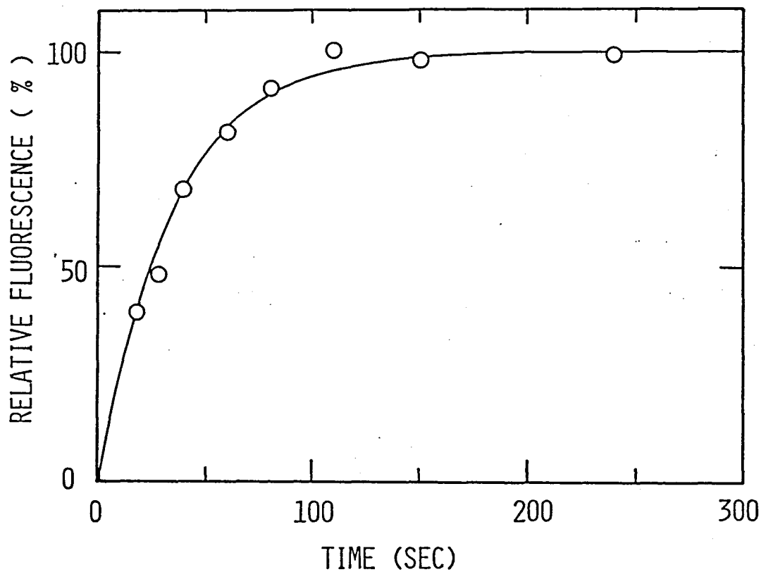
Fig. 4.5. A double-jump experiment measuring the process of U_2 to U_1 in mechanism 4.1 after unfolding. pH 7.5, 25°C. Formation of U_1 species was monitored by taking samples at the indicated times of unfolding and measuring the refolding kinetics by fluorescence at 350 nm. All the mixing procedures were made manually. The ordinate shows the fluorescence change for the slow phase observed in refolding process relative to the maximum fluorescence change obtained at infinite time in the unfolding conditions. Unfolding conditions: 3 M GuHCl; protein concentration, 0.6 mg/ml. Refolding conditions: 0.8 M GuHCl; protein concentration, 0.02 mg/ml. The solid line indicates the theoretical curve with a rate constant of 3.2 \times 10^{-2} \text{ s}^{-1} .
