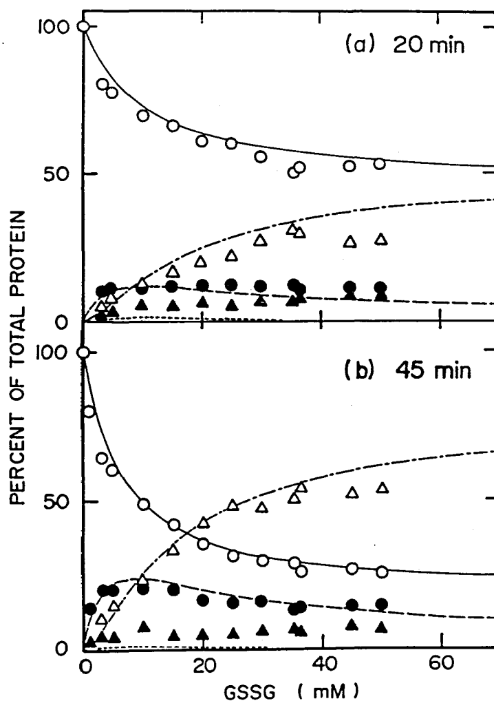
Fig. 7.4. Dependence on the GSSG concentration of the concentrations of species formed during regeneration of reduced C_L fragment. Reduced C_L fragment (0.03 mM) was reacted with various concentrations of GSSG for (a) 20 min and (b) 45 min, when the reaction was quenched by addition of iodoacetamide, and the concentrations of each species were determined electrophoretically. The symbols used are the same as for Fig. 7.3. The curves were calculated with kinetic mechanism 7.3 (see the text) and the values for the rate constants in Table 7.I.
