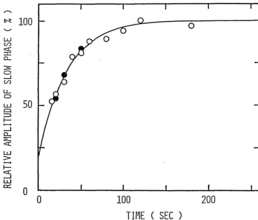
Fig. 5.3. A double-jump experiment measuring the process of U_2 to U_1 in mechanism 5.1 after unfolding. pH 7.5, 25°C. Formation of the U_1 species was monitored by taking samples at the indicated times of unfolding and measuring the refolding kinetics by fluorescence at 400 nm (○) or at 350 nm (●). All the mixing procedures were made manually. The ordinate shows the fluorescence change for the slow phase observed in refolding process relative to the maximum fluorescence change obtained at infinite time in the unfolding conditions. Initial conditions: 0 M GuHCl, protein concentration, 2.5 mg/ml. Unfolding conditions: 4 M GuHCl, protein concentration, 1.2 mg/ml. Refolding conditions: 0.07 M GuHCl, protein concentration, 0.02 mg/ml. The solid line indicates the theoretical curve with a rate constant of 3 \times 10^{-2} \text{ s}^{-1} .
