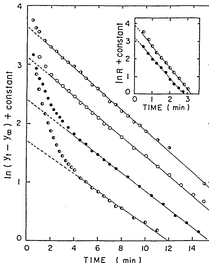
Fig. 6.9. First-order plots of the refolding reactions of Bence Jones protein Nag measured in terms of ultraviolet absorption at 292 nm (●), CD at 224 nm (○), tryptophyl fluorescence at 350 nm (●), and ANS fluorescence at 470 nm (○). The conditions for CD measurement were as described in the legend to Fig 6.7. For ultraviolet absorption measurements, the protein concentration was 0.43 mg/ml and the final GuHCl concentration was 0.08 M. For tryptophyl fluorescence measurements, the protein concentration was 0.02 mg/ml and the final GuHCl concentration was 0.03 M. Excitation was at 280 nm. ANS fluorescence was measured in the presence of 0.01 mM ANS and at a protein concentration of 0.16 mg/ml. The final GuHCl concentration was 0.07 M. Excitation was at 365 nm. The inset shows the first-order plots for the detectable fast phase. The fluorescence change in the first-order slow phase is subtracted from the observed fluorescence change, and the logarithm of the residue R is plotted against time. ○, Tryptophyl fluorescence; ●, ANS fluorescence.
