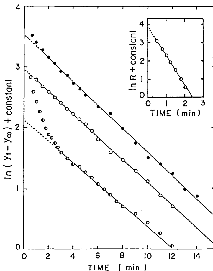
Fig. 6.10. First-order plots of the refolding reaction of Bence Jones protein T 0 d measured in terms of tryptophyl fluorescence at 350 nm (●), CD at 225 nm (○), and ANS fluorescence at 470 nm (◐). The conditions for CD measurement were as described in the legend to Fig. 6.7. For tryptophyl fluorescence measurements, the protein concentration was 0.043 mg/ml and the final GuHCl concentration was 0.03 M. Excitation was at 280 nm. ANS fluorescence was measured in the presence of 0.01 mM ANS and at a protein concentration of 0.14 mg/ml. The final GuHCl concentration was 0.1 M. Excitation was at 365 nm. The inset shows a first-order plot of the detectable fast phase measured in the presence of ANS.
