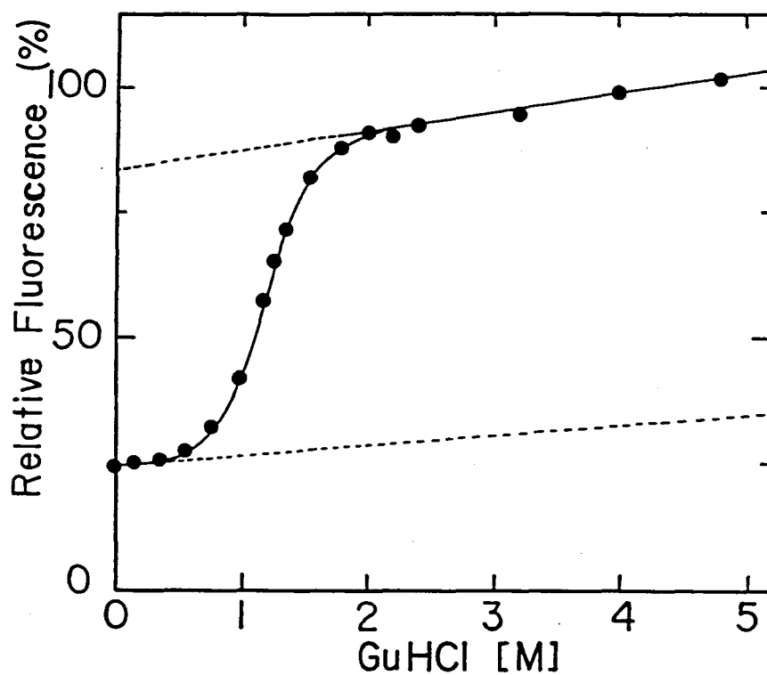
Fig. 3.11. Fluorescence at 350 nm of intact C_L fragment as a function of GuHCl concentration. pH 7.5, 25°C. Excitation wavelength, 295 nm; protein concentration, 0.04 mg/ml. Solid line indicates theoretical curve constructed using Eqs. (3.1) and (3.2) and the values of \Delta n and \Delta G_D^{H_2O} obtained on the basis of k = 0.6 (Table 3.II).
