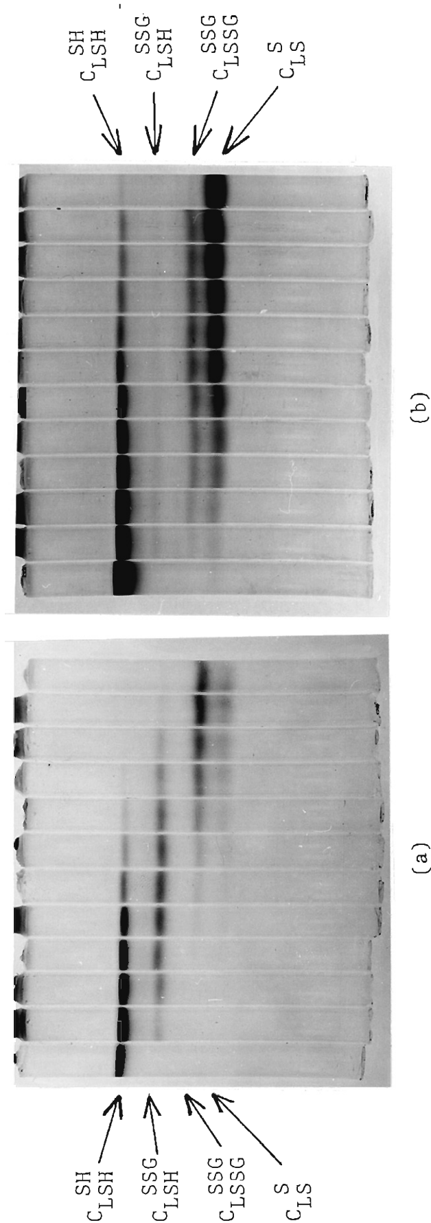
Fig. 7.1. Separation by gel electrophoresis in 15 % polyacrylamide at pH 9.5 of the species trapped during regeneration of reduced C_L fragment by 3 mM GSSG in the presence (a) and absence of 8 M urea (b). Reduced C_L fragment (0.03 mM) was regenerated at 25°C and at pH 8.1 for various times, when the reaction was quenched by addition of iodoacetamide to 0.1 M. Left to right: (a) 0, 0.5, 1, 1.5, 2, 3, 4, 5.5, 7.5, 10, 15 and 20 min; (b) 0, 0.2, 0.4, 0.7, 1, 1.5, 2, 2.5, 3, 3.5, 4 and 20 h.
