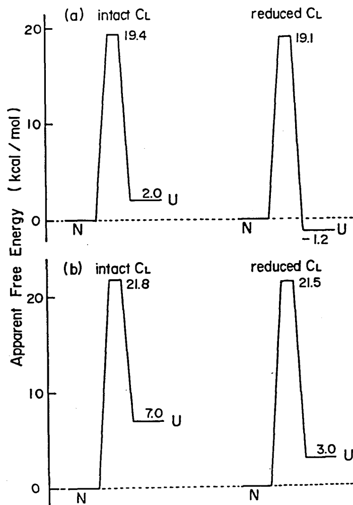
Fig. 5.8. Free-energy profiles for the unfolding and refolding of the intact and reduced C_L fragments in the presence of 1 M GuHCl (a) and in the absence of GuHCl (b). pH 7.5, 25°C. N and U represent the native and denatured states, respectively. The energy levels of the native states of the intact and reduced C_L fragments were set to zero (see the text).
