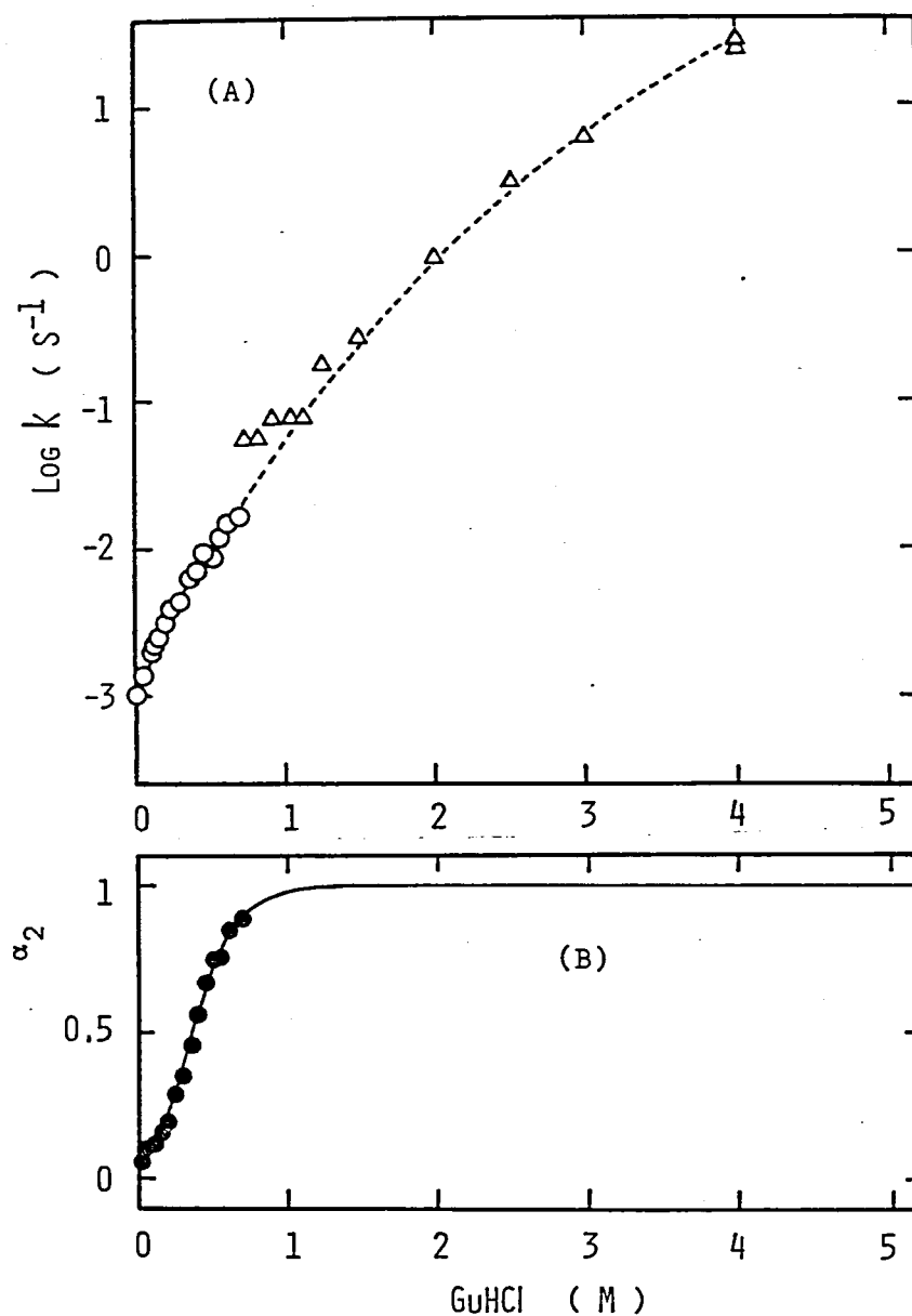
Fig. 5.4. The dependence on GuHCl concentration of the apparent rate constant (○) for the slow phase (A) and the relative amplitude of the fast phase (B) determined by SH titration of the reduced C_L fragment by DTNB. pH 7.5, 25°C. The SH groups of the reduced C_L fragment at a protein concentration of 0.06 mg/ml were titrated with 0.5 mM DTNB and the reaction was monitored by the absorbance change at 412 nm. The triangles in (A) represent the values of \lambda_2 shown in Fig 5.2(A).
