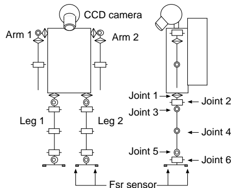
FIGURE 6.1: A model of biped locomotion robot
