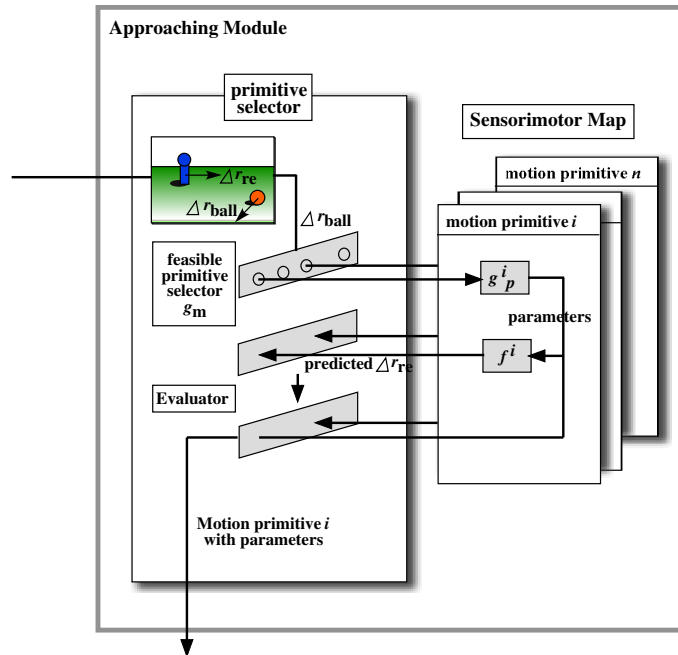
FIGURE 7.3: An overview of the approaching module
