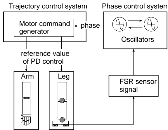
FIGURE 6.2: A walking control system
