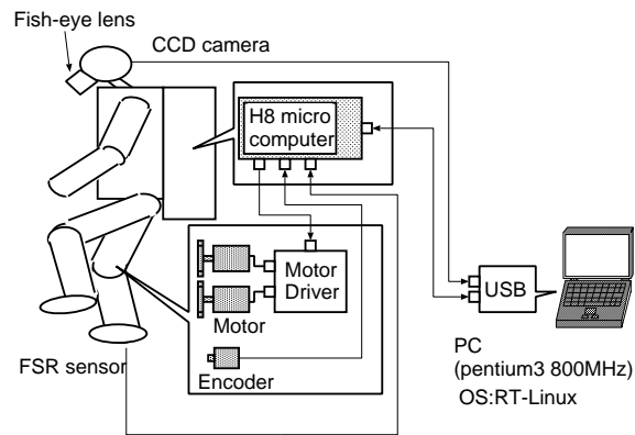
FIGURE 6.11: Overview of robot system
