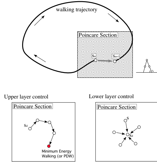
FIGURE 3.2: Poincaré section is taken at heel strike. On this plane, the lower layer of the controller tries to keep the state at heel contact in the same area as the desired one which is given by the upper layer. The upper layer of the controller tries to search the desired state which realize walking mode with minimum energy.
