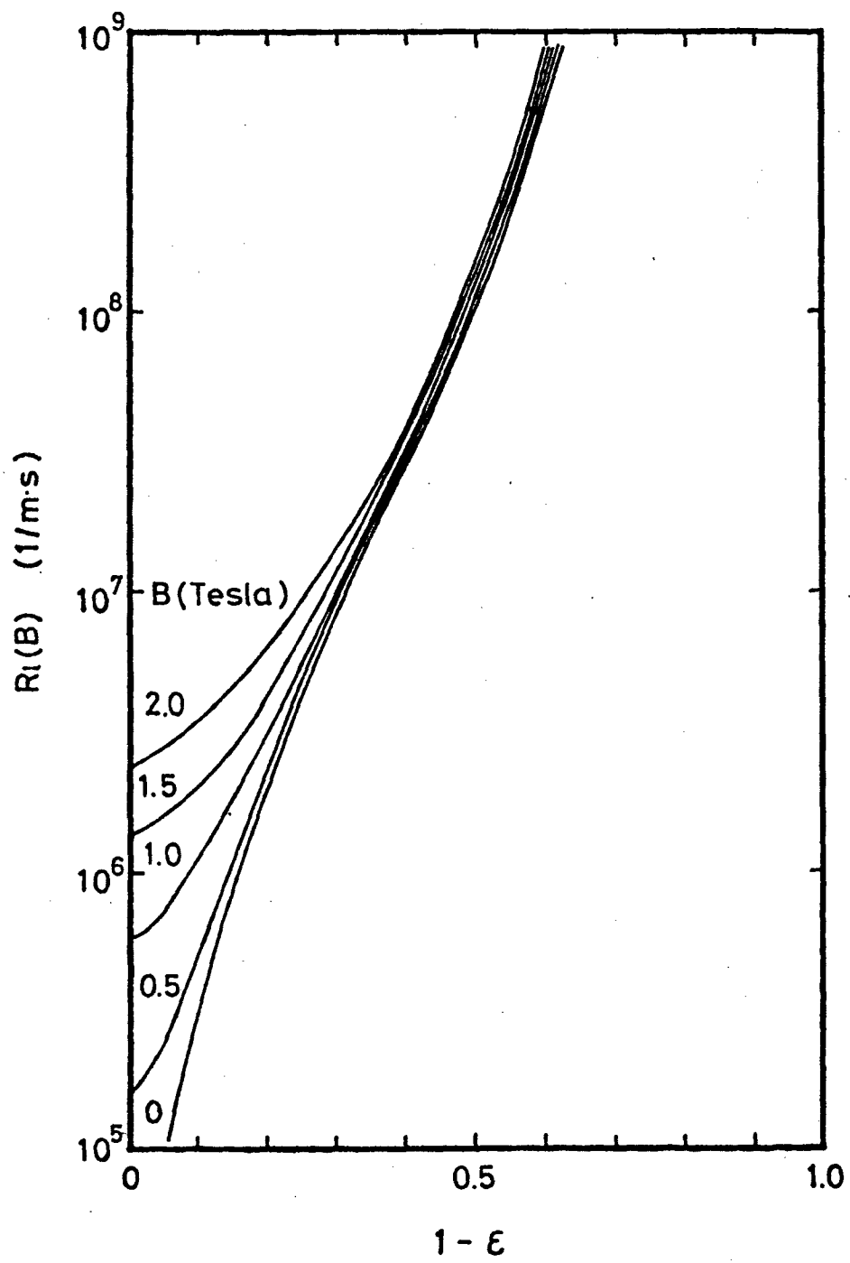
Fig.4-6 R_l(B) vs. (1 - \epsilon)
