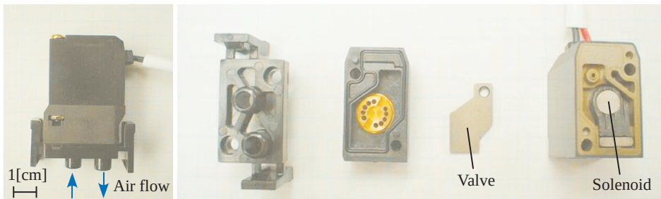
Fig. 2.2 High-speed solenoid valve (Satake Co. Ltd.)
