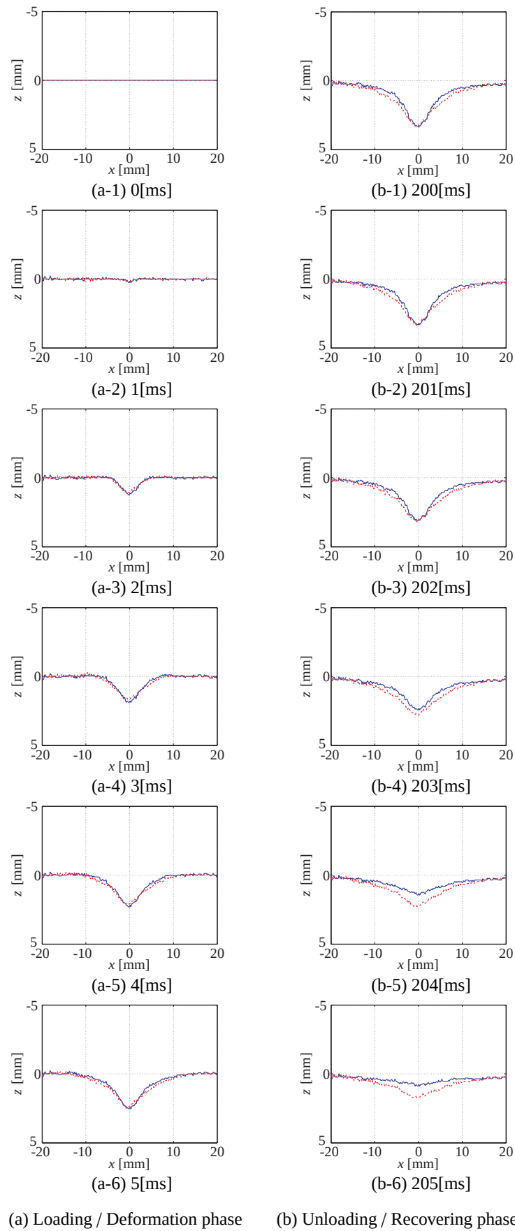
Fig. 2.9 2D deformation
