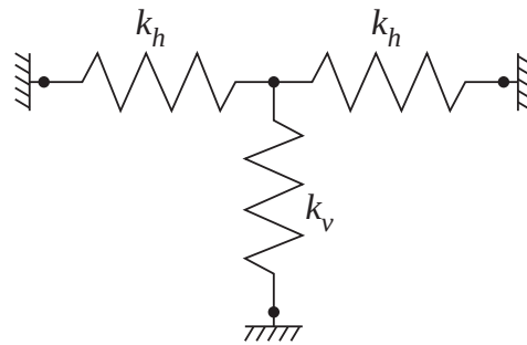
Fig. 7.1 Deformation model
