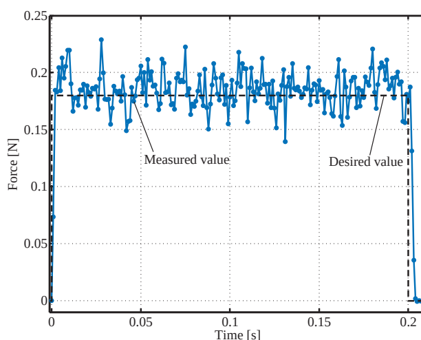
Fig. 2.7 Time history of external force
