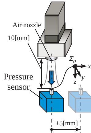
Fig. 2.5 Pressure measurement
