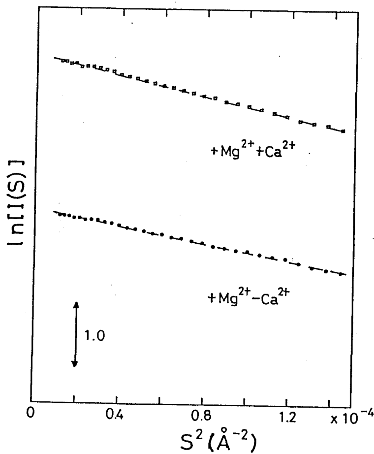
Figure 14: The Guinier plots, \ln[I(S)] vs. S^2 of SAXS profiles from Tn-C solutions that contain different amounts of \text{Ca}^{2+} in the presence of \text{Mg}^{2+} ; \text{Mg}_2\text{Ca}_0\text{Tn-C} ( \circ ) and \text{Mg}_2\text{Ca}_2\text{Tn-C} ( \square ). The sample buffer was 0.1 M KCl, 2mM EGTA, 2 mM \text{MgCl}_2 , and 10 mM MOPSO//KOH(pH 7.0). The concentration of Tn-C was 8 mg/ml.
