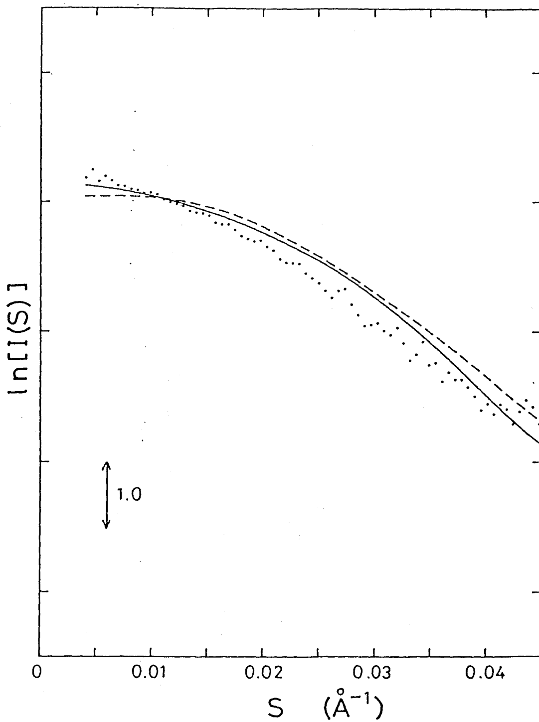
Figure 24 (a): SAXS profile calculated from the structure of TRIC in crystalline state. The dotted line represents \text{Ca}^{2+} -free TRIC. Symbols are the same as in Figure 23.
