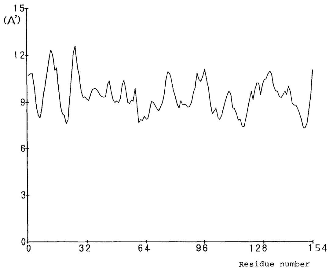
Fig. 4-12 Temperature factors of the \text{Ca} atoms.
