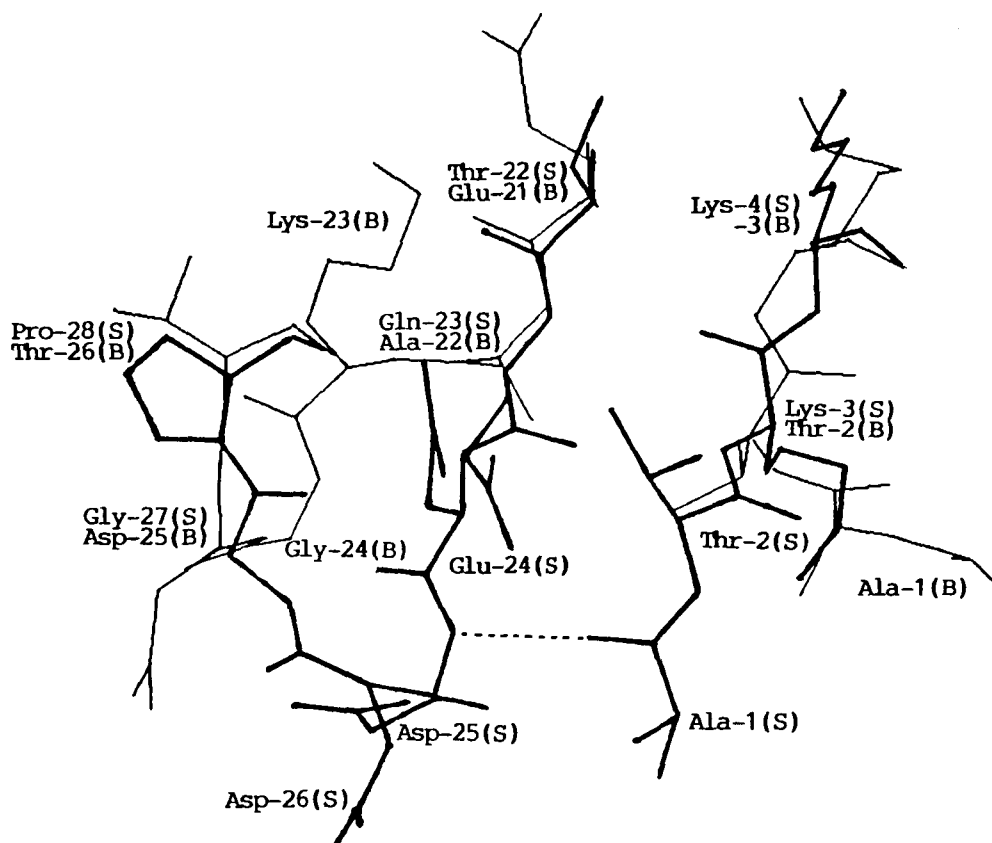
Fig. 5-5 Most different region comparing between spinach and bovine SODs (Group I in text). The thick line is spinach SOD and the thin is bovine one. (B) indicates bovine SOD and (S) indicates spinach SOD. The dotted line is the hydrogen bond between the hydrogen atom of N-H in Asp-25 and the oxygen atom of C-O in Ala-1.
