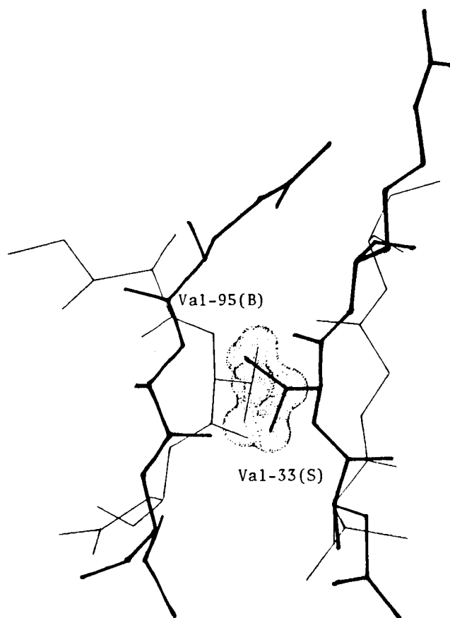
Fig. 5-6 Residue replacement (Group II in text). The thick line is spinach SOD and the thin is bovine one. Side chains of both Val-33 of spinach SOD and Val-95 of bovine SOD are shown with their molecular surfaces. (B) indicates bovine SOD and (S) indicates spinach SOD.
