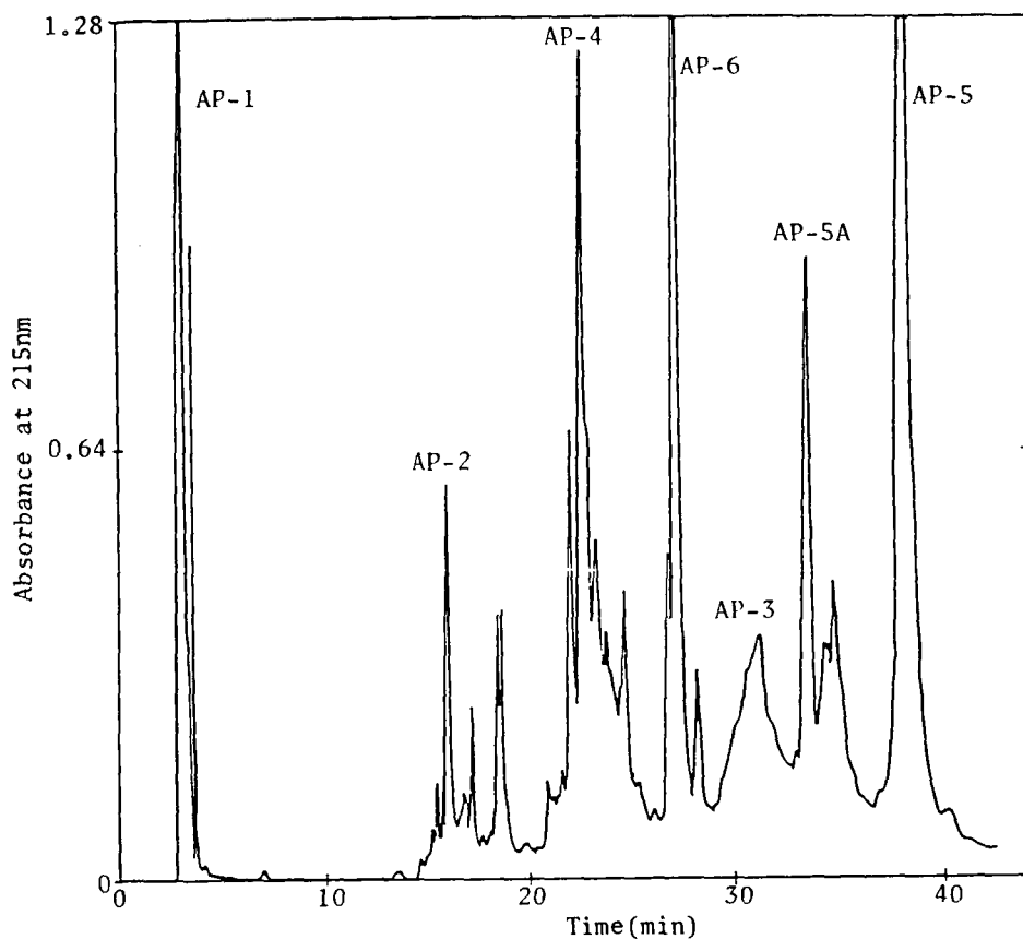
Fig. 3-2 Separation of peptides obtained by A. lyticus lysylendopeptidase digestion of the performic acid-oxidized enzyme by HPLC. The sample was dissolved in 100 \mu l of 0.1% trifluoroacetic acid and chromatographed on a Baker bond wide pore butyl column (0.46 x 25 cm, C4, 330 A) at a flow rate of 1.0 ml/min. For other details, see text. Peptides in the peaks indicated were collected and lyophilized. Some other peaks in the figure were not collected because of their low yields.
