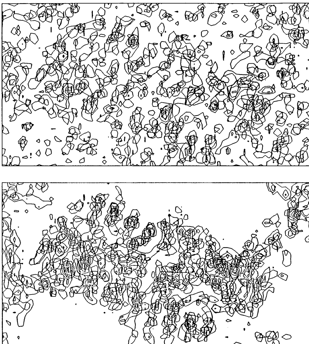
Fig. 4-4 The development of the electron density map using molecular replacement method. Upper is the original M.I.R. map at 2.8 Å resolution. Lower is the map after molecular replacement averaging at 2.5 Å resolution. Both of the map are viewed down along the 2-fold axis between the subunits.
