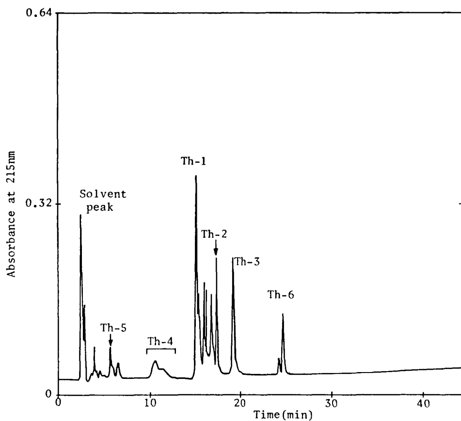
Fig. 3-3 Separation of thermolysin peptides from AP-5 by HPLC. The same conditions as described in Fig. 3-2 were used.
