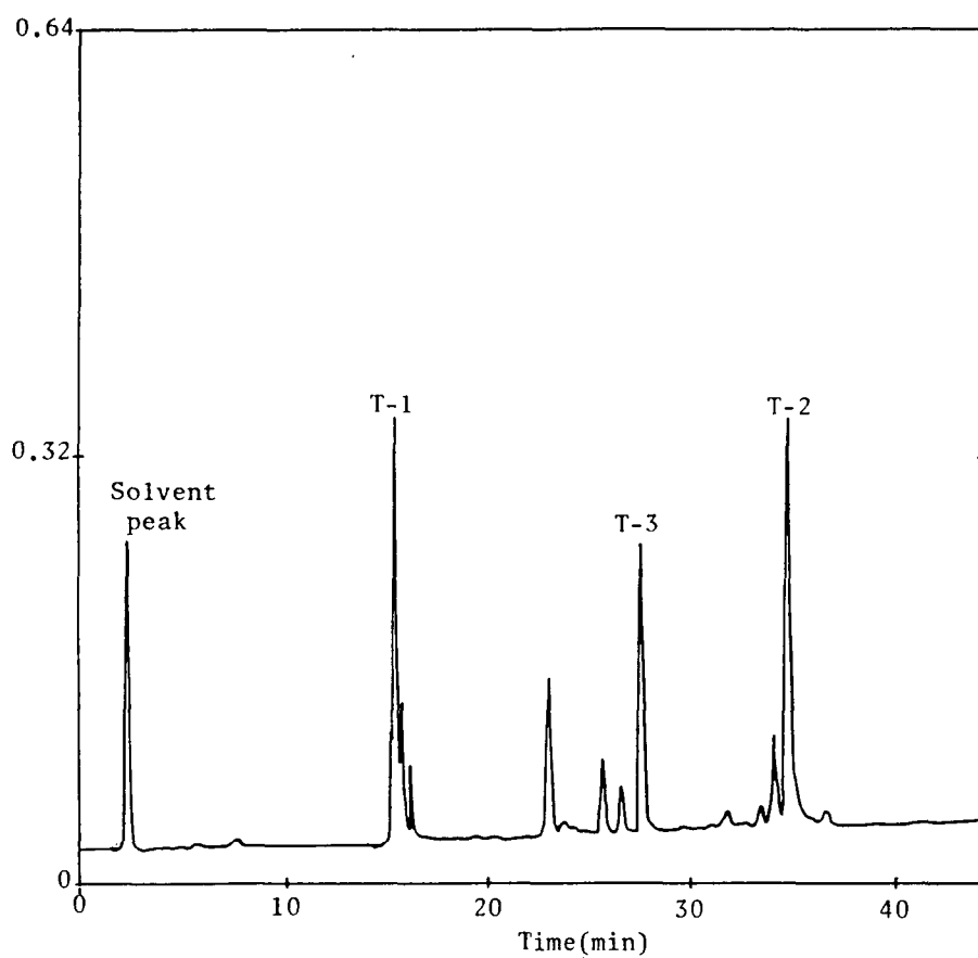
Fig. 3-4 Separation of tryptic peptides from AP-5 by HPLC. The same conditions as described in Fig. 3-2 were used.
