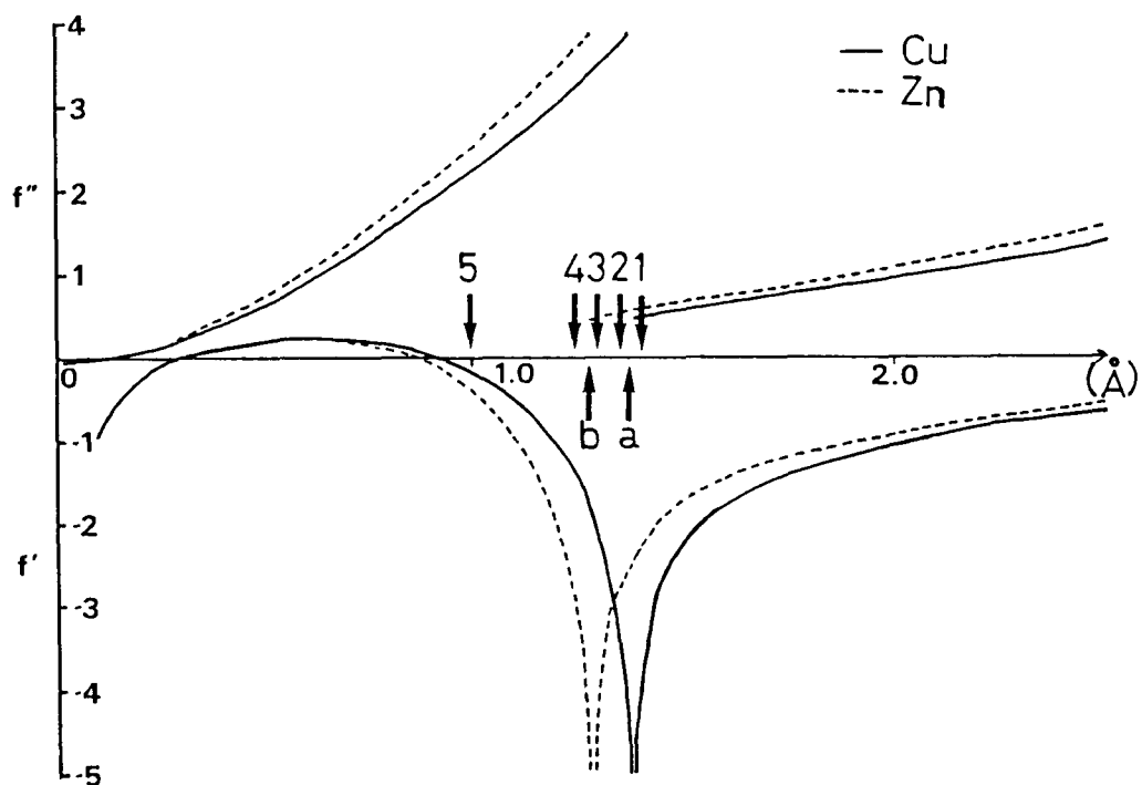
Fig. 4-6 Variation of f' and f'' of Cu and Zn with wavelength. The arrows with the numbers 1 to 5 indicate the wavelengths at which data were collected, and the arrows with the characters a and b are the absorption edges of Cu and Zn, respectively.
