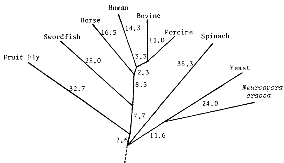
Fig. 5-8 Phylogenetic tree of Cu,Zn-SOD. The numbers along the branches show the inferred numbers of amino acid substitutions.
