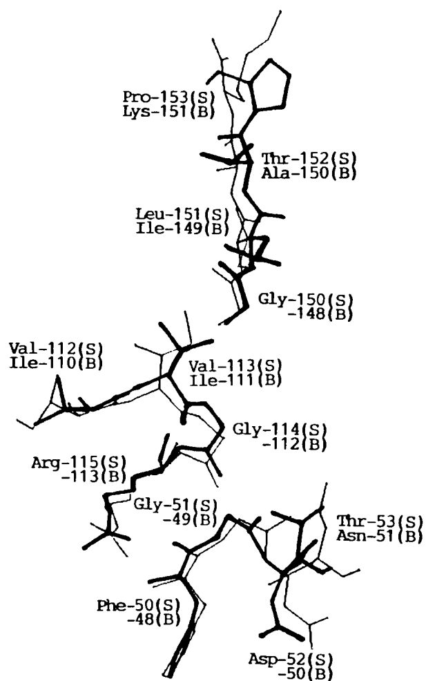
Fig. 5-4 Comparison of the dimer contact areas between spinach and bovine SODs. The thick line is spinach SOD and the thin is bovine one. (B) indicates bovine SOD and (S) indicates spinach SOD.
