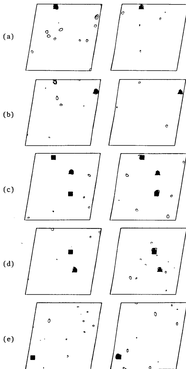
Fig. 4-7 Anomalous difference Fourier maps: left-hand side, 1.373 Å data set; right-hand side, 1.275 Å data set. The triangles are four \text{Cu}^{2+} ion positions and the squares are four \text{Zn}^{2+} ion positions in an asymmetric unit. The sections are (a) 4/50, (b) 6/50, (c) 13/50, (d) 17/50, and (e) 24/50 of the crystallographic b axis. At 4/50 and 6/50, the same peaks appear on the left-hand map. Contours are in equal intervals of positive density and are chosen to show the highest peak in each map with four contour levels. The edges of the maps correspond to half the unit cell in a along the horizontal direction and the full unit cell in c along the vertical direction.
