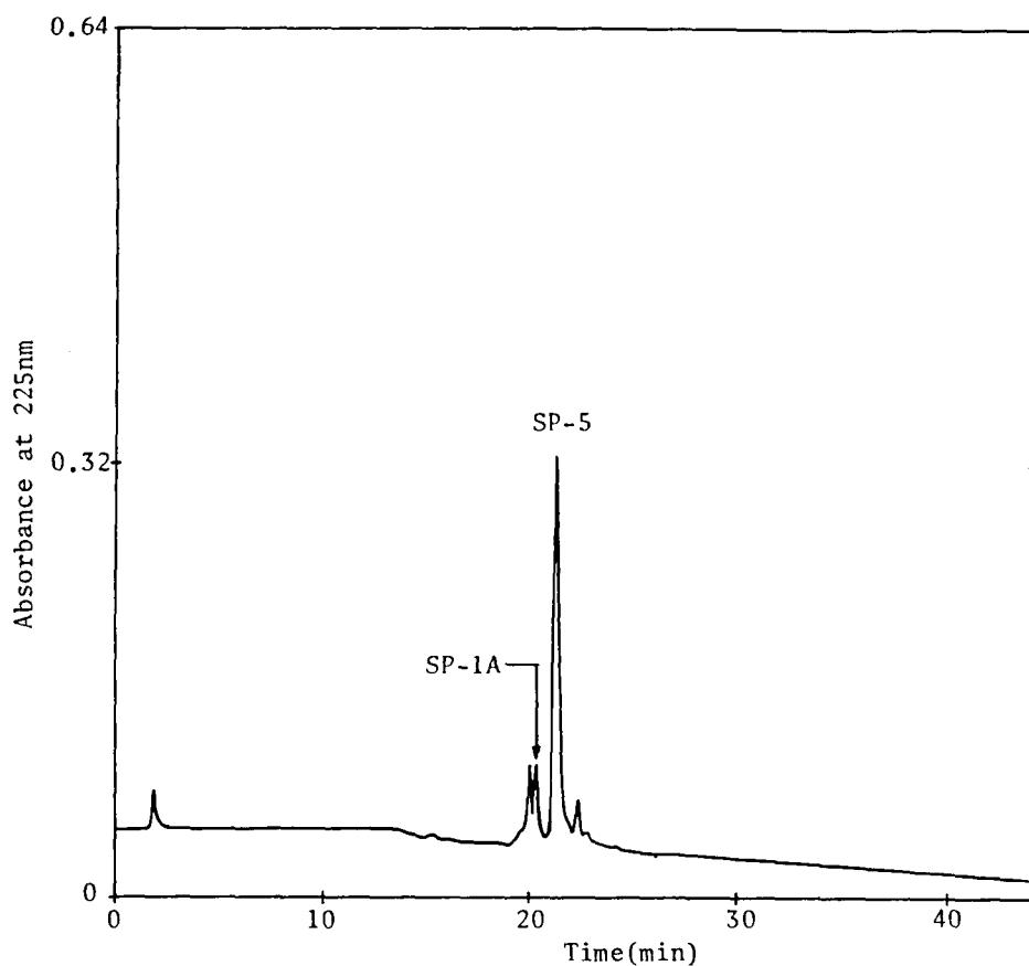
Fig. 3-6 Rechromatography of fraction SP-A by HPLC. The sample was dissolved in 100 \mu l of 0.1 M ammonium formate and chromatographed on a Baker bond wide pore butyl column (0.46 x 25 cm, C4, 330 A) at a flow rate of 1.0 ml/min.
