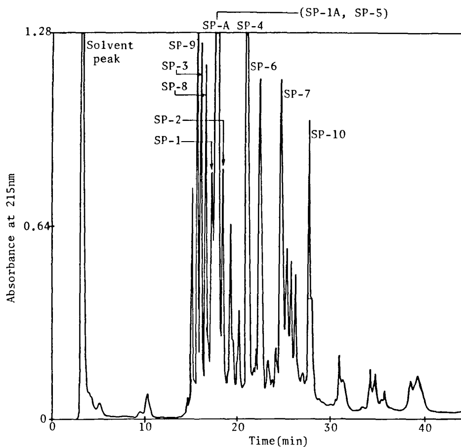
Fig. 3-5 Separation of peptides obtained by S. aureus V8 protease digestion of the performic acid-oxidized enzyme by HPLC. The same conditions as described in Fig. 3-2 were used.
