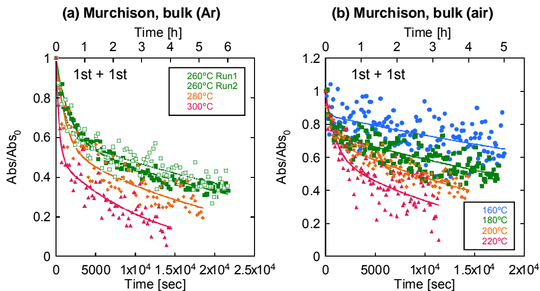
Fig. 5-2. The decrease with time of the peak height of aliphatic C-H (2930 cm -1 ) normalized to that at t = 0 sec (Abs 0 ) during the heating experiments of bulk Murchison meteorite. (a) 2 runs under Ar flow at 260°C, 280°C and 300°C. (b) Under air at 160°C, 180°C, 200°C and 220°C. The fitting curves were based on the combination of two first-order reaction model (eq. 5-6) (see 5.4.4).
