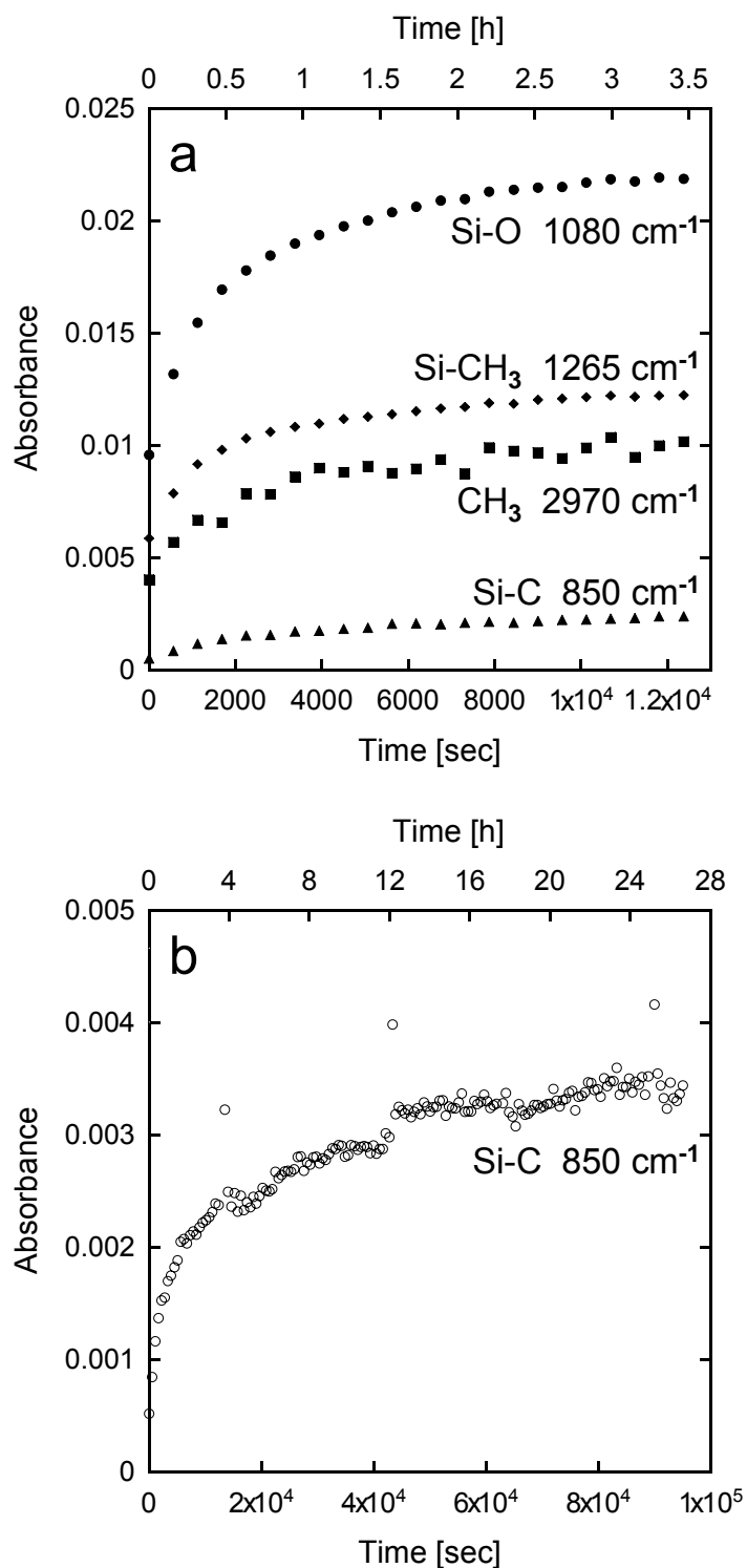
Fig. 2-6. Changes with time in infrared absorption peak heights of volatiles from the silicone rubber in the long path gas cell. (a) 2970 cm -1 peak due to CH 3 , 1265 cm -1 peak due to Si-CH 3 , 1080 cm -1 peak due to Si-O, and 850 cm -1 peak due to Si-C for 3.5 hours. (b) 850 cm -1 peak due to Si-C for 26 hours.
