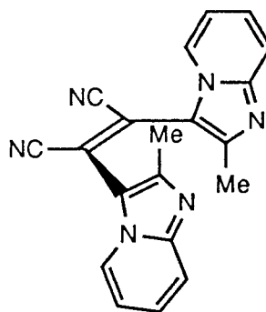
anti-parallel orientation
