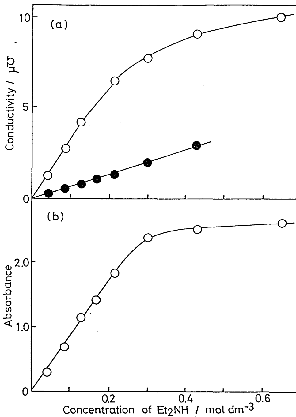
Figure 4-2. (a) Conductivity change of 18\text{E-Et}_2\text{NH} system in \text{CH}_2\text{Cl}_2 . ( \circ ), with 18\text{E} ( 4.3 \times 10^{-5} \text{ mol dm}^{-3} ); ( \bullet ), without 18\text{E} . (b) Absorption intensity change of 18\text{E-Et}_2\text{NH} system in \text{CH}_2\text{Cl}_2 at 510 nm.
