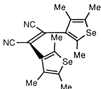
Anti-parallel orientation
