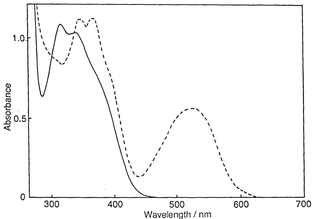
Figure 1-1. Absorption spectra of 5Z ( 1.6 \times 10^{-4} mol dm ^{-3} ) (—) and in the photostationary state under irradiation with 313 nm light (---).
