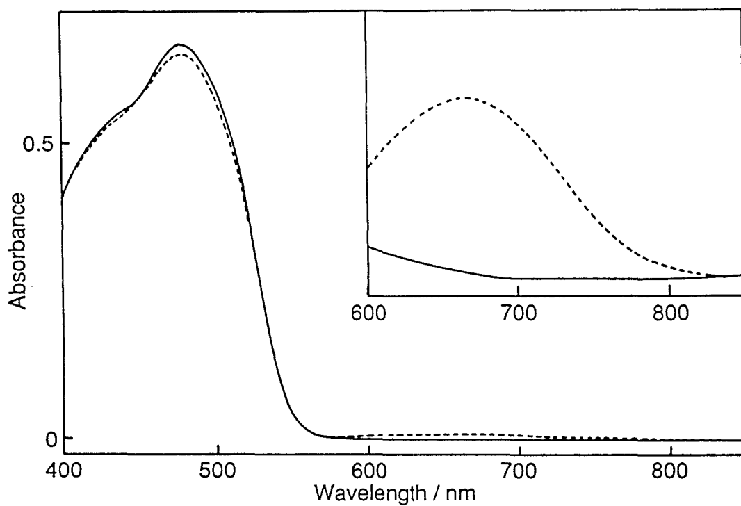
Figure 1-8. Absorption spectra of 10Z ( 1.0 \times 10^{-4} mol dm ^{-3} ) (—) and in the photostationary state under irradiation with 490 nm light (---).
