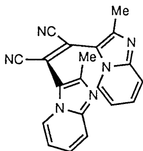
parallel orientation
