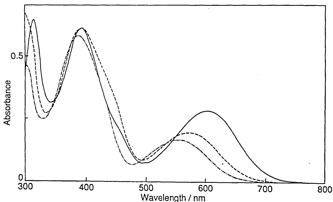
Figure 2-3. Absorption spectra of 13Z + 13C (total concentration, 1.0 \times 10^{-4} mol dm -3 ) at the photostationary state in hexane (---), in benzene (-.-) and in HMPA (—). Conversion from the open-ring to the closed-ring form was 39% in hexane, 44% in benzene, and 75% in HMPA. The absorption bands longer than 500 nm and at around 400 nm are ascribable to 13C , and shoulders at around 450 nm to 13Z .
