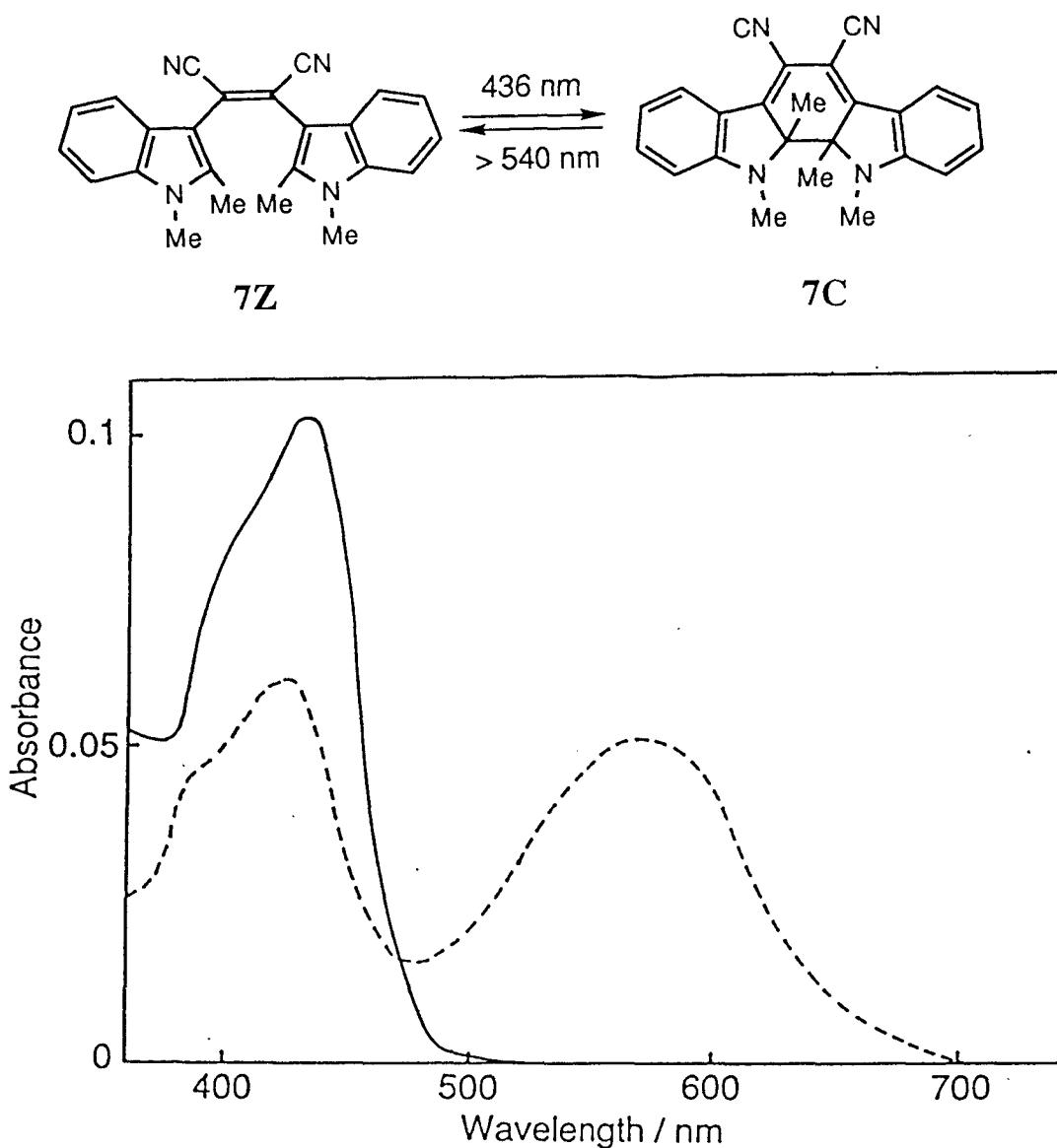
Figure 1-5. Absorption spectra of 7Z (—) and 7C (---) ( 0.7 \times 10^{-5} mol dm -3 ) in benzene.
