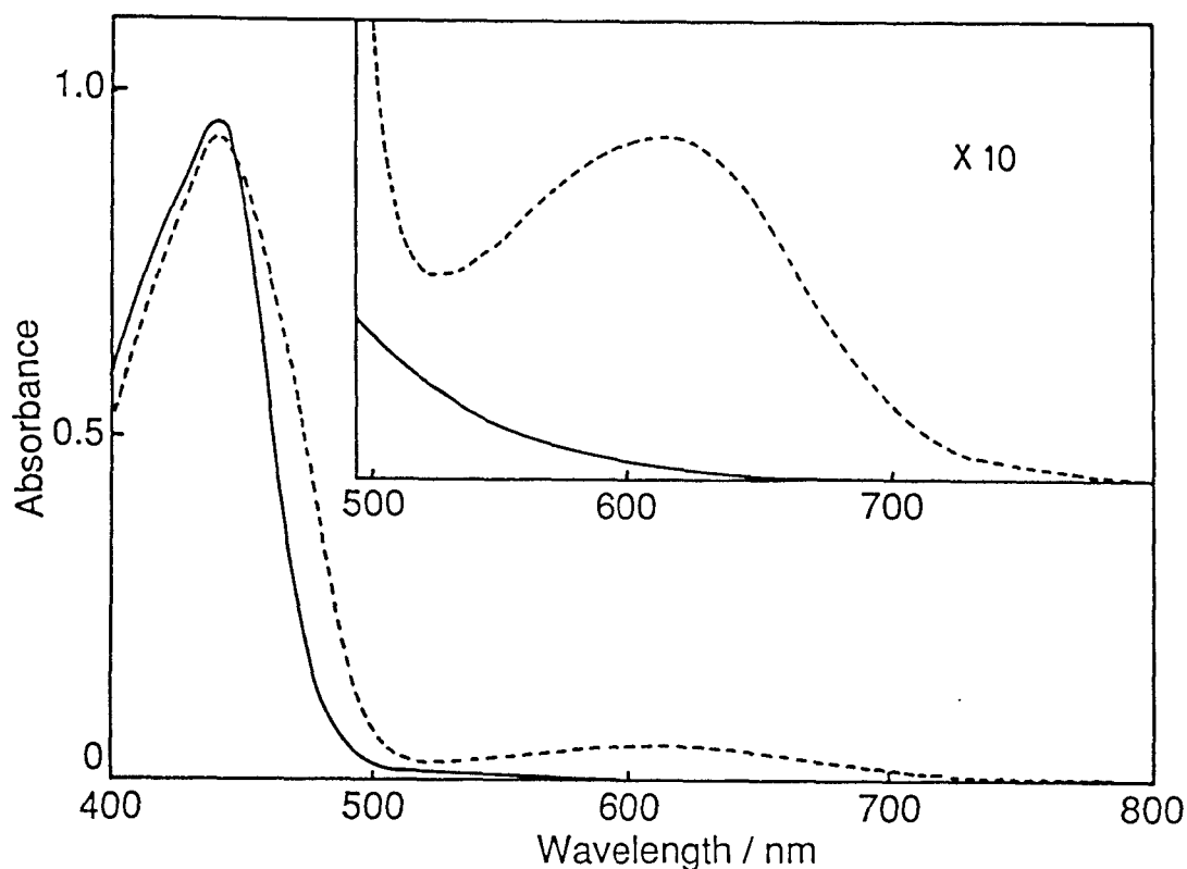
Figure 1-7. Absorption spectra of 9Z ( 1.0 \times 10^{-4} mol dm ^{-3} ) (—) and in the photostationary state under irradiation with 440 nm light (---).
