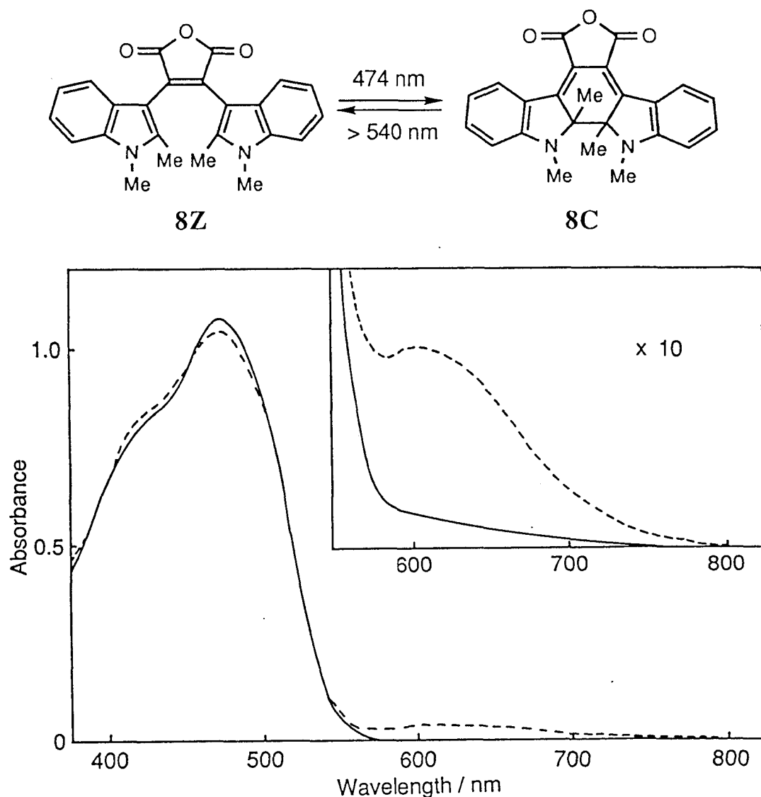
Figure 1-6. Absorption spectra of 8Z (1.1 × 10 -4 mol dm -3 ) (—) and in the photostationary state under irradiation with 436 nm light (---).
