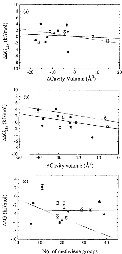
Figure III-7. Correlation of cavity volume and packing density with the thermodynamic parameters of denaturation for the mutant proteins. Val → Ala mutants are shown as solid circles and Ile → Val as open circles. The continuous lines show the linear regression of all the proteins. (a) \Delta\Delta G_{cav} ( = \Delta\Delta G - \Delta\Delta G_{tr} ) and the difference in the total cavity volume between each mutant protein and the wild-type structure using the probe size 1.20 Å (Connolly, 1983, 1993). (b) \Delta\Delta G_{cav} ( = \Delta\Delta G - \Delta\Delta G_{tr} ) and the difference in the total cavity volume between each mutant protein and the wild-type structure using the probe size 1.40 Å (Connolly, 1983, 1993). The \Delta\Delta G_{tr} values in Figures (a) and (b) are corrected by the accessibility of each residues. The dotted lines in Figures (a) and (b) indicate that proposed by Eriksson et al. (1992). (c) \Delta\Delta G and the packing density (number of methylene groups within 6 Å of the removed atoms). The dotted line shows the best fit of the barnase and chymotrypsin inhibitor 2 data to a linear equation obtained by Otzen et al. (1995).
