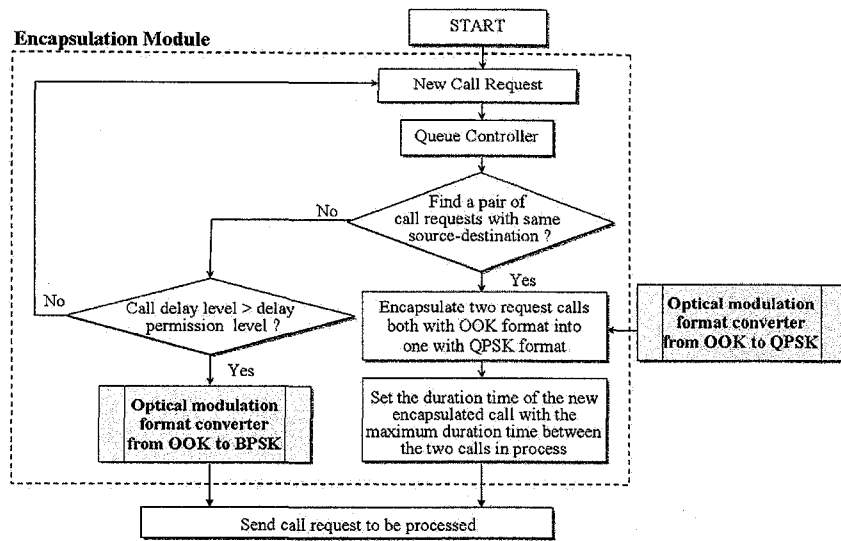
Fig. 4.4: Flow diagram of the optical modulation conversion functionality.
