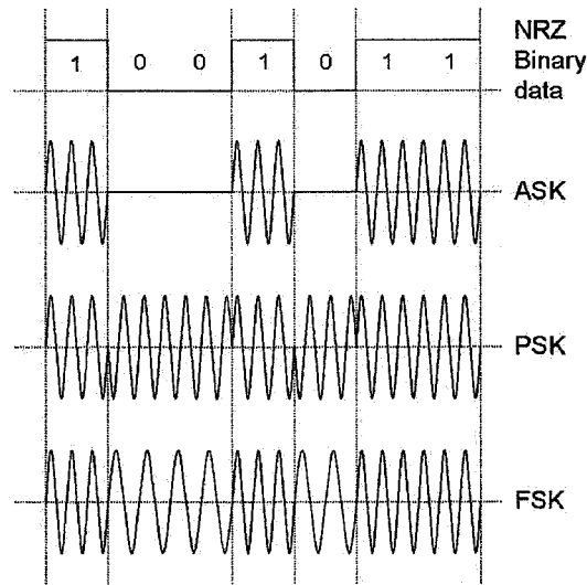
Fig. 2.4: Optical modulation formats.
