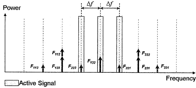
Fig. 2.1: Three copropagating equally-spaced channels with the generated products of frequencies f_{ijk} due to FWM crosstalk.
