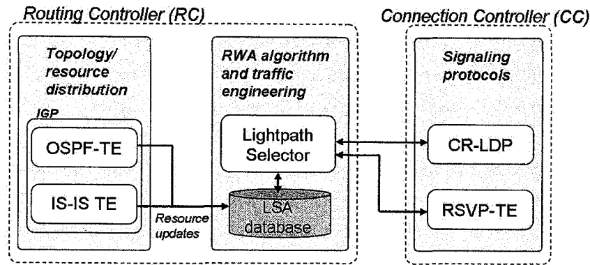
Fig. 1.3: GMPLS building blocks for lightpath routing.
