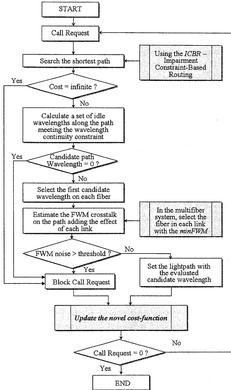
Fig. 3.1: Simulation Flow Diagram.
