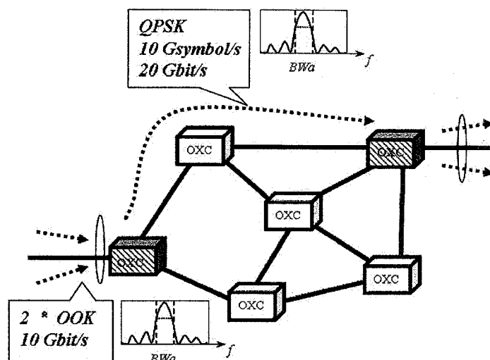
Fig. 4.2: Illustration of an all-optical modulation format conversion at the gateway node, lightpath from source to destination node with QPSK modulation format.
