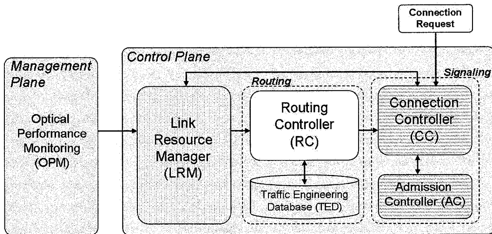
Fig. 1.2: Control plane of a distributed ASON/GMPLS-based architecture.
