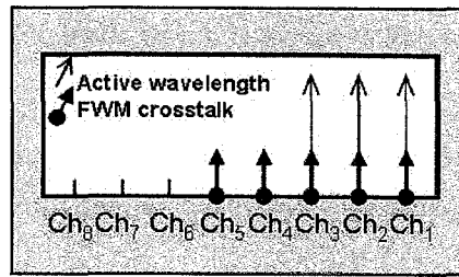
Fig. 3.10: FWM products illustration inside a system spectral window.
