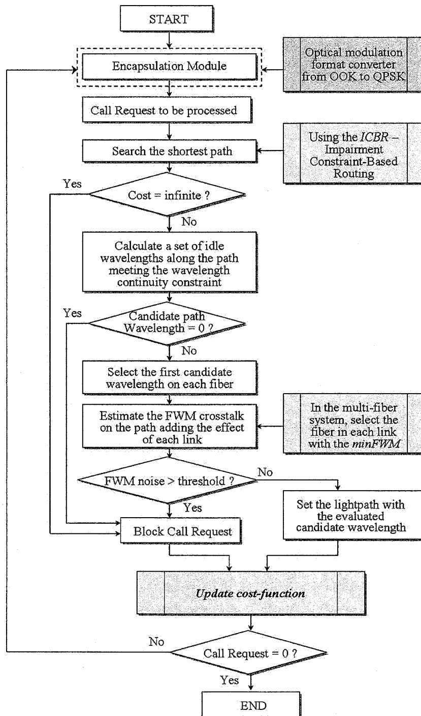
Fig. 4.3: Flow diagram of the simulation ICBR scheme incorporating the modulation format conversion interface.
