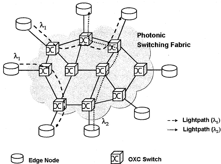
Fig. 1.1: Wavelength-routed optical network architecture.
