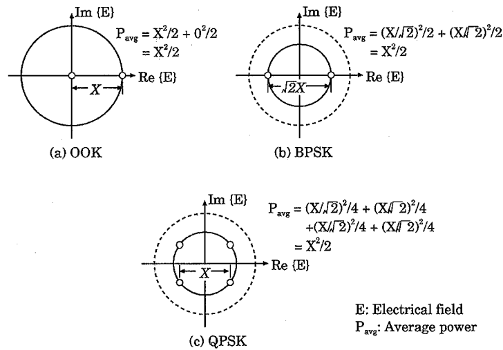
Fig. 2.5: Constellation diagram of OOK, BPSK and QPSK modulation formats.
