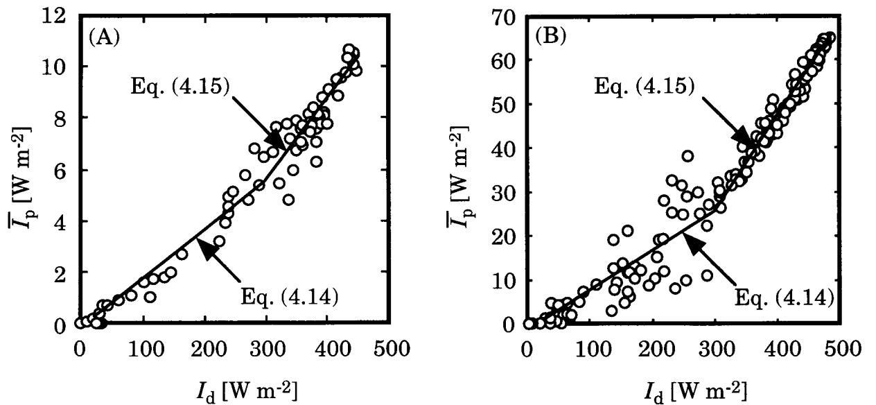
Fig. 4.10 Relationship between light intensity of direct irradiation from the sun and light intensity on surface of illumination plate. (A) Lens-type sunlight collection, (B) Mirror-type sunlight collection
