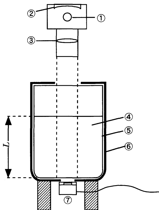
① 500 W xenon lamp, ② concave mirror, ③ convex lens, ④ cell suspension, ⑤ beaker of glass, ⑥ black paper, ⑦ quantum sensor
