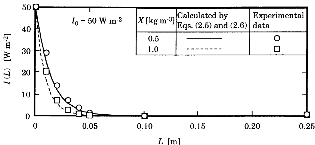
Fig. 2.8 Light intensity in cell suspension of Chlorella sp. UK001
