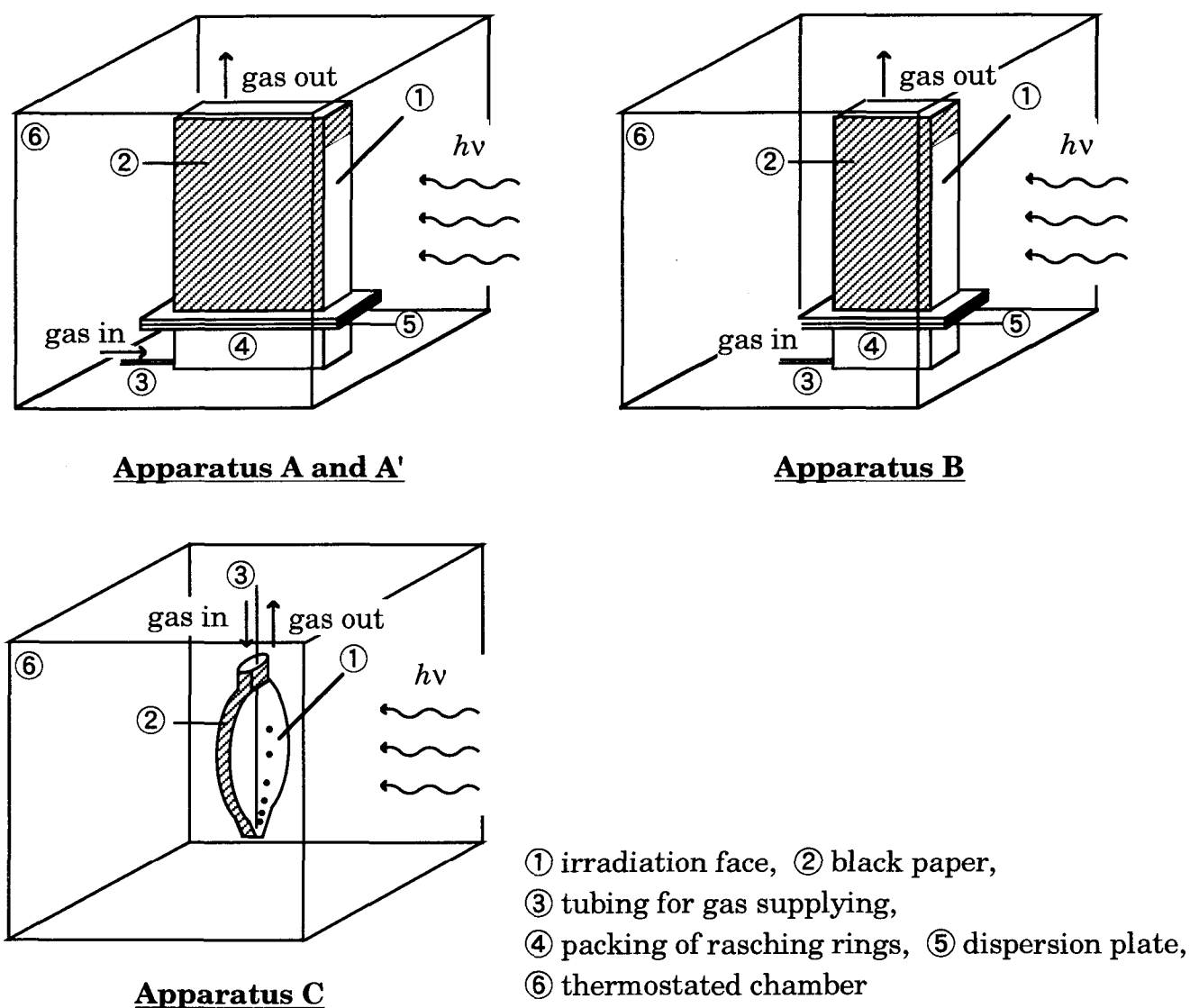
Fig. 3.1 Schematic drawing of culture apparatuses for microalgal cells
