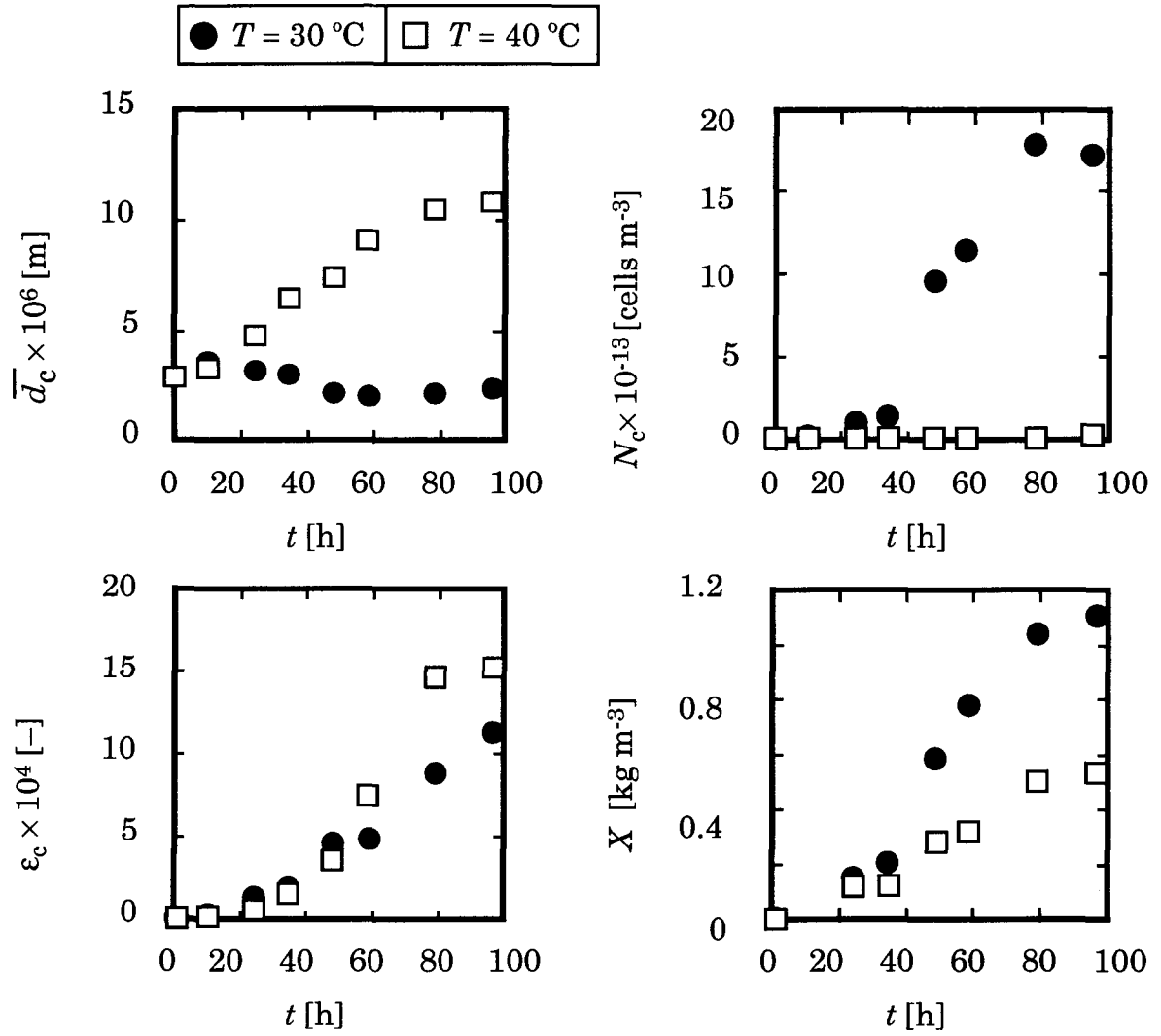
Fig. 1.14 Time courses of cultures of Chlorella sp. UK001 cell at 30 and 40 °C I_0 = 21.8 \text{ W m}^{-2} , N_c^0 = 2 \times 10^{12} \text{ cells m}^{-3} , d_c^0 = 2.3 \mu\text{m} (SD = 0.36 \mu\text{m} ), \epsilon_c^0 = 1.3 \times 10^{-5} , X^0 = 0.02 \text{ kg m}^{-3} , t = 96 \text{ h}
