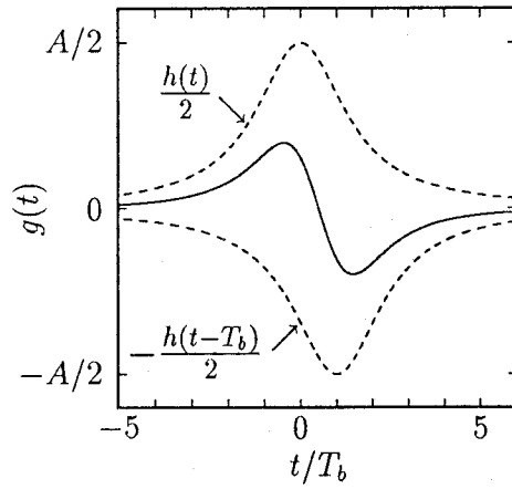
(b) Input waveform of equalizer ( K=3 )
