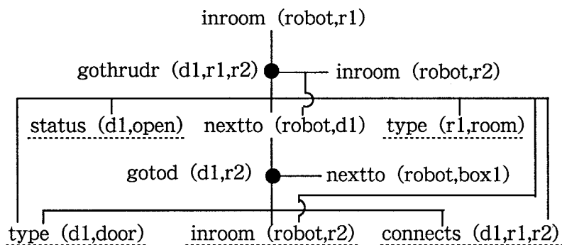
Fig.5.6 説明木
