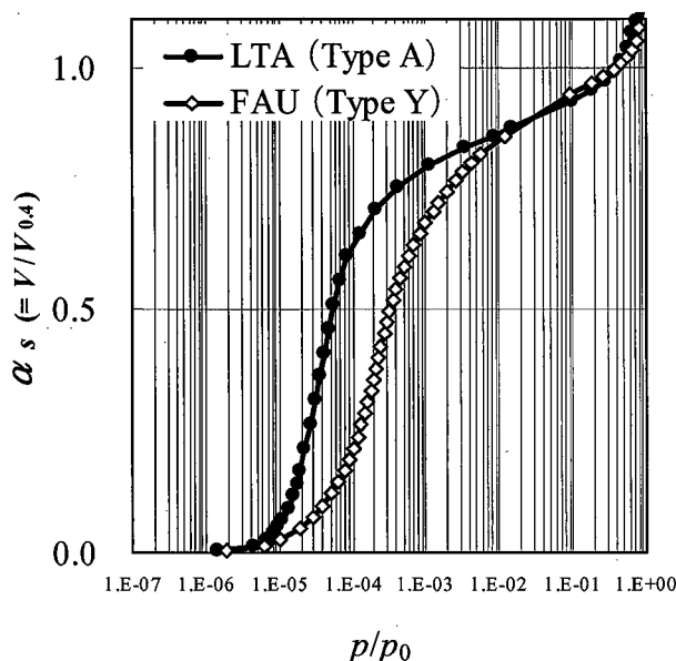
Figure 4-4. High resolution Ar adsorption isotherms at 87.3 K for zeolites of group B.
