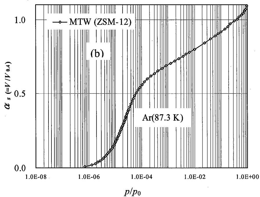
Figure 5-5. High resolution adsorption isotherms for zeolites ; (a) Ar and N_2 isotherms for MFI (b) Ar isotherm for MTW.
