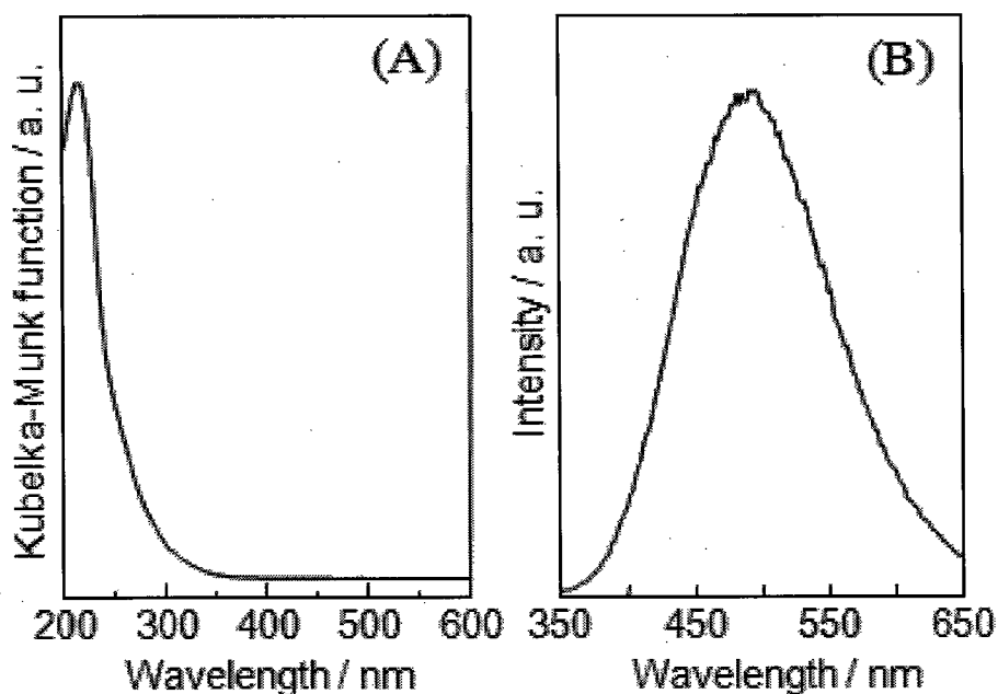
Figure 6-2. UV-vis (A) and photoluminescence spectrum (B) of TS-1( F1 ) measured at 298 K.
