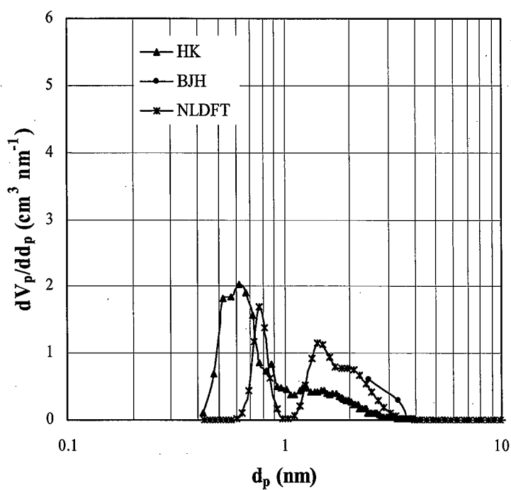
Figure 3-7. PSD calculation from various analysis methods
