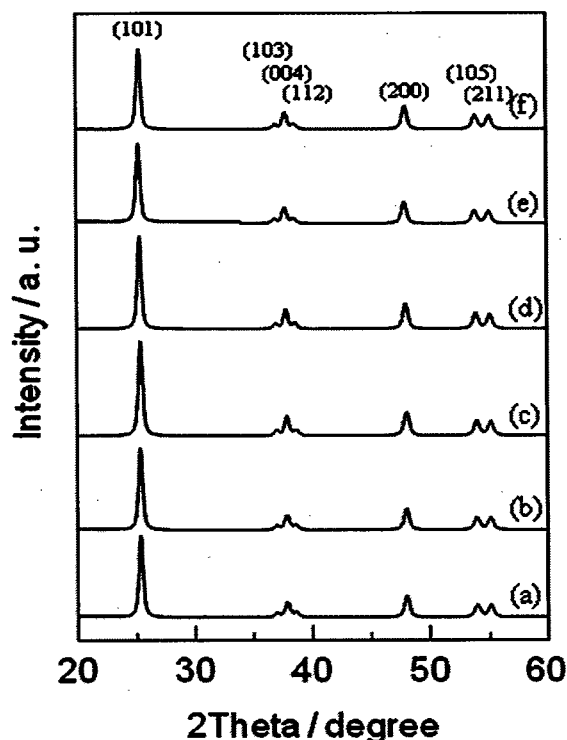
Figure 7-1. XRD patterns of (a) sol-gel \text{TiO}_2 , (b) sol-gel \text{V/TiO}_2(1.0) , (c) \text{HT-TiO}_2 and (d-f) \text{HT-V/TiO}_2(n) ( n = (d) 0.2, (e) 1.0 and (f) 2.0).
