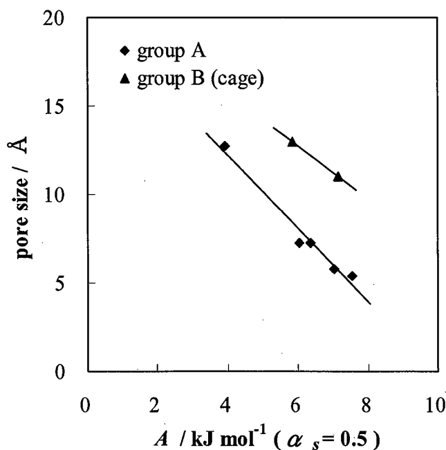
Figure 4-5. Polanyi adsorption potentials vs. pore size or cage size of zeolites.
