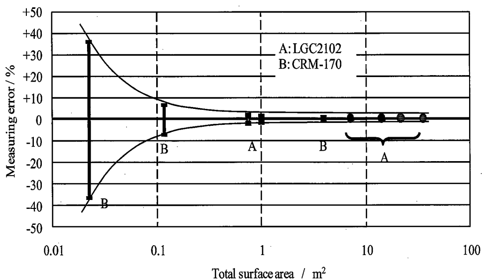
Figure 2-4. Reproducibility against total surface area
