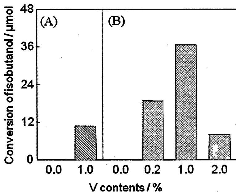
Figure 7-3. Photocatalytic degradation of isobutanol diluted in water over pure \text{TiO}_2 and \text{V/TiO}_2 with different contents of vanadium prepared by (A) sol-gel and (B) hydrothermal treatment in the presence of \text{NH}_4\text{F} under visible light ( \lambda > 430 \text{ nm} ) irradiation. Reaction time: 24 h
