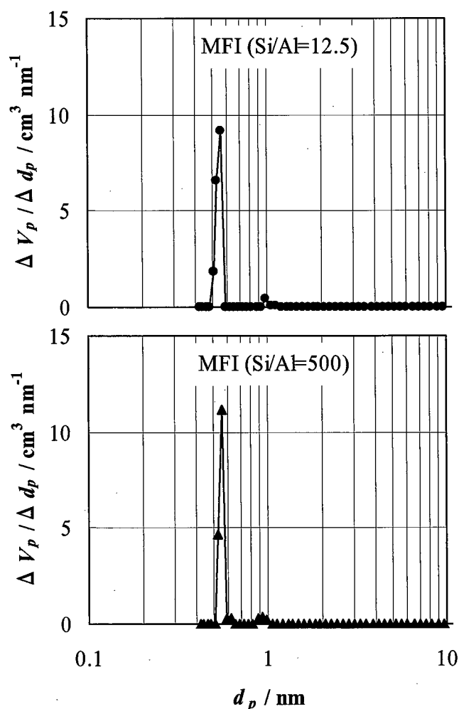
Figure 5-3. Pore size distributions for MFI zeolites (GCMC, BELSim).
