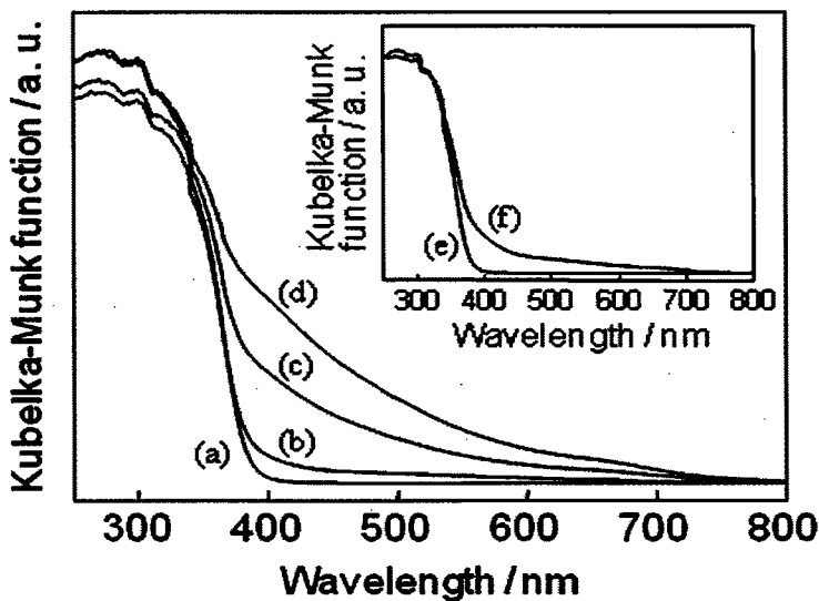
Figure 7-2. UV-vis spectra of pure \text{TiO}_2 and \text{V/TiO}_2 prepared by the sol-gel and hydrothermal treatments
