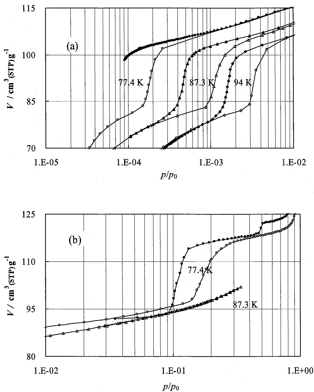
Figure 5-6. High resolution adsorption-desorption isotherms for MFI zeolite (Si/Al=500) ; (a) Ar isotherms (b) \text{N}_2 isotherms.
