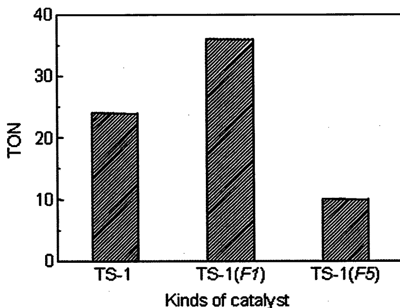
Figure 6-4. The turnover number (TON) for ammoximation of cyclohexanone to cyclohexanone oxime on each catalyst at 353 K. Reaction time: 1h.
