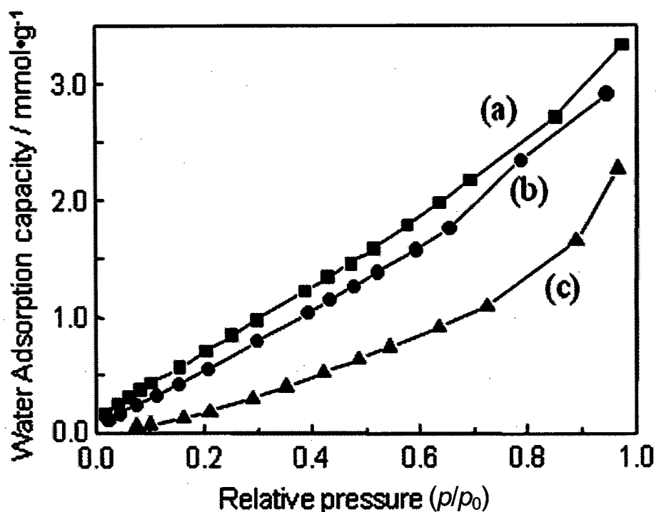
Figure 6-3. Water adsorption isotherms of (a) TS-1, (b) TS-1( F1 ) and (c) TS-1( F5 ) measured at 298 K.
