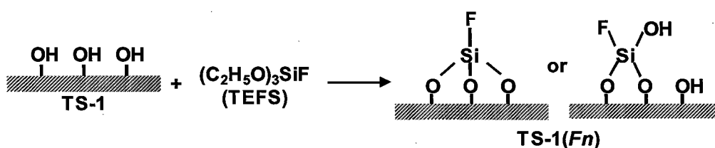
Scheme 6-1. Reaction scheme for surface modification by TEF.
