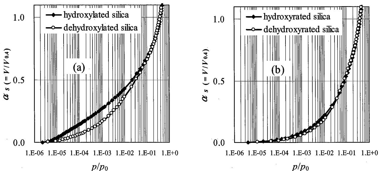
Figure 5-1. High resolution adsorption isotherms for nonporous silicas ; (a) N 2 isotherms at 77.4 K (b) Ar isotherms at 87.3 K.
