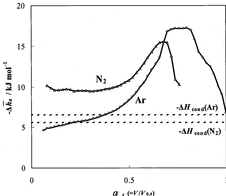
Figure 5-7. Differential adsorption enthalpies for MFI zeolite (Si/Al=500).
