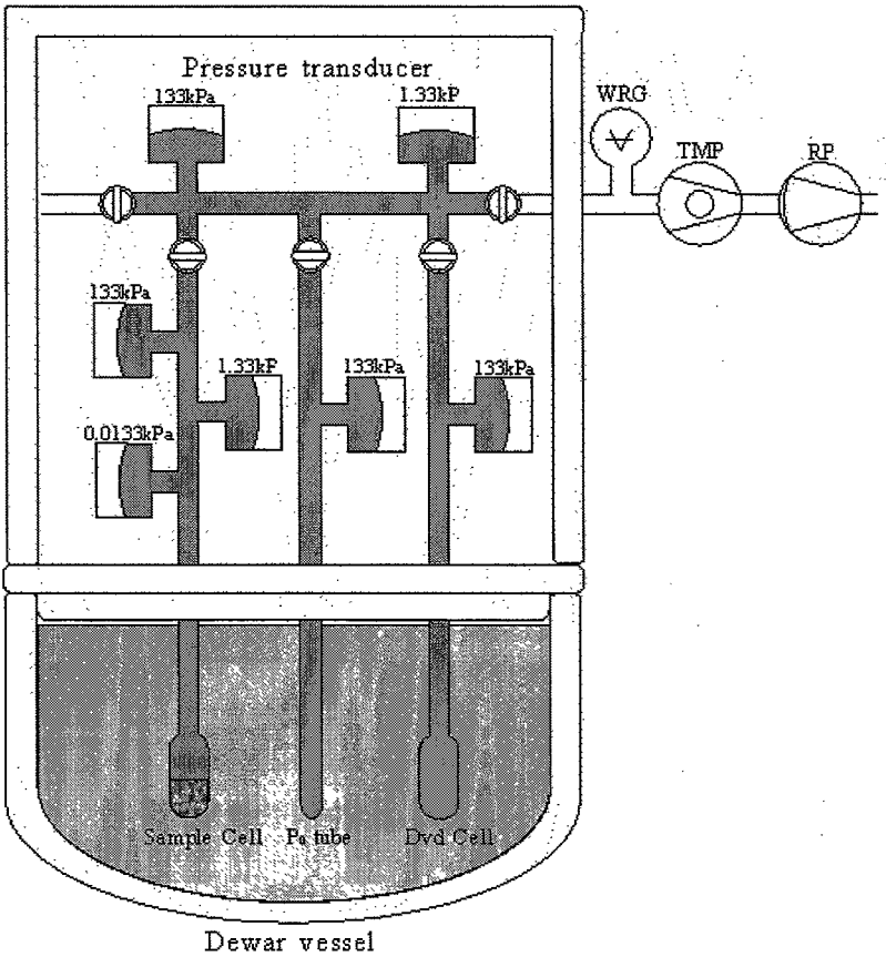
Figure 3-1. Process flow diagram of BELSORP-max™
