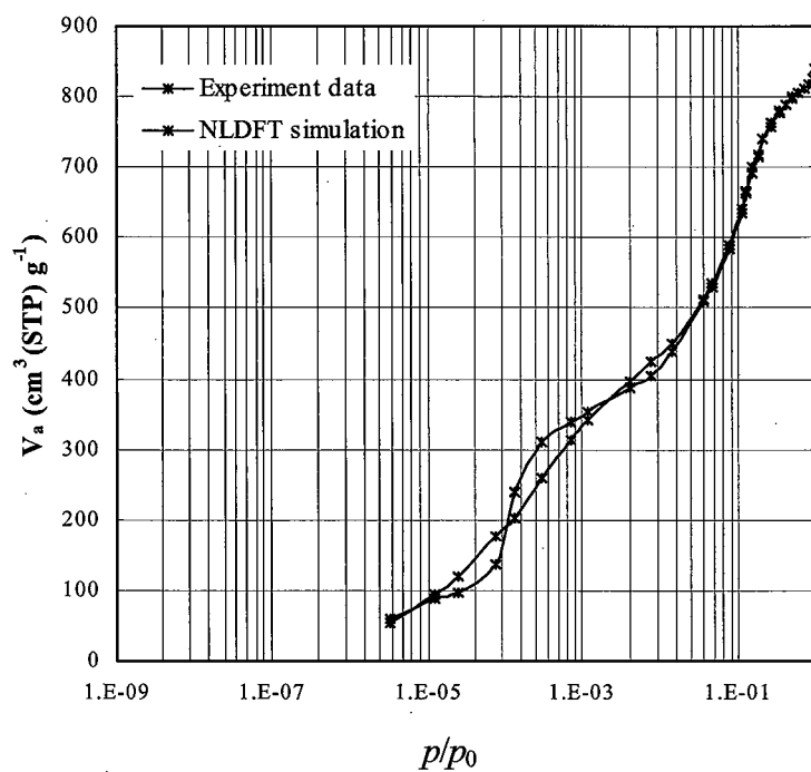
Figure 3-6. Adsorption isotherm of N_2 at 77K from p/p_0=10^{-6} for MPAC
