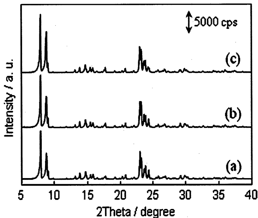
Figure 6-1. XRD patterns of (a) TS-1, (b) TS-1( F1 ) and (c) TS-1( F5 ).
