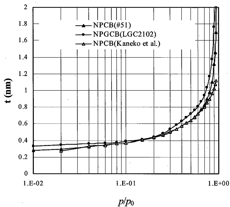
Figure 3-4. Standard t -curve of N_2 at 77K for NPCB and NPGCB
