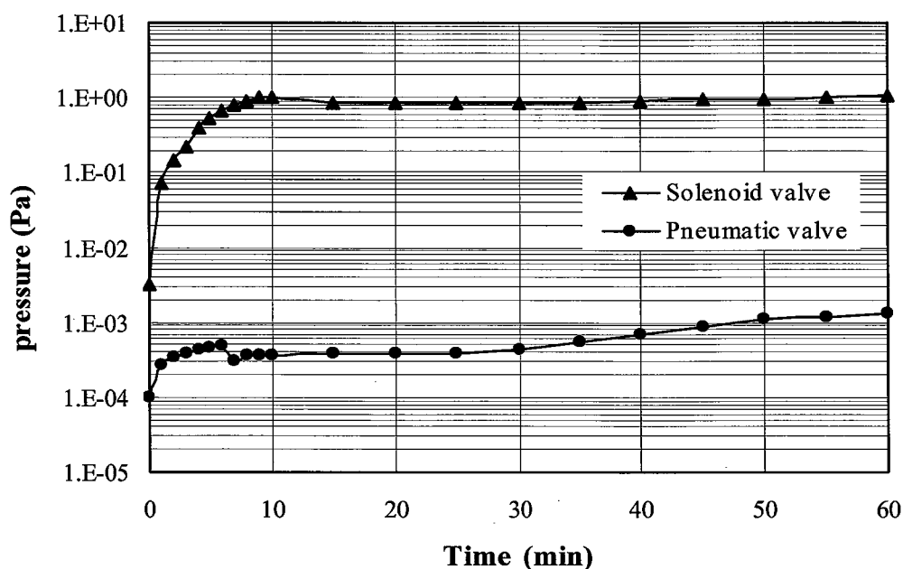
Figure 3-2. Comparison to gas emission amount (pressure increasing) in sample port closed by solenoid valves or pneumatic valves after several hours vacuuming
