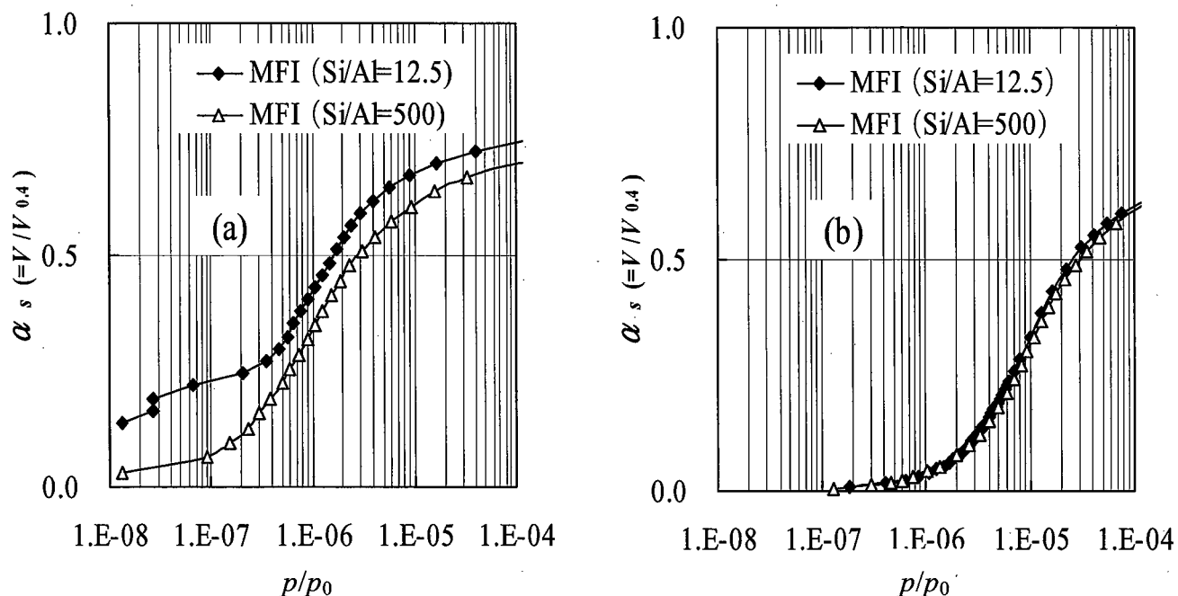
Figure 5-2. High resolution adsorption isotherms for MFI zeolites ; (a) N 2 isotherms at 77.4 K (b) Ar isotherms at 87.3 K.
