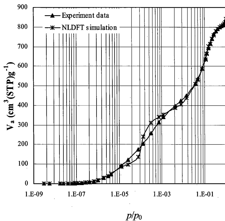
Figure 3-5. Adsorption isotherm of N_2 at 77K from p/p_0=10^{-9} for MPAC
