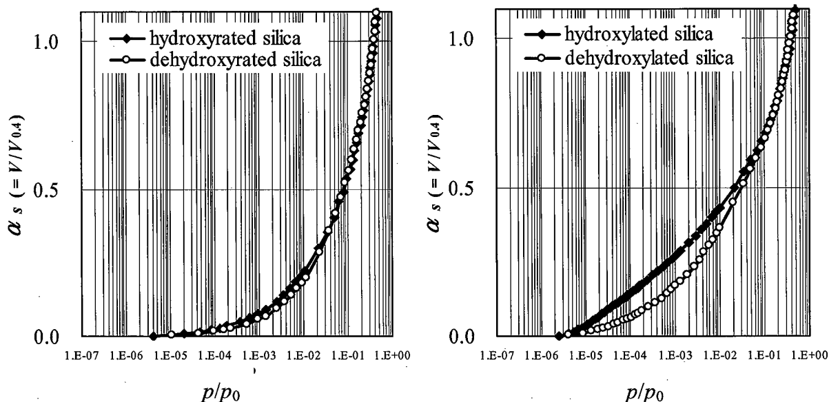
Figure 4-1. High resolution adsorption isotherms for nonporous silicas ; (a) Ar isotherms at 87.3 K (b) N 2 isotherms at 77.4 K.
