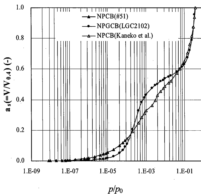
Figure 3-3. Standard \alpha_s -curve of N_2 at 77K for NPCB and NPGCB
