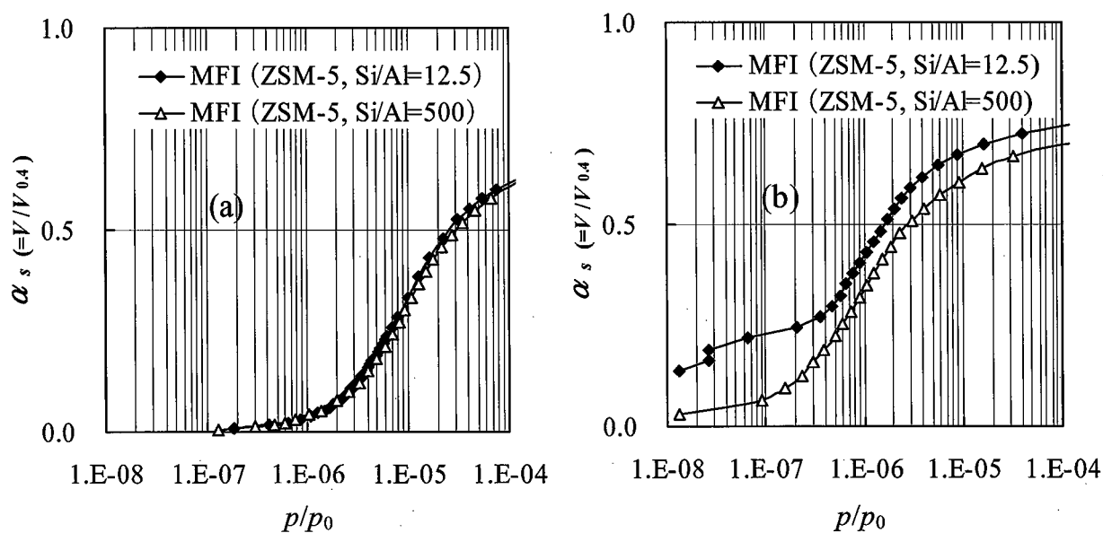
Figure 4-2. High resolution adsorption isotherms for MFI zeolites ; (a) Ar isotherms at 87.3 K (b) N_2 isotherms at 77.4 K.
