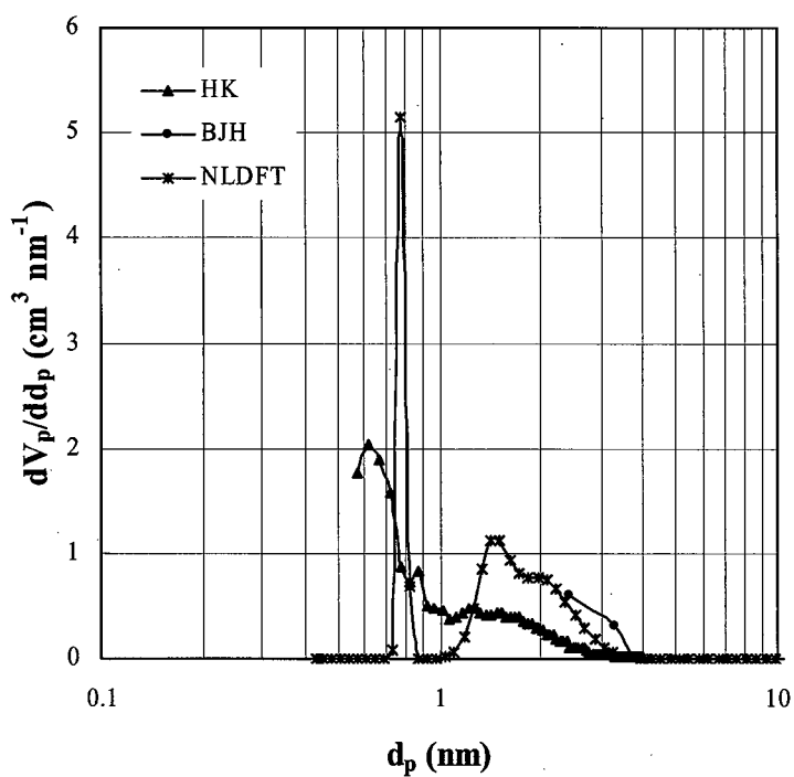
Figure 3-8. PSD calculation from various analysis methods
