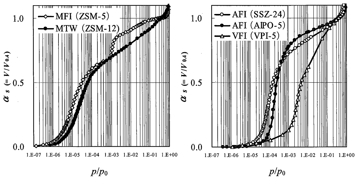
Figure 4-3. High resolution Ar adsorption isotherms at 87.3 K for zeolites of group A.
