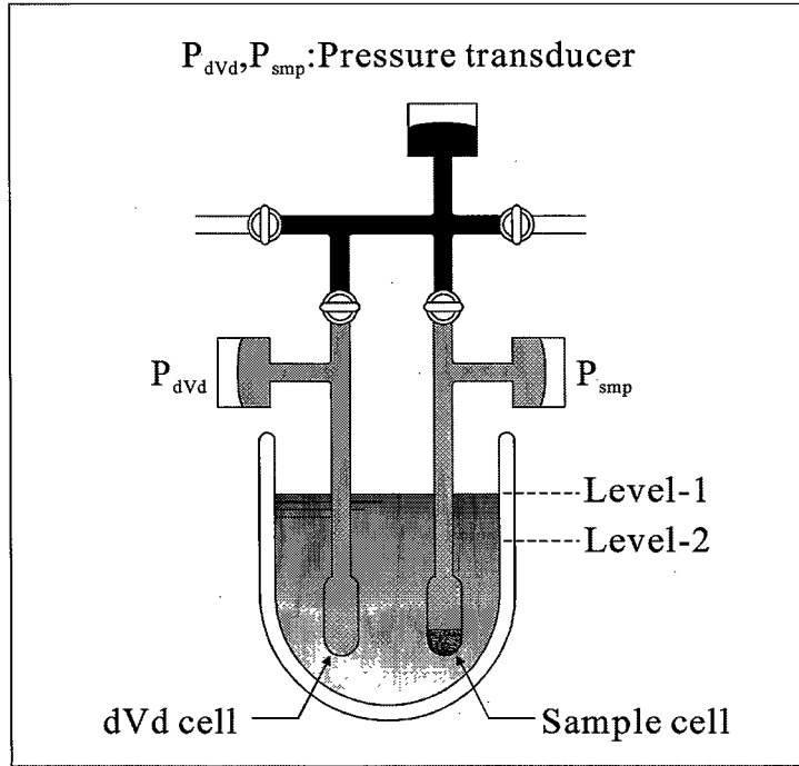
Figure 2-1. Principle of continuous dead volume measurement
