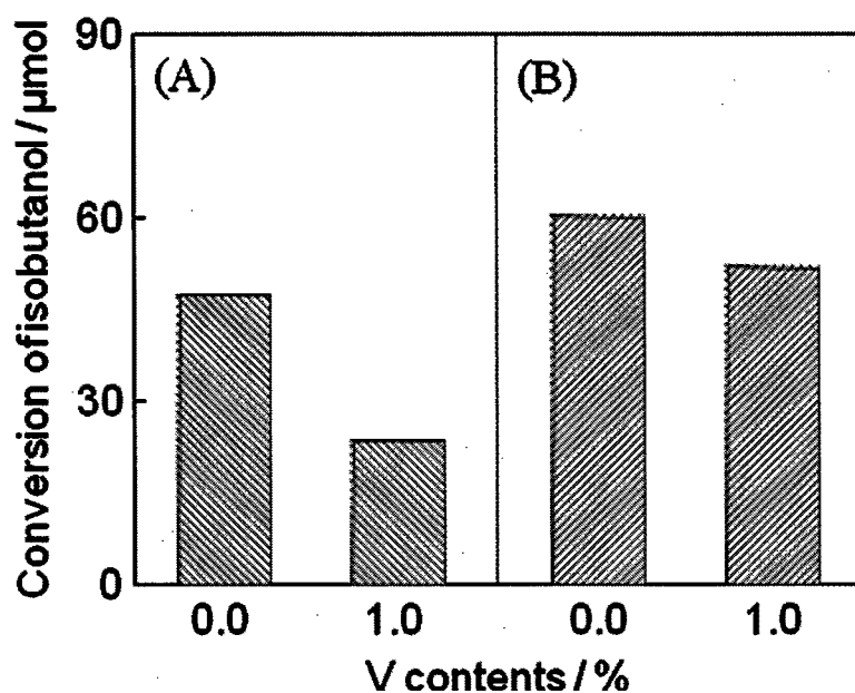
Figure 7-4. Photocatalytic degradation of isobutanol diluted in water over pure \text{TiO}_2 and \text{V/TiO}_2(1.0) prepared by (A) sol-gel and (B) hydrothermal treatment in the presence of \text{NH}_4\text{F} under UV light irradiation. Reaction time: 1 h
