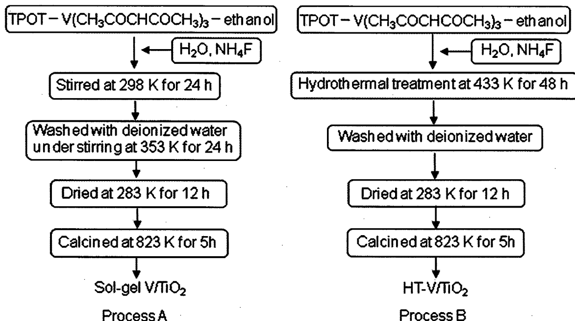
Scheme 1. Synthesis of Sol-gel V/TiO 2 and HT-V/TiO 2
