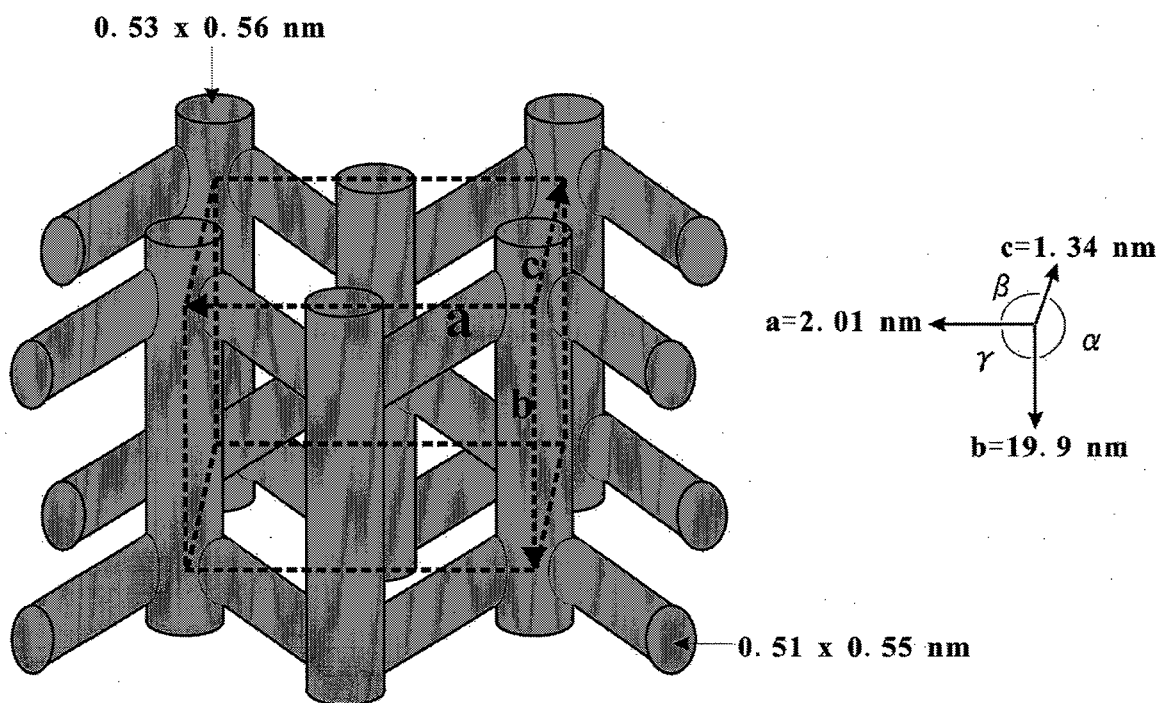
Figure 5-4. Channel structure of MFI zeolites.
