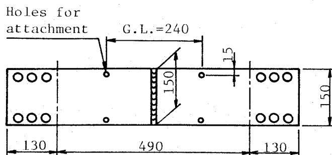
P-type specimen
