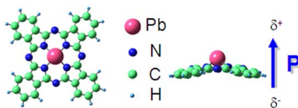
Fig. 2.15: Optimized molecular geometry by DFT calculation (see, ref. [45]) of a PbPc molecule is shown.
