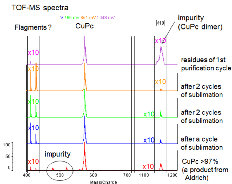
Fig. 2.17: Pure grade of sublimated Copper phthalocyanine (CuPc) is evaluated by MALDI (Laser Desorption Ionization) mass spectra. A product from Aldrich (97% purity) is purified 3 times of sublimation cycles at 673 K. A peak at 574 is derived from pure CuPc. A peak derived from impurity (at 1150, derived from CuPc dimer) is gradually decreased by repeated sublimation cycles. Origins of two peaks around 410 are unknown; maybe they derived from fragments of CuPc (metal-free phthalocyanine).
