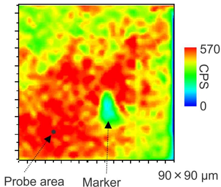
Fig. 3.9: 90×90 \mu\text{m} surface image of PbPc/HOPG (0.3 ML film without annealing) based on the photoemission intensity at the H0 peak in Fig. 3.8 . The right-hand-scale shows the photoelectron counting rate. We selected sample position in large domains. Marker near the center was made with an intense laser irradiation.
