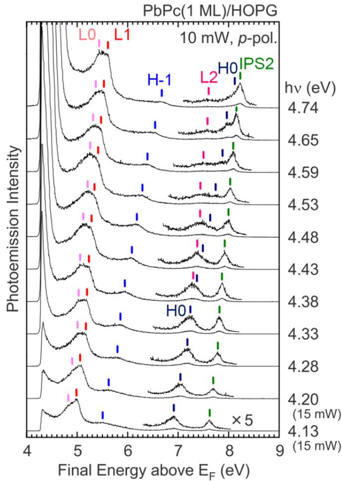
Fig. 3.10: 2PPE spectra for a PbPc film (annealed, 1 ML) on HOPG measured with p-polarized light. The photon energies are shown at the right-hand side. The spectra for h\nu > 4.38 eV were measured with nearly constant laser power of 10 mW. The spectra for photon energies of 4.20 eV and 4.13 eV were measured with the laser power of 15 mW. No normalization was made on the spectra. The spectra at high final energy region were magnified by 5 times. The energies of each peak are marked by bars. At photon energy higher than 4.3 eV, the peak H0 split into two components, L2 and H0.
