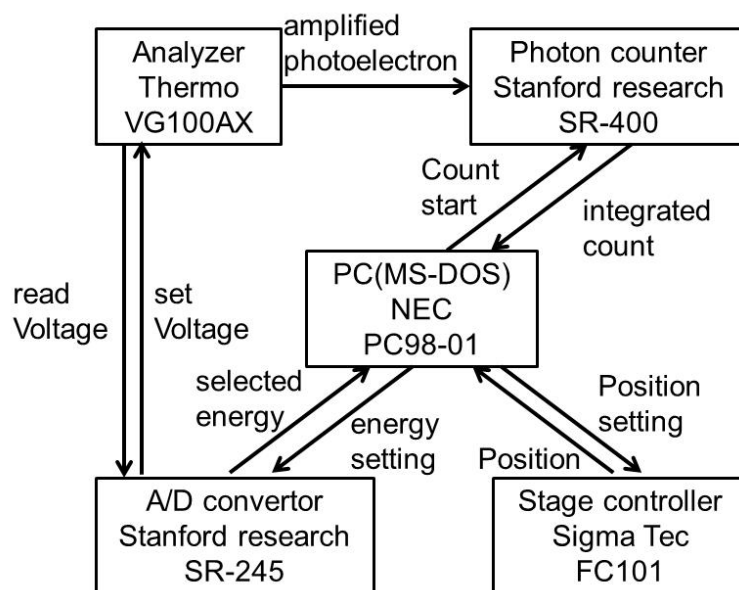
Fig. 2.11: Schematic sketch of the control systems of Micro-2PPE. Photoelectron measurement and sample manipulation are performed by a MS-DOS based PC.
