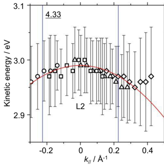
Fig. 6.3: Dispersion of L2 is shown. Peak positions of L2 is plotted against k_{||} . Four symbols (circle, square, triangle, diamond) are used to distinguish results obtained from different measurements. By parabolic fitting, (in the range of -0.3 < k_{||} < 0.3 ) the effective of L2 is m^* / m_e = -10 (solid curve). The fitting curve is shown as red line. The blue solid lines indicated the zone boundaries of IPS2L, which have been shown in chapter 5 .
