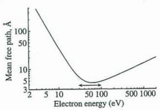
Fig. 2.1: 'Universal curve' showing, schematically how the inelastic mean free path of an electron in a solid varies with its kinetic energy, from ref. [46]. The double arrow indicates the range where surface sensitivity is greatest. To obtain accurate values of the inelastic mean free path, see ref. [46].
