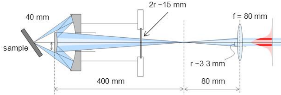
Fig. 2.7: Optical configuration of Schwarzschild objective mirror is shown. The objective mirror is composed of two sapphire mirrors with aluminum coating. These mirrors are bonded to mirror holder (made of beryllium copper) in the UHV chamber. To avoid electronic field by charging effect of dielectric parts, the mirror holder is coated by graphite. The incident laser light is regard as a gauss beam (the intensity curve of a gauss beam is drawn by pink polygon). Intensity of light axis is strong; however, light near axis is reflected by the first mirror. Only red part is reach to the sample. Thus, we must optimize to the size of laser pulse before the magnifying lens to maximize the intensity of photoelectron.
