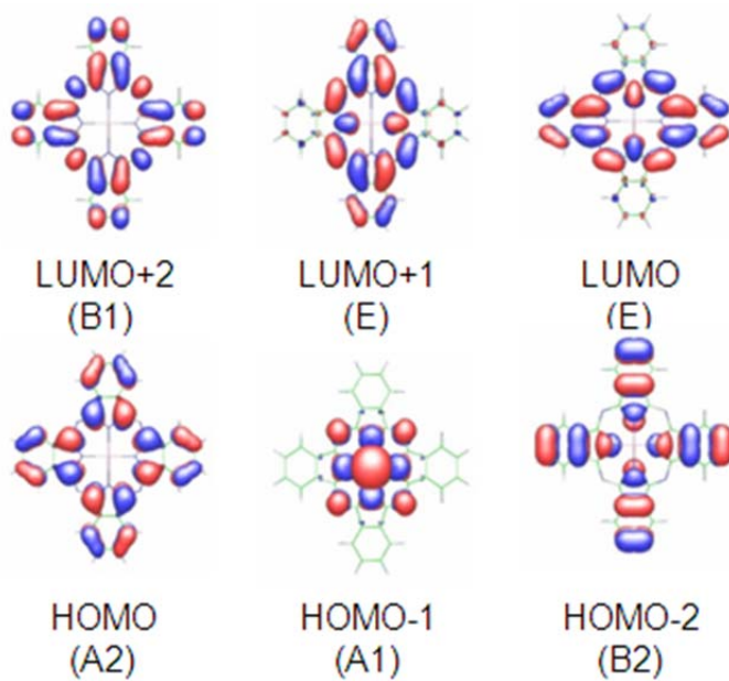
Fig. 3.14: (Top) The energy levels of PbPc (annealed, 1 ML) and the calculated molecular orbital energies from HOMO-1 to LUMO+4 (L+4) of free PbPc. The molecular orbital energies are aligned with the experimental vacuum level. LUMO and LUMO+1 are degenerated in a free PbPc molecule. The block-arrows show the observed resonances from the H0 level to the L2 and to IPS. (bottom) The molecular orbital of PbPc from HOMO-2 to LUMO+2 calculated by DFT with B3LYP method and LANL2DZ basis set. Except for HOMO-1, the molecular orbitals mainly composed with \pi orbital of phthalocyanine ring.
