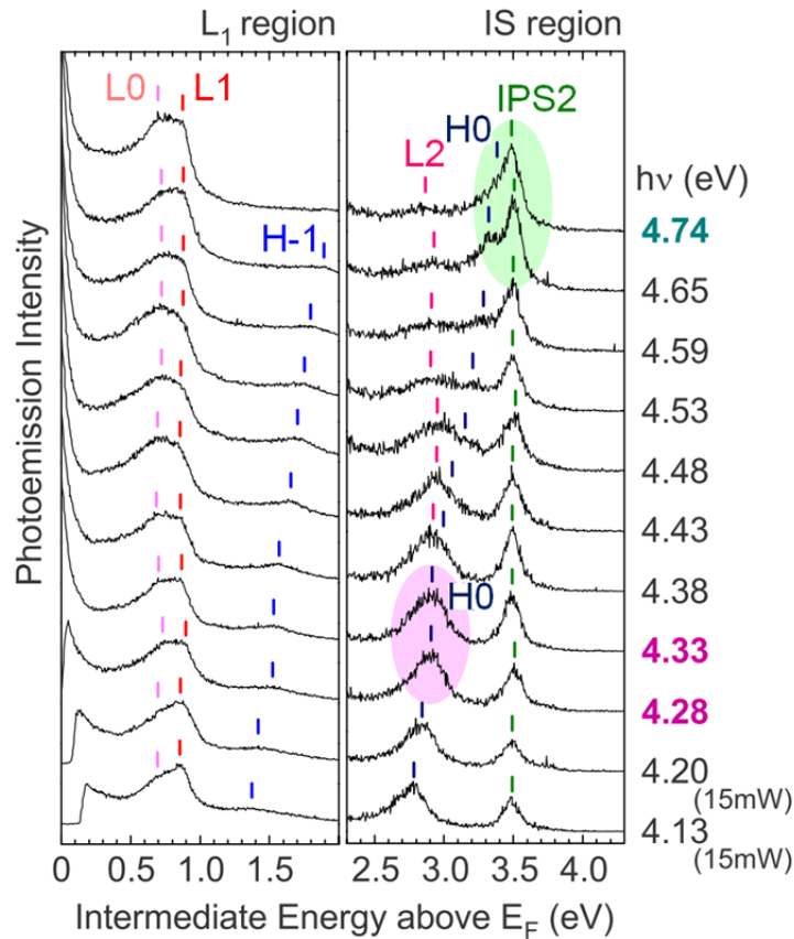
Fig. 3.13: 2PPE results of PbPc (annealed, 1 ML) are plotted on the horizontal axis of the intermediate energy with respect to E_F . The traces of the right panel are expanded by about 10 times to those of the left panel. The peak positions of unoccupied states align on the vertical lines, while those of occupied states moves by one of the photon energy increment. Photoemission is enhanced at photon energy of about 4.3 eV by the resonant between levels for the H0 and L2 features. The H0 peak is enhanced again when it comes closer to the IPS peak, reflecting the resonance between the levels of the H0 and IPS features at the photon energy of about 4.8 eV.
