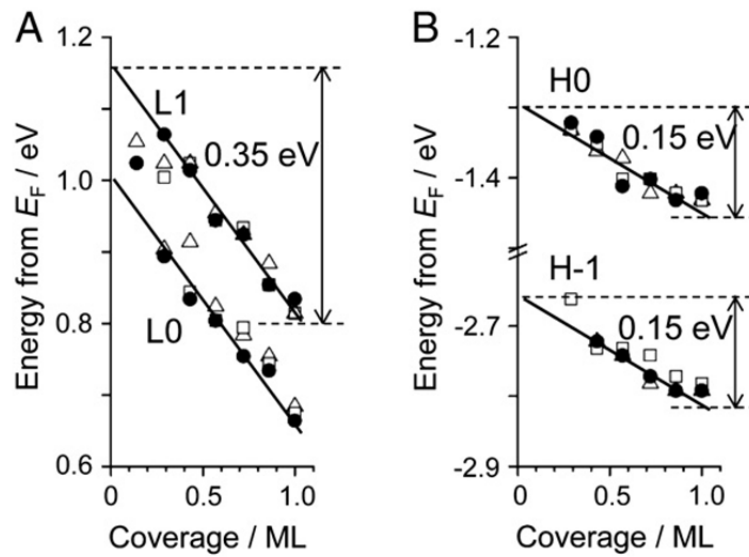
Fig. 4.2: The peak positions in Fig. 4.1 are plotted as a function of coverage. The different marks show data points for different experimental runs. The energy shifts (0.35 eV) of the L0 and L1 peaks shown in (a) are larger than that for the H-1 and H0 peaks shown in (b). The shifts for the HOMO and HOMO-1 levels are both 0.15 eV/ML which is comparable to the VL shift of 0.18 eV / ML. The shifts for L0 and L1, larger by 0.2 eV than the occupied level shifts, are due to the intermolecular interaction.
