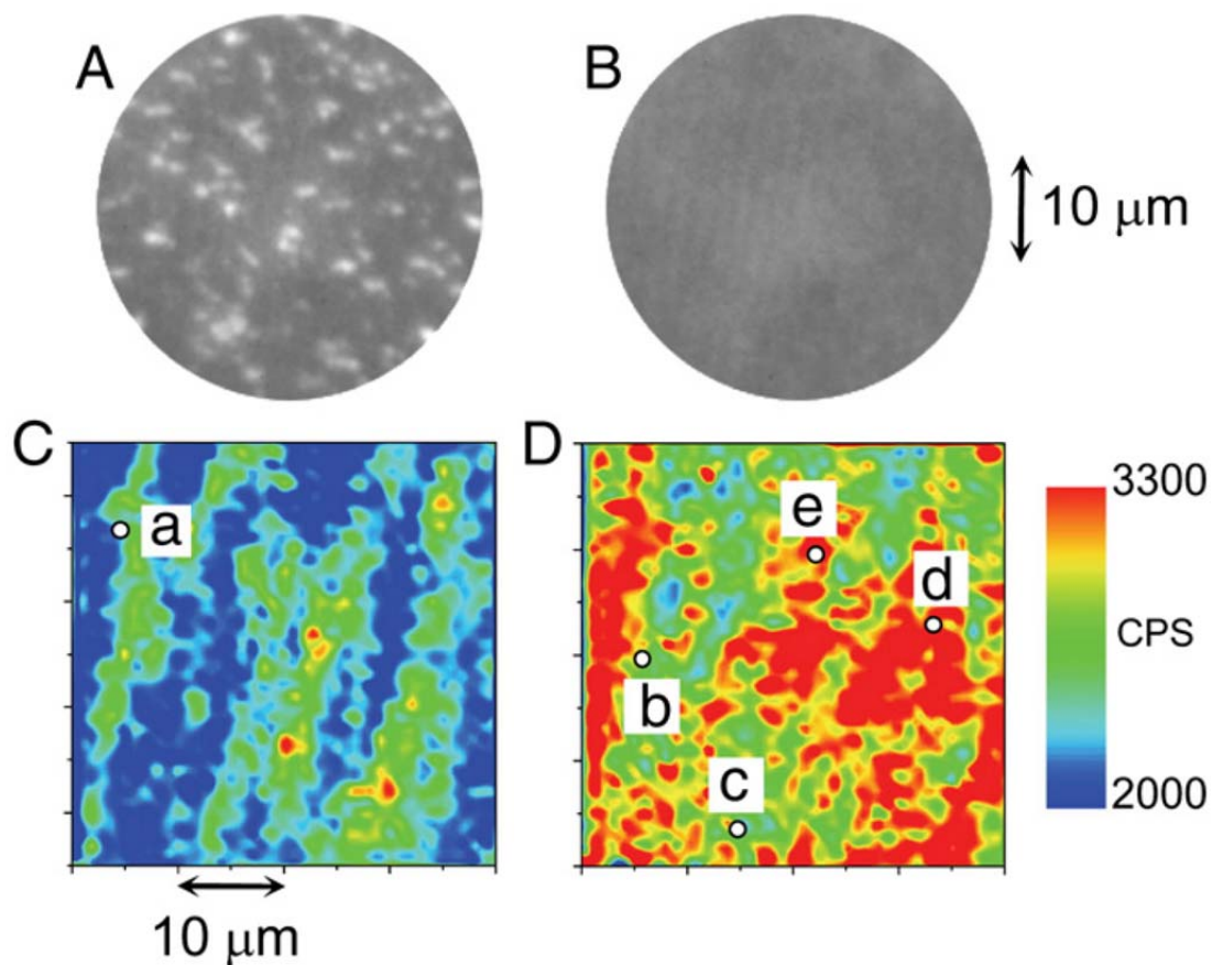
Fig. 4.3: Surface images of the 0.3 ML films. Top images are one-photon PEEM images of as-deposited film (a) and annealed film (b) measured with p-polarized light at photon energies of 5.70 eV. The brightness of the image is proportional to the molecular density. The bright patches in (a) due to the metastable bilayer are quenched by annealing, as shown in (b). The molecular density in (b) seems to be uniform. Bottom images are micro-2PPE images measured at the energy of the L1 peak. The photon energy is 4.33 eV. The lateral inhomogeneity of the as-deposited film (c) is enhanced for the annealed film (d). Comparison of (b) and (d) indicates that the intensity of the L1 peak is governed by a factor other than the number of molecules within the probe spot of 0.4 \mu\text{m} . Micro-2PPE spectra at points A to E are shown in Fig. 4.4 .
