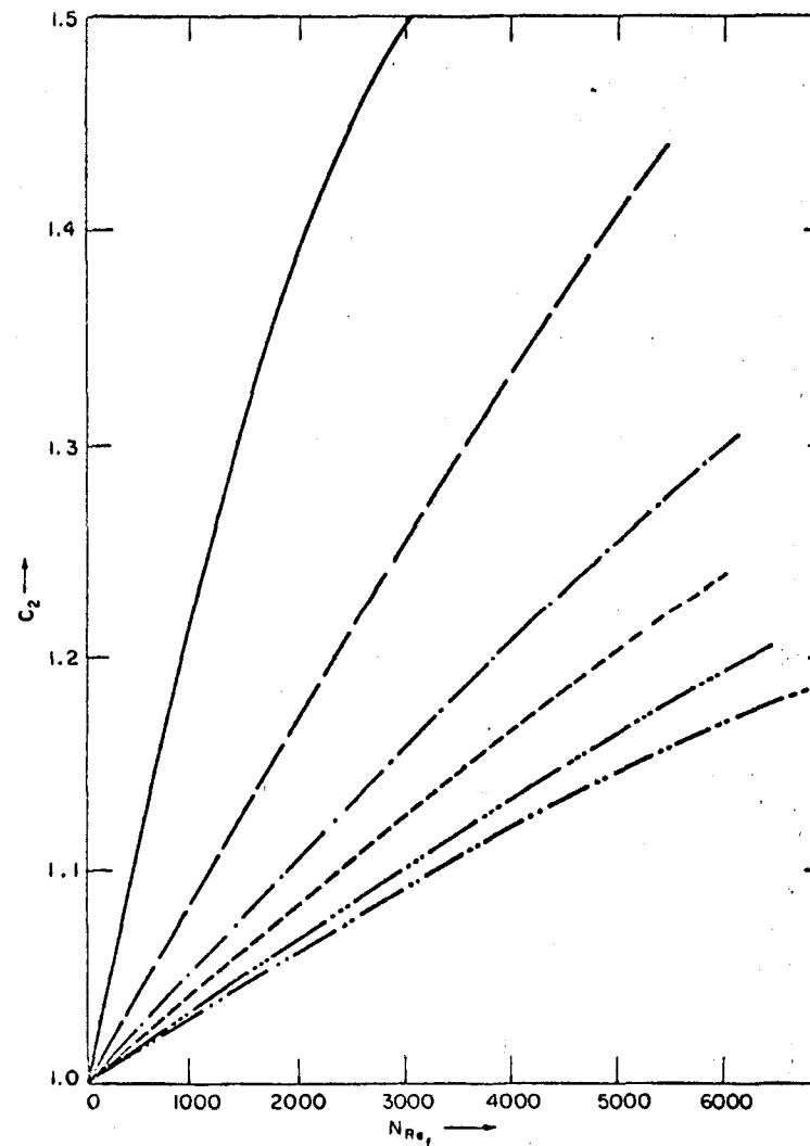
Fig. 3.2. Coefficient C_2 against liquid Reynolds number for various values of bubble Reynolds number
