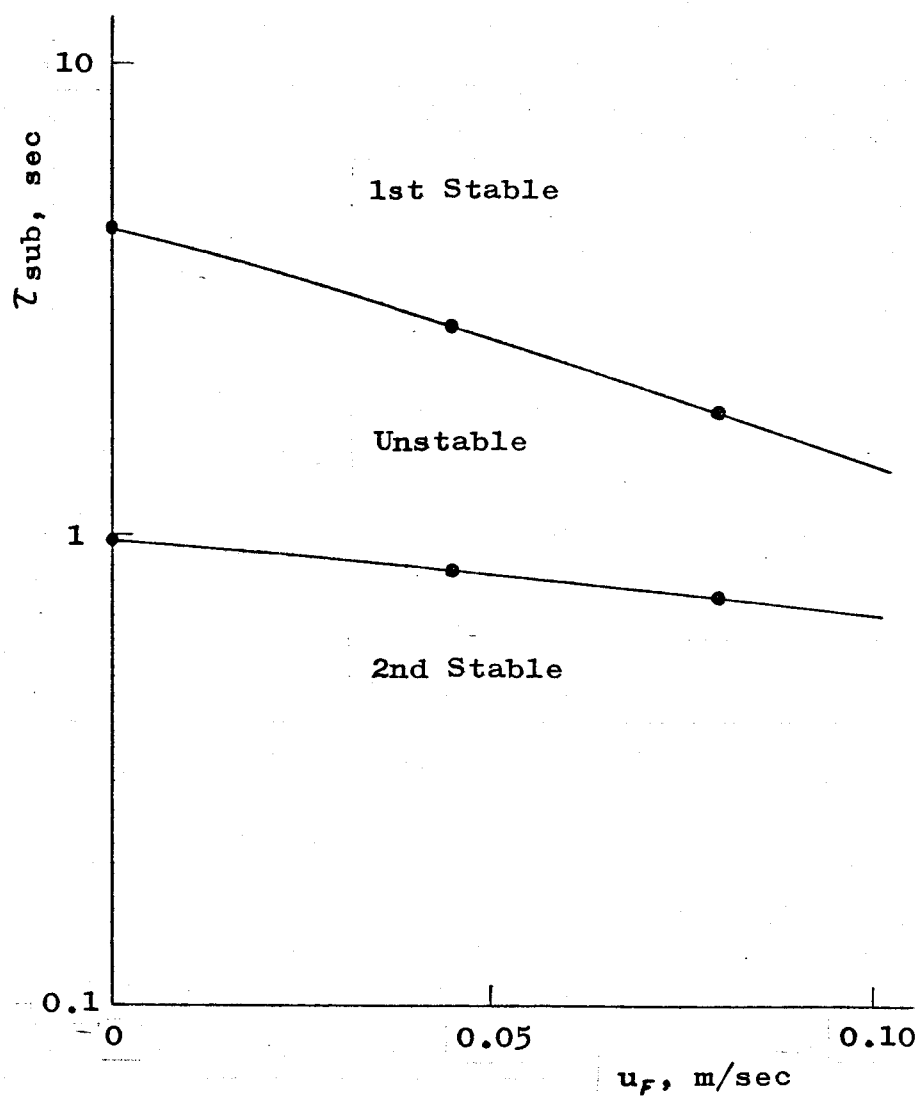
Fig.1.8. Stability division in (u_f, \tau_{sub}) plane.
