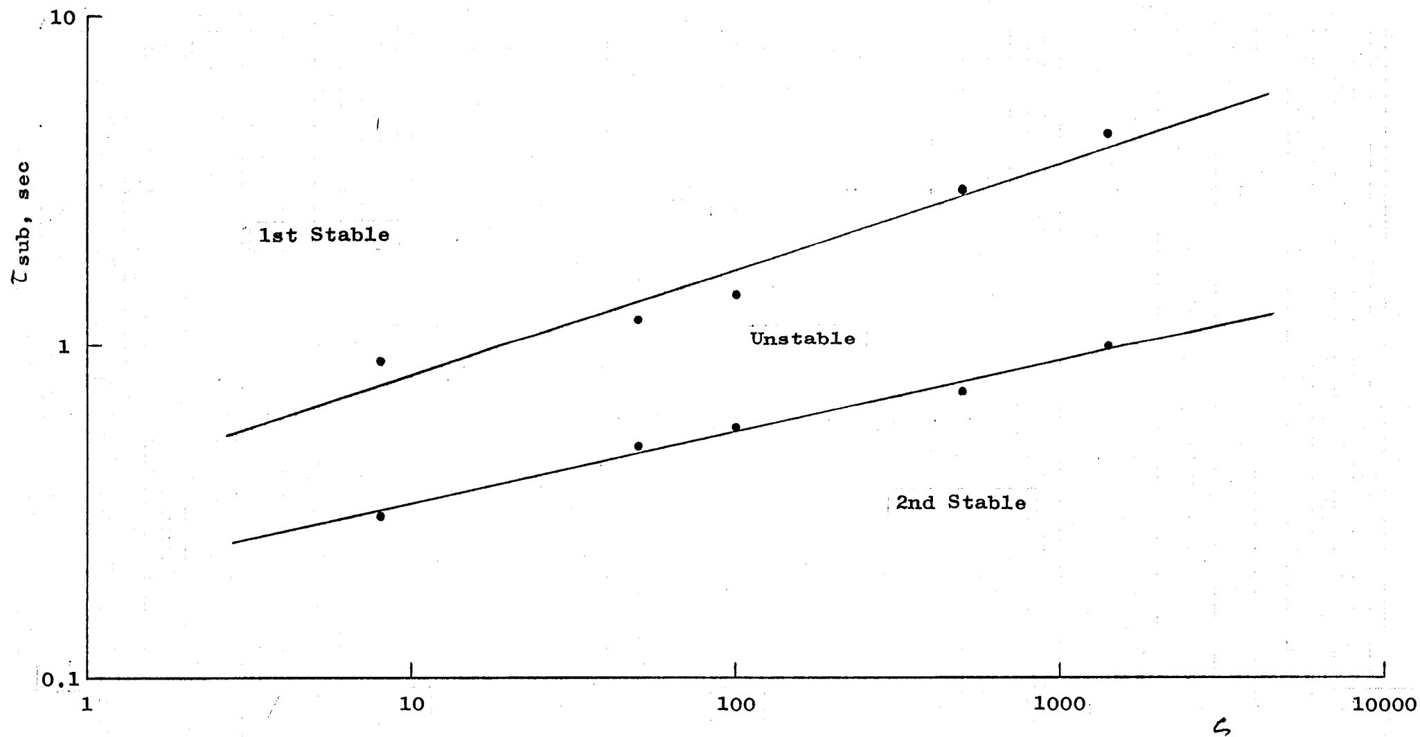
Fig.1.7. Stability division in (\zeta, \tau_{\text{sub}}) plane. (Natural circulation)
