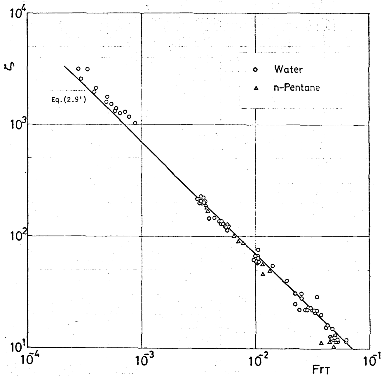
Fig.2.3. Relation of N with Frr (Natural Circulation)
