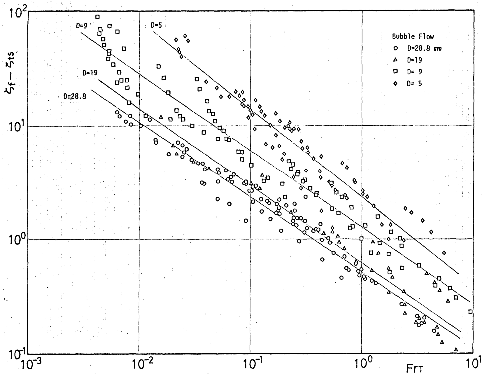
Fig.2.7. Data of Inoue and Aoki adjusted in (Fr\tau, \zeta_f - \zeta_{ts}) plane
