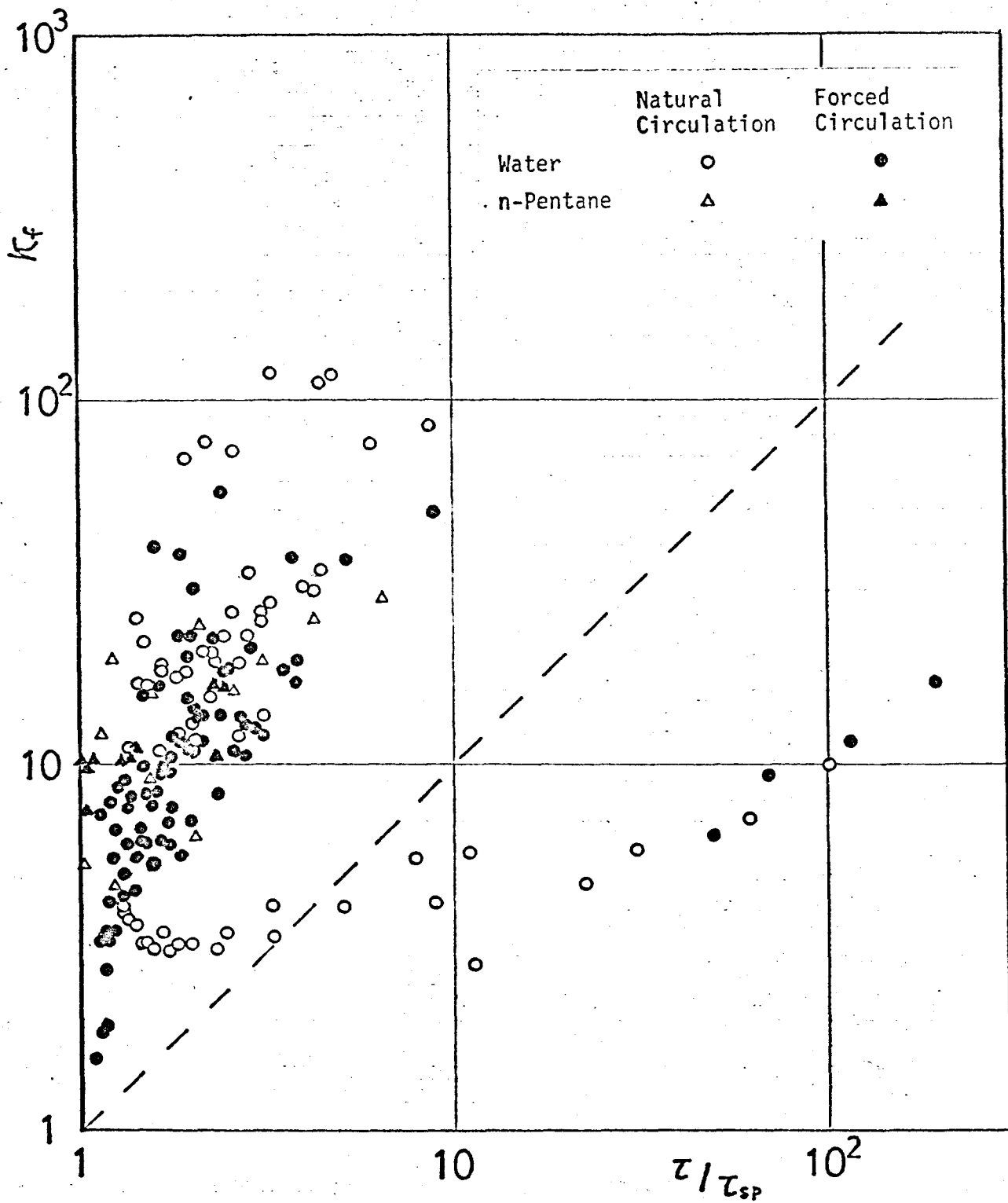
Fig.2.10. Comparison of present data with equation (2.22) of Bankoff
