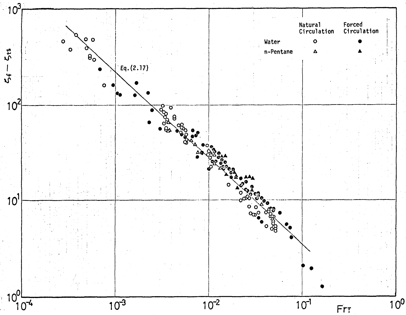
Fig.2.5. Relation of (\zeta_f - \zeta_{ts}) with Fr\tau
