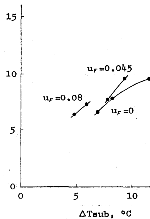
(c) Effect of forced flow velocity u_F [m/sec] at \zeta=1400 & q=1300 kcal/m² sec.
