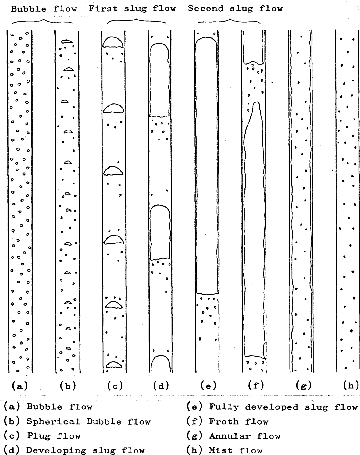
Fig.1.4 Flow patterns of vertical two-phase flows
