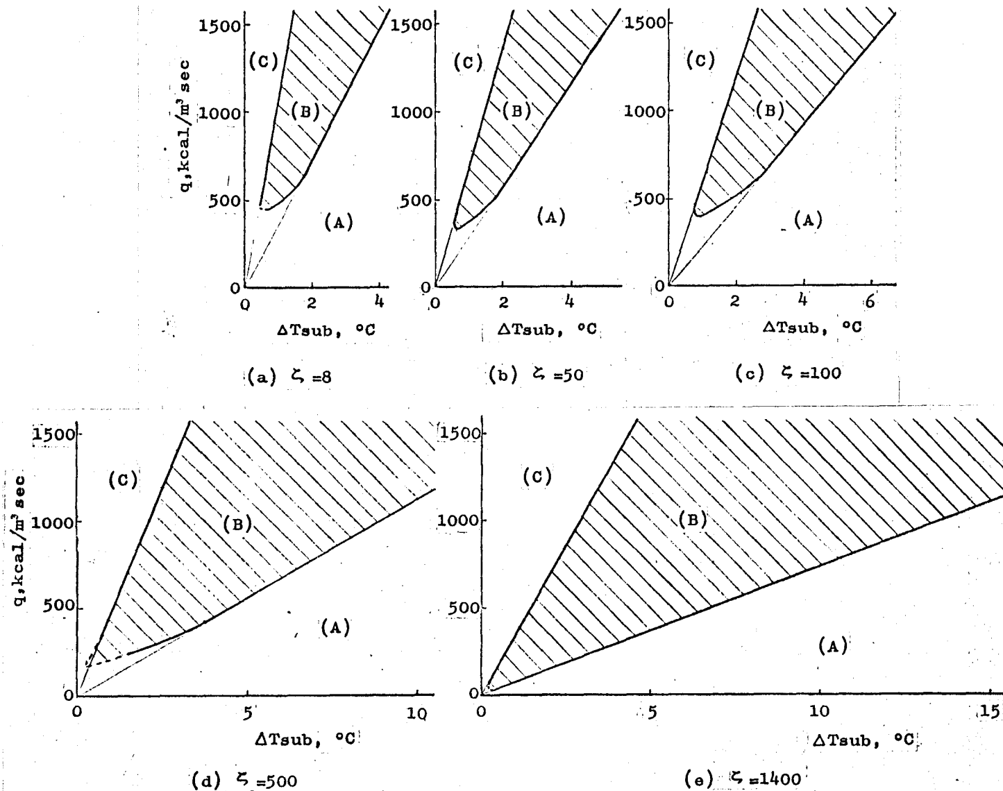
Fig.1.5. Stability division in (\Delta T_{sub}, q) plane. (Natural circulation) (A) is the 1st stable region, (B) is the unstable region, and (C) is the 2nd stable region.
