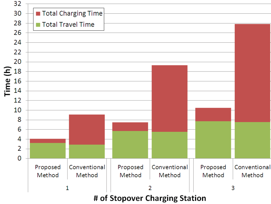
Figure 3.5: Travel and charging time according to # of stopover charging stations (in 2011)
