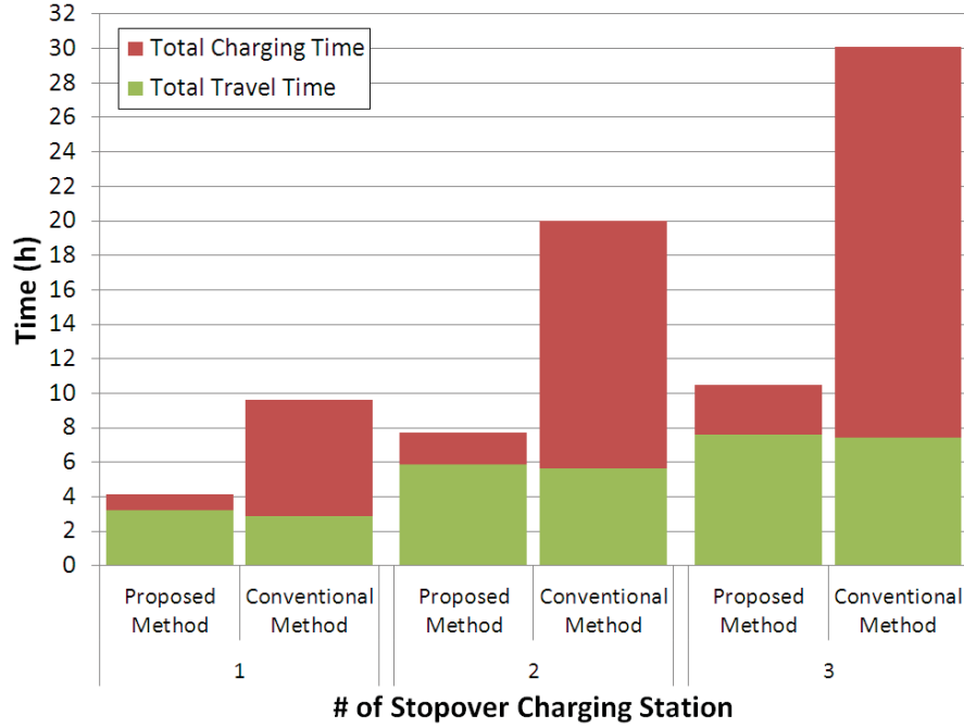
Figure 3.4: Travel and charging time according to # of stopover charging stations (in 2010)
