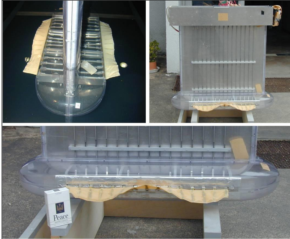
Fig. 1.2 Model-1 of the Squid-robot
