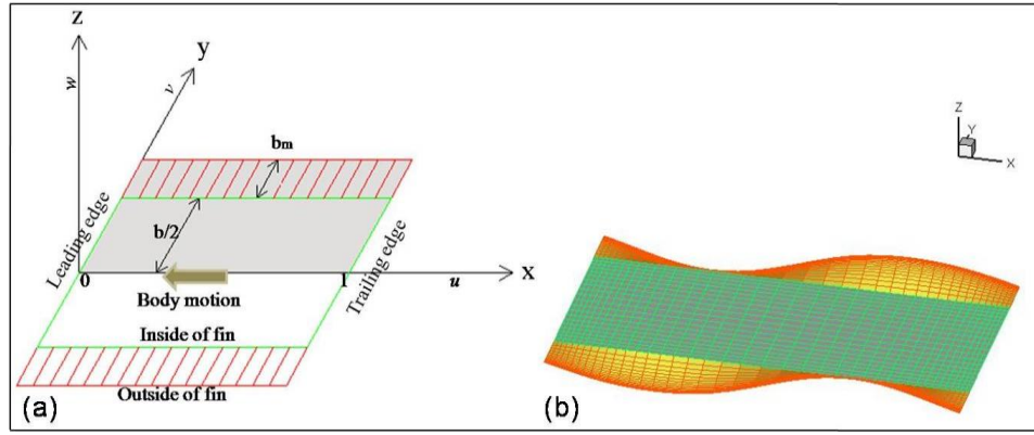
Fig. 2.3 (a) Simple model sketch and coordinate system; (b) Computational Model with undulating side fin
