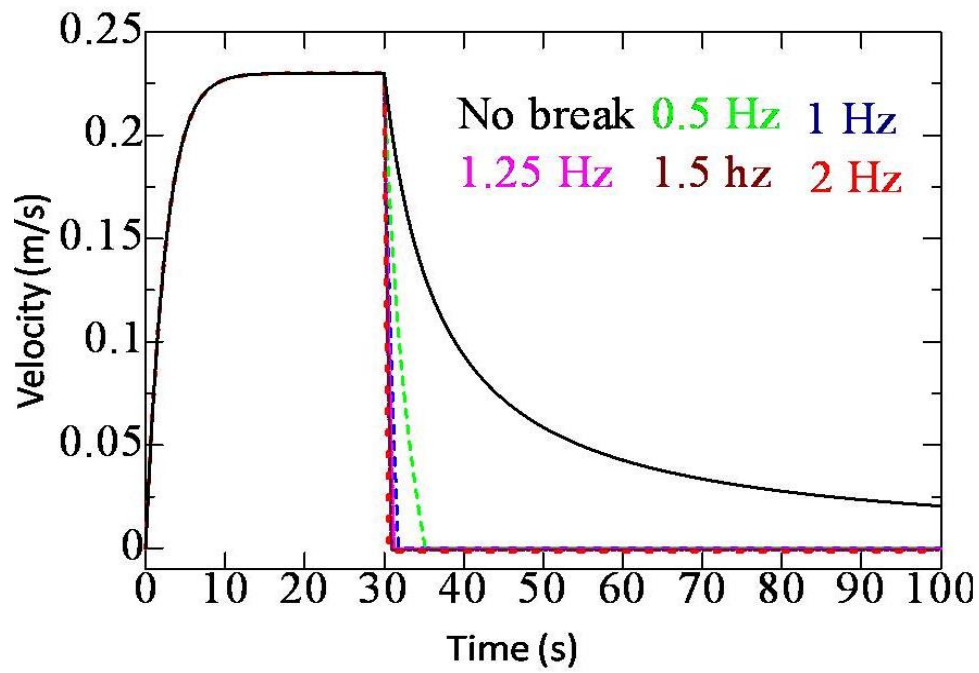
Fig. 3.9 Velocity with respect to time in translational motion
