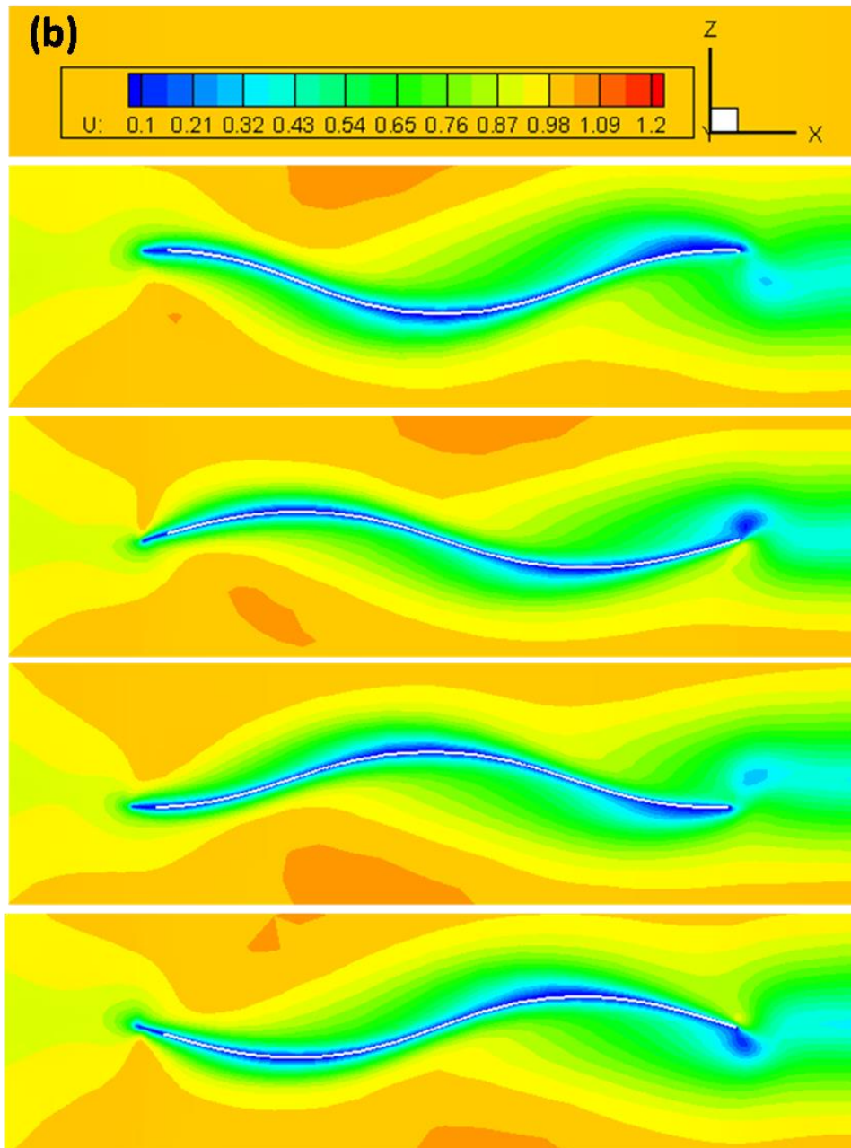
Fig. 2.28 (b) Contours of x-directional velocity distribution at \theta = 45 , n = 3.18
