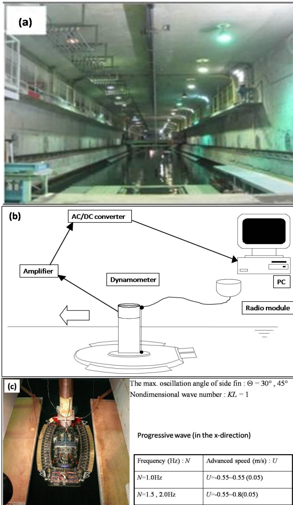
Fig. 2.1 (a) Towing Tank of Osaka University; (b) Sketch of the experimental set up (c) Picture of the experiment with experimental condition
