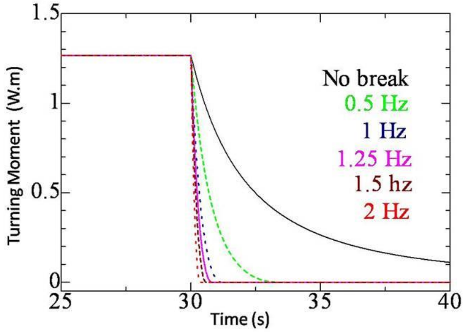
Fig. 3.15 The moment of inertia with respect to time (enlarged view)
