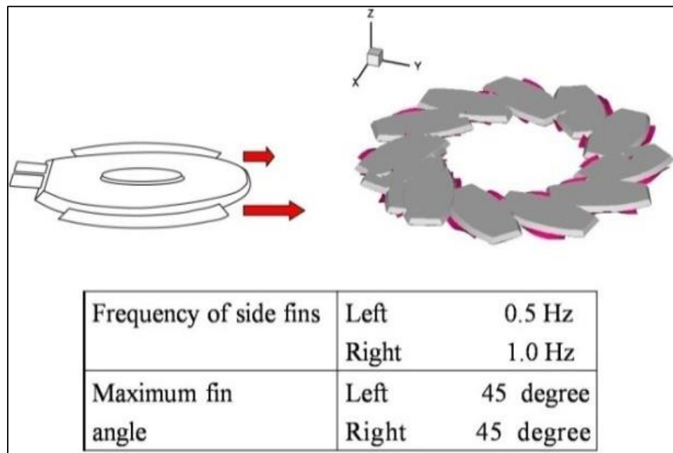
Fig. 4.1 Sketch of the principal of circular motion
