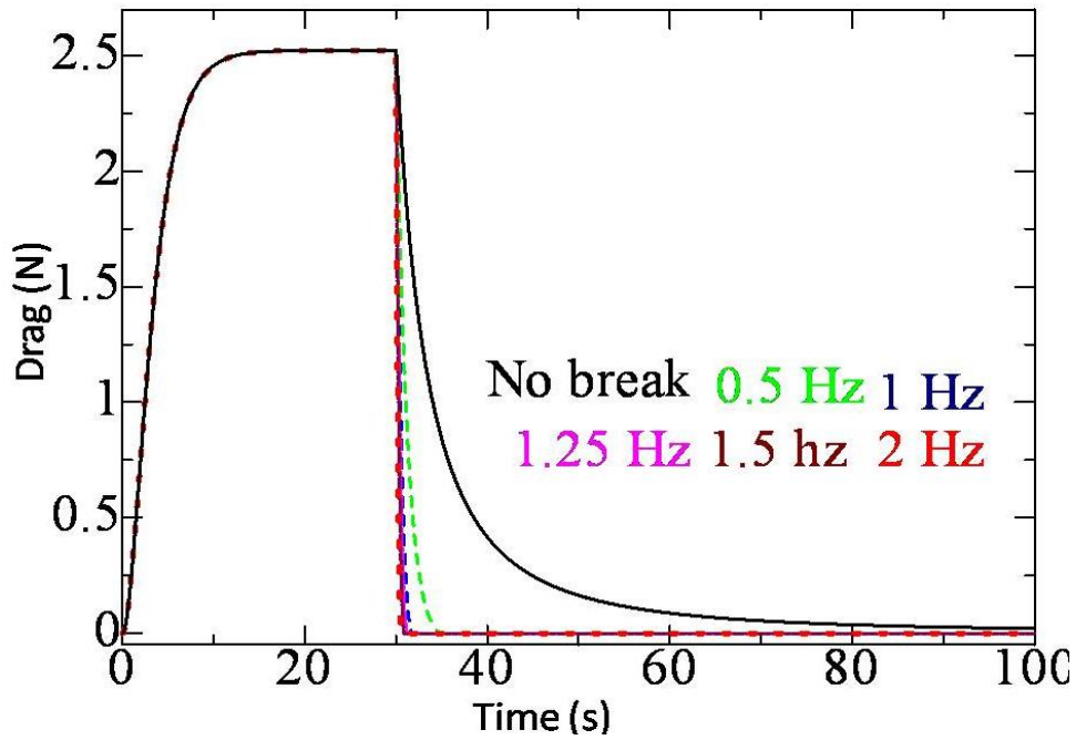
Fig.3.11 Drag at different braking frequency in translational motion
