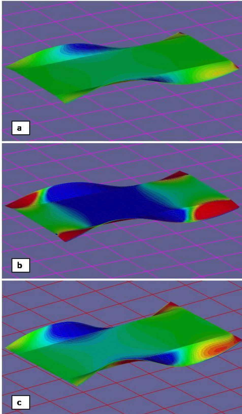
Fig. 2.14: Pressure distribution on the upper and lower surface of the body and fins with AR = 0.1 (a) n = 3 , \theta = 30^\circ ; (b) n = 6 , \theta = 30^\circ and (c) n = 3 , \theta = 45^\circ
