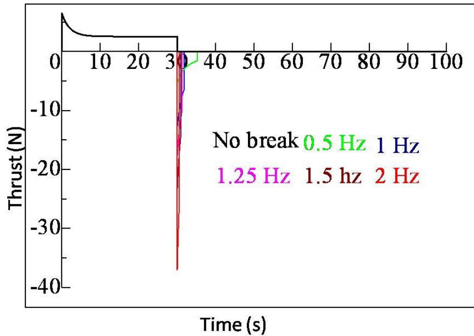
Fig.3.10 Thrust at different braking frequency in translational motion
