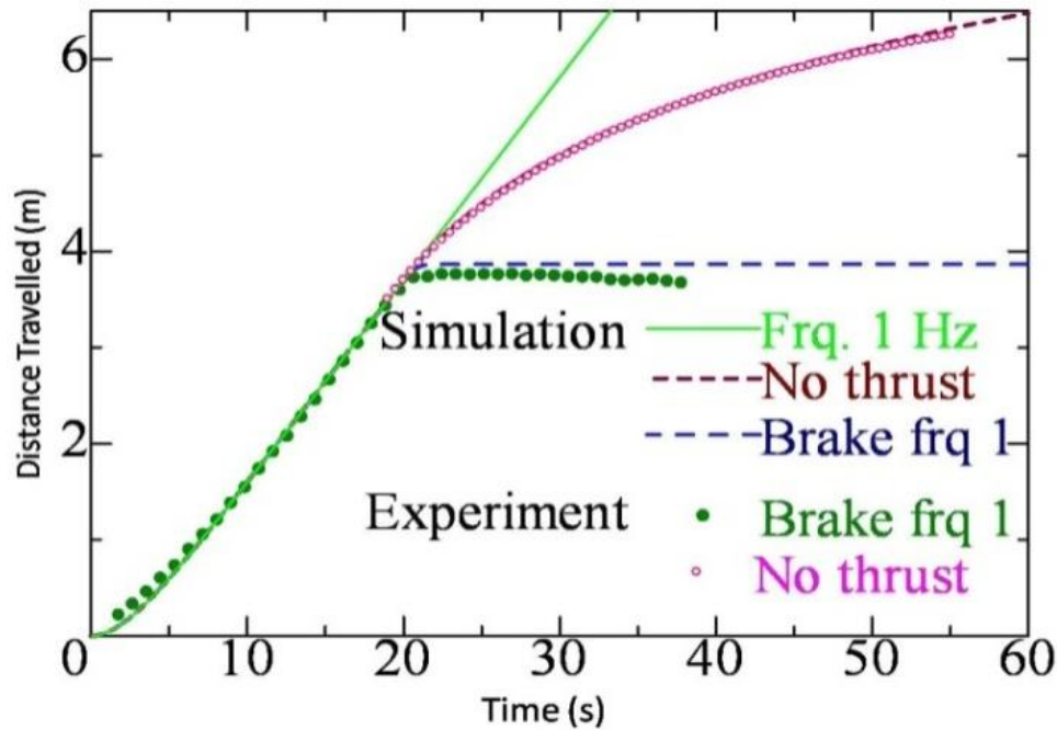
Fig. 3.6 Comparison of experimental and simulation results in case of translational motion with and without brake
