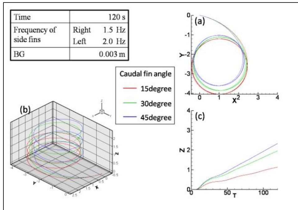
Fig. 4.9 Spiral motion where caudal fins were used to change of depth
