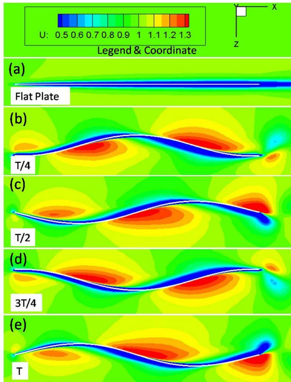
Fig. 2.12 u -velocity distribution on a flat plate and around a fin ( AR = 0.1 , \theta = 30^\circ ) for n = 4 at four time steps in one period
