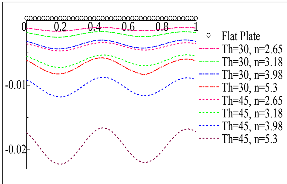
Fig. 2.27 Total x-directional force for different frequencies and fin angles produced by fin only (one period)
