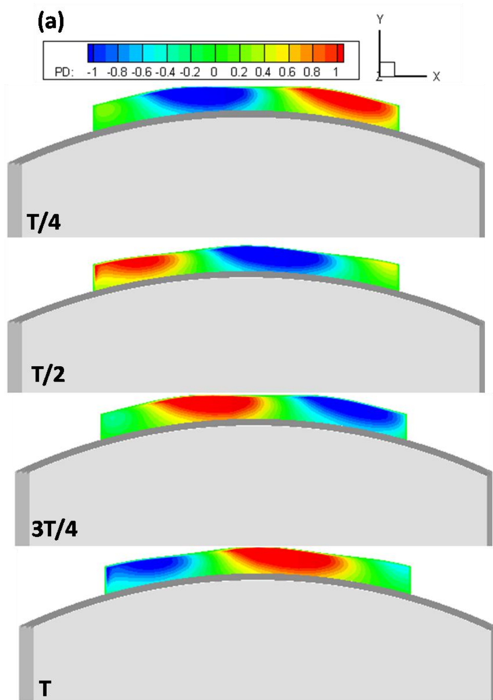
Fig 2.31 (a) The distribution of pressure difference on the fin at \theta = 30 , n = 3.18
