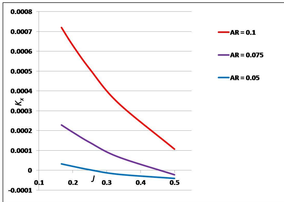
Fig. 2.18 Fin open characteristics, \theta = 30^\circ
