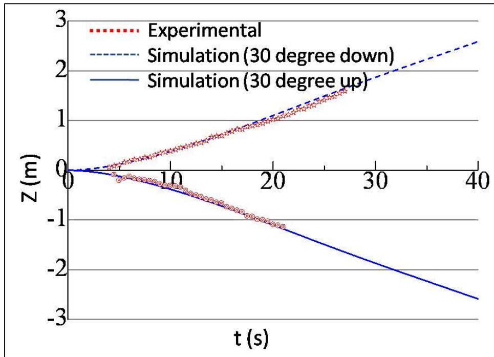
Fig. 4.7 Time history of the models in z-direction for vertical motion at +30 degree and -30 degree change of center of oscillation
