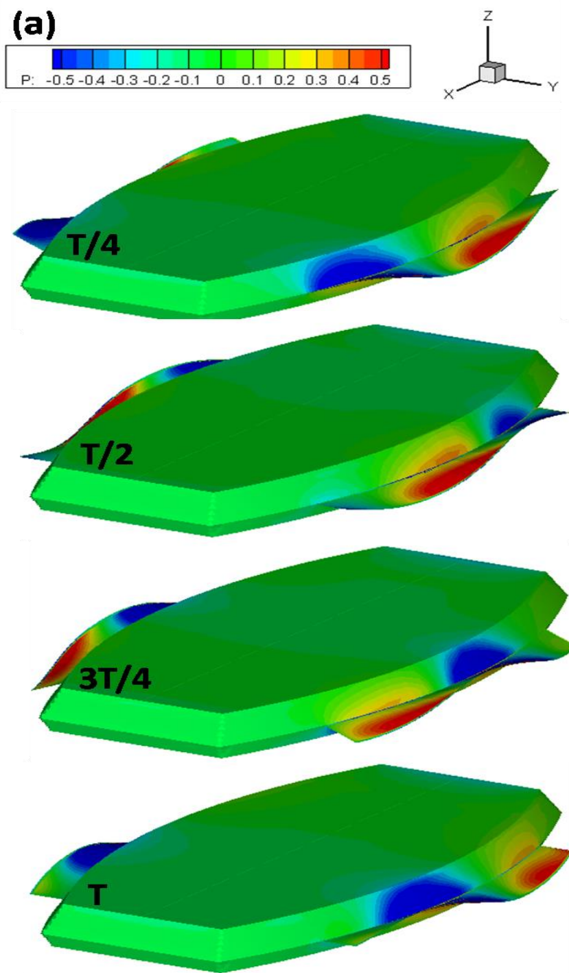
Fig. 2.30 (a) Pressure distribution on the Model-4 of Squid-robot at \theta = 30 , n = 3.18
