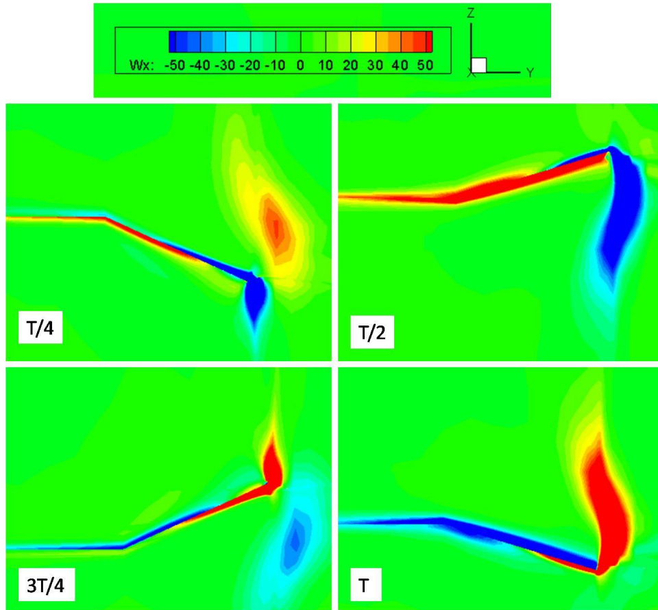
Fig. 2.13: \omega_x -vorticity distribution at the rear end of a fin of AR = 0.1 , n = 4 and \theta = 30^\circ at four time steps in one period
