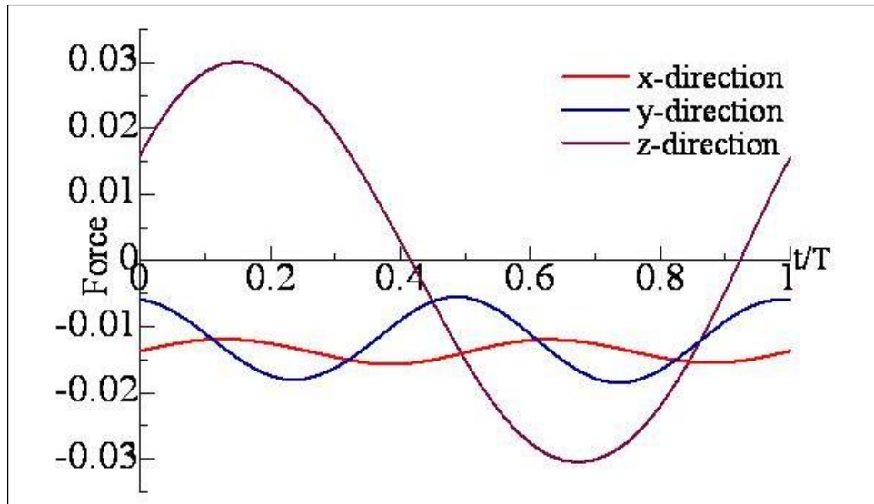
Fig. 2.9 x, y and z direction pressure forces produced by undulating side fin
