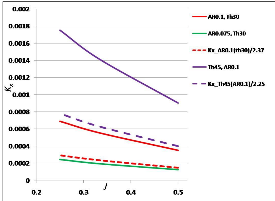
Fig. 2.21 The relation between k_x & AR and k_x & \Theta
