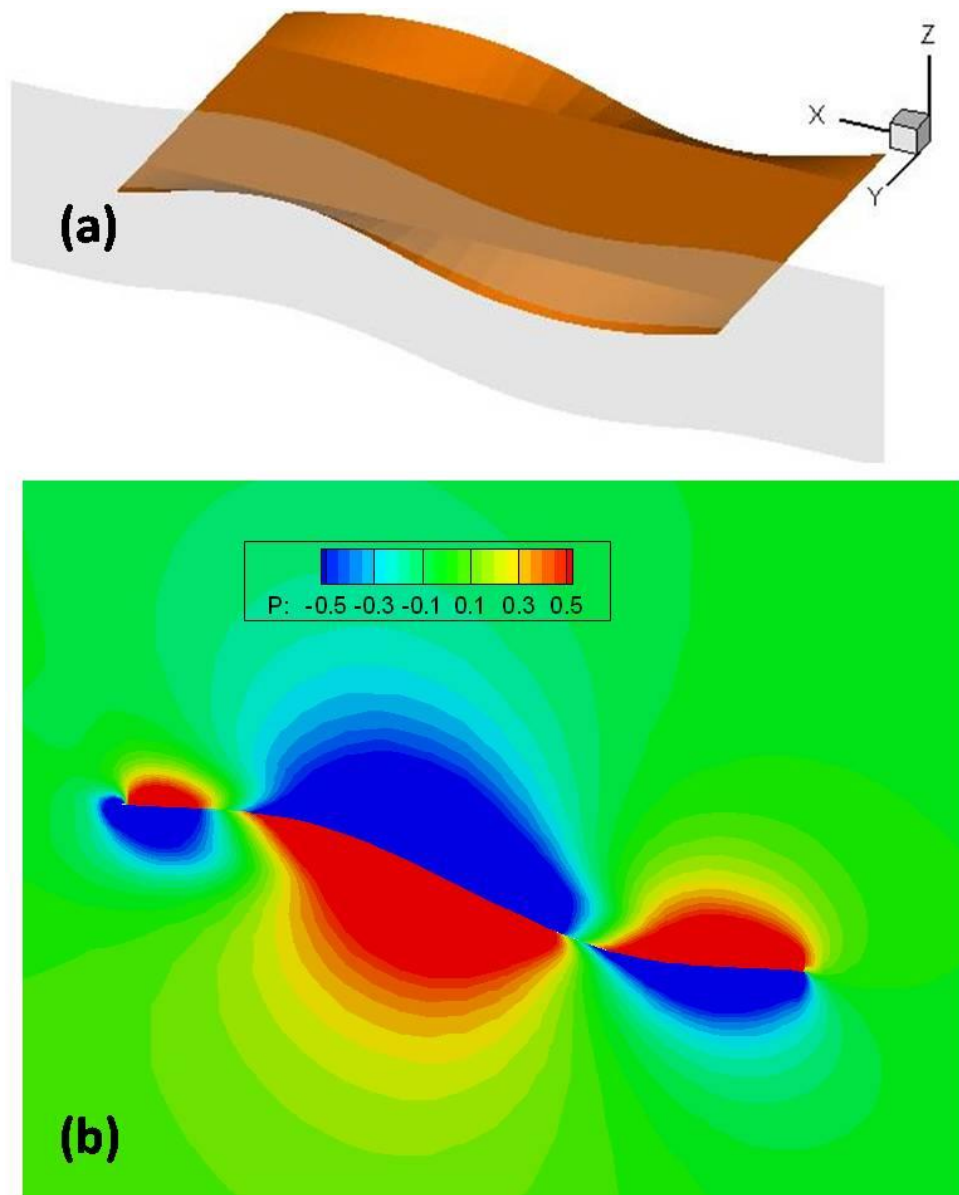
Fig. 2.15: (a) Slicing position at y = 0.275 ; (b) Pressure distribution on the upper and lower surfaces of the fin at y = 0.275
