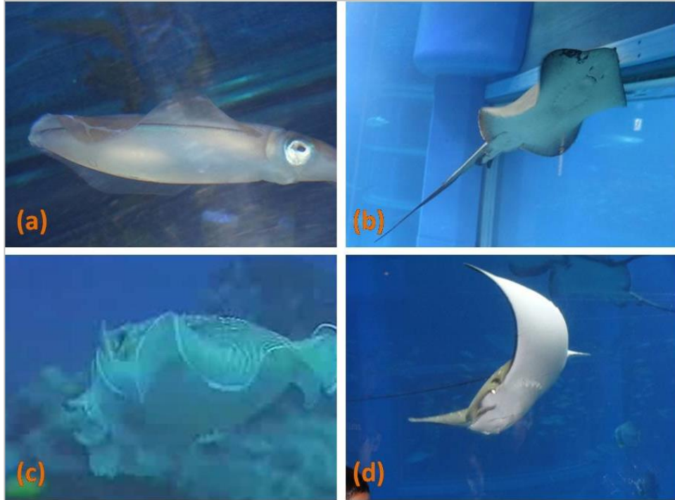
Fig. 1.1 Fishes which use undulating side fins for swimming; (a) Squid, (b) Stingray, (c) Cuttlefish, (d) Manta
