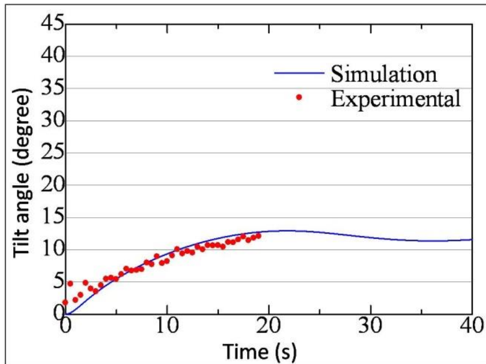
Fig. 4.8 Time history of the tilt angle for vertical motion
