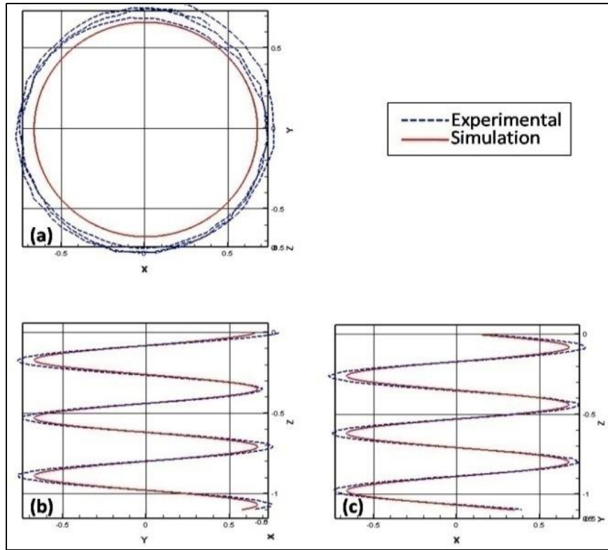
Fig. 4.14 Trajectory of the centre of gravity of the models in (a) XY-plane, (b) YZ-plane and (c) ZX-plane
