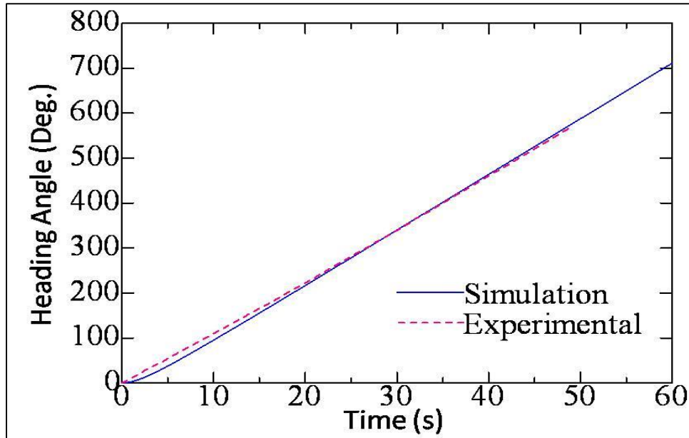
Fig. 4.6 Time history of the heading angle in circular motion
