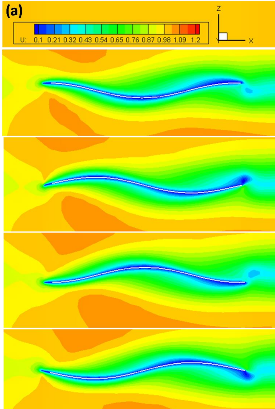
Fig. 2.28 (a) Contours of x -directional velocity distribution at \Theta = 30 , n = 3.18
