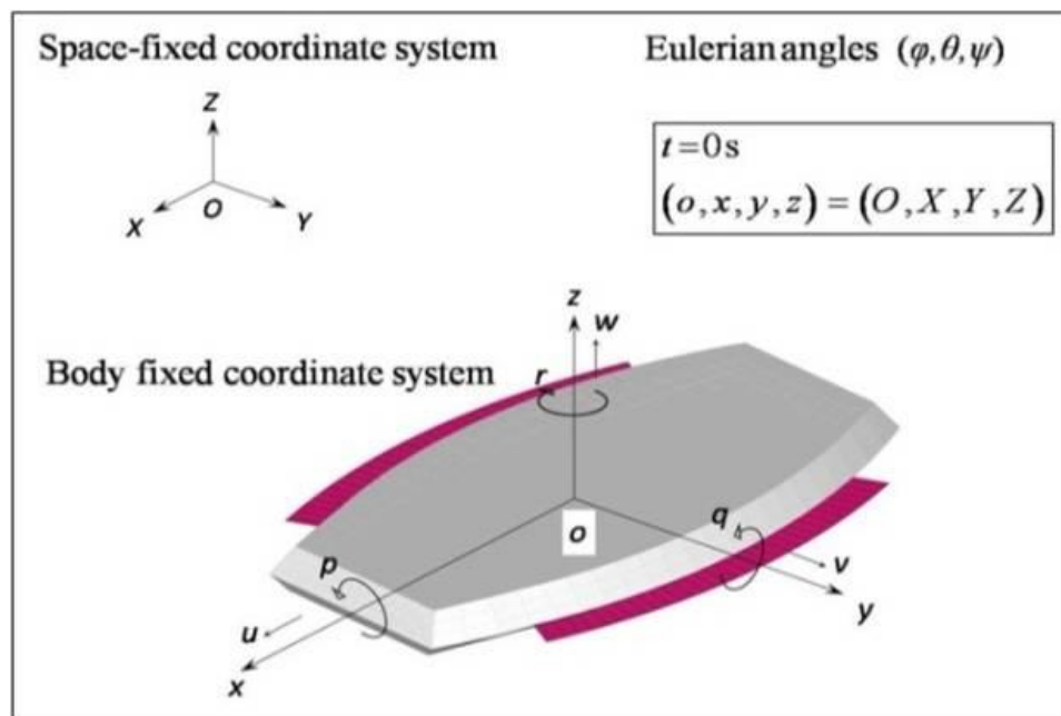
Fig. 3.3 Sketch of the coordinate system
