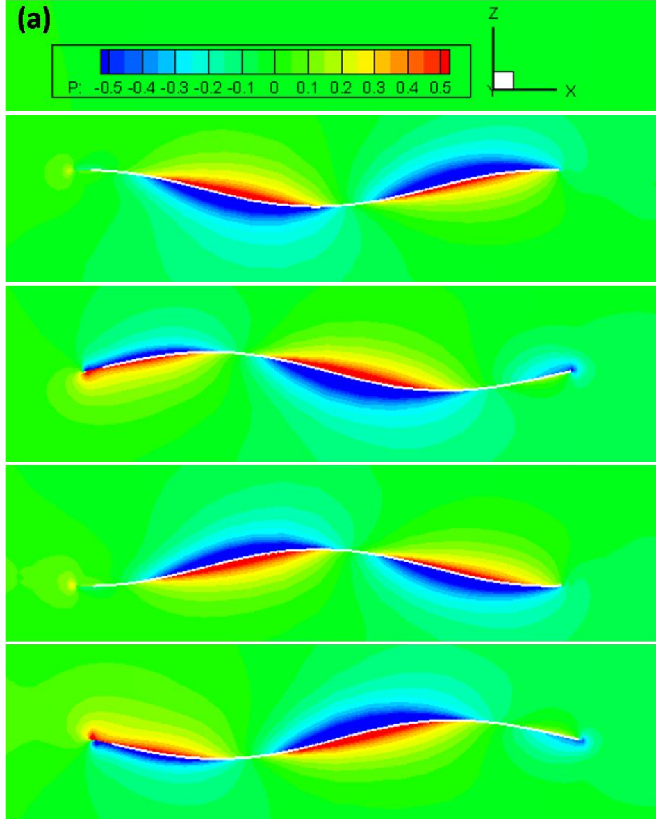
Fig. 2.29 (a) Contours of x -directional pressure distribution at \Theta = 30 , n = 3.18
