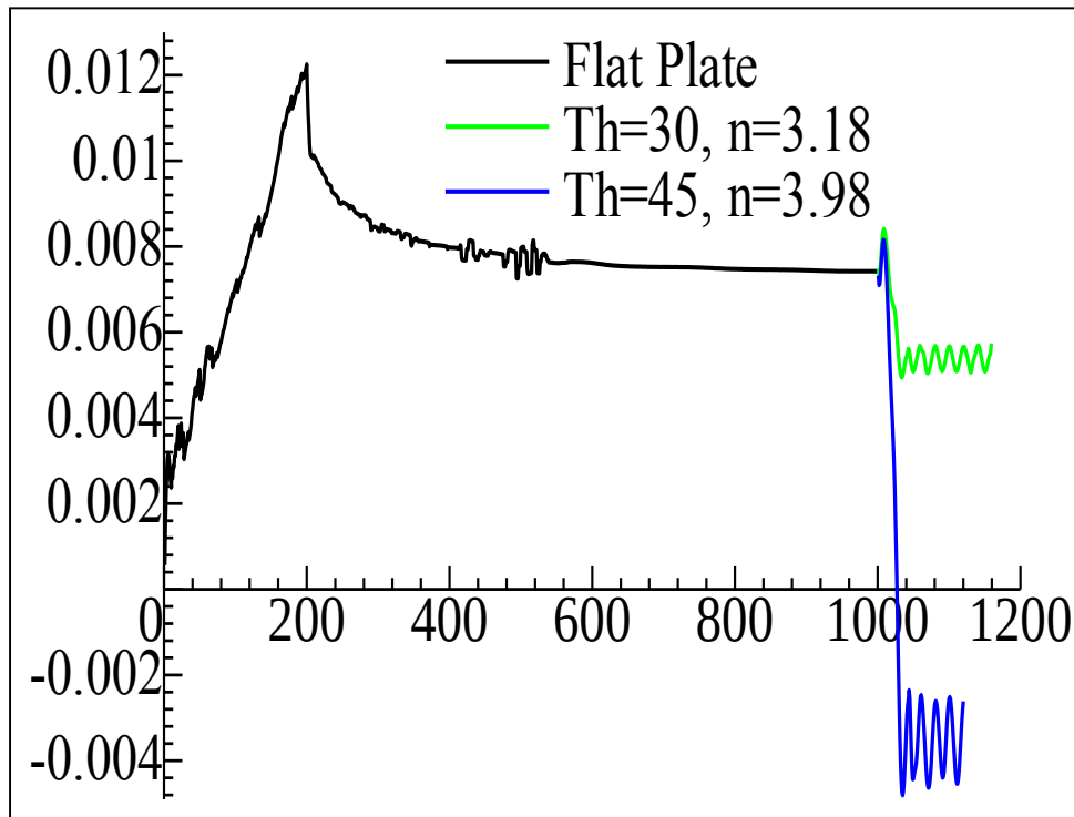
Fig. 2.24 Total x-directional force produced by body and fin
