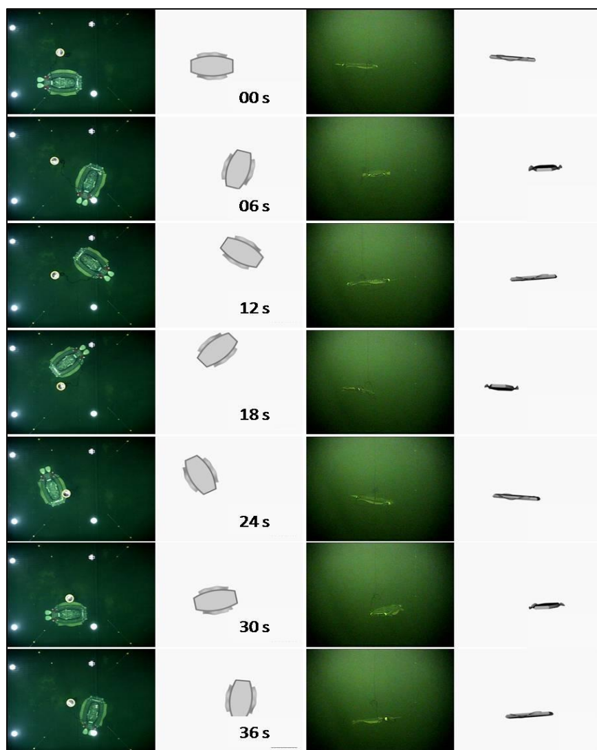
Fig. 4.16 Comparison of simulation result and experimental film in case of spiral motion by only side fins in 3D space
