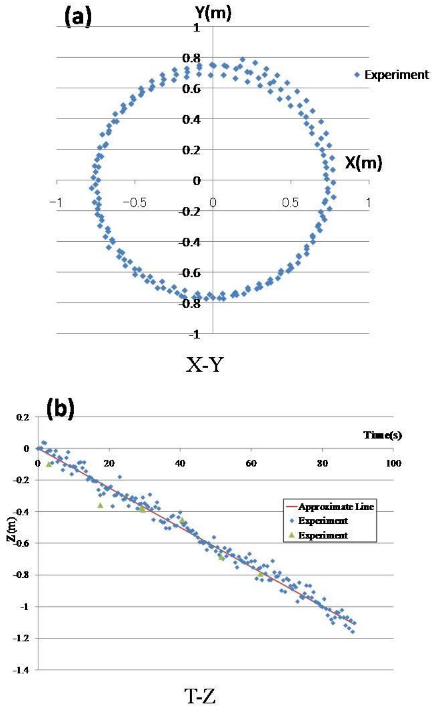
Fig. 4.12 Experimental result of spiral motion without caudal fins (a) Trajectory of the centre of gravity, (b) Distance in z-direction
