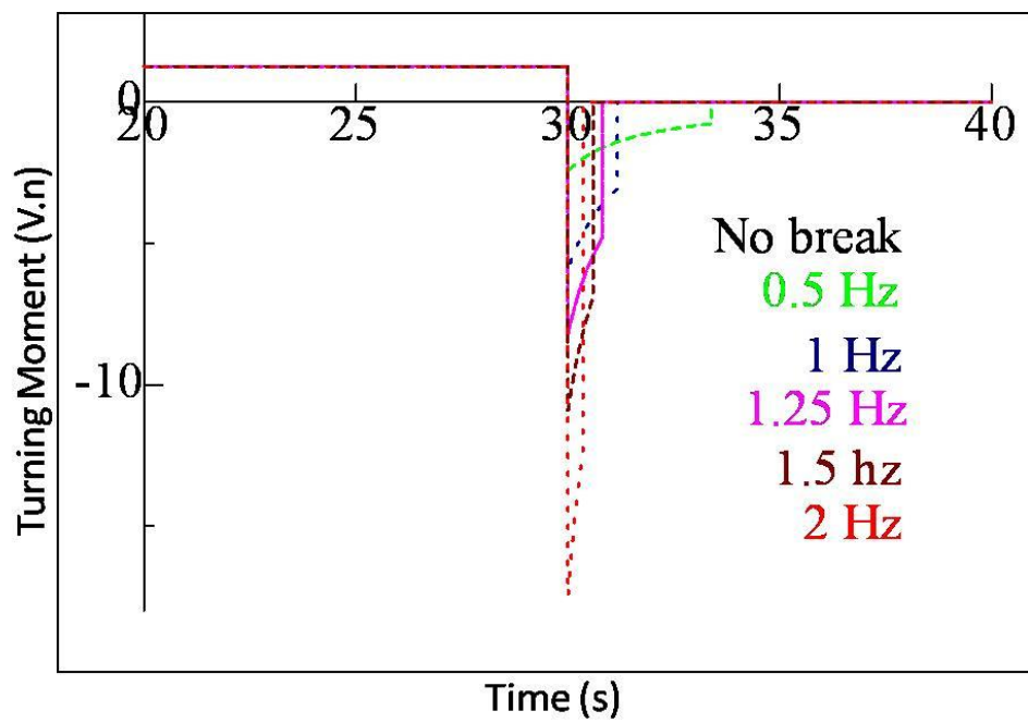
Fig. 3.14 The moment in angular motion with respect to time (enlarged view)
