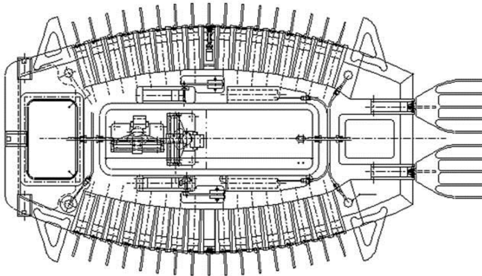
Fig. 2.2 Design of Model-4
