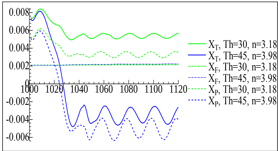
Fig. 2.25 Total force, frictional force and pressure force produced by body and fin
