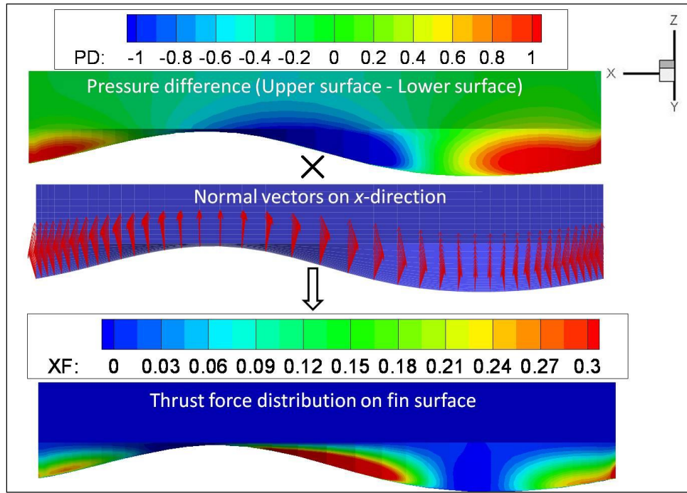
Fig. 2.16 The method of thrust calculation
