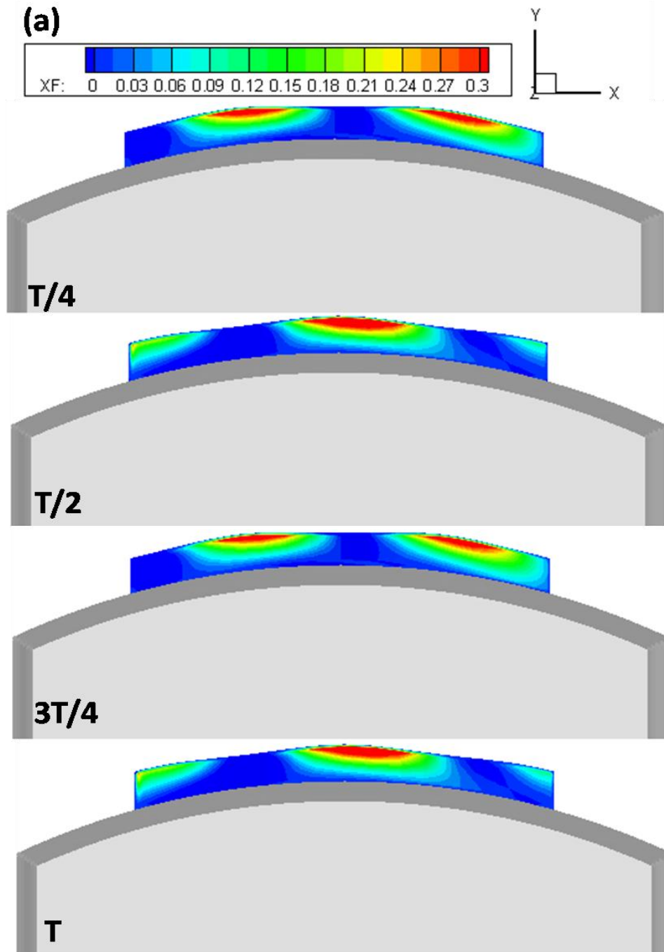
Fig 2.32 (a) The distribution of x -directional thrust force on the fin at \theta = 30 , n = 3.18
