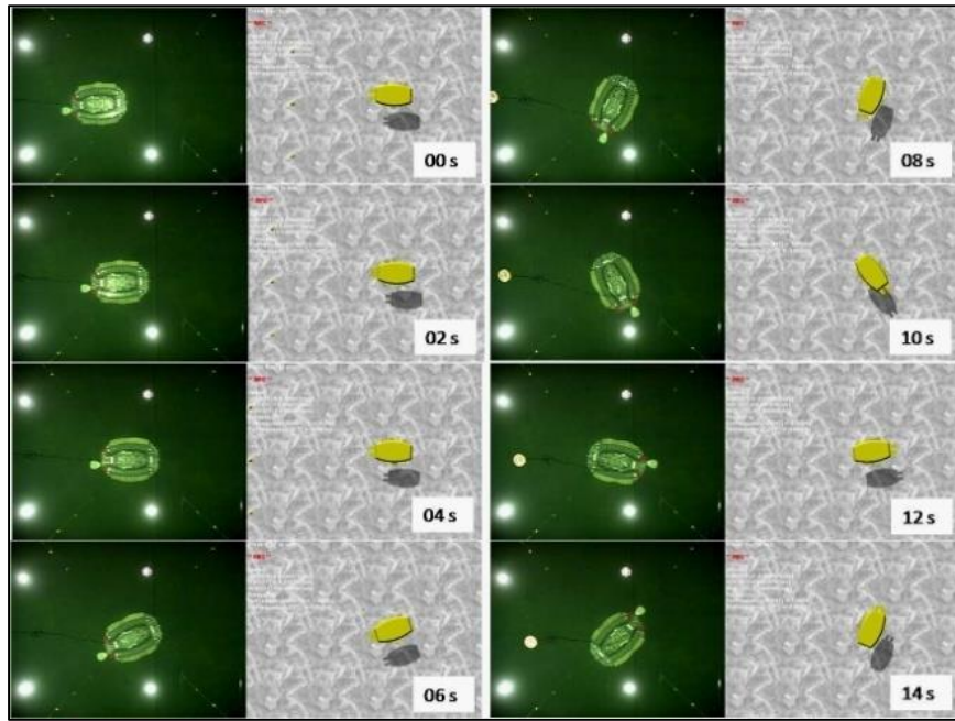
Fig. 4.20 Comparison experimental film and the real time simulator
