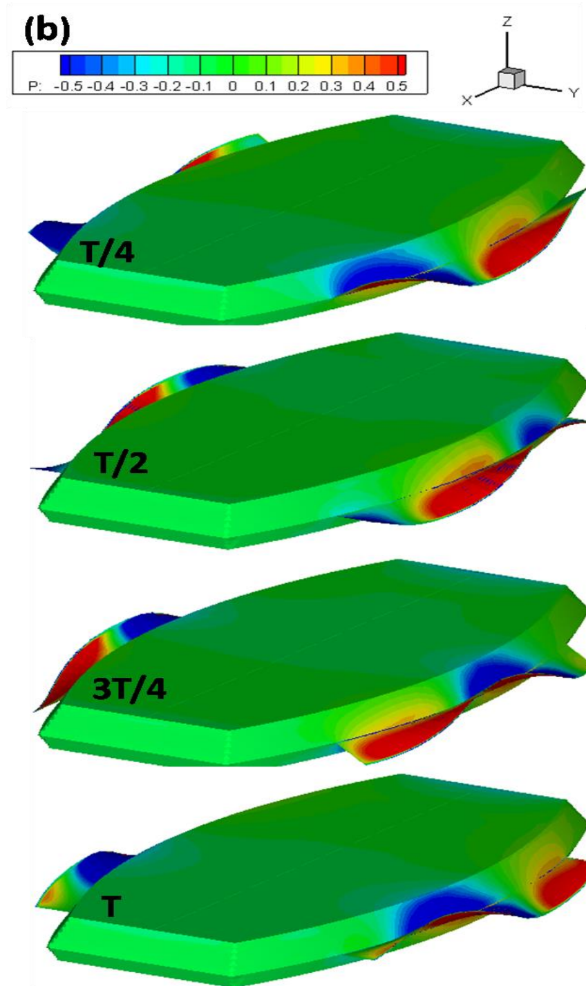
Fig. 2.30 (b) Pressure distribution on the Model-4 of Squid-robot at \theta = 45^\circ , n = 3.18
