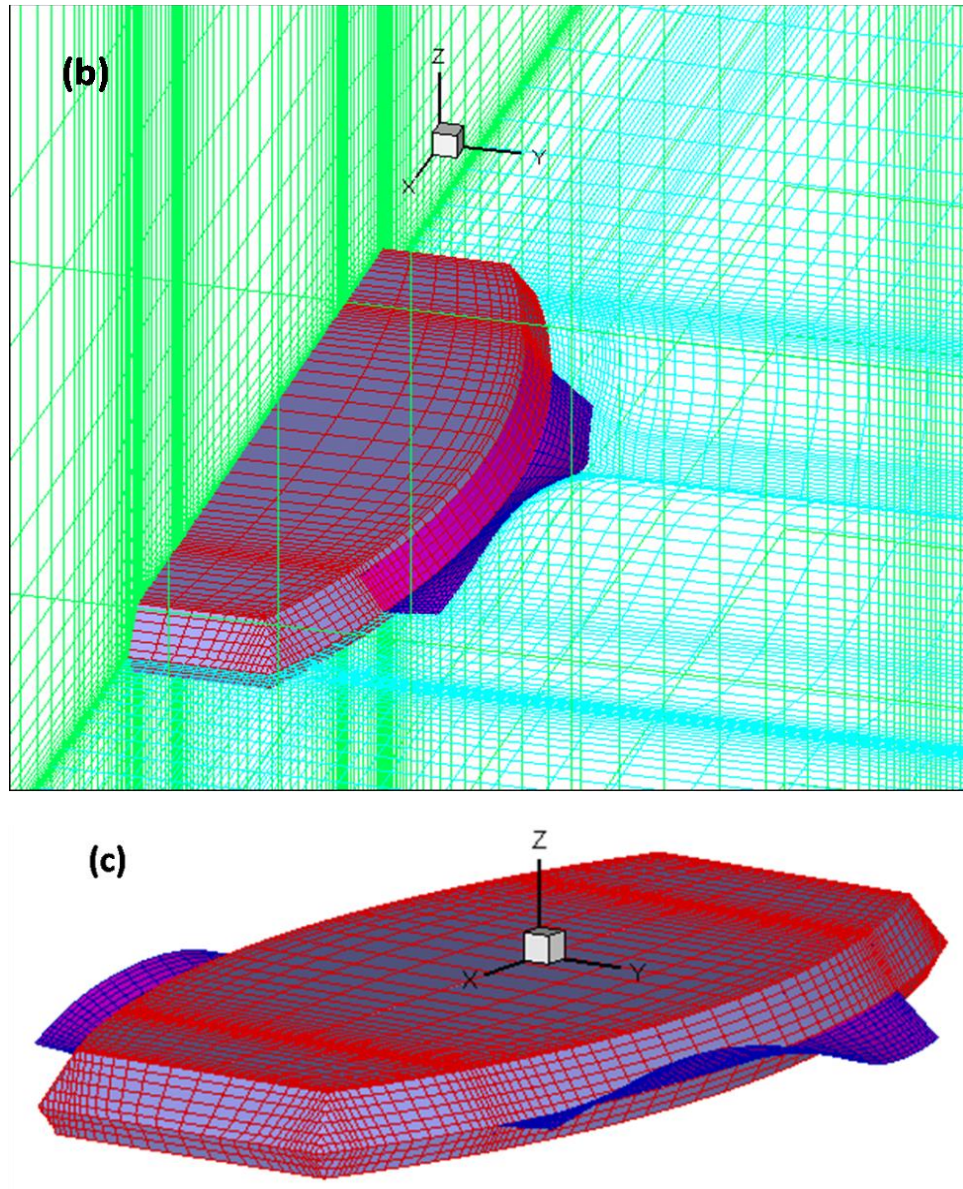
Fig. 2.6 Computational grid around Model-4 (a) Full grid, (b) Enlarged view (half) near the body, (c) Body grid
