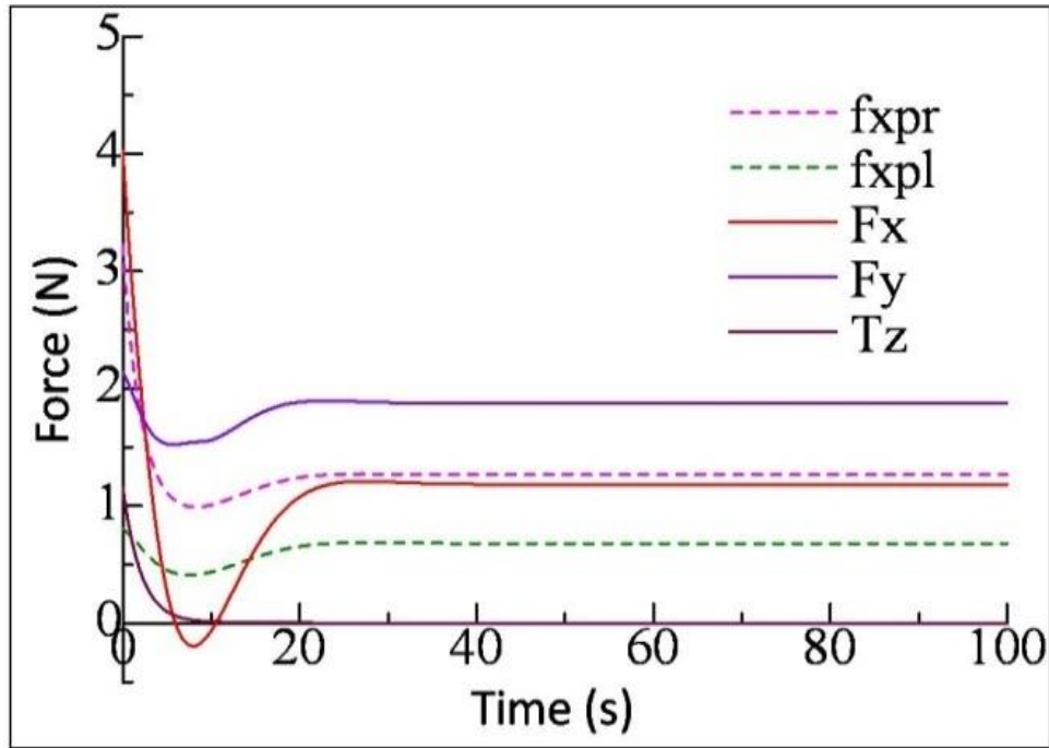
Fig. 4.3 Time history of the forces in circular motion
