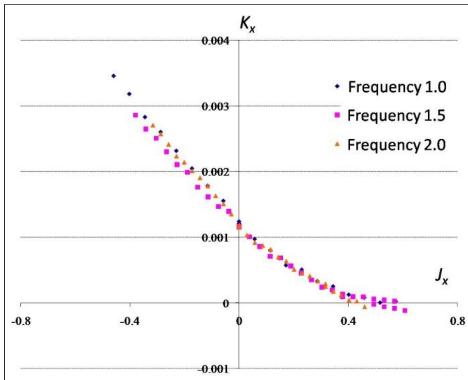
Fig.3.1 Fin Open characteristics ( K_x - J_x )
