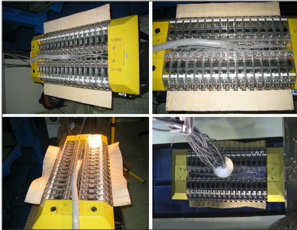
Fig. 1.3 Model-2 of the Squid-robot
