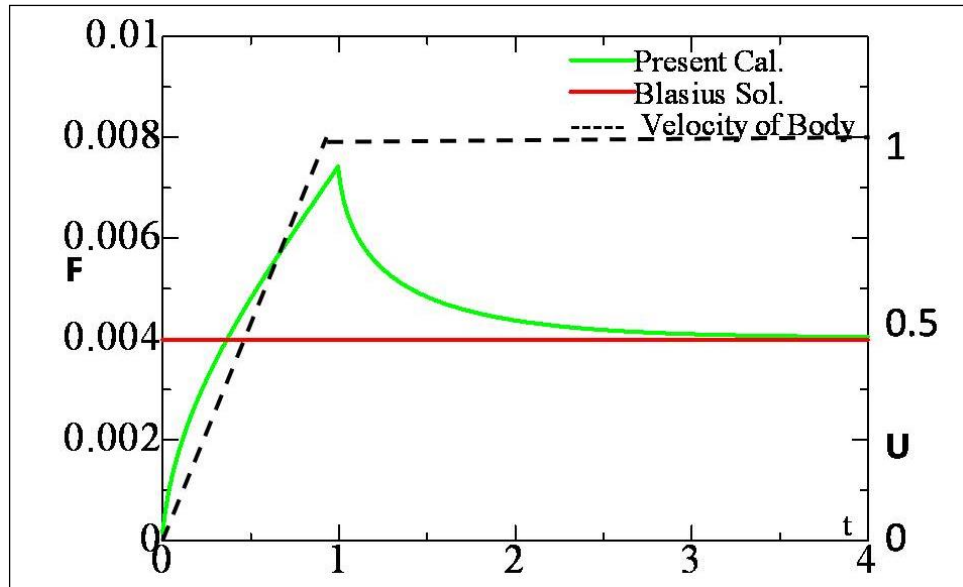
Fig. 2.7 Frictional force for a flat plate in acceleration stage and constant velocity stage
