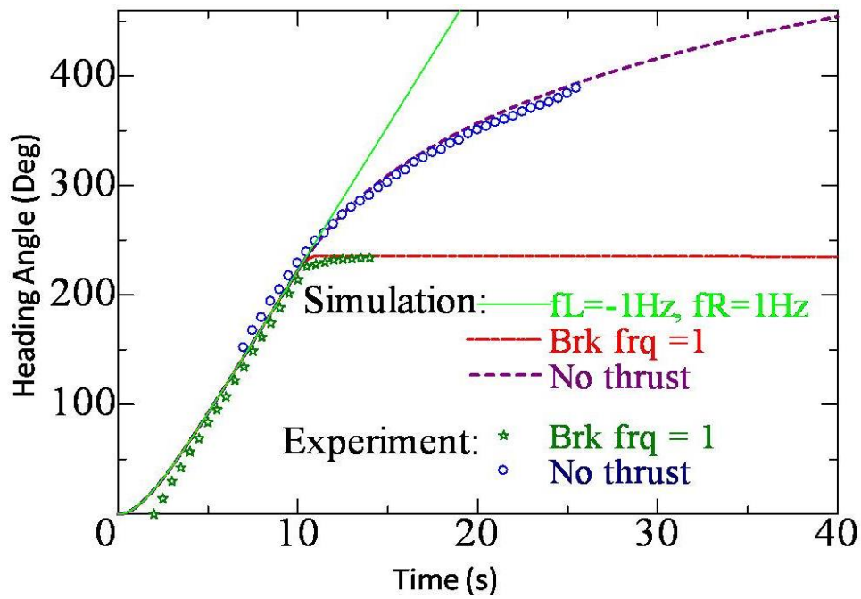
Fig. 3.7 Comparison of experimental and simulation results of heading angle in case of rotational motion with and without brake
