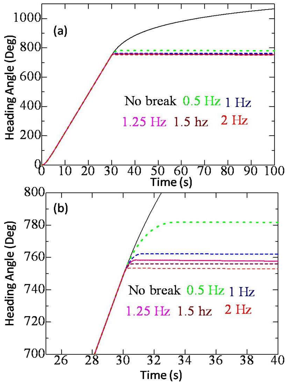
Fig. 3.12 (a) Heading angle in rotational motion with respect to time; (b) Enlarged view near the stopping point
