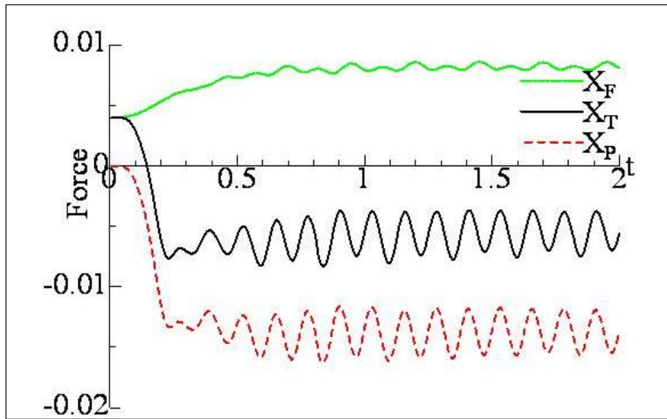
Fig. 2.8 Time history of x -directional forces for AR = 0.1 , n = 4 and \theta = 30^\circ
