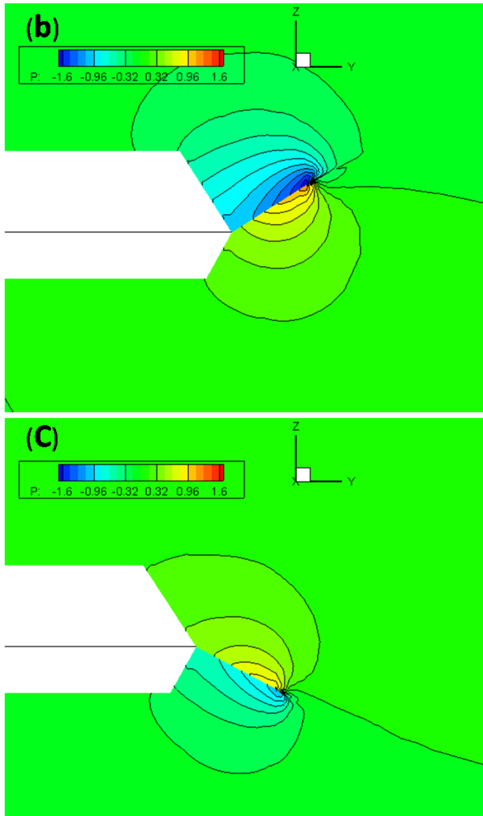
Fig. 2.36 Sectional view of pressure distribution at different x-stations on the body and on the fin of Model-4
