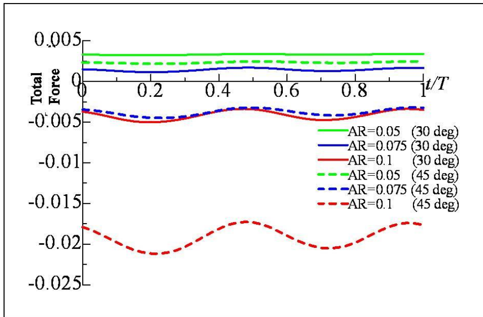
Fig. 2.11 Time history (one period) of the x-directional total force for n = 4 at different aspect ratios and maximum fin angles
