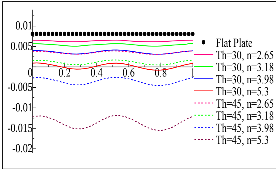
Fig. 2.26 Total x-directional force for different frequencies and fin angles produced by body and fin (one period)
