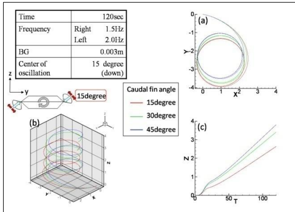
Fig. 4.10 Spiral motion where caudal fins and the side fins were used to change of depth
