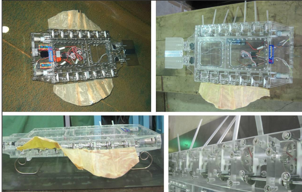
Fig. 1.6 Model-5 of the Squid-robot
