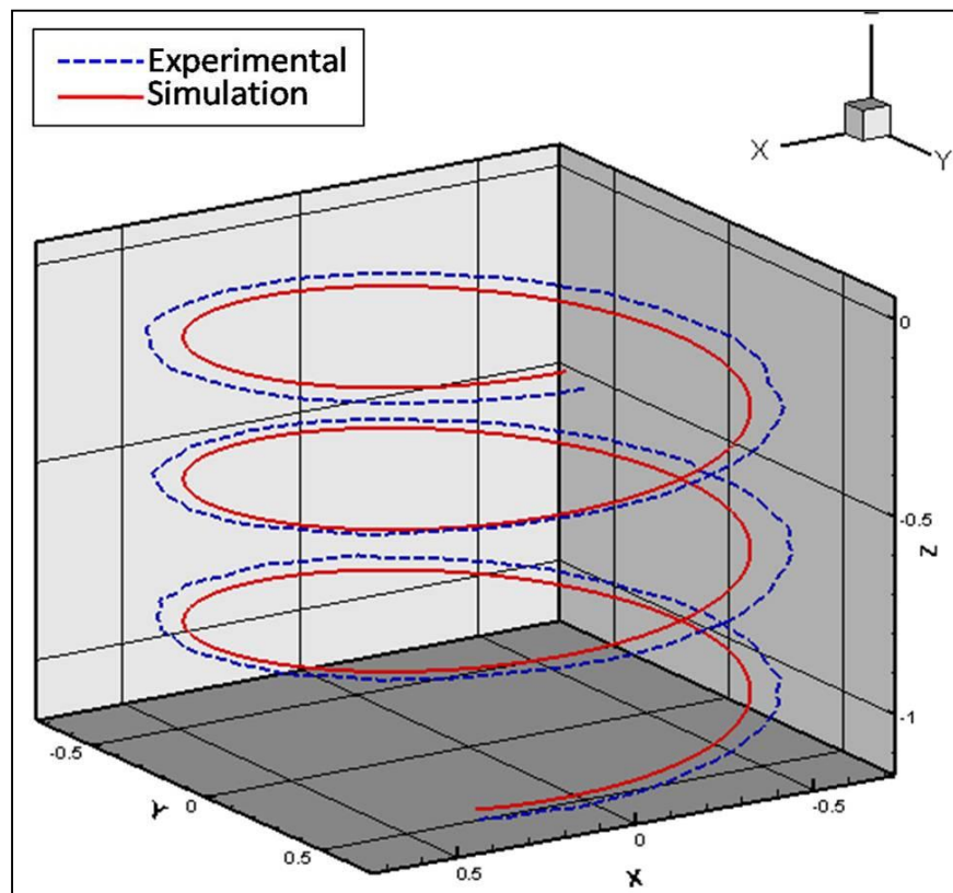
Fig. 4.13 Path of the centre of gravity of the models for spiral motion in 3D space
