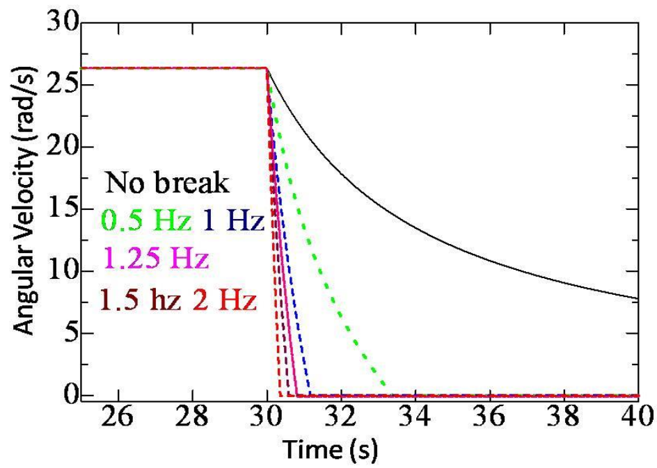
Fig. 3.13: The angular velocity with respect to time (enlarged view)
