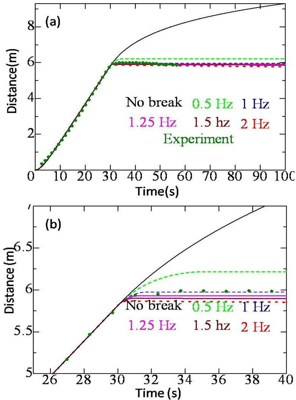
Fig. 3.8 (a) Travelled distance in translational motion with respect to time; (b) Enlarged view near the stopping point
