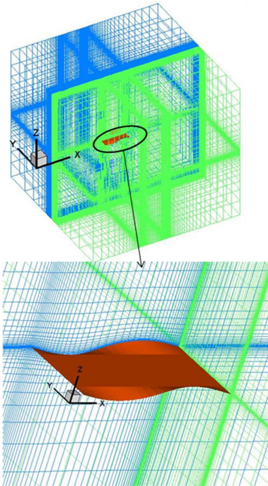
Fig. 2.5: (a) Full Computational grid of one time step (b) Enlarged view near the fin
