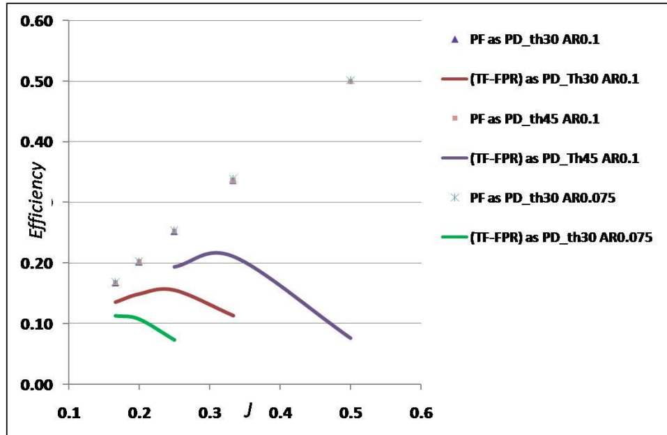
Fig. 2.20 Efficiency of the undulating side fin at different conditions
