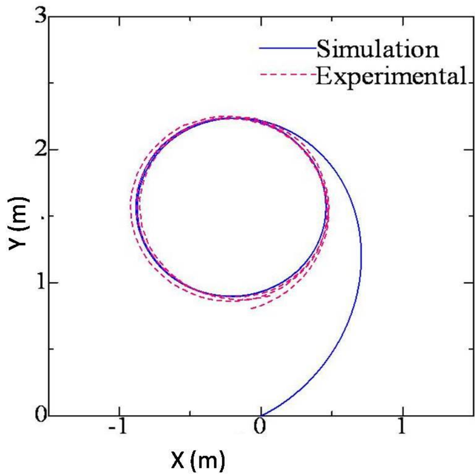
Fig. 4.5 Trace of the centre of gravity of the models in circular motion
