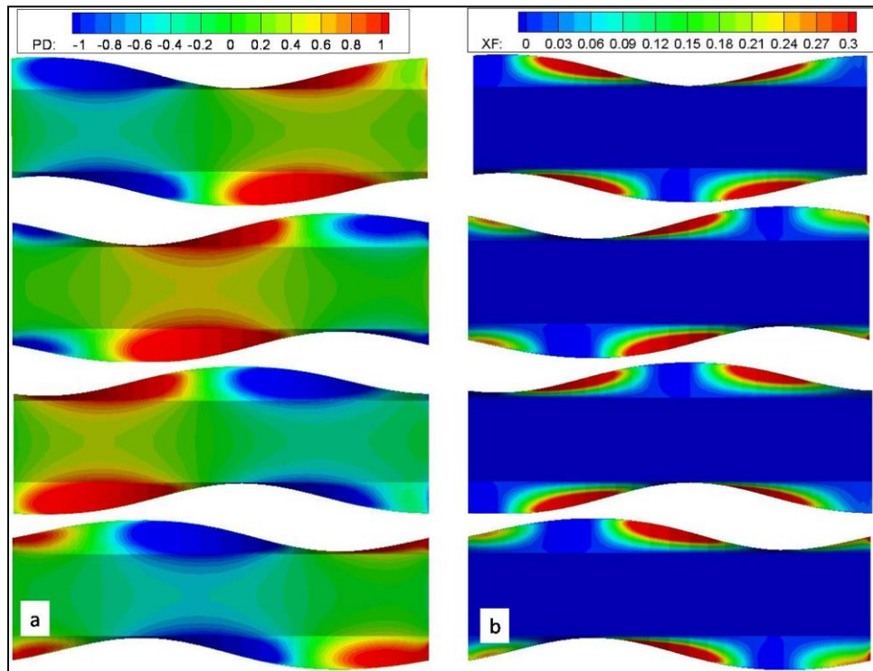
Fig. 2.17 (a) Distribution of pressure difference ( p_{\text{upper}} - p_{\text{lower}} ); (b) Distribution of x-directional thrust force on the full body of AR = 0.1 , n = 4 and \theta = 30^\circ at four time steps in one period
