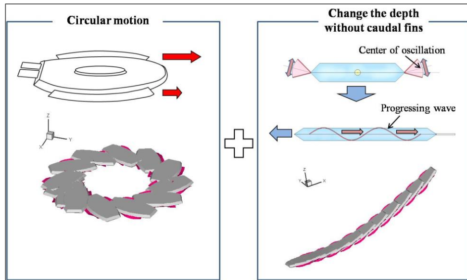
Fig. 4.11 Formation of spiral motion without caudal fins
