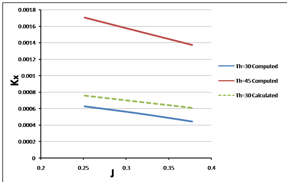
Fig. 2.33 Fin open characteristic \Theta = 30 and \Theta = 45
