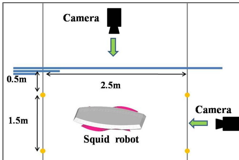
Fig. 3.2 Sketch of the experimental setup
