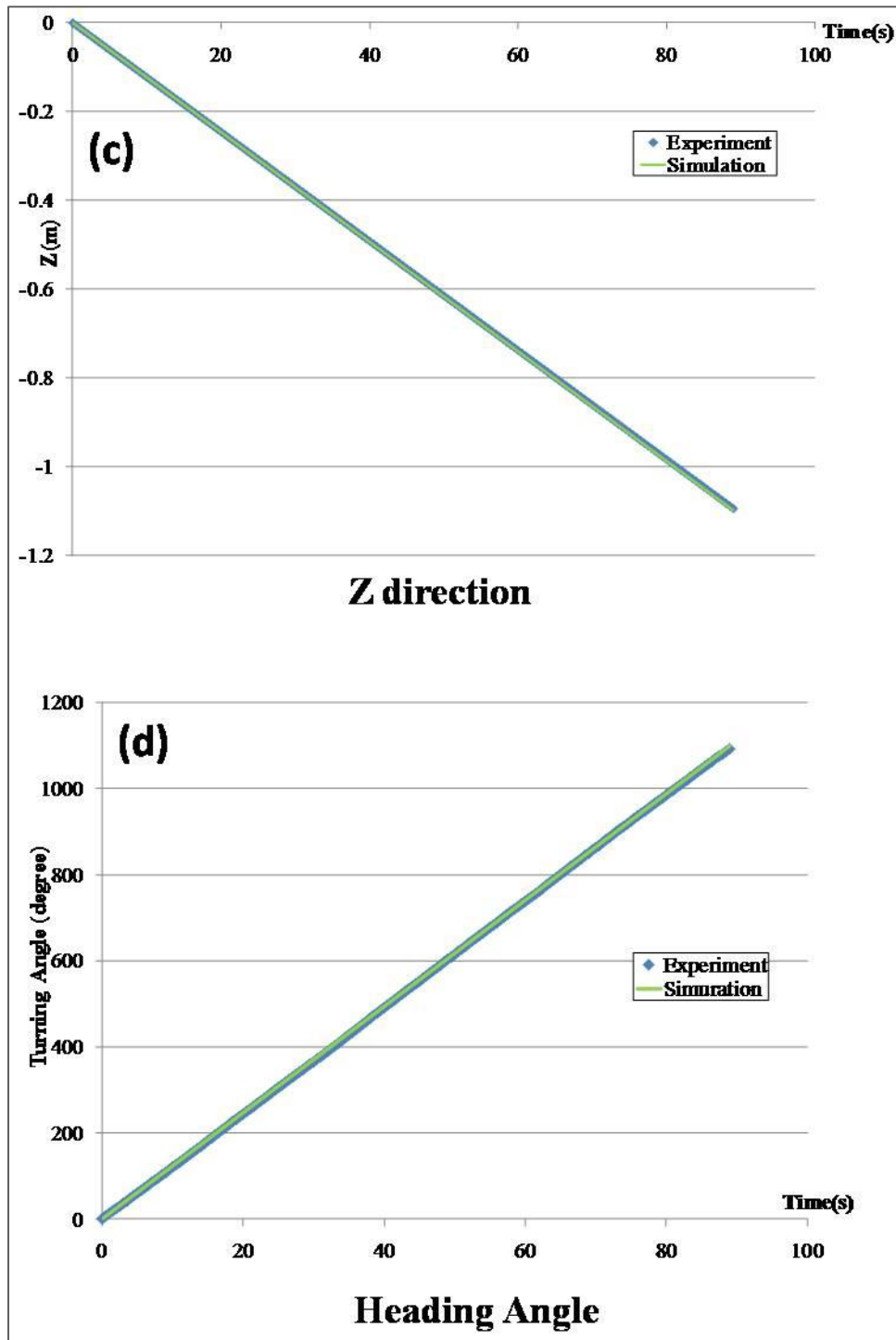
Fig. 4.15 The time series of X, Y, Z direction and heading angel
