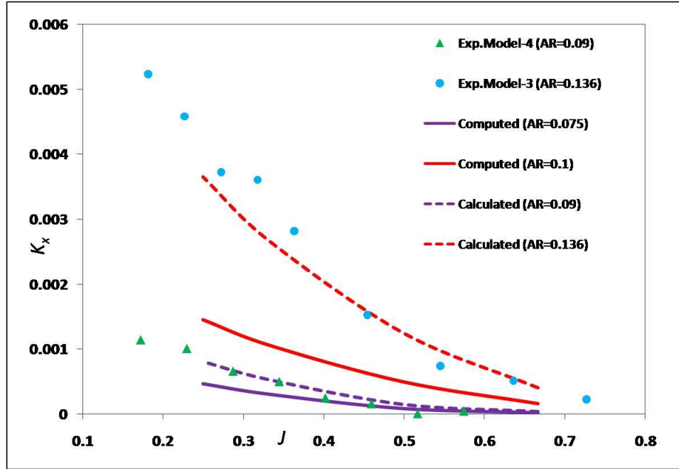
Fig. 2.23 Comparison among the computed, calculated and experimental results, \theta = 45^\circ
