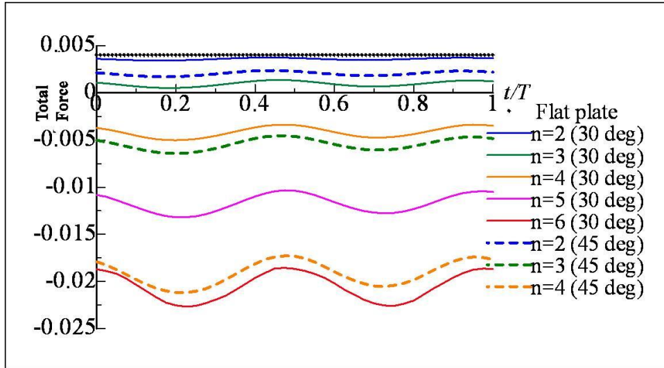
Fig. 2.10 Time history (one period) of the x-directional total force for AR = 0.1 at different frequencies and maximum fin angles
