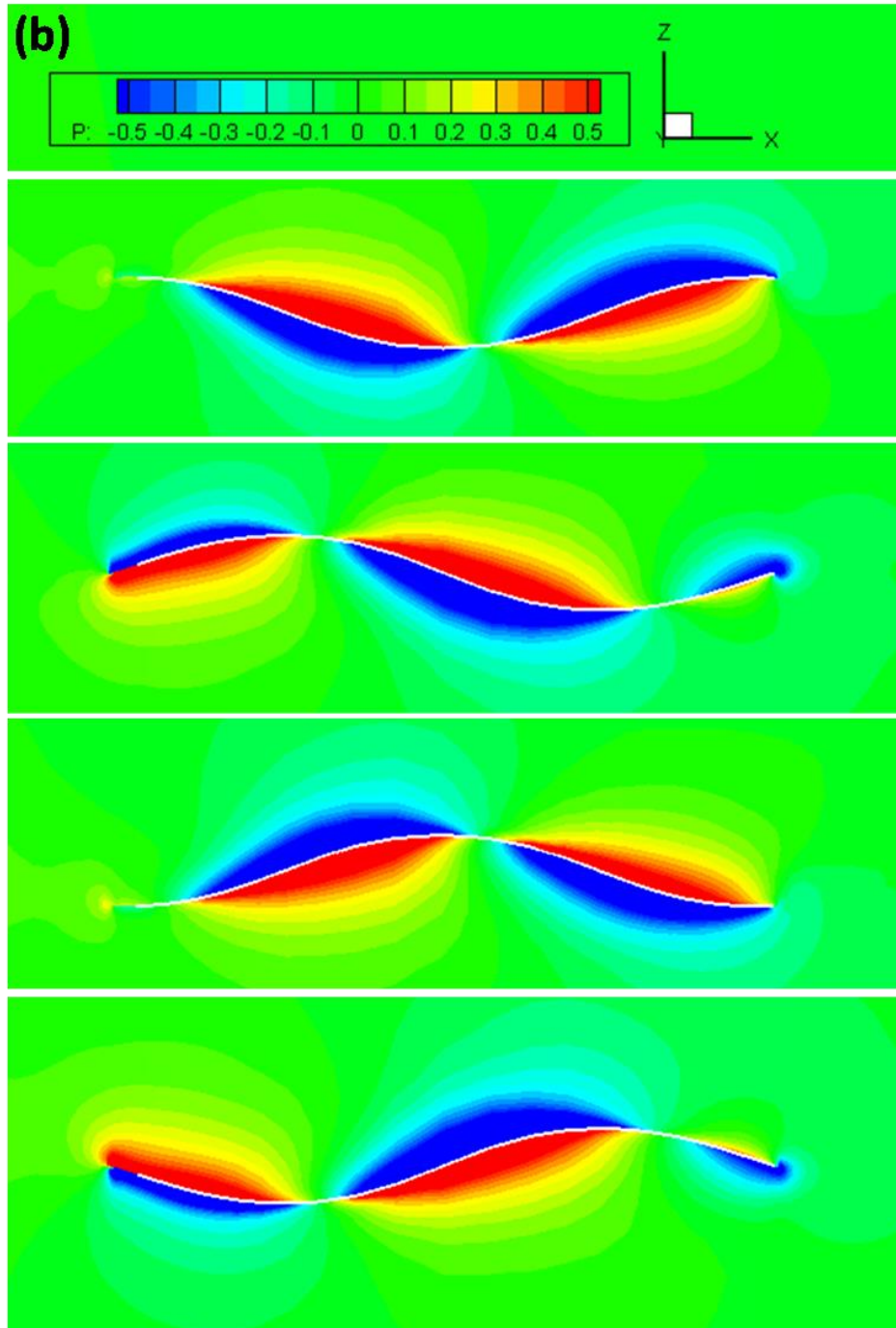
Fig. 2.29 (b) Contours of x -directional pressure distribution at \theta = 45 , n = 3.18
