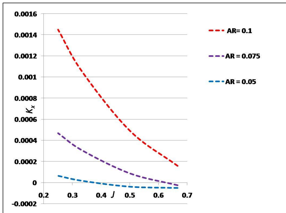
Fig. 2.19 Fin open characteristics, \theta = 45^\circ
