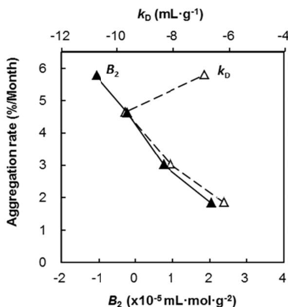
Figure 2.8. Relationship between aggregation propensity and B_2 or k_D for MAb-C
