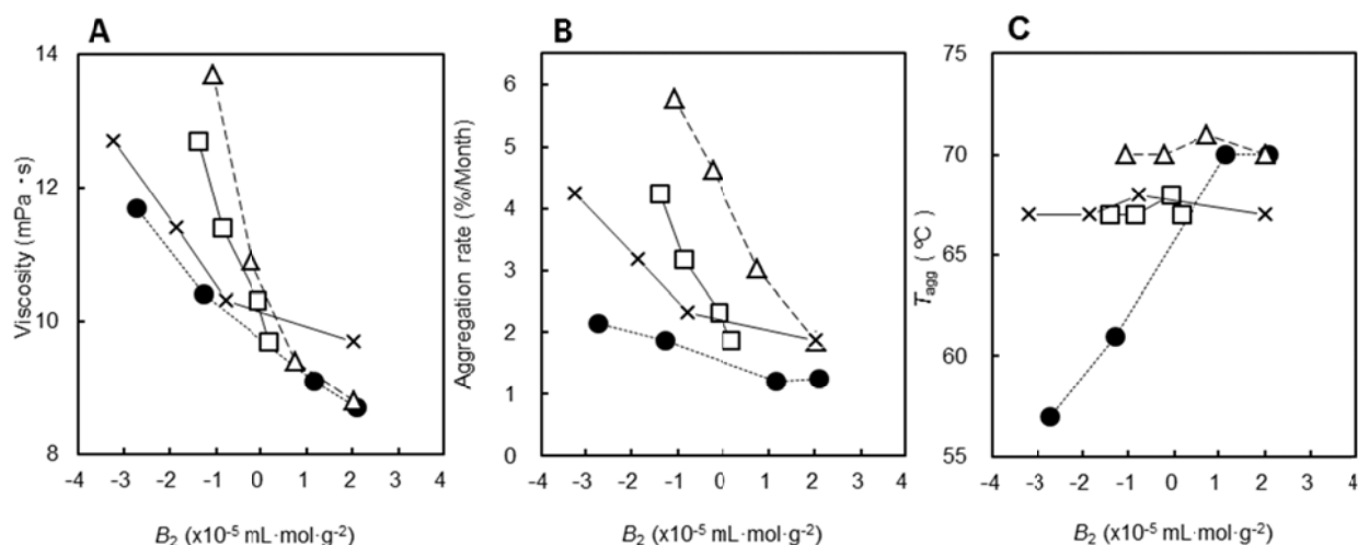
Figure 2.10. Correlation of B_2 with viscosity (A), aggregation propensity (B), and thermal stability (C): MAb-A (●), MAb-B (×: 1-3 mg/mL, □: 5-10 mg/mL), and MAb-C (Δ) B_2 values were obtained from AUC-SE. T_{agg} values were obtained from DLS. Viscosities were obtained at a concentration of 150 mg/mL, and aggregation rates were estimated based on SEC.
