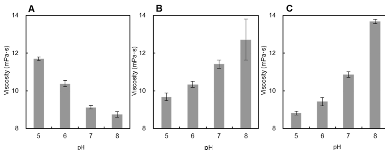
Figure 2.6. pH dependencies of viscosity
