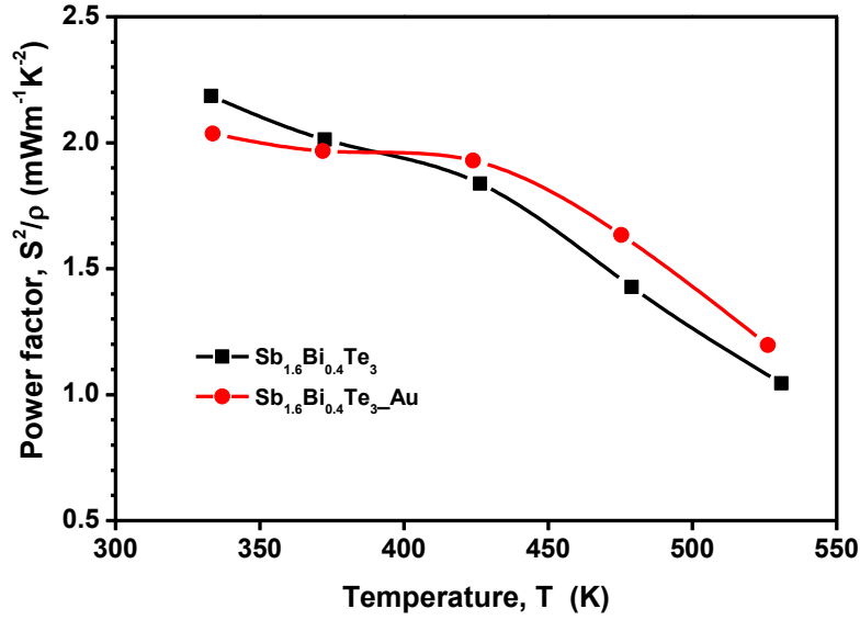
Figure 4. 15 Temperature dependences of the power factor S^2/\rho , of the Sb 1.6 Bi 0.4 Te 3 -Au bulk sample as compared with those of Sb 1.6 Bi 0.4 Te 3 .
