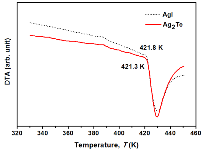
Figure 3.5 DTA curves of \text{Ag}_2\text{Te} and \text{AgI} . The values are corresponding to the phase transition temperature.
