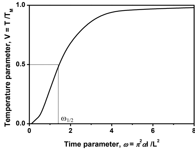
Figure. 2.8 Dimensionless plot of rear surface temperature history
