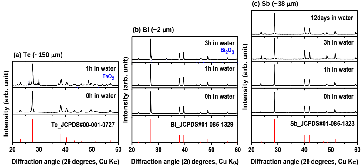
Figure 4.5 Stability of (a) Te microparticles, (b) Bi microparticles, and (c) Sb microparticles in the water as time passed. Te and Bi microparticles were easily oxidized in water in several hours, whereas Sb microparticles did not oxidize for over 10 days in water.
