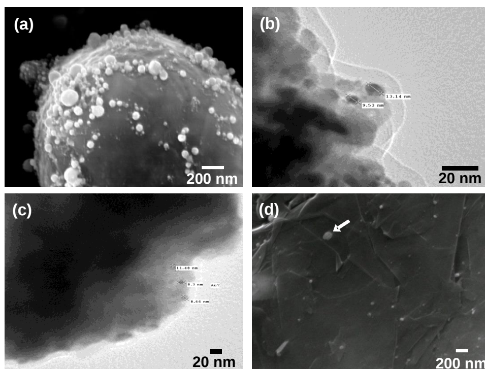
Figure 4.8 (a) SEM and (b) TEM images of Sb_Au composite after \gamma -ray irradiation. Nano-sized Au nanoparticles are supported on the surface of Sb particle. (c) TEM image of a \text{Sb}_{1.6}\text{Bi}_{0.4}\text{Te}_3 _Au after ball-milling. (d) SEM image of \text{Sb}_{1.6}\text{Bi}_{0.4}\text{Te}_3 _Au bulk sample. Au particles retain their nanosize during ball-milling and hot-pressing. One of the nanoparticles is indicated by an arrow.
