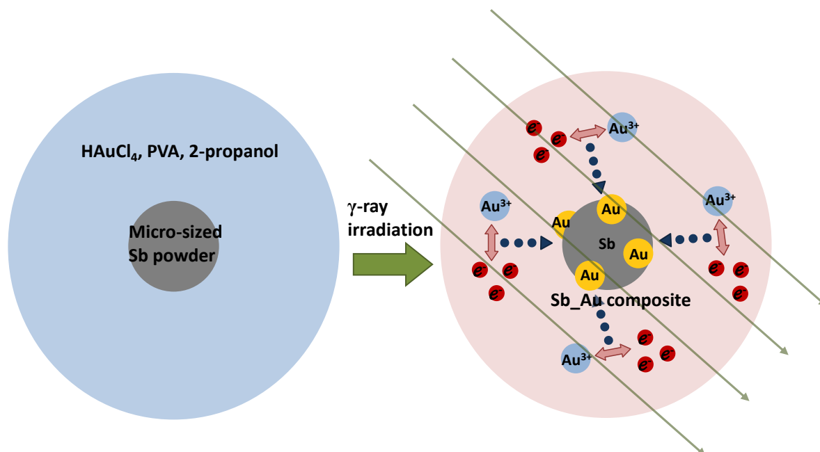
Figure 4.7 Process of the creation of Au nanoparticles on the surface of Sb particles during \gamma -ray irradiation. Hydrated electron ( e_{\text{aq}}^- ) and H radicals ( \text{H}\cdot ) generated by the \gamma -ray irradiation act as strong reducing agents, and they reduce Au ions down to the metallic state.
