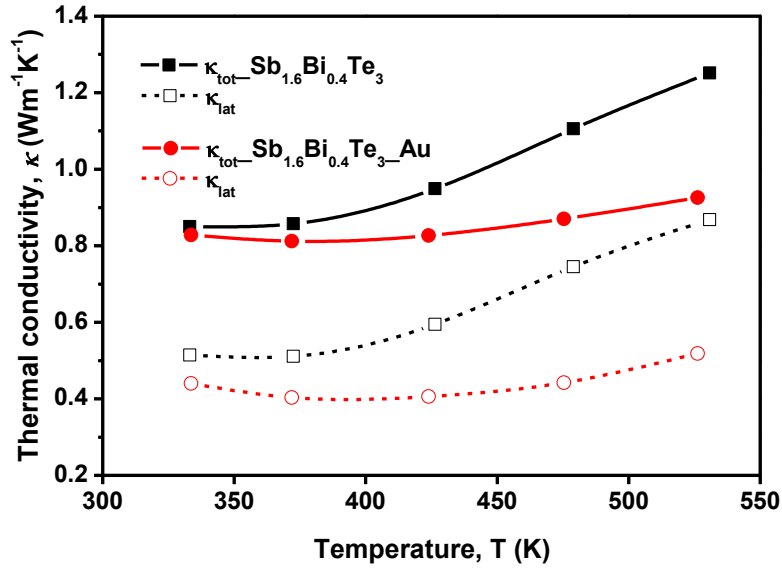
Figure 4. 16 Temperature dependences of the thermal conductivity \kappa , of the Sb 1.6 Bi 0.4 Te 3 -Au bulk sample as compared with those of Sb 1.6 Bi 0.4 Te 3 .
