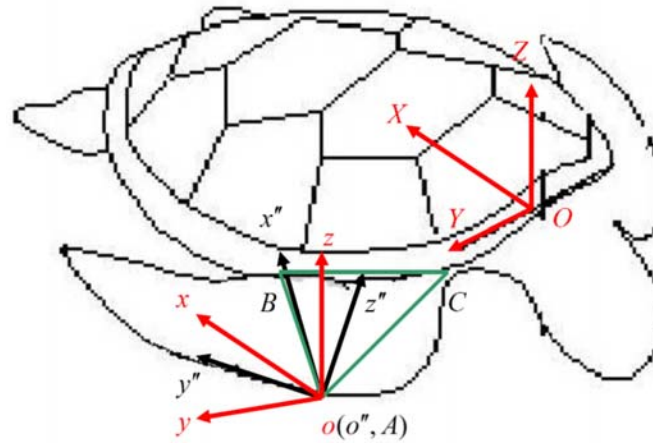
Figure 2.17 Determination of Euler angle \gamma and \phi
