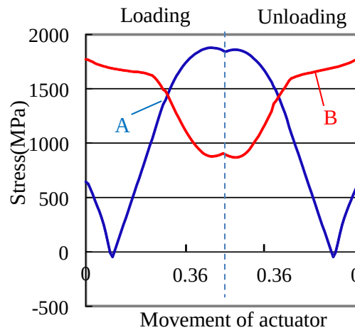
Fig. 5.2 Stress history of point A and point B of model M ( R1=1.38 , R2=1.38 )
