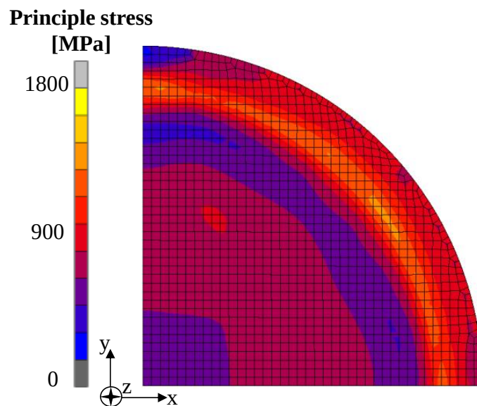
Fig. 3.5 Principle stress after cutting frame
