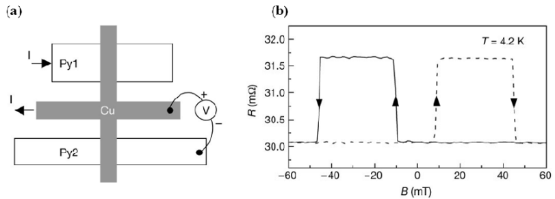
Figure 1-19. Electrical spin injection and accumulation in an Py/Cu/Py spin valve. (a) Nonlocal measurement geometry. (b) Nonlocal MR loop measured at 4.2 K. From Ref. [58].
