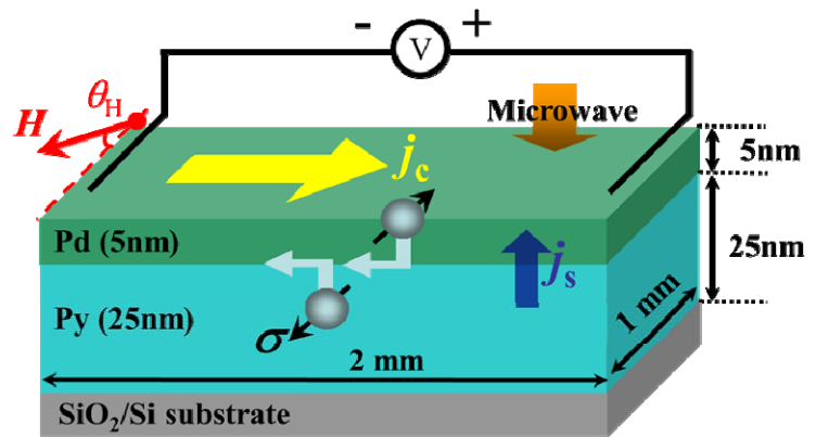
Figure 4-1. Schematic illustration of the Py/Pd bilayer sample used in this study. H represents an external magnetic field and \theta_H the angle of the external magnetic field. The dimensions of the sample are shown in the figure.
