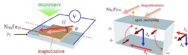
Figure 1-25. Schematic view of Py/Pt spin pumping device. From Ref. [88].
