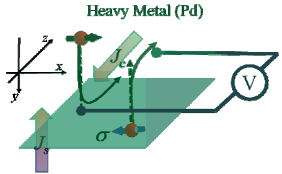
Figure 2-7. A schematic view of ISHE.
