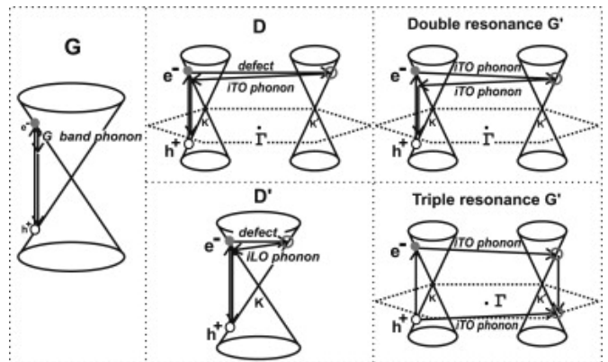
Figure 1-17. The origins from the main bands in graphene. From Ref. [49].
