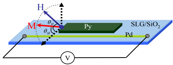
Figure 3-11. A schematic illustration of Py/SLG/Pd.
