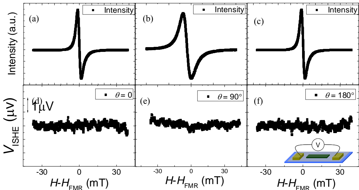
Figure 3-6. (a)-(f) Results of control experiment of Py/SLG sample. a-c) Ferromagnetic resonance spectra of the Py under the external magnetic field at a) 0^\circ , b) 90^\circ and c) 180^\circ under the microwave power of 200 mW. d-f) Electromotive forces from the Pd wire on the SLG when \theta is set to be d) 0^\circ , e) 90^\circ and f) 180^\circ . No electromotive force was detected from the sample.
