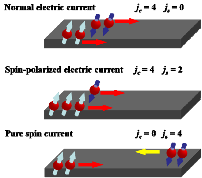
Figure 2-1. Concept of electric current and spin current.
