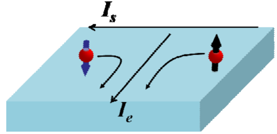
Figure 2-6. A schematic view of ISHE.
