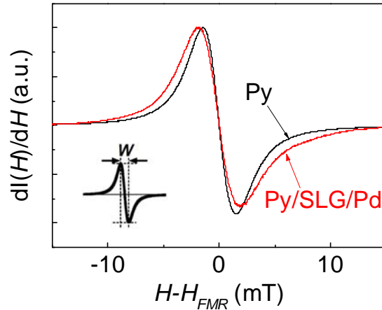
Figure 3-12. The black and red solid lines are the FMR spectrum of the Py on the \text{SiO}_2 substrate and the Py/SLG/Pd on the \text{SiO}_2 substrate, respectively.
