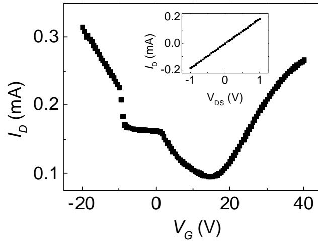
Figure 3-9. FET characteristics of SLG sample 1. The inset shows the the I - V curve of the source-drain current. The measurement was carried out at room temperature.
