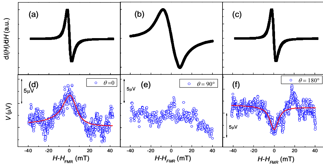
Figure 3-5. Results on spin pumping and spin transport in sample #2. (a)-(c) Ferromagnetic resonance of the Py under \theta is set to be (a) 0^\circ , (b) 90^\circ and (c) 180^\circ under the microwave power of 200 mW. (d)-(f) Electromotive forces from the Pd wire on the SLG when \theta is set to be (d) 0^\circ , (e) 90^\circ and (f) 180^\circ under the microwave power of 200 mW. Electromotive forces can be observed as expected, indicating successful dynamical spin injection. However, the signal was weak and noisy. The red solid lines in (d) and (f) show the fitting lines obtained by using Eq. (3, 4).
