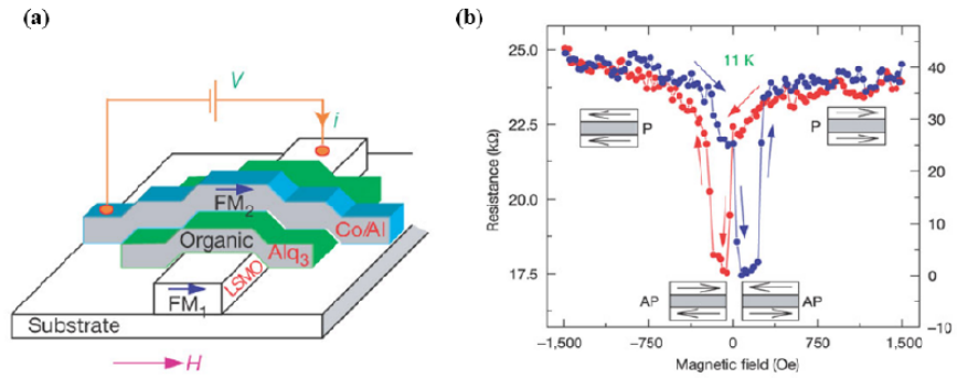
Figure 1-6. Organic semiconductor spin valves. (a) \text{Alq}_3 device geometry. One FM electrode is LSMO, and the other FM electrode is Co. (b) MR loop measured at 11 K with a negative MR of 40%. From Ref. [25].
