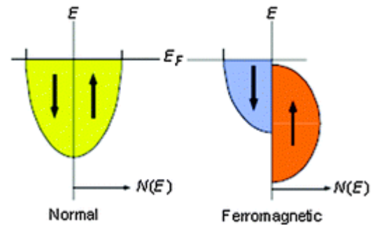
Figure 1-1. The DOS for a non-magnetic material and a ferromagnetic material.
