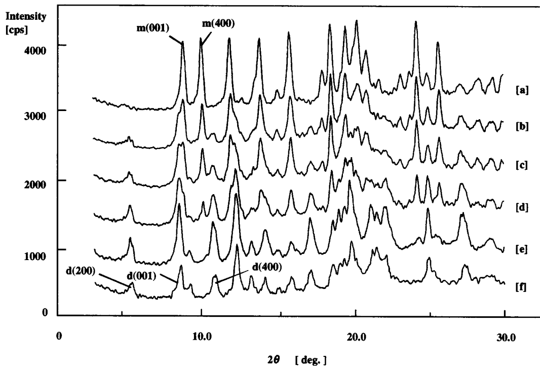
Fig. 5 X-ray powder diffraction patterns of (a) a 1:1 complex(12) of 1a with (-)- 2a (b) after UV irradiation for 10min (c) after UV irradiation for 30min (d) after UV irradiation for 90min (e) after UV irradiation for 4hr (f) a 2:1 complex(13) of (-)- 2a with (-)- 3a m(001) and m (400) in [a] are the mirror indices for complex(12). d(200) ,d (001) and d(400)in [f] are the mirror indices for complex(13).
