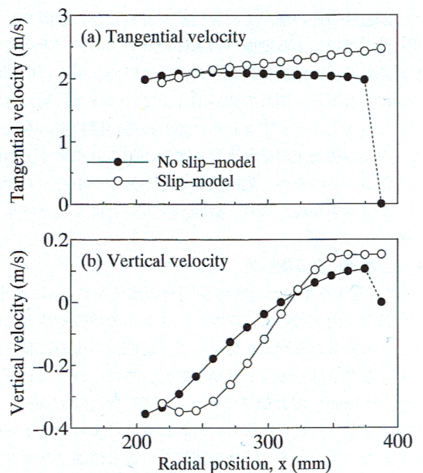
Fig. 10. Radial profile of the tangential and vertical velocities at z=500\text{ mm} .
