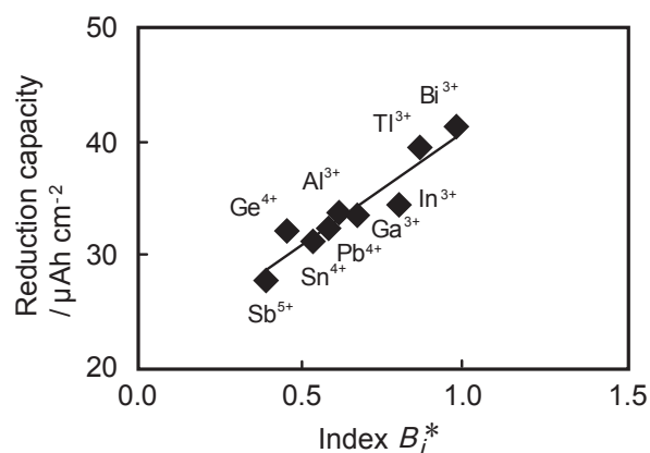
Fig. 7 Relationship between electrochemical reduction capacity and reciprocal value of columbic bonding strength for metallic ion and oxygen ion expressed by formula of (r_i+1.40)^2/2 Z_i .
