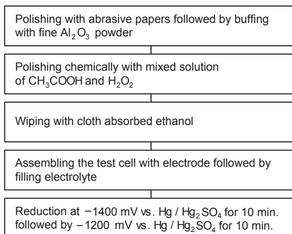
Fig. 2 Procedure of pretreatment of lead alloy electrode.
