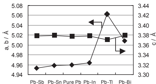
Fig. 5 Lattice constant of \beta -PbO 2 formed on surface of various alloy substrates.
