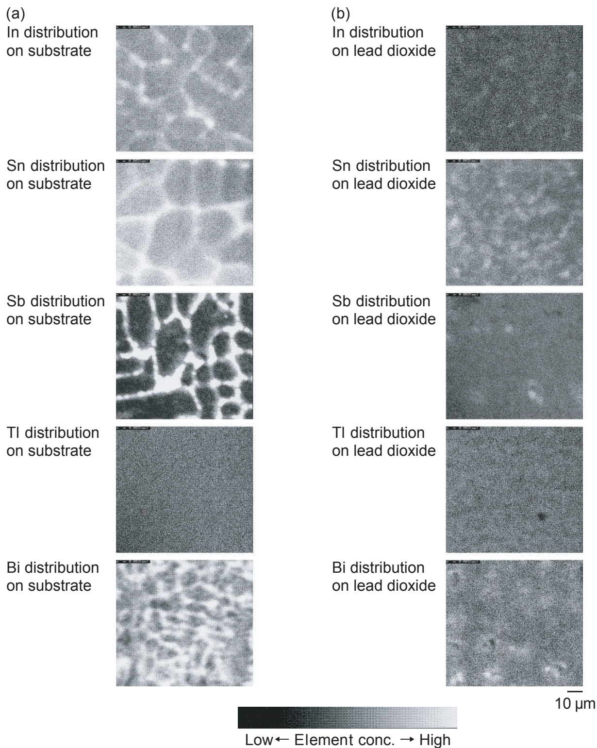
Fig. 6 Distribution of various elements in alloy substrate (a) and lead dioxide layer (b) formed on its substrate.
