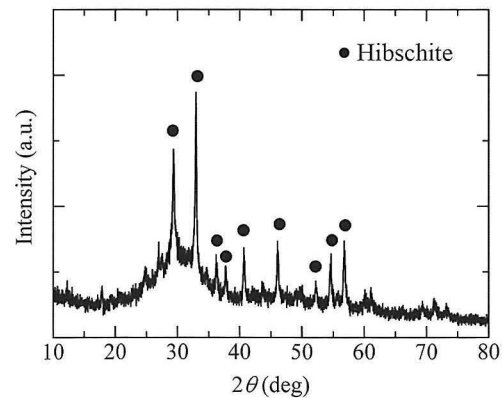
Fig.4 XRD pattern for solidified BF slag compact after the hydrothermal-hot-pressing at 573 K for 1 h
