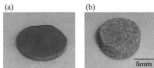
Fig.5 Solidified slag compacts after the hydrothermal hot pressing; initial particle size (a) <15 \mu\text{m} , (b) 250 ~ 500 \mu\text{m}
