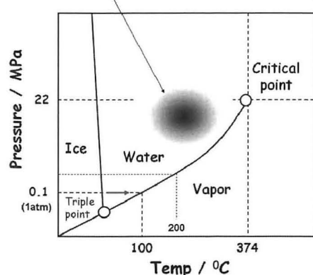
Fig.1 Phase diagram of H 2 O
