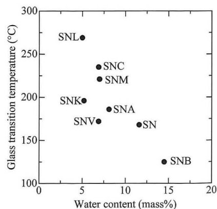
Fig.7 Relationship between glass transition temperature and water content of the glass after the hydrothermal treatment; SiO_2 - Na_2O - M_xO_y ( M_xO_y \sim 0 (SN), Al_2O_3 (SNA), B_2O_3 (SNB), CaO (SNC), K_2O (SNK), Li_2O (SNL), MgO (SNM), V_2O_5 (SNV))
