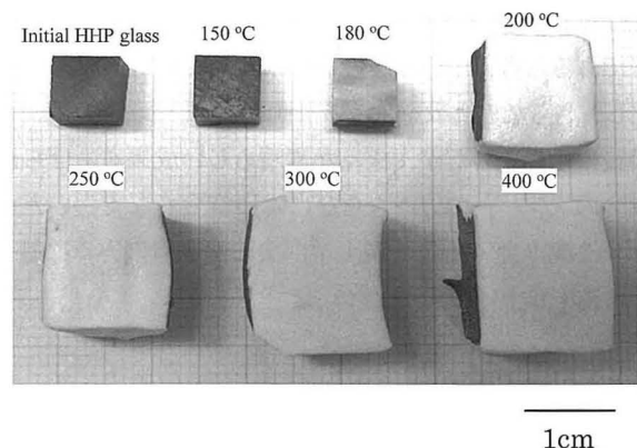
Fig.9 Change in macroscopic shapes of the hydrothermally treated 63mass%SiO 2 -27mass%Na 2 O-10mass%B 2 O 3 glass after firing at 150-400℃
