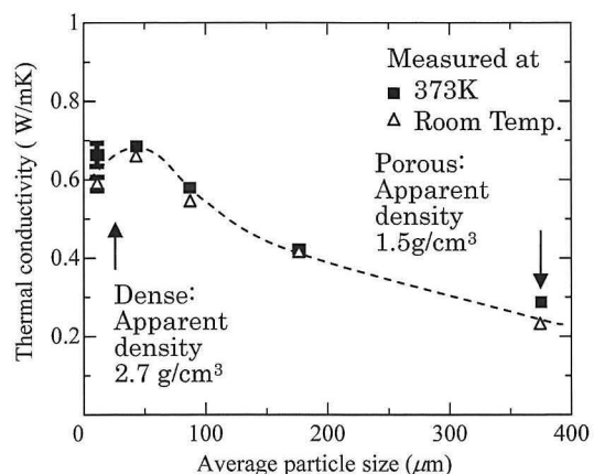
Fig.6 Change in the thermal conductivity of the solidified slag with the average particle size of original slag particles
