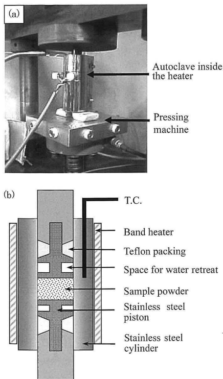
Fig.3 Apparatus for hydrothermal hot pressing (a), and schematic diagram of an autoclave (b)
