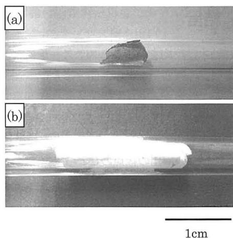
Fig.11 Change in shapes of the hydrothermally treated 63mass%SiO 2 -27mass%Na 2 O-10mass%B 2 O 3 glass particles placed in the glass tube ; (a) before, (b) after firing by gas burner
