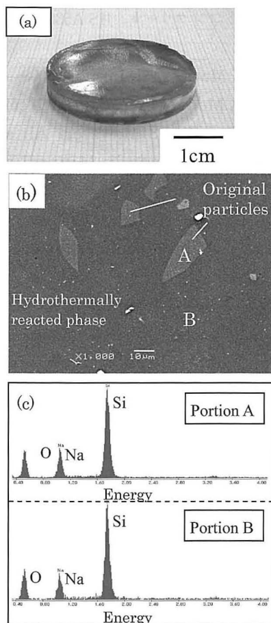
Fig.8 (a) Obtained compact of the 63mass%SiO 2 -27mass%Na 2 O-10mass%B 2 O 3 glass powder after the hydrothermal hot pressing at 523 K. (b) SEM micrograph of the hydrothermally treated 63mass%SiO 2 -27mass%Na 2 O-10mass%B 2 O 3 glass, and (c) EDX profiles for the portions A and B in (b)
