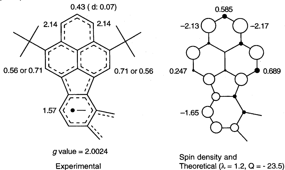
Figure 3.5.4. Experimental and theoretical hyperfine coupling constants (in G) along with spin density of 3.2^{\bullet}(-) and 3.3^{\bullet}(-) . In parentheses, a coupling constant of deuteron. Open-circle and closed-circle represent positive and negative spin density, respectively.
