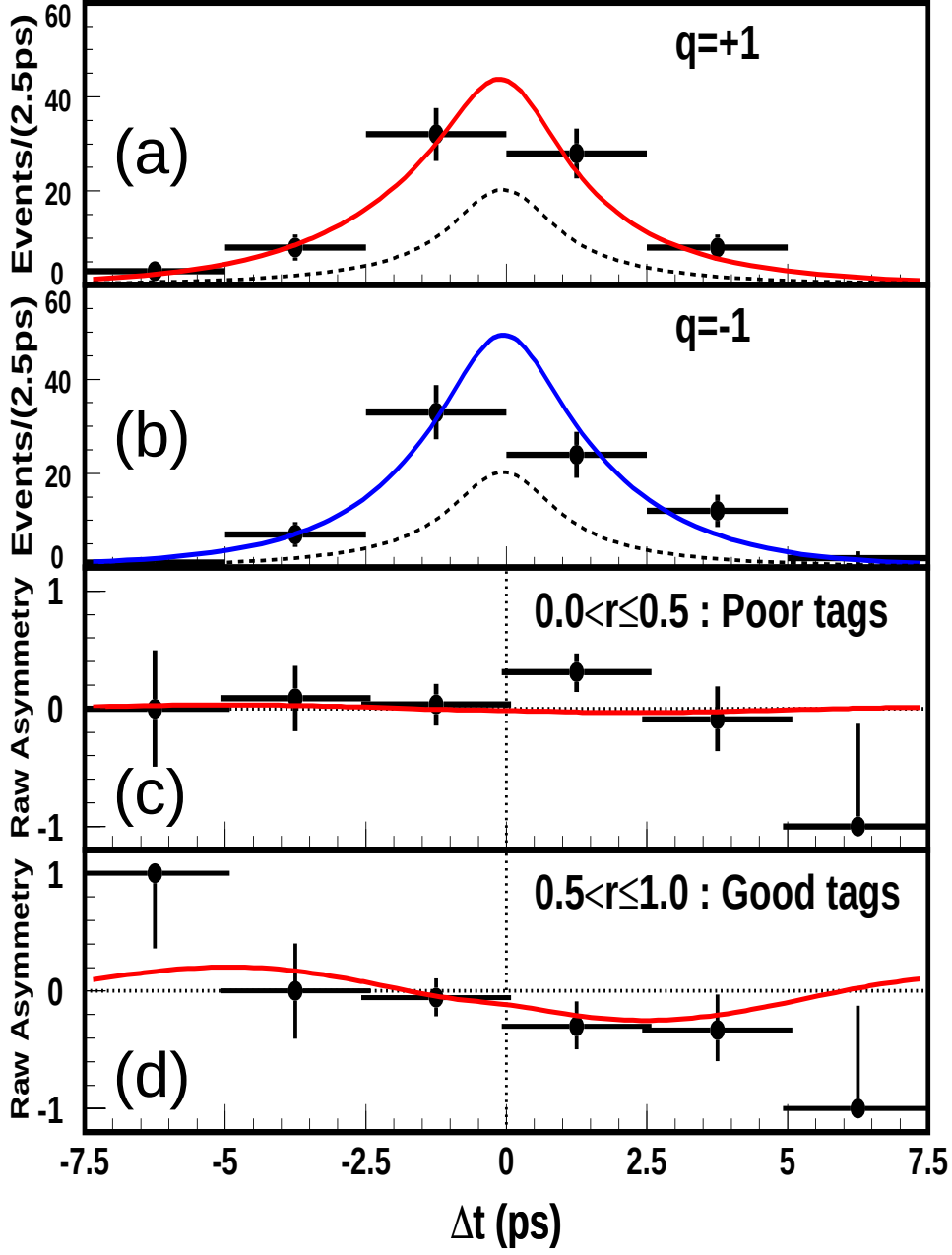
Figure 6.3: The \Delta t distributions with a 140 \text{ fb}^{-1} data sample: (a) q = +1 tagged candidates; (b) q = -1 tagged candidates; (c) time dependent CP asymmetry for 0 < r \leq 0.5 candidates; (d) time dependent CP asymmetry for 0.5 < r \leq 1.0 candidates. Filled circles with error bars show data, the solid lines show the fit results and dashed lines show the background.
