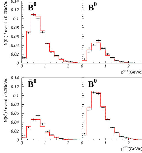
Figure C.4: The cms momentum distributions of kaon candidates for \overline{B}^0 and B^0 . The points are for the data of control samples, while the histograms with solid line and dotted line are for the EvtGen-MC and QQ-MC, respectively. The distribution of kaon cms momentum is made with a requirement on K/\pi ID to exclude the dominating pion component. Upper two figures and lower two figures are for K^- -like tracks and for K^+ -like tracks, respectively. Upper right and lower left figures contain kaons from cascade b \rightarrow c \rightarrow s transition.
