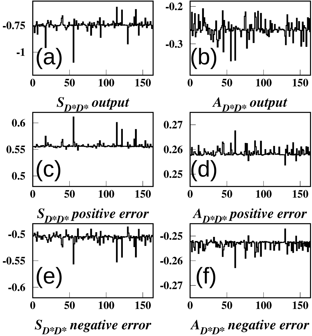
Figure 6.13: Special event scanning during CP asymmetries measurement for (a) S_{D^*+D^{*-}} output; (b) A_{D^*+D^{*-}} output; (c) S_{D^*+D^{*-}} positive error; (d) A_{D^*+D^{*-}} positive error; (e) S_{D^*+D^{*-}} negative error; (f) A_{D^*+D^{*-}} negative error. The horizontal axis shows the id of the removed event.
