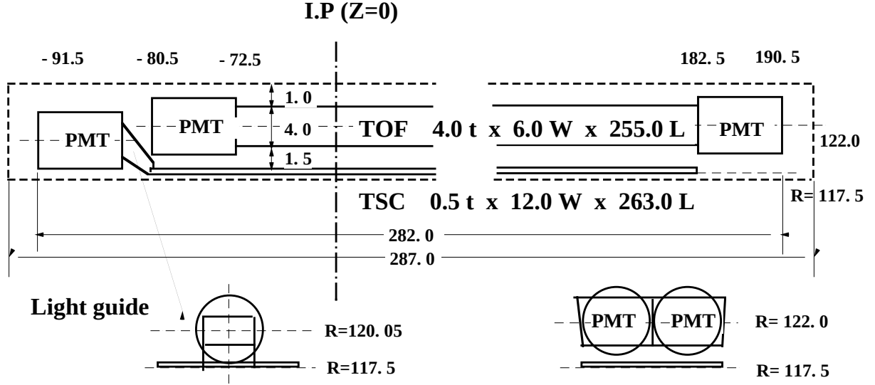
Figure 3.17: Dimensions of a TOF/TSC module.
