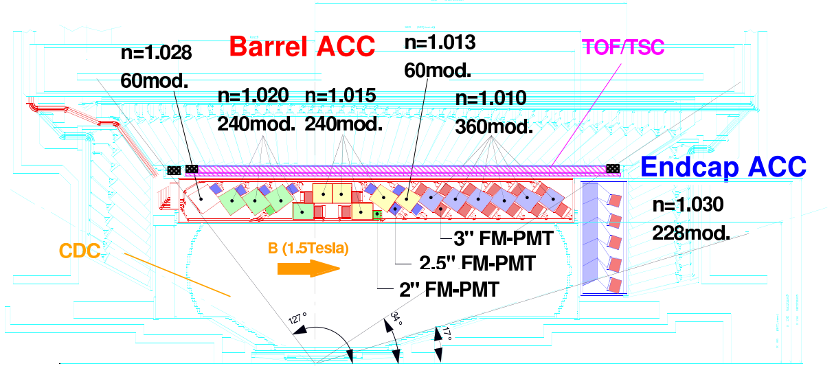
Figure 3.15: The arrangement of ACC.
