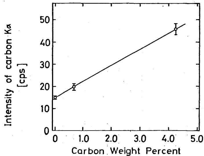
Fig.2-3 The calibration curve for carbon in electron probe micro analysis.
