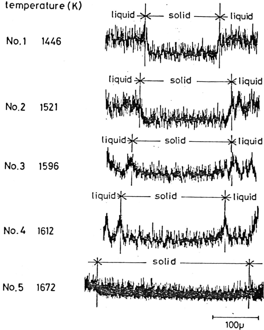
Fig.2-4 Carbon distribution in quenched specimen.
