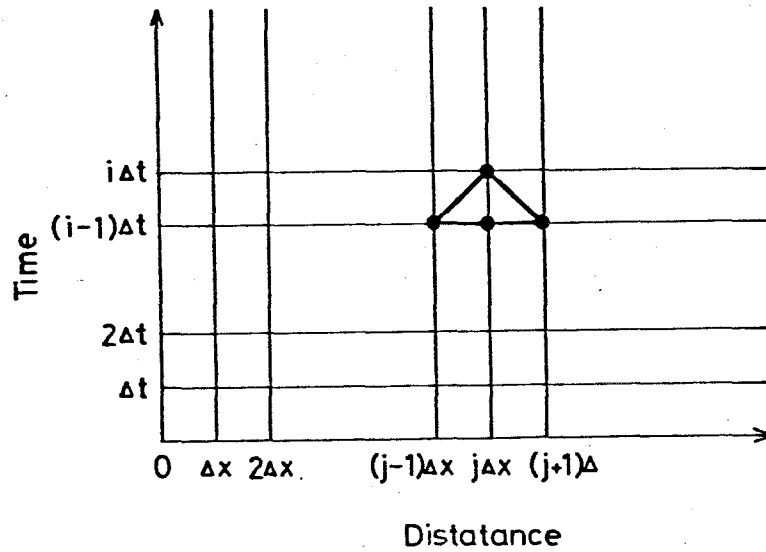
Fig.2-6 Explicit method.
