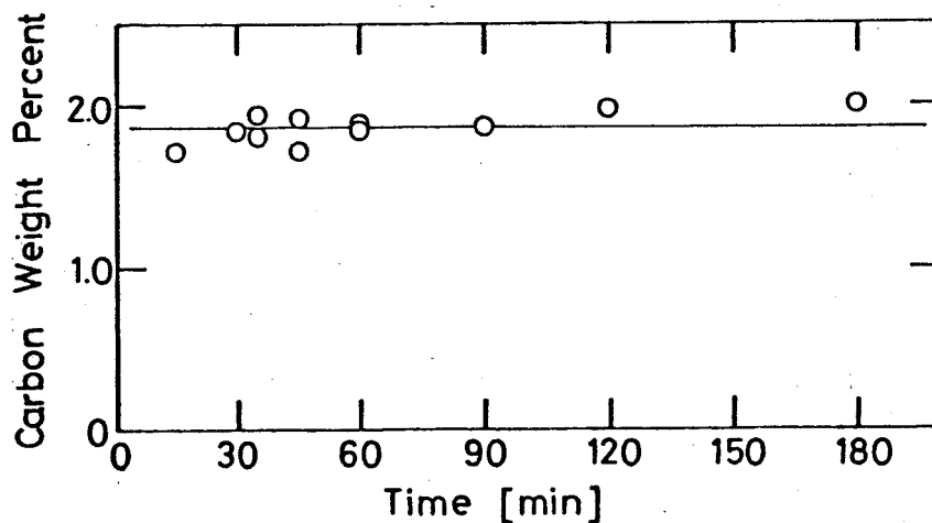
Fig.2-2 Carbon concentration in austenite of the F e – C alloy held at 1446K with equilibration time.
