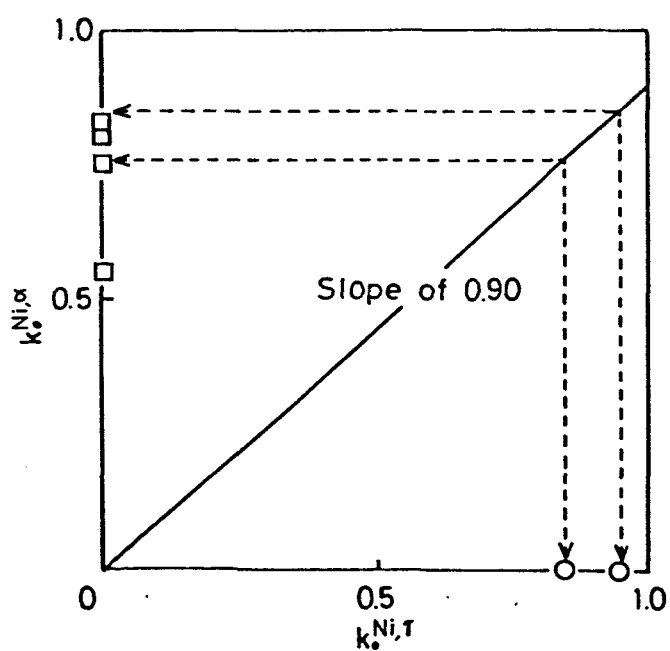
Fig. 6-9 Comparison of calculated k_0^{Ni, \alpha} / k_0^{Ni, \tau} of Ni with the experimental results.
