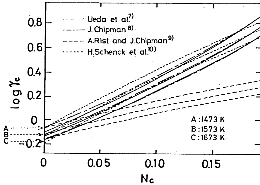
Fig.2-9 Activity coefficient of carbon in liquid iron.
