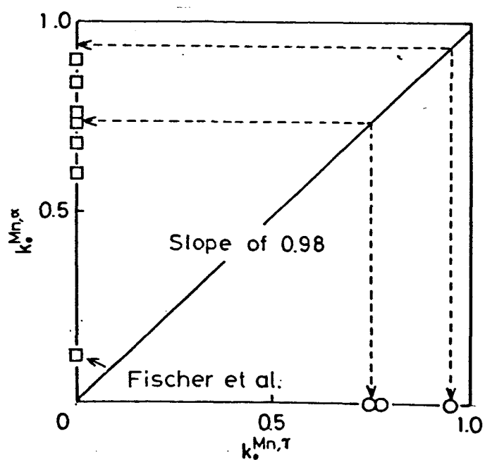
Fig. 6-10 Comparison of calculated k_0^{Mn, \alpha} / k_0^{Mn, \tau} of Mn with the experimental results.
