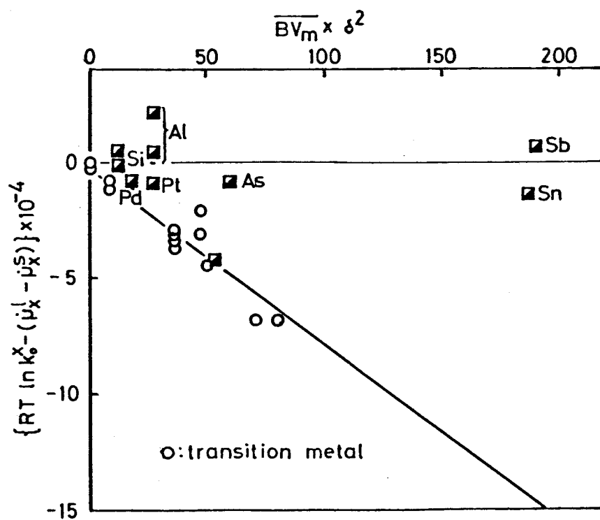
Fig.3-11 Relation between RT \ln k_0^x - (\dot{\mu}_x^l - \dot{\mu}_x^s) and \overline{BV}_m \times \delta^2 for semi-metals and noble metals as solute in iron base alloys.
