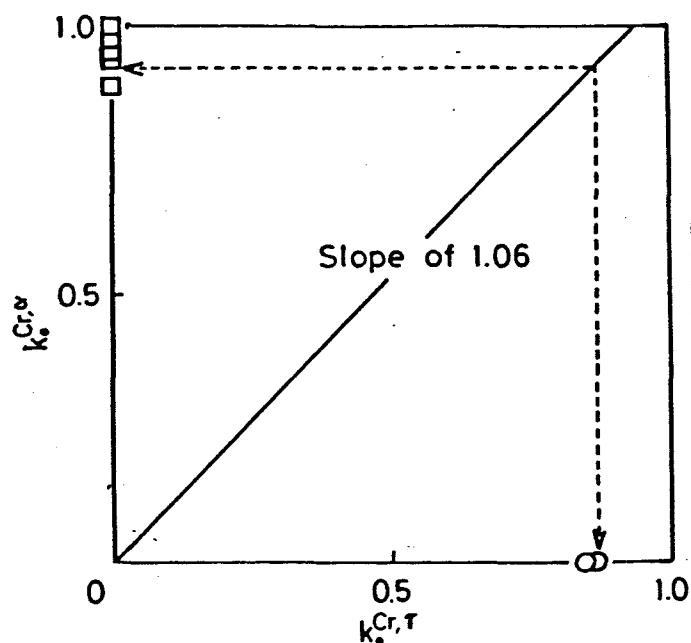
Fig. 6-8 Comparison of calculated k_0^{Cr, \alpha} / k_0^{Cr, \tau} of Cr with the experimental results.
