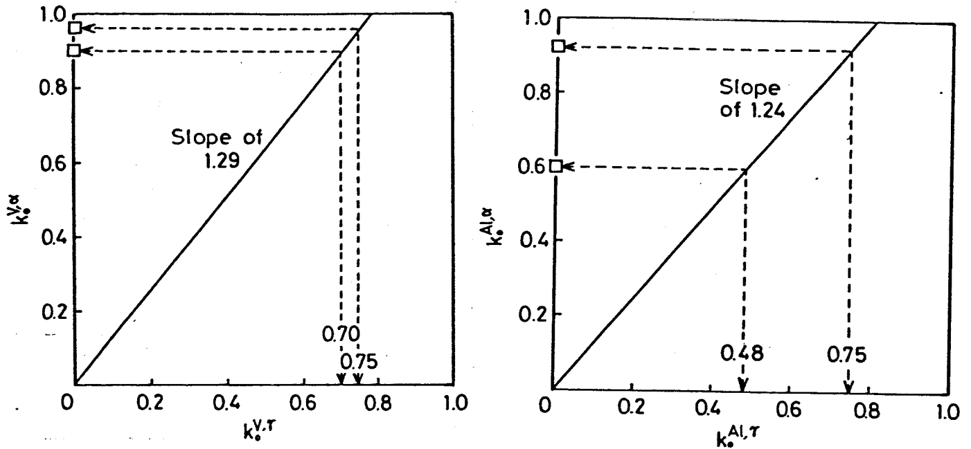
Fig.6-15 Estimation of k_0^{V,\gamma} and k_0^{Al,\gamma} from k_0^{X,\alpha}/k_0^{X,\gamma} .
