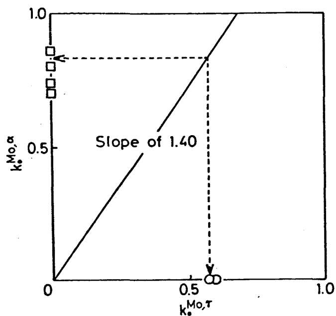
Fig. 6-7 Comparison of calculated k_0^{Mo, \alpha} / k_0^{Mo, \tau} of Mo with the experimental results.
