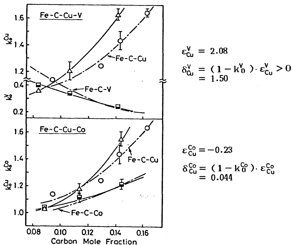
Fig.5-4 Change of the equilibrium distribution coefficients of \text{Cu} , \text{V} and \text{Co} with the concentration of \text{C} in \text{Fe}-\text{C}-\text{Cu} base systems.
