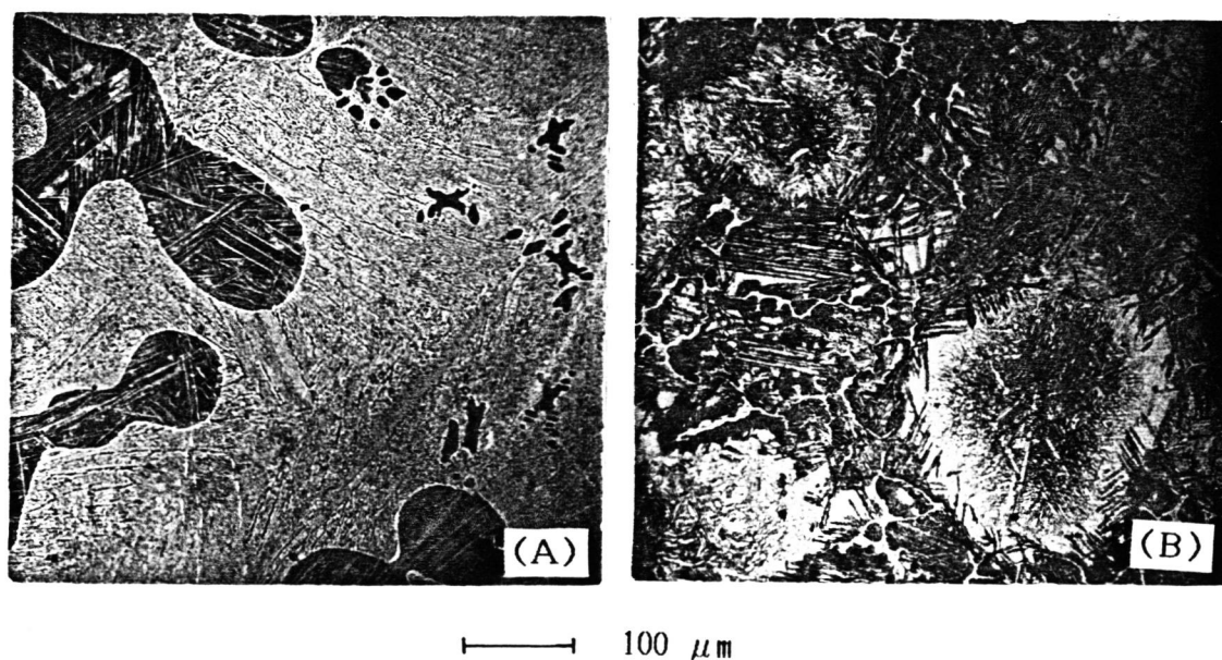
Photo.2-2 Microstructures of quenched specimens, (A) No.1 and (B) No.5.
