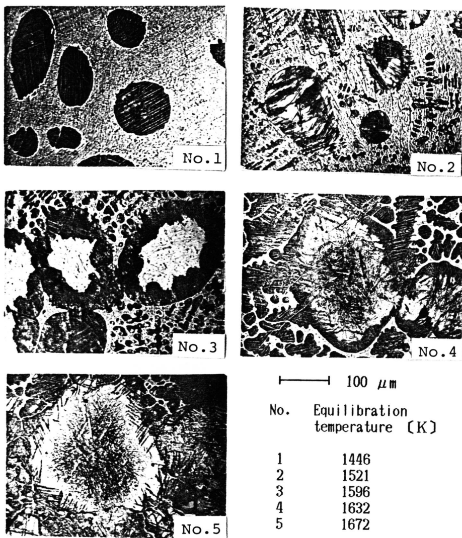
Photo.2-1 Microstructures of quenched specimens.
