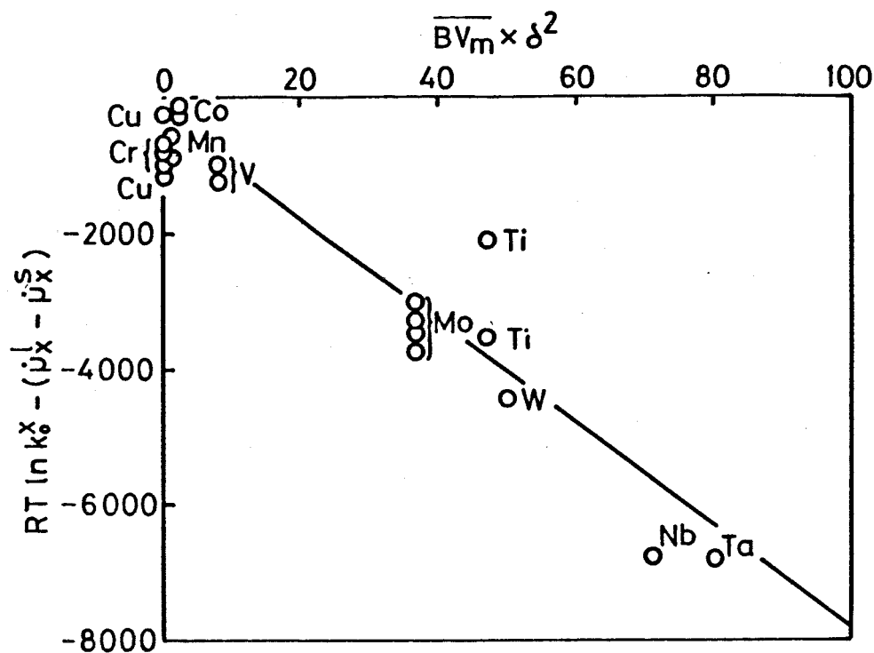
Fig.3-10 Relation between RT \ln k_0^x - (\dot{\mu}_x^l - \dot{\mu}_x^s) and \overline{BV}_m \times \delta^2 for substitutional transition elements as solute in iron base alloys.
