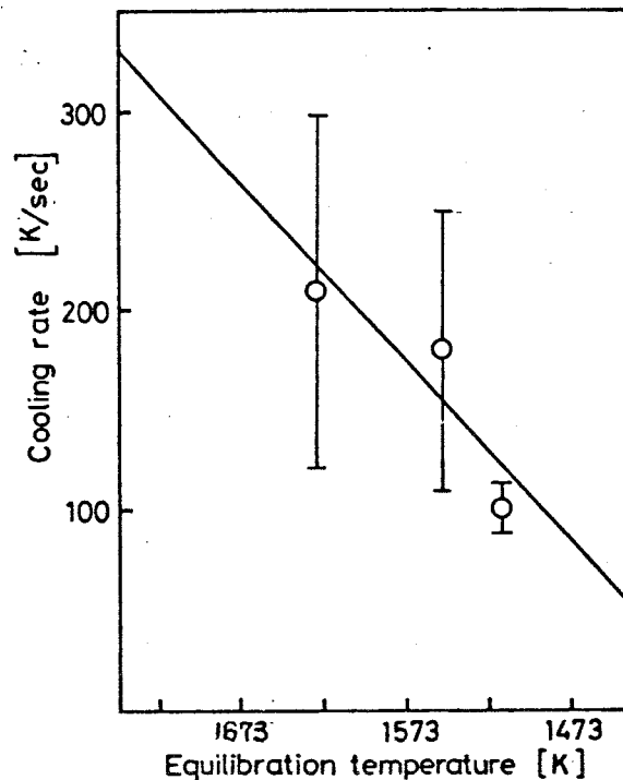
Fig.2-7 Change of cooling rates of the Fe-C alloy with equilibration temperature before cooling.
