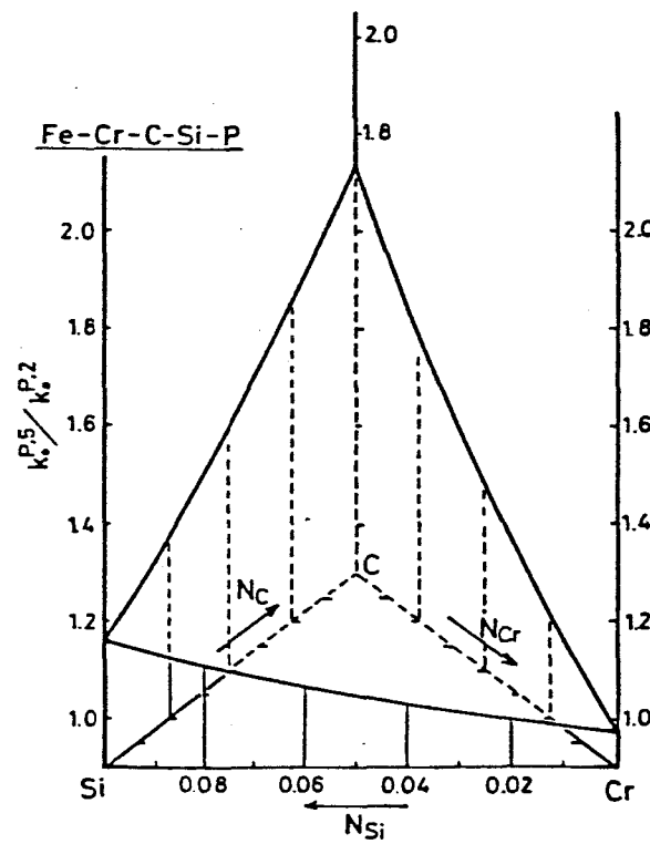
Fig.5-7 Change of D I C of P with the concentration of Cr, C and Si in chromium steels.
