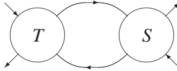
Fig. 6. Addition of tangles.
