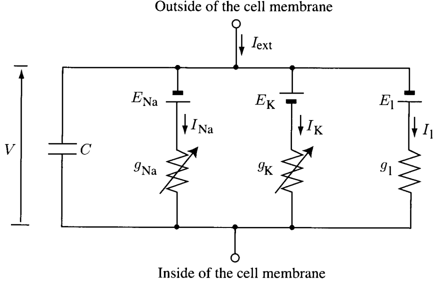
Figure 3.1: Equivalent circuit of a squid giant axon considered in the HH model.
