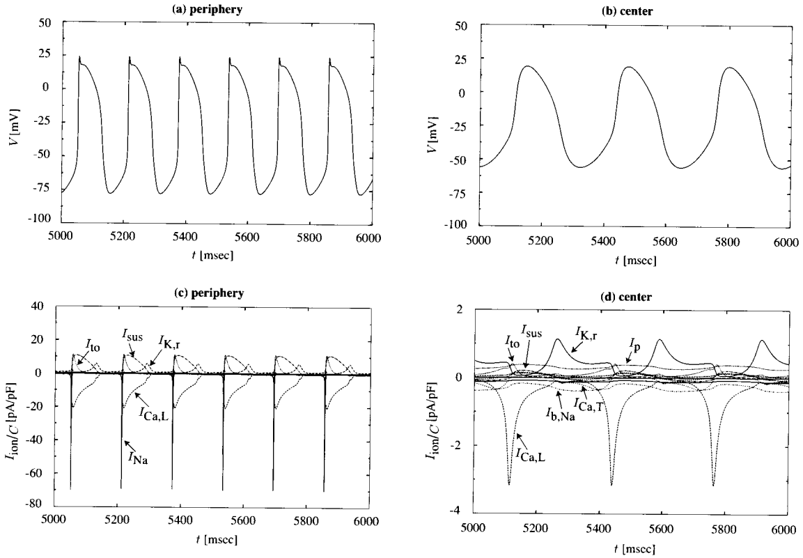
Figure 6.1: Temporal variations of (a) (b) membrane potential and (c) (d) membrane currents in normal condition ( I_{\text{ext}} = 0.0 pA, c_{\text{ion}} = 1.0 ). In the panel (c) and (d), the inward currents and outward currents are denoted by negative and positive values, respectively.
