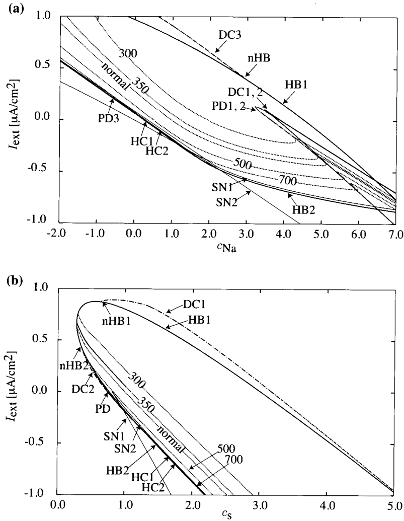
Figure 5.15: Two-parameter bifurcation diagram as for the the ion channel current I_{ion} (ion = Na and s) and the external current I_{ext} .
