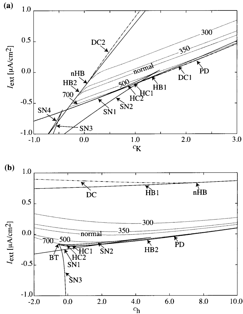
Figure 5.16: Two-parameter bifurcation diagram as for the ion channel current I_{ion} (ion = K and h) and the external current I_{ext} .
