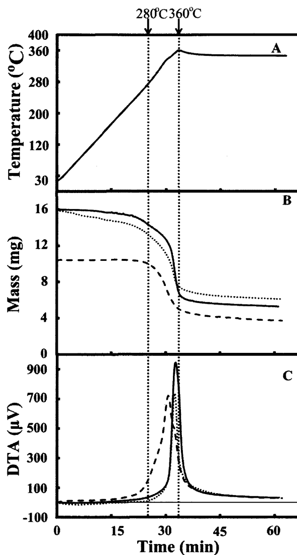
Fig. 4. 3. TG and DTA analysis of 60% triolein and total lipids extracted from oleaginous fungi. Furnace temperature (A) was linearly increased from 30 to 360 °C and isothermally held at 360 °C for 30 min. TG (B) and DTA (C) curves were obtained using about 15 mg of total lipids extracted from M. alpina IFO32281 (closed line) and M. alliacea YN-15 (dotted line) or about 10 mg of 60% triolein (broken line). The temperature range between 280 and 360 °C is indicated by two vertical dotted lines. The zero baseline for the DTA curves (0 \mu\text{V} ) is indicated by a horizontal line.
