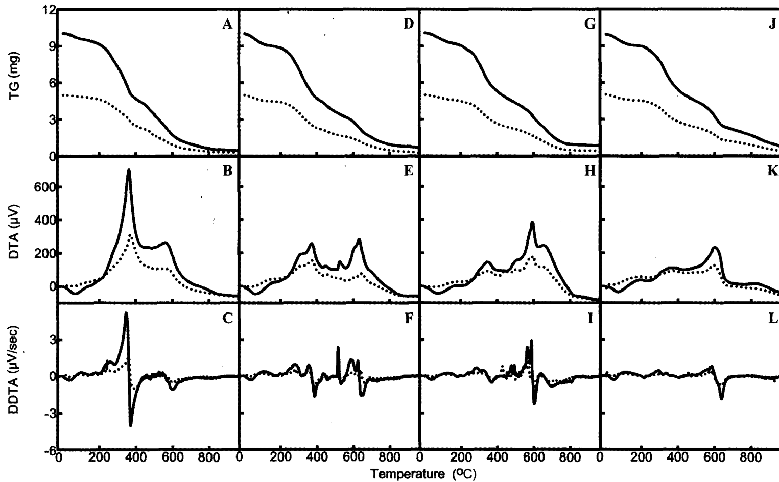
Fig. 3. 2. TG, DTA, and differential DTA (DDTA) curves for microbial samples of 5 mg (broken line) and 10 mg (closed line). The microorganisms examined were M. alpina IFO32281 (A, B, and C), R. opacus B-4 (D, E, and F), S. cerevisiae (G, H, and I), and E. coli JM109 (J, K, and L).
