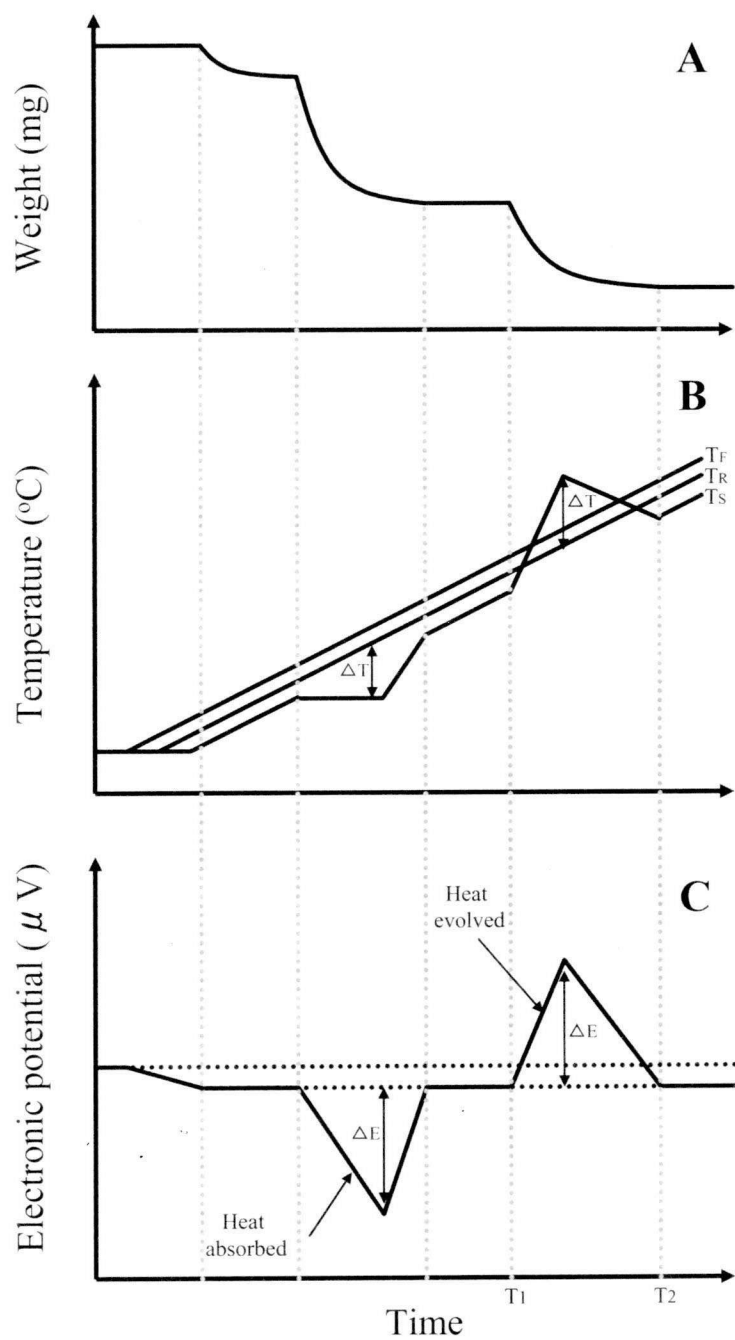
Fig. 1 Principle of TGA and DTA measurements
