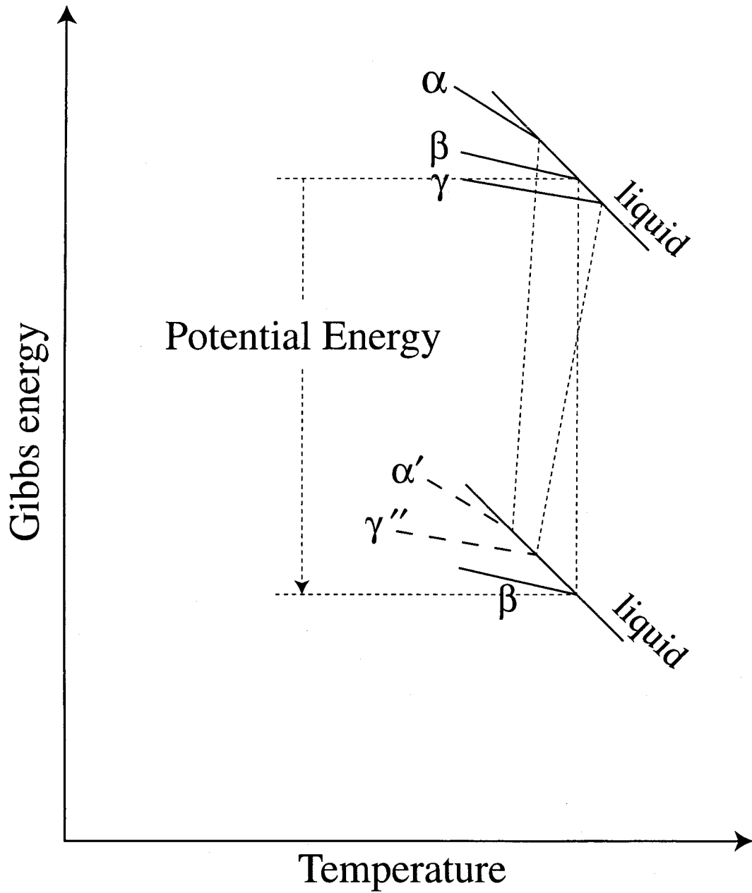
Fig. 4.25: Schematic illustration of the Gibbs energies of the bulk phases formed at the position where the \gamma -beta is most stable. See the details in the text.
