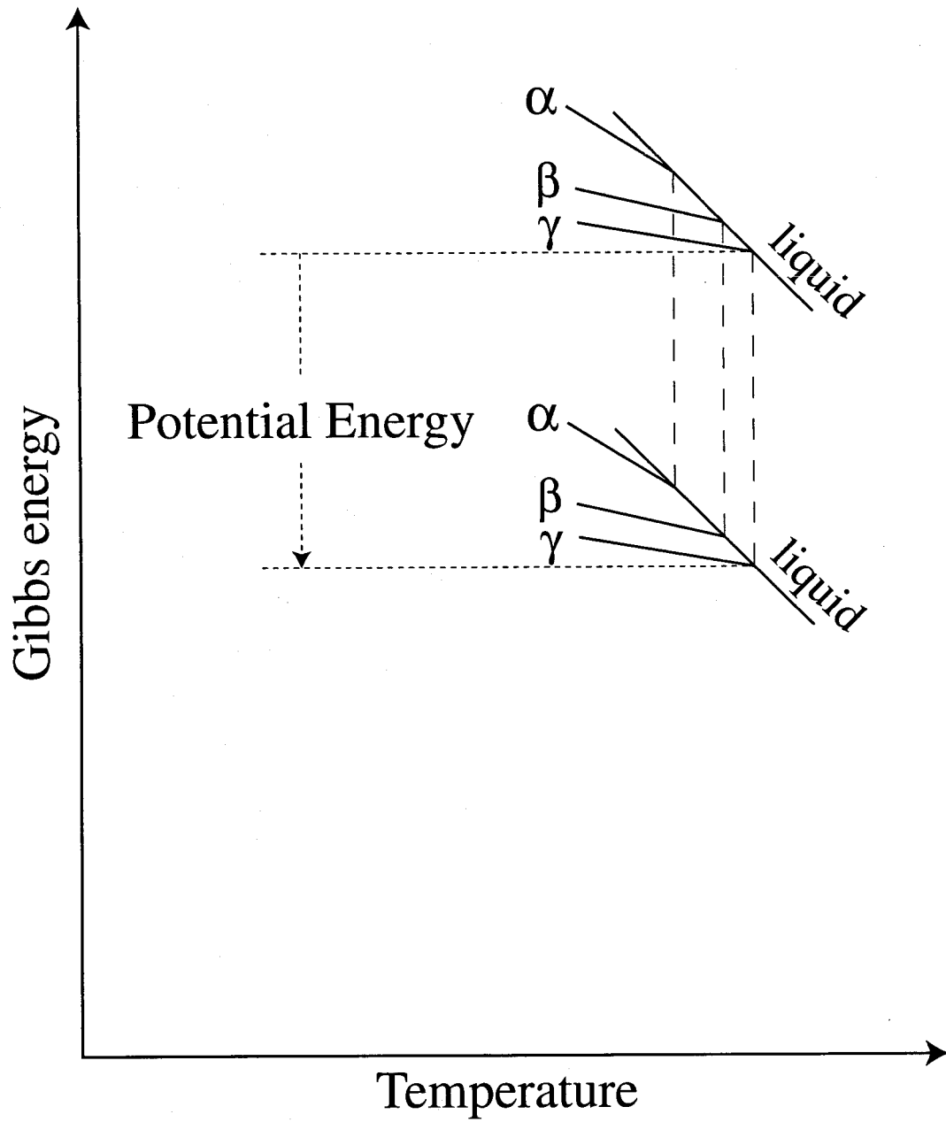
Fig. 4.26: Schematic illustration of the Gibbs energies of the bulk phases formed at the position where the \gamma -phase is most stable. See the details in the text.
