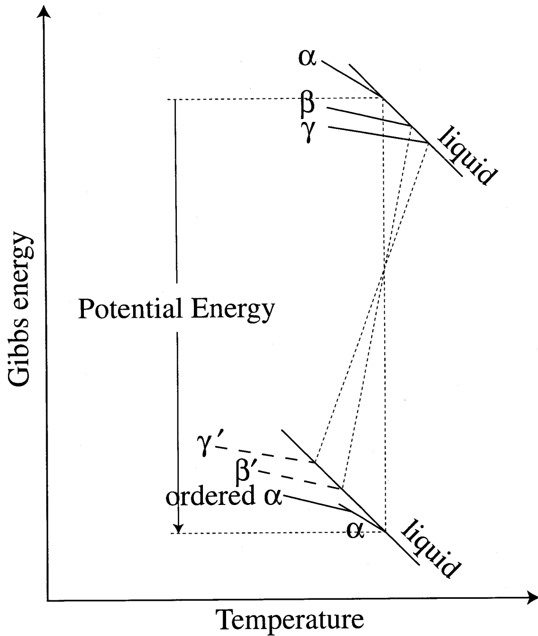
Fig. 4.24: Schematic illustration of the Gibbs energies of the bulk phases formed at the position where the \alpha -phase is most stable. See the details in the text.
