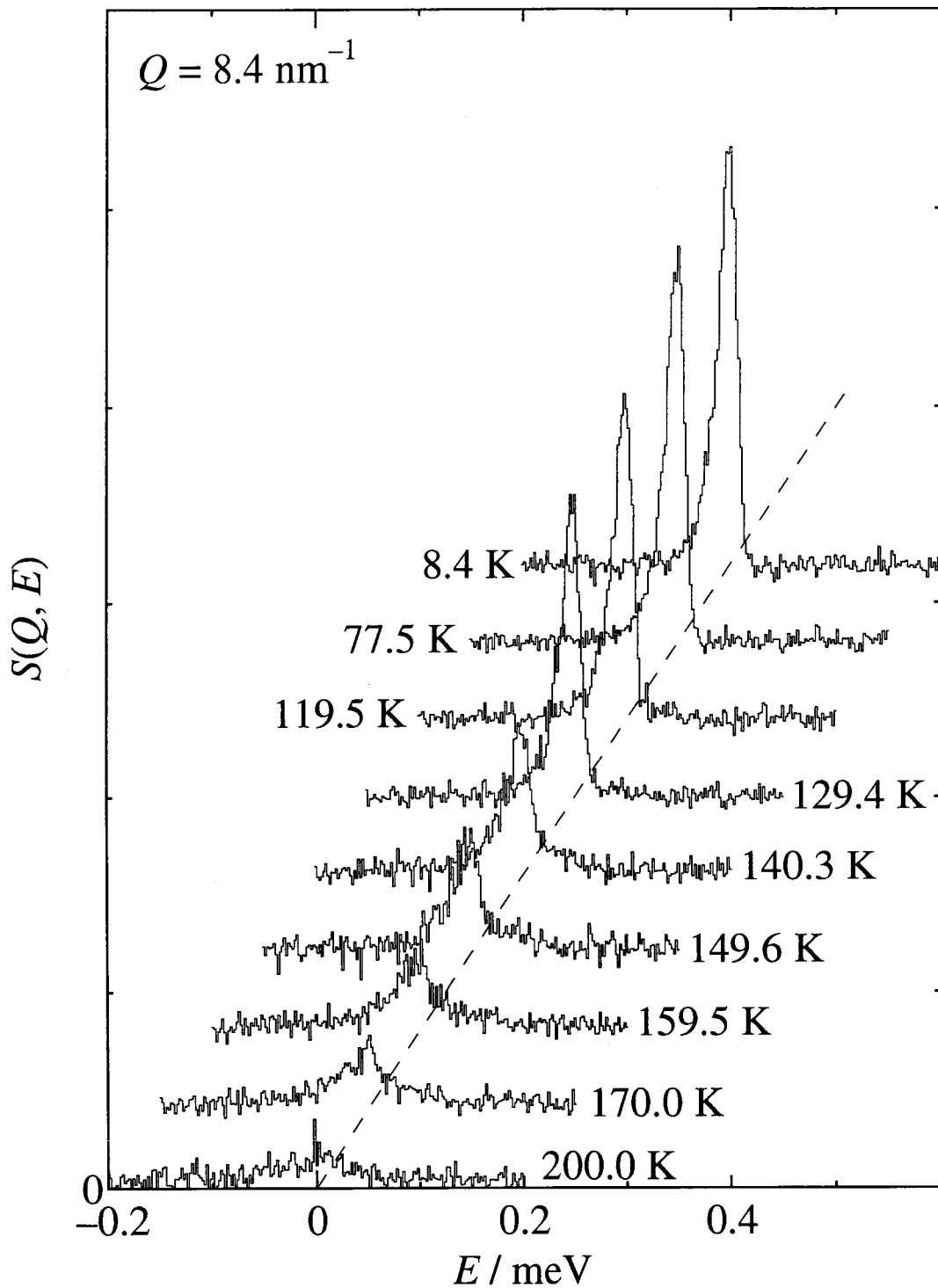
Fig. 3.8: Neutron scattering spectra obtained on LAM-80ET for TMS/graphite at \theta = 1.55 at Q = 8.4 \text{ nm}^{-1} with an instrumental resolution \Delta E = 15 \mu\text{eV} . The background contribution has already been subtracted.
