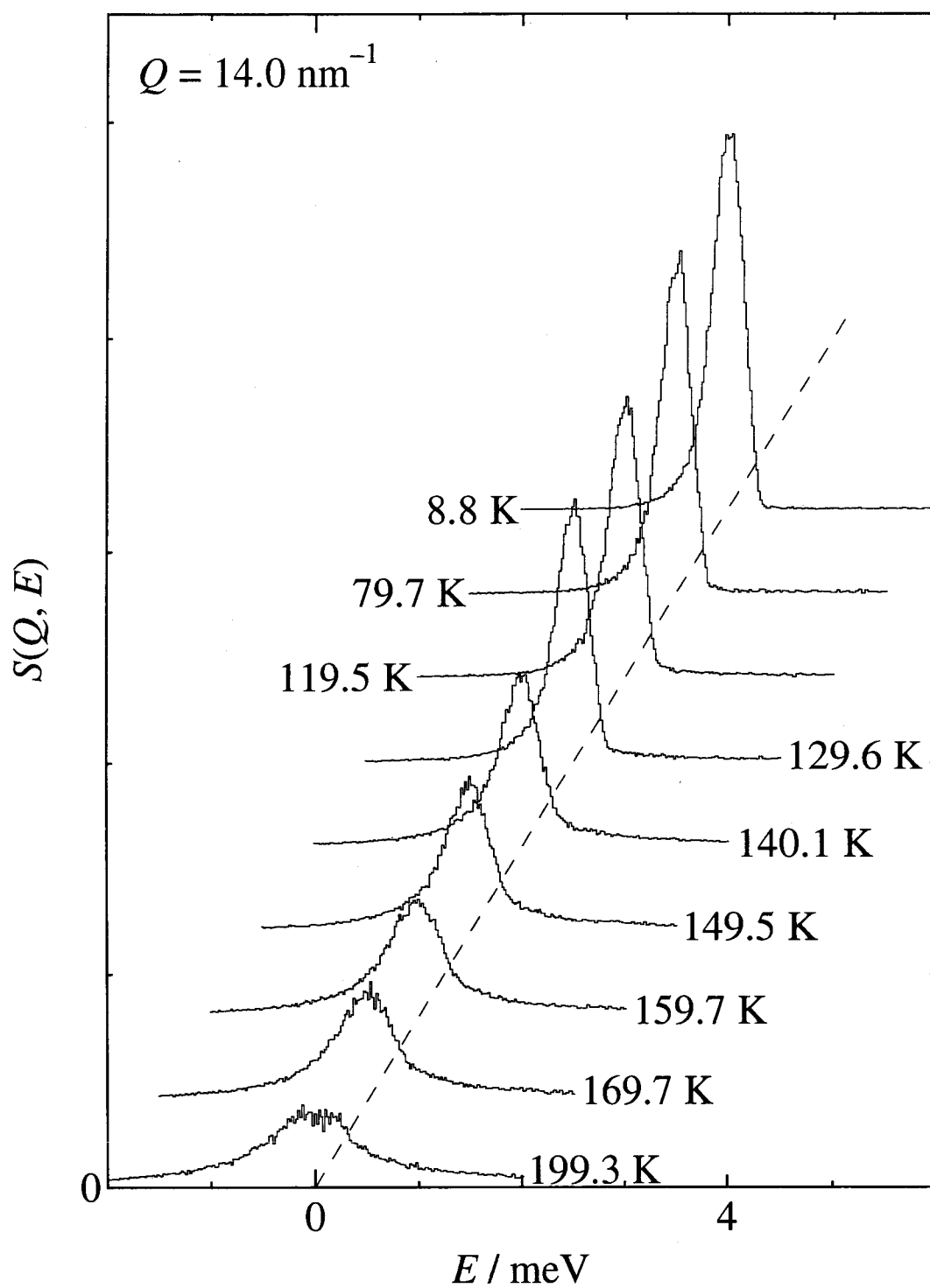
Fig. 3.10: Neutron scattering spectra obtained on LAM-40 for TMS/graphite at \theta = 1.54 at Q = 14.0 \text{ nm}^{-1} with an instrumental resolution \Delta E = 200 \text{ } \mu\text{eV} . The background contribution has already been subtracted.
