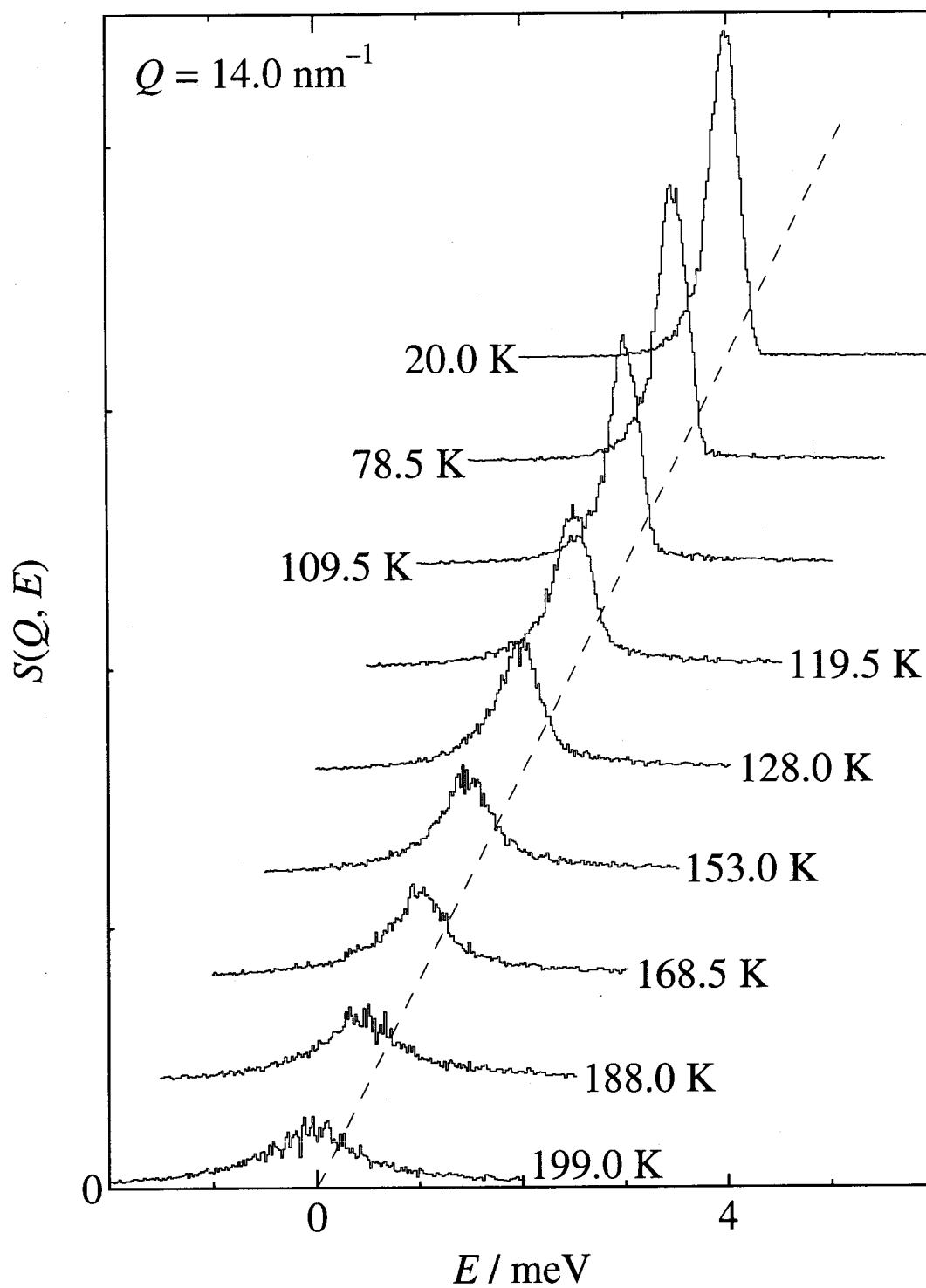
Fig. 3.5: Neutron scattering spectra obtained on LAM-40 for TMS/graphite at \theta = 1.02 at Q = 14.0 \text{ nm}^{-1} with an instrumental resolution \Delta E = 200 \text{ } \mu\text{eV} . The background contribution has already been subtracted.
