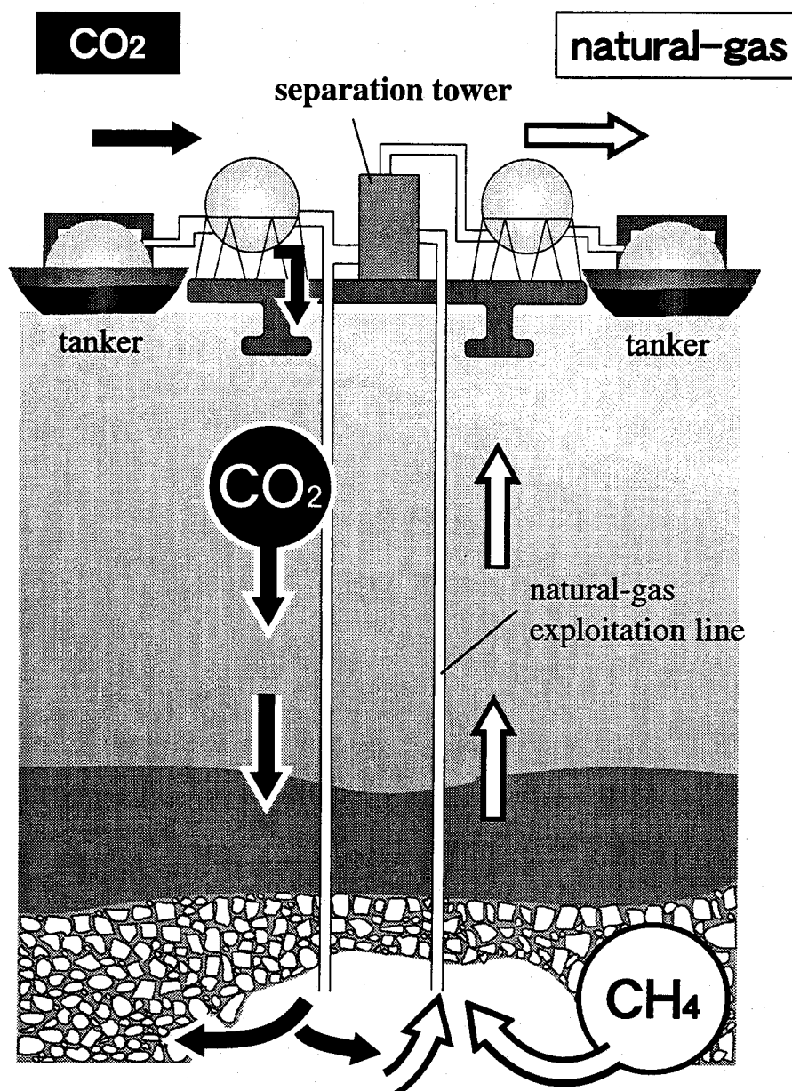
Fig. 6 Schematic illustration of the simultaneous process for the natural-gas exploitation and \text{CO}_2 isolation
