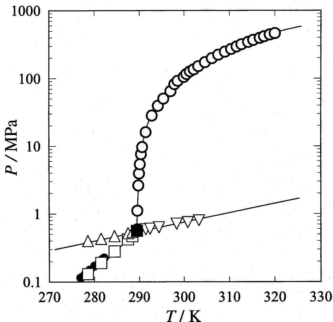
Fig. 4-1 Three-phase coexisting curves of the cyclopropane hydrate system: O, H+L_1+L_2 in the present study; □, H+L_1+G in the present study; ●, Hafemann and Miller(1969); Δ, H+L_2+G in the present study; ▽, L_1+L_2+G in the present study; ■, quadruple point
