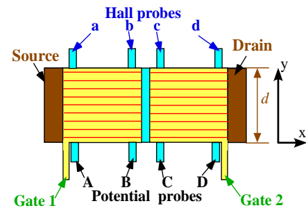
Figure 9. Top view of the tunneling device. There is a potential barrier in the central part (blue region) of the device. Horizontal red lines indicate the centres of y-direction for Landau orbitals with L = 0 . The interval between the red lines is enlarged to bring them into view. The width of the device is described by the symbol d .
