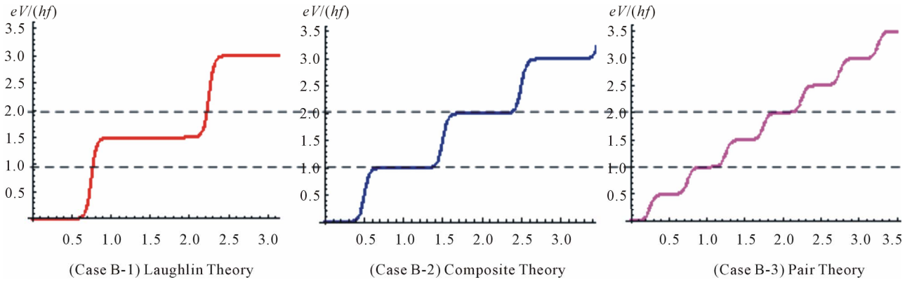
Figure 7. Behaviours of voltage steps for three theories at the filling factor 2/3 . The horizontal axis indicates the electric current (arbitrary unit).
